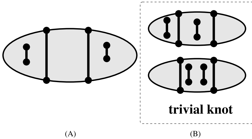
Fig. 6. Ribbon singularities for ribbon number two knots.
