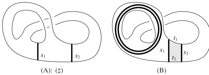
Fig. 3. Genus one surface F and the intersection with S .
