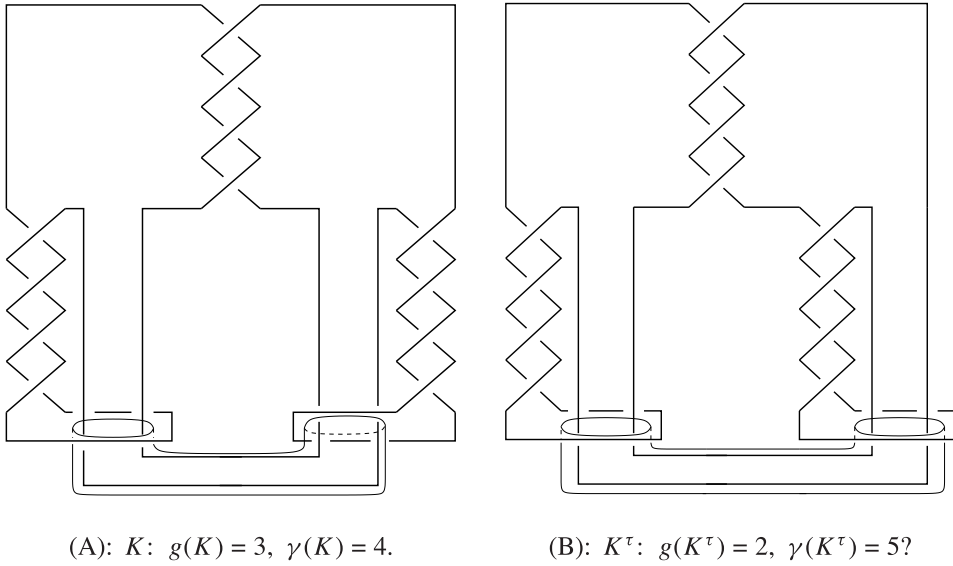
Fig. 2. Candidate of mutative knots of distinct crosscap numbers.
