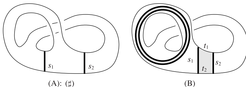
Fig. 3. Genus one surface F and the intersection with S .
