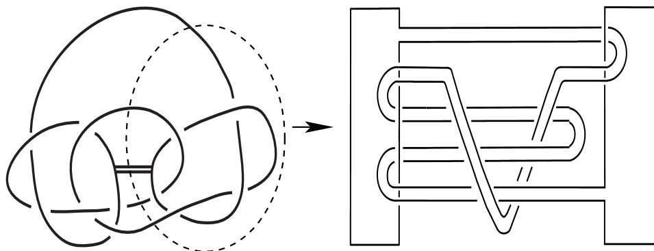
Fig. 7. The Kinoshita-Terasaka knot.
