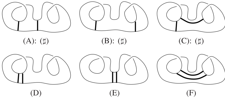
Fig. 4. Two arcs on a non-orientable surface with crosscap number two.
