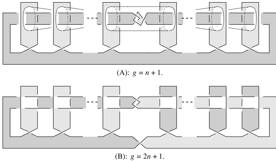
Fig. 1. Mutative knots of distinct genera.
