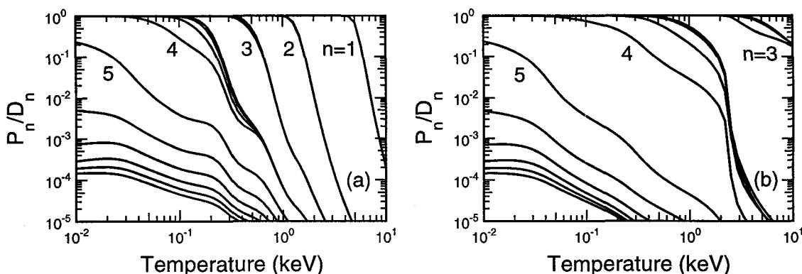
Figure 2.10: Electronic population of the average ion model divided by the statistical weight of the level. (a) Local thermodynamic equilibrium (LTE). (b) Collisional radiative equilibrium (CRE). l -splitting effect is more important in the CRE than in the LTE.
