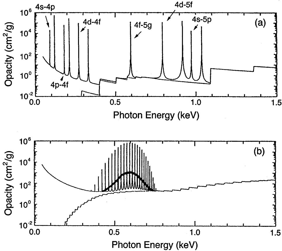
Figure 2.13: Opacity of the gold plasma in the CRE where the electron temperature is 200 eV, and the density 0.01 g/cm 3 . (a) Simple Lorentzian line profile. (b) Line group of the 4f - 5g transition composed of lines from different charge states. The thick line profile corresponds to the Gaussian profile, the half width of which is determined by the standard deviation of the line group.
