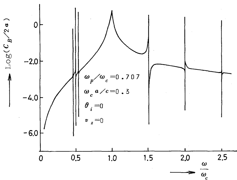
(b) \Omega/\omega_c = 0.5
