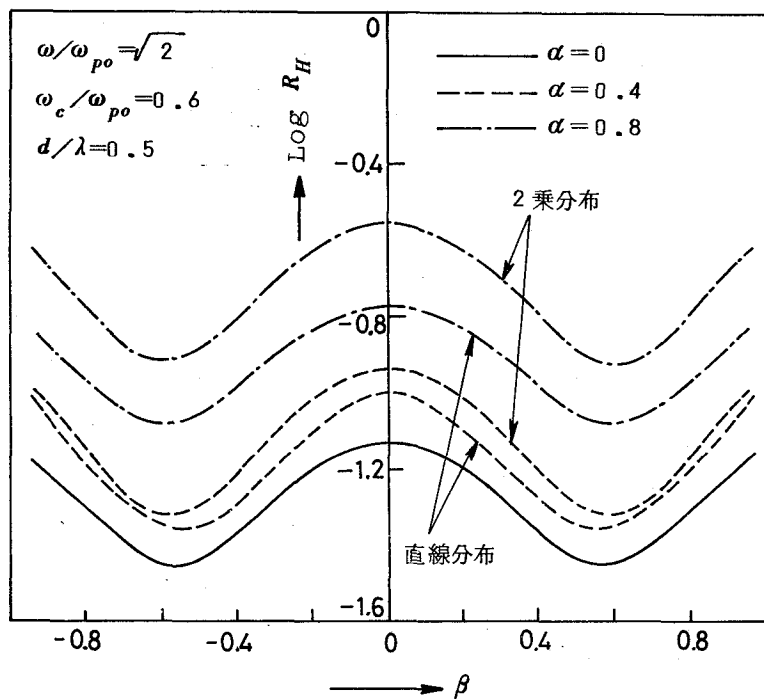
(a) \theta_i = 0
