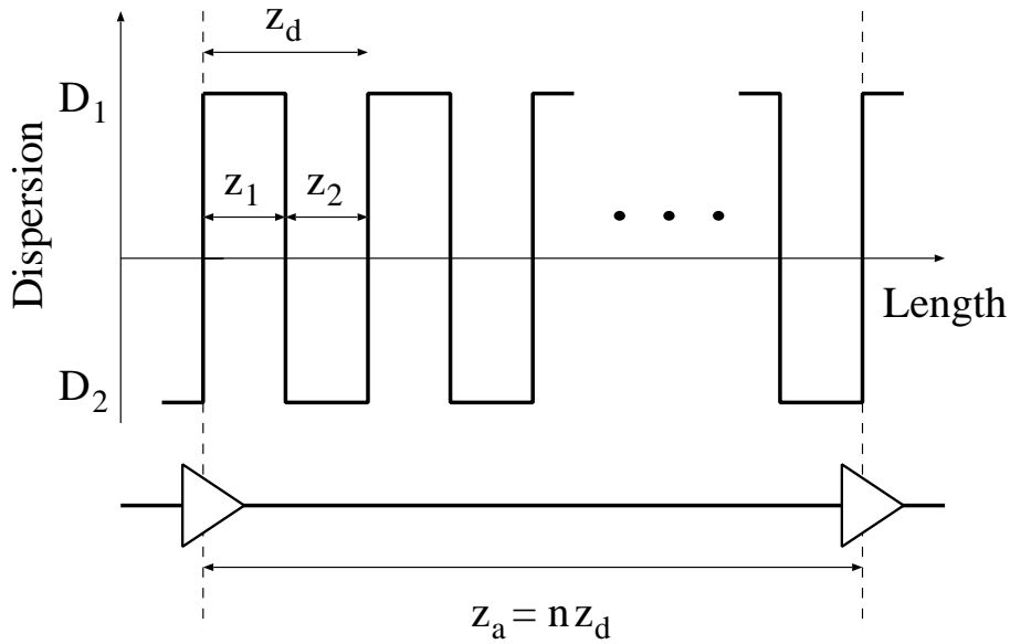
Figure 4.2: Densely dispersion managed system.
