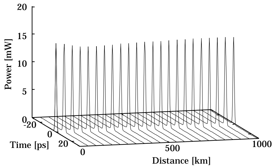
Figure 4.6: Propagation of DDMS in the profile shown in Fig. 4.5.
