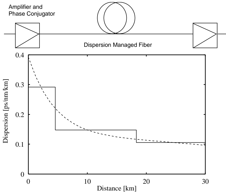
Figure 5.4: Dispersion profile. Solid: stepwise approximation. Dashed: (5.9).
