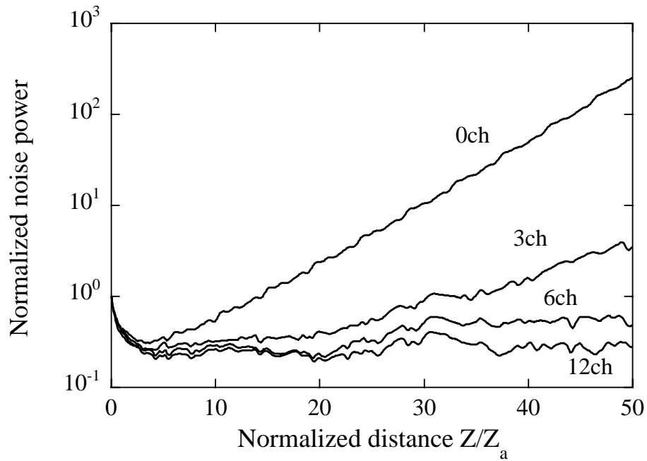
Figure 5.6: The normalized noise power as a function of distance for the several number of wavelength channels copropagating with the signal.
