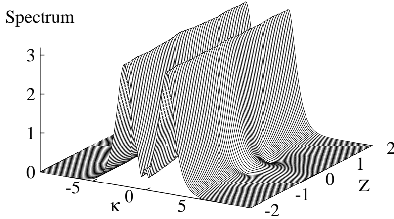
Figure 3.1: Spectrum of two colliding solitons in a lossless fiber. Two solitons collide at Z = 0 in time domain. The channel spacing \Delta B = 4.0 .
