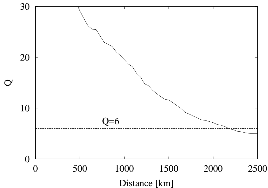
Figure 4.7: The Q factor versus transmission distance for 160 Gbit/s DDMS system with GVD profile shown in Fig. 4.5.
