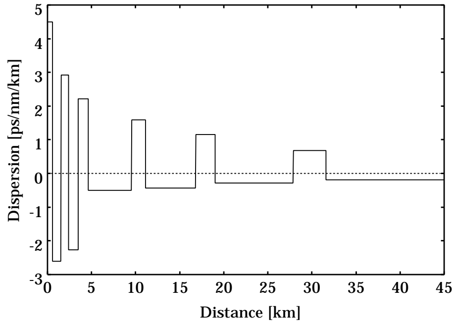
Figure 4.5: An example of dispersion profile in DDMS system.
