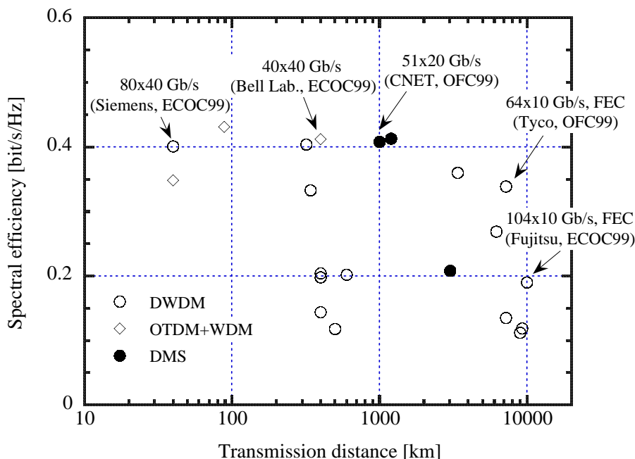
Figure 6.1: Spectral efficiency versus transmission distance in recent experimental results shown in Fig. 1.1. Total capacities are denoted as the number of wavelength channels times the bit-rate per single channel.
