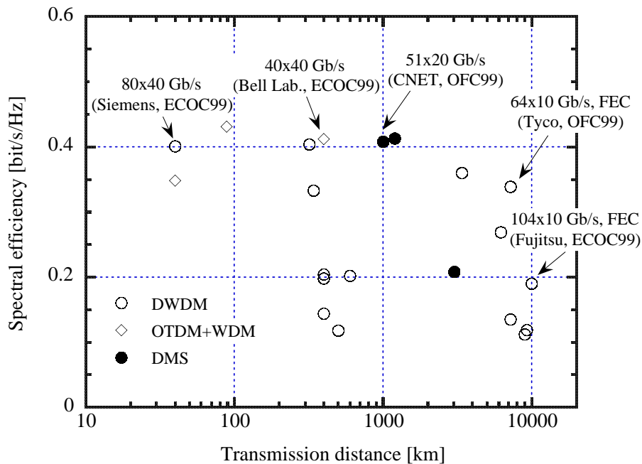
Figure 6.1: Spectral efficiency versus transmission distance in recent experimental results shown in Fig. 1.1. Total capacities are denoted as the number of wavelength channels times the bit-rate per single channel.
