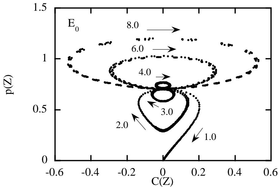
Figure 2.6: Poincaré maps for the solutions of (2.19a) and (2.19b) with several values of E_0 and the fixed initial condition p(0) = 1/\sqrt{2} and C(0) = 0 .
