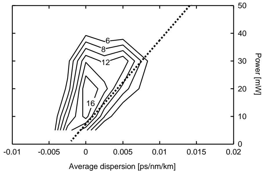
Figure 4.4: Contour map of Q values measured for 160 Gbit/s DDMS transmission over 2,000 km with variable launched power. GVD profile has a variable \langle D \rangle with fixed DM strength of S = 1.6 .
