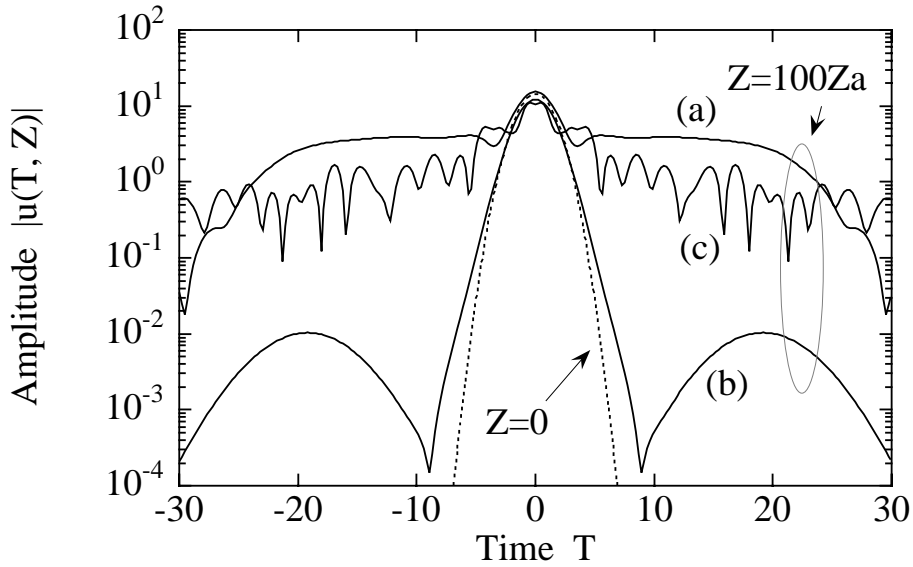
Figure 5.1: Waveforms of a DM soliton at Z = 0 (dotted line) and Z = 100Z_a (solid lines). (a) With guiding filter ( \delta = 0.161 , \beta = 0.6 ), (b) With guiding filter and nonlinear gain ( \delta = 0.0 , \beta = 0.6 , \gamma_1 = 4.6 \times 10^{-2} , \gamma_2 = -1.6 \times 10^{-3} ), (c) Without any control.
