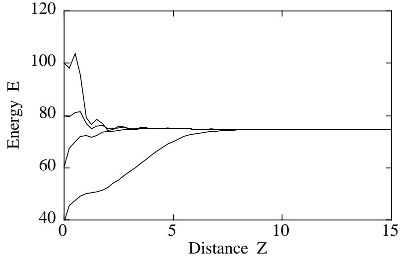
Figure 5.2: Acquisition of the steady state energy E by guiding filter and nonlinear gain. The same parameters are used as (b) in Fig. 5.1. E(0)=40, 60, 80, 100 .
