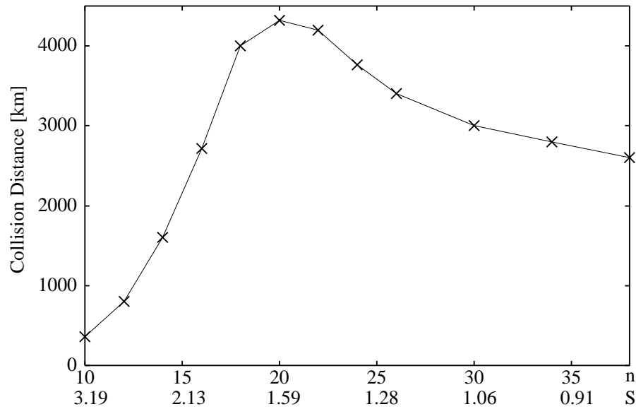
Figure 4.3: Dependence of collision distance on n (and corresponding S parameter). A pair of solitons, whose pulse width is set to be constant (2 ps), are initially separated by 6.25 ps.
