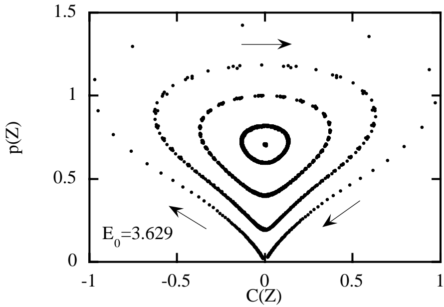
Figure 2.5: Poincaré maps for the solutions of (2.19a) and (2.19b) with several values of p(0) and C(0) and the fixed energy E_0 = 3.629 .
