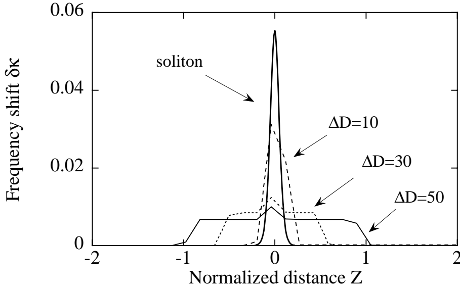
Figure 3.4: Collision-induced frequency shift of a DM soliton and a classical soliton versus normalized distance. Here the classical soliton propagates in a fiber with uniform dispersion equivalent to the averaged value of the dispersion profile.
