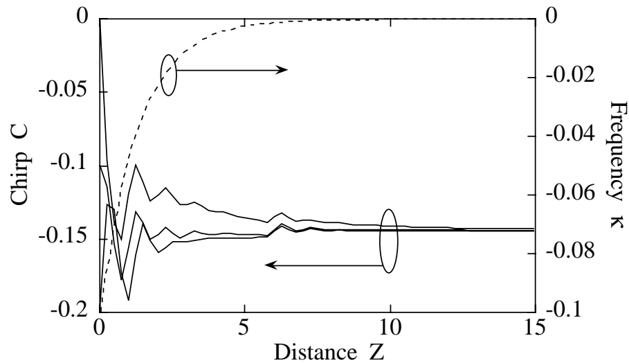
Figure 5.3: Acquisition of the steady state frequency \kappa and chirp C by guiding filter and nonlinear gain. The same parameters are used as (b) in Fig. 5.1. \kappa(0) = -0.1 , and C(0)=-0.2, -0.1, 0 .
