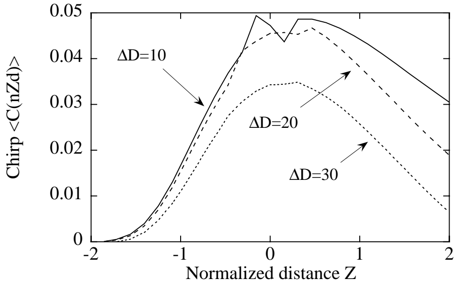
Figure 3.3: The evolution of chirp C at every midpoint of the anomalous GVD segment of the dispersion profile. The initial channel spacing is the same as Fig. 3.2.
