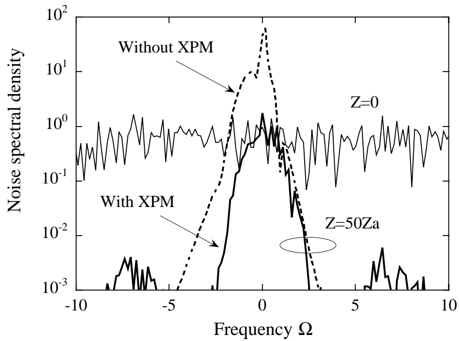
Figure 5.7: The noise spectral densities at Z = 0 and Z = 50Z_a .
