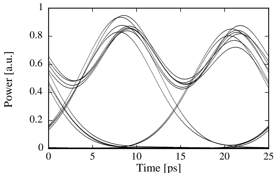
Figure 5.5: Received eye diagram formed from 32 bits data detected by electrical filter with 42 GHz bandwidth.
