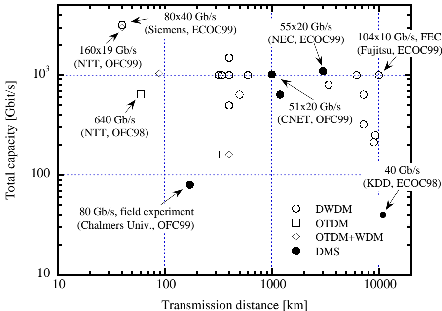
Figure 1.1: Recent experimental results of high-speed optical transmissions. Total capacities are denoted as the number of wavelength channels times the bit rate per single channel.
