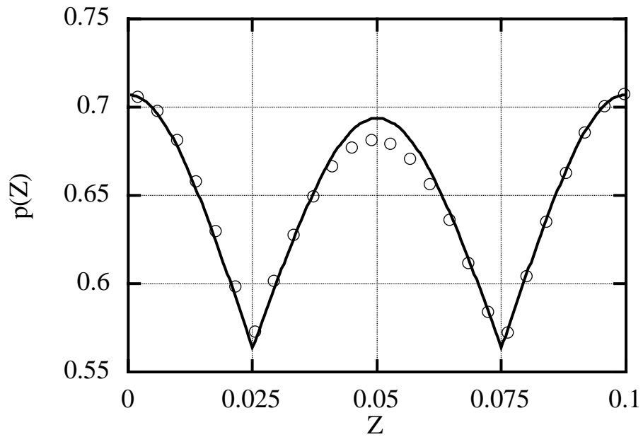
Figure 2.2: The evolution of p(Z) obtained by solving (2.19a) and (2.19b) (solid line) and by a direct numerical simulation of (2.1) with the same initial condition (dots).
