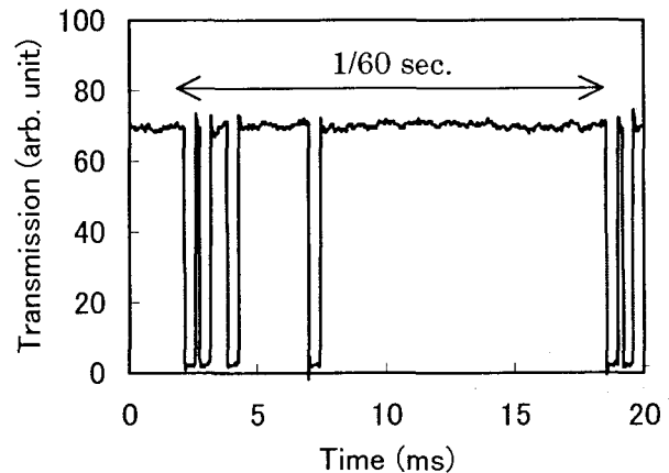
Fig.2 Optical response in 4bits TD operation.
