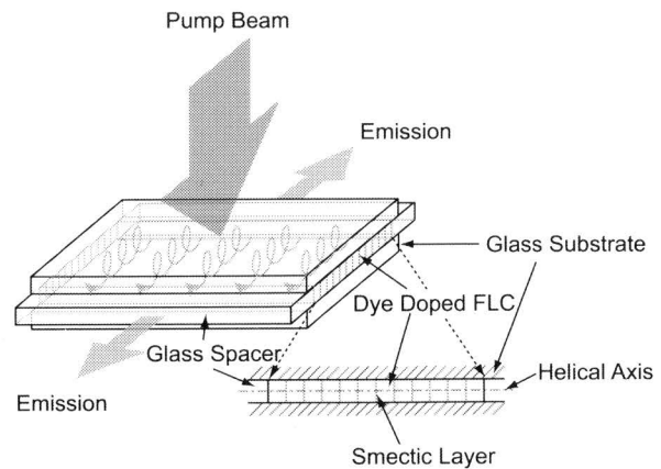
Fig.1. A cell configuration of waveguide laser. The waveguide laser output beam is emitted through a glass spacer.
