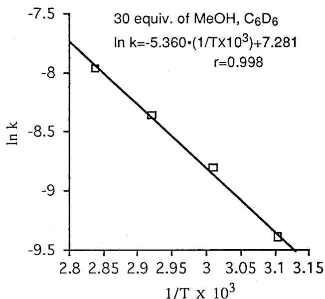
Logarithms of Rate Constants in the Reaction of 1a with 30 equiv. of Methanol in C 6 D 6 .
