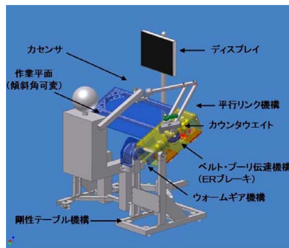
図 4-36 PLEMO System
