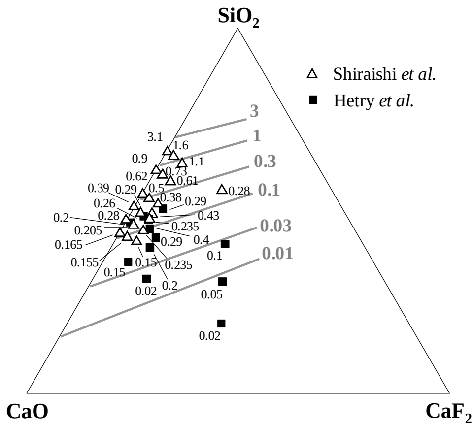
Figure 14 Viscosity (Pa·s) of molten \text{SiO}_2 -CaO- \text{CaF}_2 (mass%) at 1873K 50,51)
