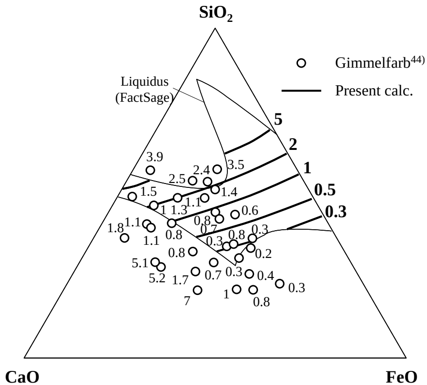
Figure 11 Viscosity (Pa·s) of \text{SiO}_2 - \text{CaO} - \text{FeO} -20 \text{Al}_2\text{O}_3 system (mass%) at 1623 K.
