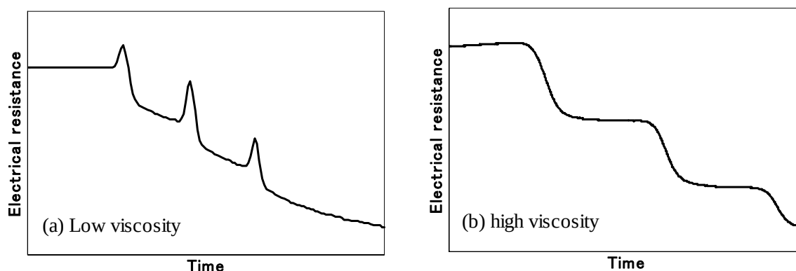
Figure 6 Schematic examples of the change in electric resistance with time Metororz aqueous solutions with (a) low and (b) high viscosity.
