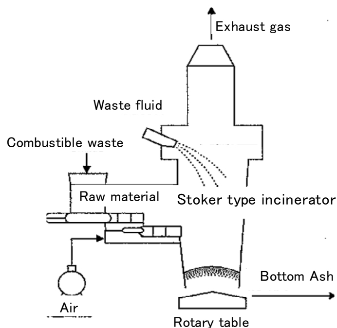
Figure 5 The general chart of the stoker type incinerator
