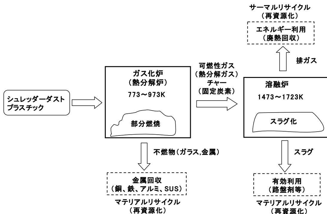
Figure 9 Principle of the gasification melting furnace
