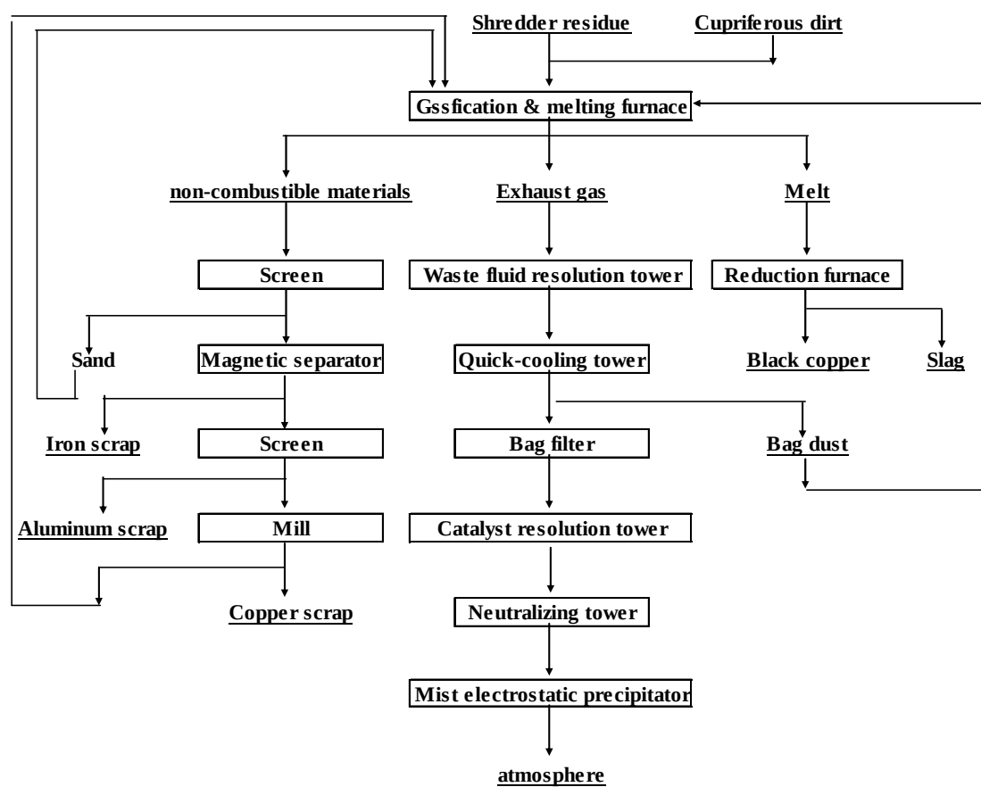
Figure 10 Flow of the gasification melting process
