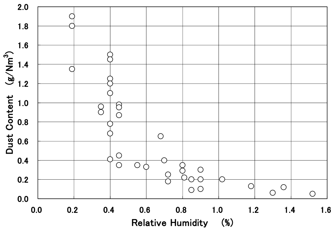
Figure 22 Relationship between relative humidity in off gas and ESP outlet dust content
