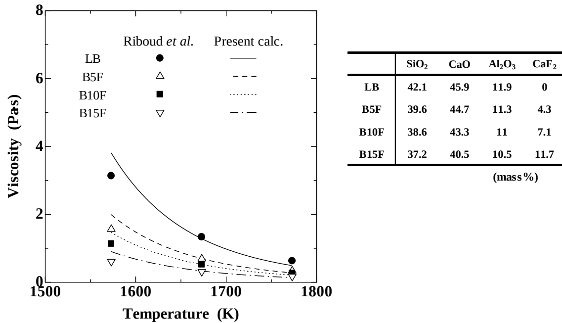
Figure 16 Viscosity for molten \text{SiO}_2\text{-CaO-Al}_2\text{O}_3\text{-CaF}_2 . 54)
