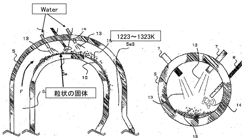
Figure 18 Prevention from adhesion of melted dust in duct
