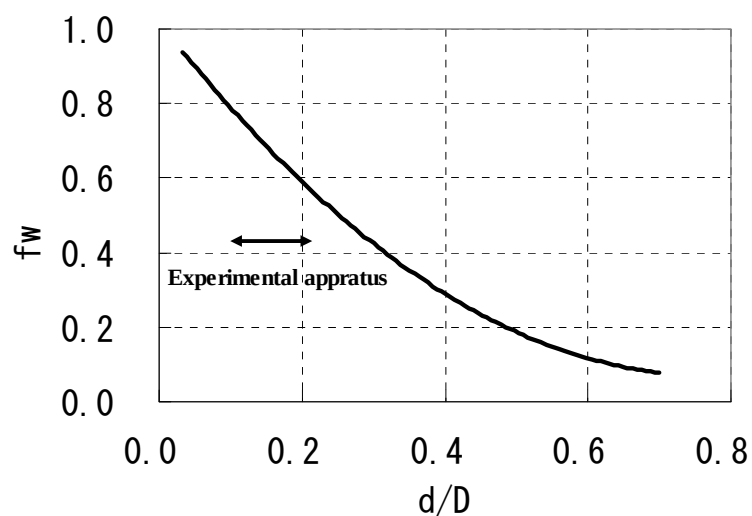
Figure 10 Change in the Faxen's factor f_w with the ratio of a ball' diameter to the diameter of cylindrical vessel ( d/D ).
