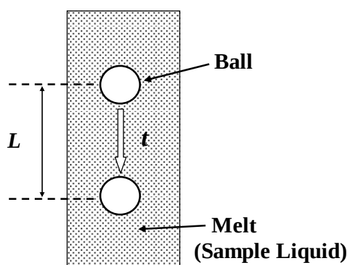
Figure 1 Schematic illustration of the falling ball method for viscosity measurement.
