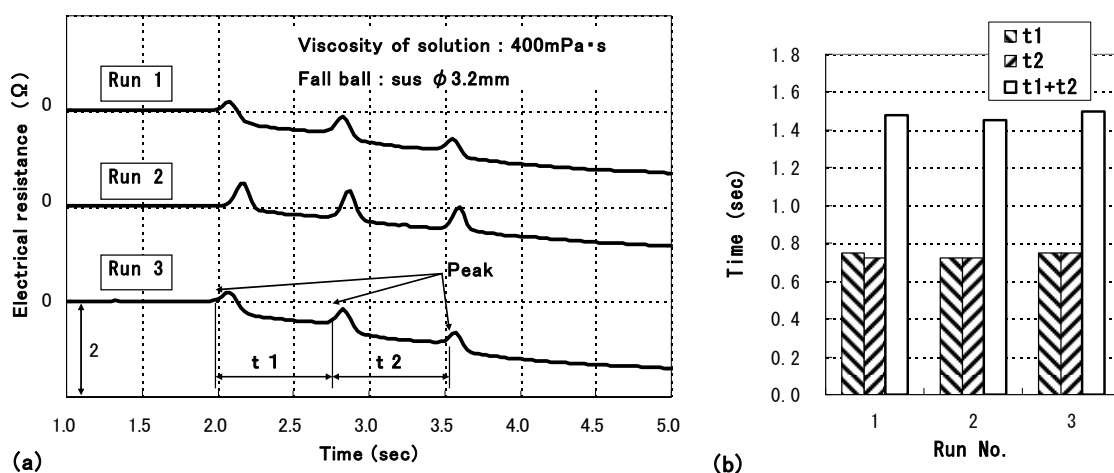
Figure 7 Change in the electric resistance with time for falling a ball in Metororz aqueous solutions with low viscosity.
