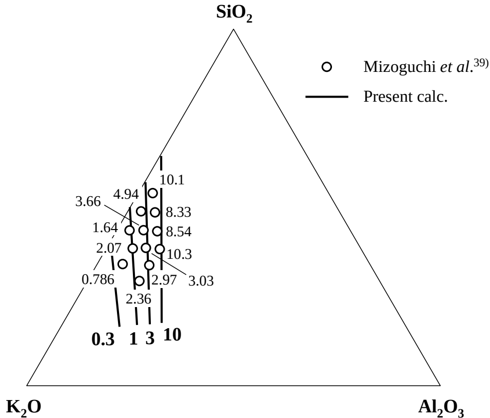
Figure 9 Viscosity (Pa·s) of SiO 2 -K 2 O-Al 2 O 3 system (mass%) at 1673 K.
