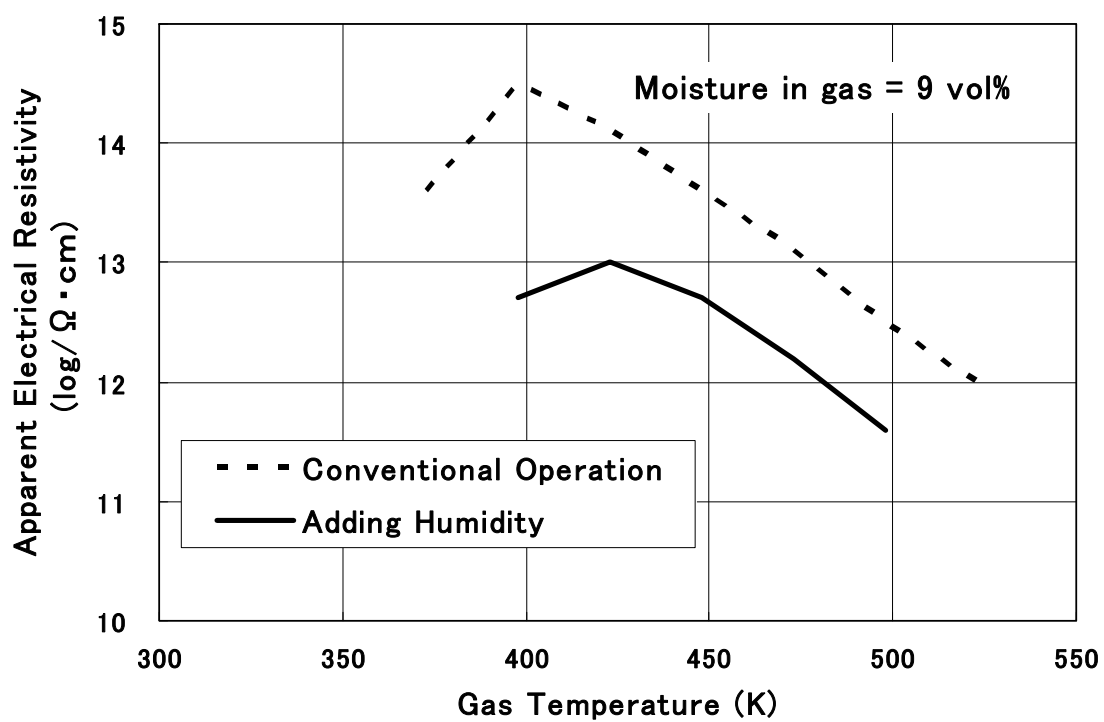
Figure 20 Change in apparent electrical resistivity of dust by adding humidity in off gas.
