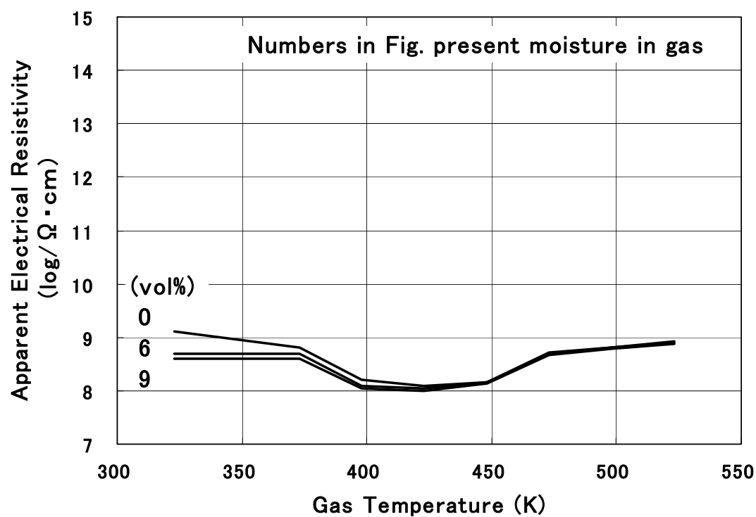
Figure 13 Apparent electrical resistivity of CdO
