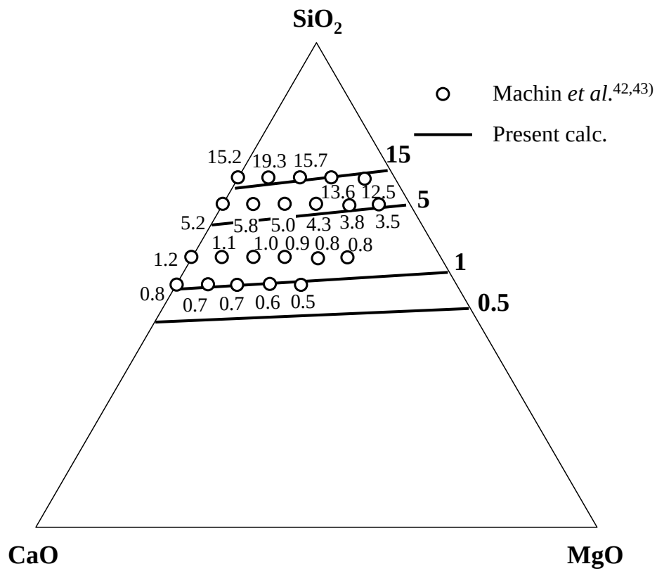
Figure 10 Viscosity (Pa·s) of \text{SiO}_2 - \text{CaO} - \text{MgO} -10 \text{Al}_2\text{O}_3 system (mass%) at 1723 K.
