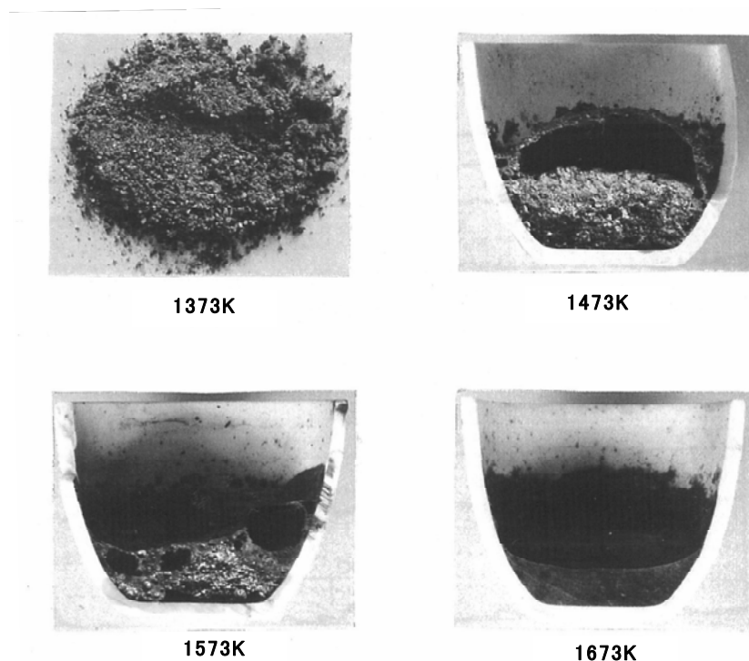
Figure 3 Experimental results of dissolution thermometry for bottom ash
