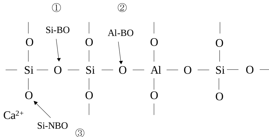
Figure 4 Three oxygen states in aluminosilicate by Susa et al. 6)
