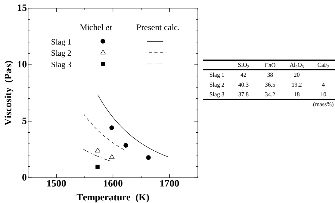
Figure 15 Viscosity of molten \text{SiO}_2\text{-CaO-Al}_2\text{O}_3\text{-CaF}_2 53)
