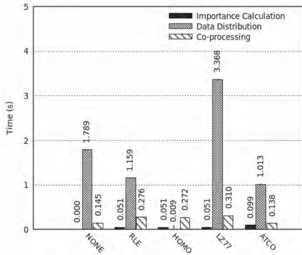
Fig. 3: Average execution times of the three main stages.
