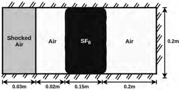
Fig. 1: Initial and boundary condition of the double-planar problem.
