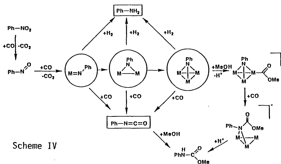
Proposed Reaction Scheme for Formation of Aniline, Isocyanate, Carbamates.
