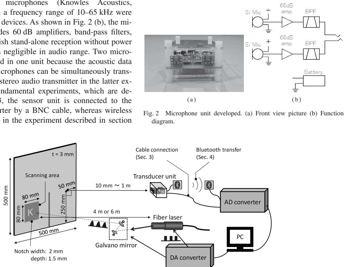
Fig. 1 Experimental system and plate specimen used in the experiments.
