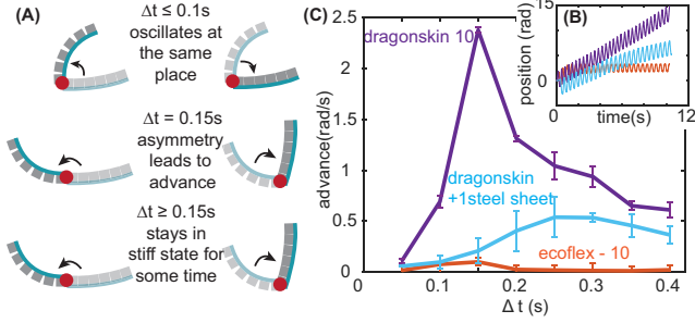
Figure 3: Closed loop control with maximum displacement 180° (a) Schematic showing appendage motion in the three conditions of \Delta t (max time between extremes) for DS-10. (b) (inset) Plot of angular position vs time showing the advance of the three different appendages, (c) Advance of the appendage vs \Delta t . Maximum advance was observed at \Delta t = 0.15 s for the appendage with DS-10 sleeve.
