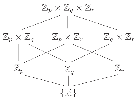
Fig. 3. The Hasse diagram of \mathbb{Z}_p \times \mathbb{Z}_q \times \mathbb{Z}_r for distinct primes p, q, r .
