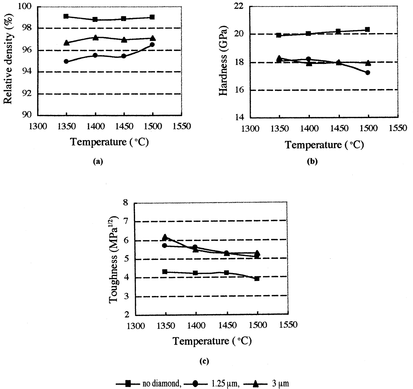
Fig.2 The variation of relative density (a), hardness (b) and indentation fracture toughness (c) of Al 2 O 3 - TiC- Diamond composite with sintering temperature for two different diamond particle size.
