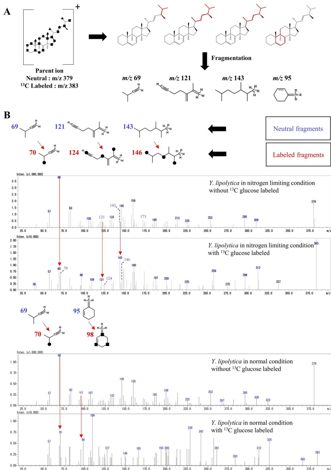
Figure 3- 4: Mass spectroscopic analysis of ^{13}\text{C} labeled ergosterol. (A), the predicted fragment from parent ion; (B), the mass spectra comparing the neutral and the labeled ergosterol product ion. The assign fragment structure elucidates the m/z increased specifically to the MVA pathway or the MEP pathway; circles indicate the theoretically
