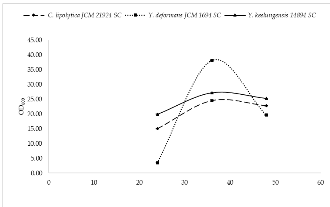
Figure 2- 7. Growth profile comparing Y. lipolytica spp. Error-bar represents the standard deviation from three replicates; Y. deformans JCM 1694 (square with dot line), Y. keelungensis JCM 14894 (triangle with dark line), C. lipolytica JCM 21924 (diamond with dash line).
