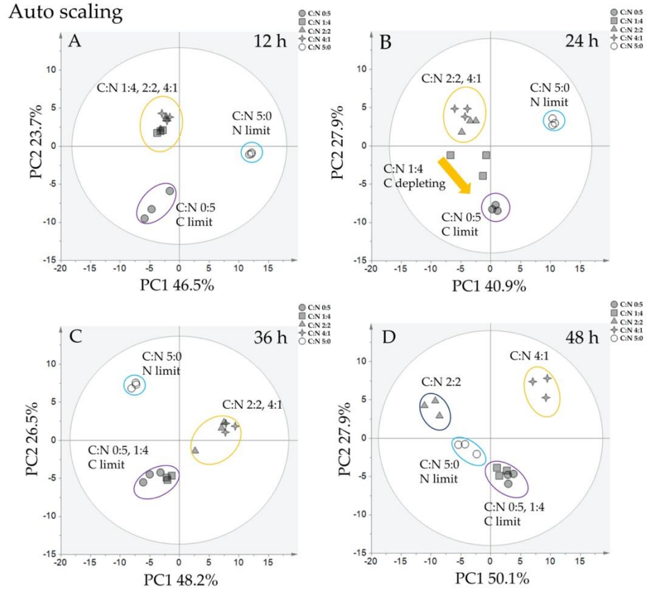
Figure 2- 4 PCA results for Y. lipolytica cultivated in different carbon-to-nitrogen ratios. PCA score plot indicating differences in metabolite profiles for different carbon-to-nitrogen ratios based on 93 metabolites. The grey ellipse indicates a 95% confidence border based on Hotelling's T2. Each point represents one replicate in each condition; 0:5 (grey circle), 1:4 (grey square), 2:2 (grey triangle), 4:1 (grey star), 5:0 (white circle). (Scale: Auto-scale; n = 3); (A) profile at 12 h, (B) profile at 24 h, (C) profile at 36 h, and (D) at profile at 48 h. The cyan ellipse indicates the nitrogen-limited samples, the purple ellipse indicates the carbon-limited samples, the yellow and blue ellipse indicates samples in which neither carbon nor nitrogen were limited. The full list of PCA loading scores is presented in Table S4.
