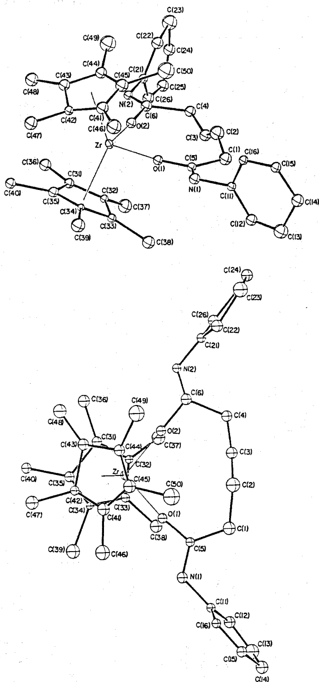
Fig. 2-3. Molecular structure of (\eta^5\text{-C}_5\text{Me}_5)_2\text{Zr}(\text{C}_4\text{H}_6)(\text{C}_6\text{H}_5\text{NCO})_2 (4a).
