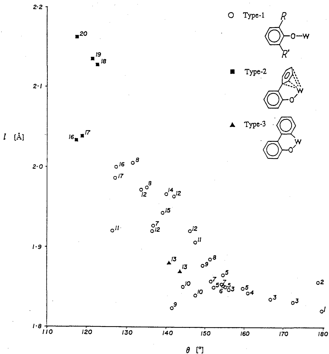
Fig. 3-6. Coordination geometry of phenoxy ligand in the molecular structures of tungsten-phenoxides by the W-O bond distance [ l ] vs. W-O-C bond angle [ \theta ] plotting. 25)
