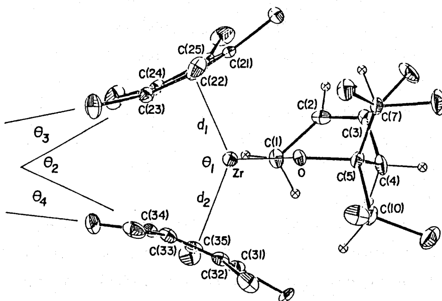
Fig. 2-8. Molecular structure of 7 viewed along the plane defined by Zr, O, and C(1) atoms.
