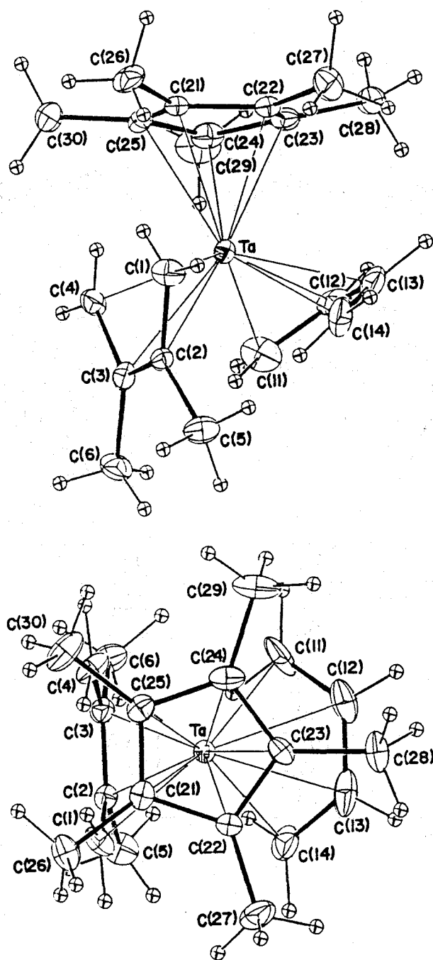
Fig. 1-8. Molecular structure of (\eta^5\text{-C}_5\text{Me}_5)\text{Ta}(\text{C}_4\text{H}_6)(\text{C}_6\text{H}_{10}) (28a).
