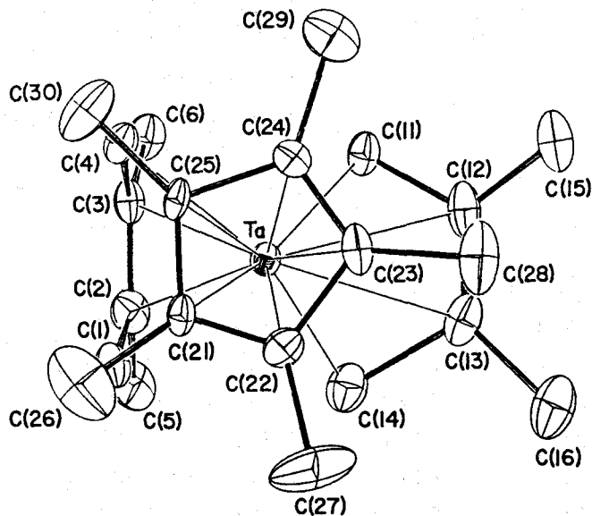
Fig. 1-6. Molecular structure of (\eta^5\text{-C}_5\text{Me}_5)\text{Ta}(\text{C}_6\text{H}_{10})_2 (23).
