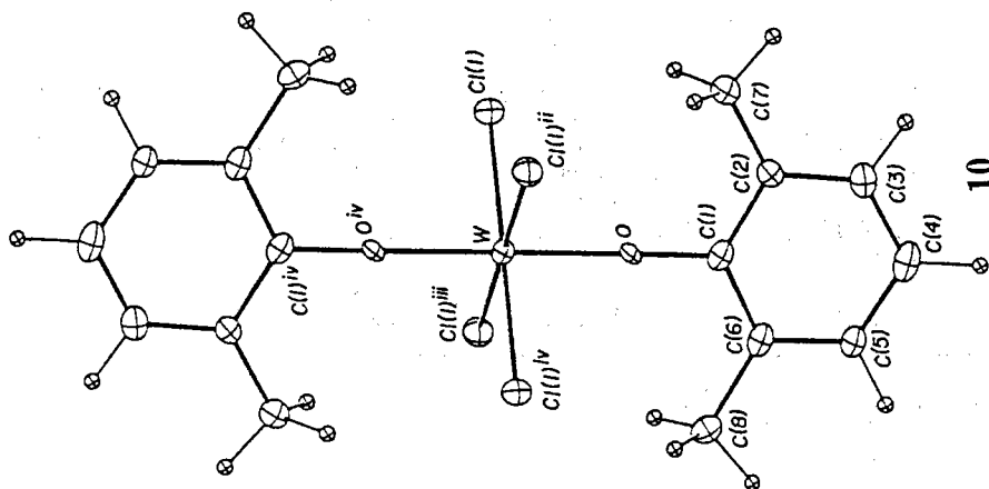
Fig. 3-5. Molecular structures of (a) \text{WCl}_5[\text{O}-2,6-(\text{CH}_3)_2\text{C}_6\text{H}_3] (9), and (b) \text{WCl}_4[\text{O}-2,6-(\text{C}_6\text{H}_5)_2\text{C}_6\text{H}_3]_2 (10).
