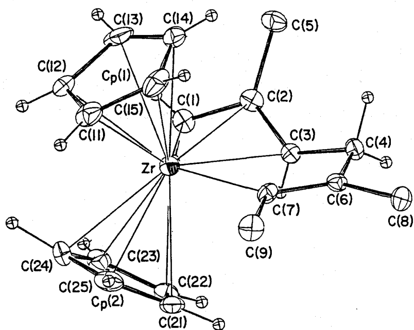
Fig. 2-9. Molecular structure of (\eta^5\text{-C}_5\text{H}_5)_2\text{Zr}[(\text{CH}_2\text{C}(\text{CH}_3)\text{CHCH}_2\text{-C}(\text{CH}_3)=\text{C}(\text{CH}_3))] .
