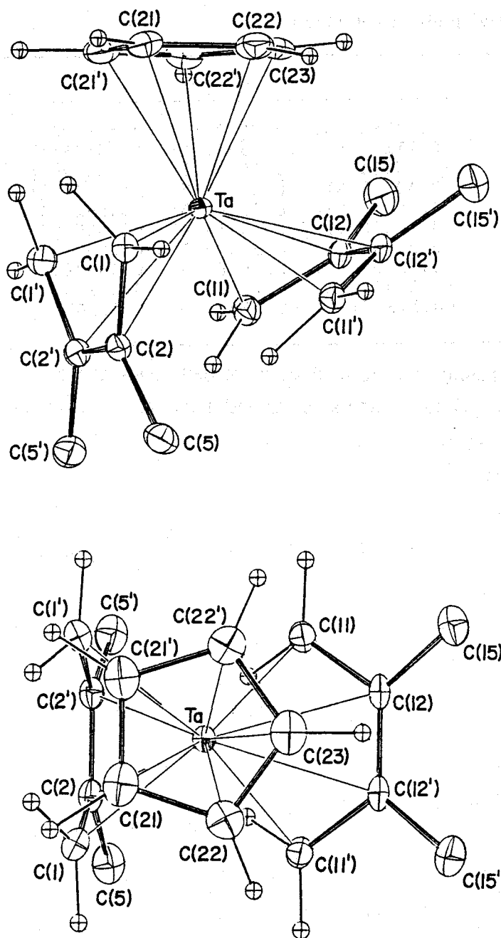
Fig. 1-5. Molecular structure of (\eta^5\text{-C}_5\text{H}_5)\text{Ta}(\text{C}_6\text{H}_{10})_2 (20).
