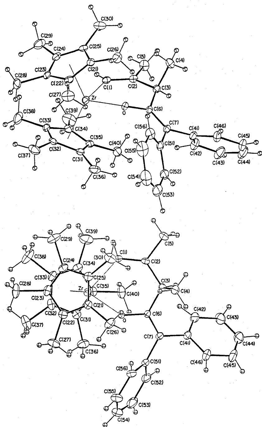
Fig. 2-4. Molecular structure of (\eta^5\text{-C}_5\text{Me}_5)_2\text{Zr}(\text{isoprene})((\text{C}_6\text{H}_5)_2\text{C}=\text{C}=\text{O}) (5).
