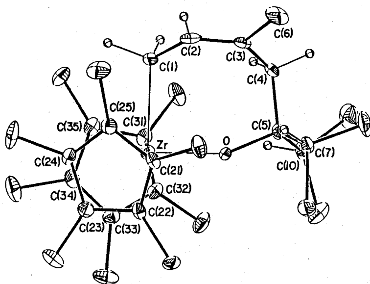
Fig. 2-7. Molecular structure of 7 projected onto the plane defined by Zr, O, and C(1) atoms.
