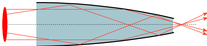
Paraboloid type
