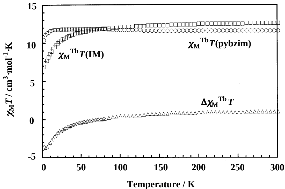
Figure 3-9. Temperature dependence of the \chi_M^{\text{Tb}}T(\text{IM}) ( \square ), \chi_M^{\text{Tb}}T(\text{pybzim}) ( \circ ) and \Delta\chi_M^{\text{Tb}}T ( \triangle ) of Tb(III) complexes.
