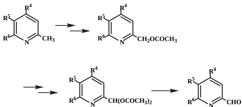
Scheme 4-1. Synthesis of n-methylpyridinecalbaldehyde
