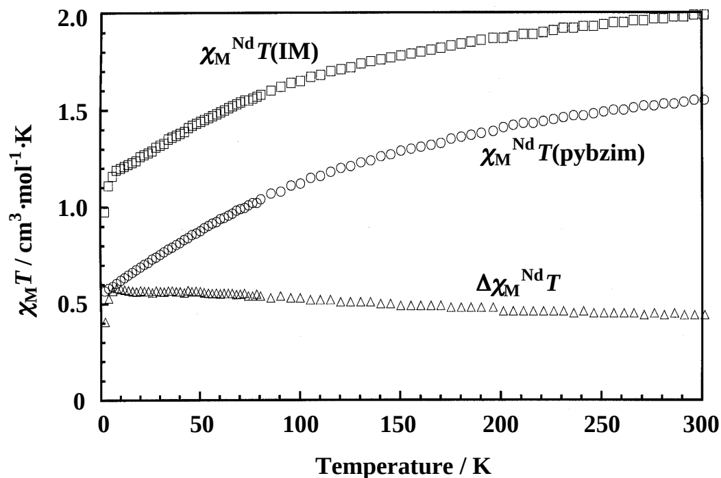
Figure 3-5. Temperature dependence of the \chi_M^{\text{Nd}} T(\text{IM}) ( \square ), \chi_M^{\text{Nd}} T(\text{pybzim}) ( \circ ) and \Delta \chi_M^{\text{Nd}} T ( \triangle ) of Nd(III) complexes.
