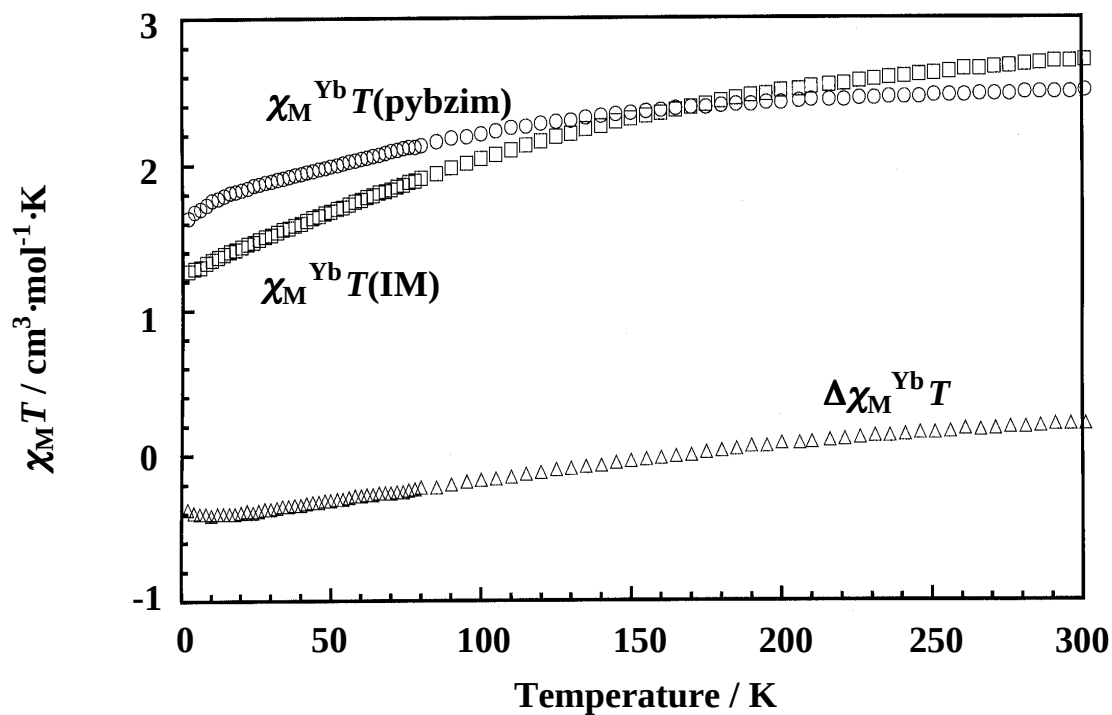
Figure 3-8. Temperature dependence of the \chi_M^{\text{Yb}}T(\text{IM}) ( \square ), \chi_M^{\text{Yb}}T(\text{pybzim}) ( \circ ) and \Delta\chi_M^{\text{Yb}}T ( \triangle ) of Yb(III) complexes.
