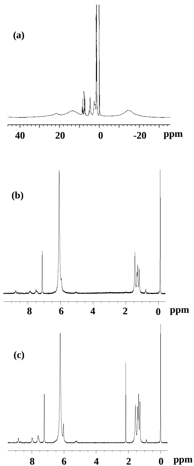
Figure 5-2. ^1\text{H} NMR spectra of free IM-2py (a), [\text{Y}(\text{hfac})_3(\text{IM-2py})] (b) and [\text{Lu}(\text{hfac})_3(\text{IM-2py})] (c).
