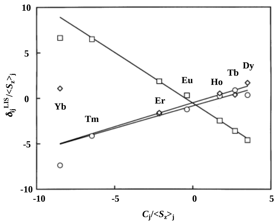
Figure 5-7. A plot of \delta_{ij}^{LIS} / \langle S_z \rangle_j vs. C_j / \langle S_z \rangle_j ( \square : hfac-CH, \diamond : 4-position proton in IM-2py, \circ : 5-position proton in IM-2py, respectively)
