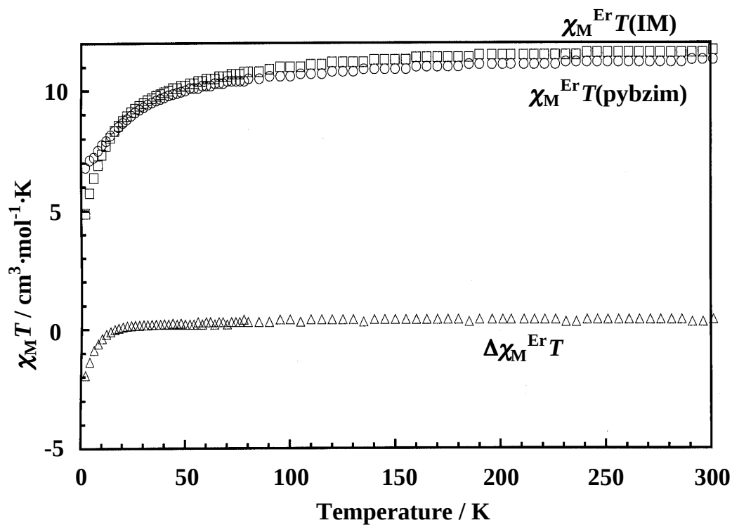
Figure 3-12. Temperature dependence of the \chi_M^{\text{Er}} T(\text{IM}) ( \square ), \chi_M^{\text{Er}} T(\text{pybzim}) ( \circ ) and \Delta\chi_M^{\text{Er}} T ( \triangle ) of Er(III) complexes.
