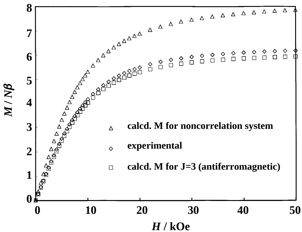
Figure 2-3. Field dependence of magnetization in the 0–50 kOe range for [Gd(hfac) 3 (IM-2py)].
