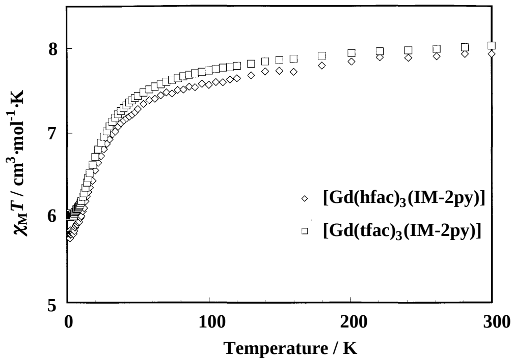
Figure 2-2. Temperature dependence of \chi_M T values in the 4.2–300 K range for [Gd( \beta -diketonato)(IM-2py)].
