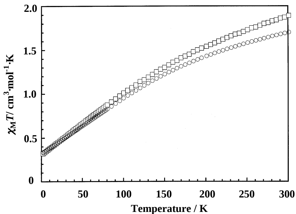
Figure 3-4. Temperature dependence of \chi_M^{\text{Eu}} T (IM) ( \square ) and the sum of \chi_M^{\text{Eu}} T(\text{pybzim}) and 0.32 \text{ cm}^3 \cdot \text{mol}^{-1} \cdot \text{K} ( \circ ), which is \chi_M^{\text{Eu}} T (IM) at 2 K.
