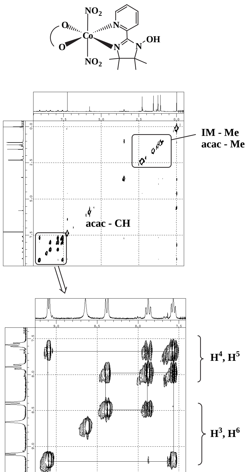
Figure 5-4. ^1\text{H} - ^1\text{H} COSY spectrum of [\text{Co}(\text{acac})((\text{NO}_2)_2(\text{IMH-2py}))]
