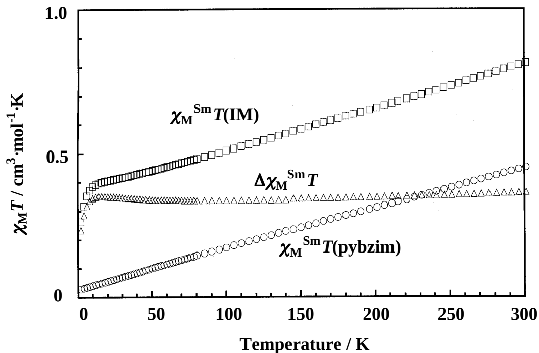
Figure 3-6. Temperature dependence of the \chi_M^{\text{Sm}} T(\text{IM}) ( \square ), \chi_M^{\text{Sm}} T(\text{pybzim}) ( \circ ) and \Delta \chi_M^{\text{Sm}} T ( \triangle ) of Sm(III) complexes.
