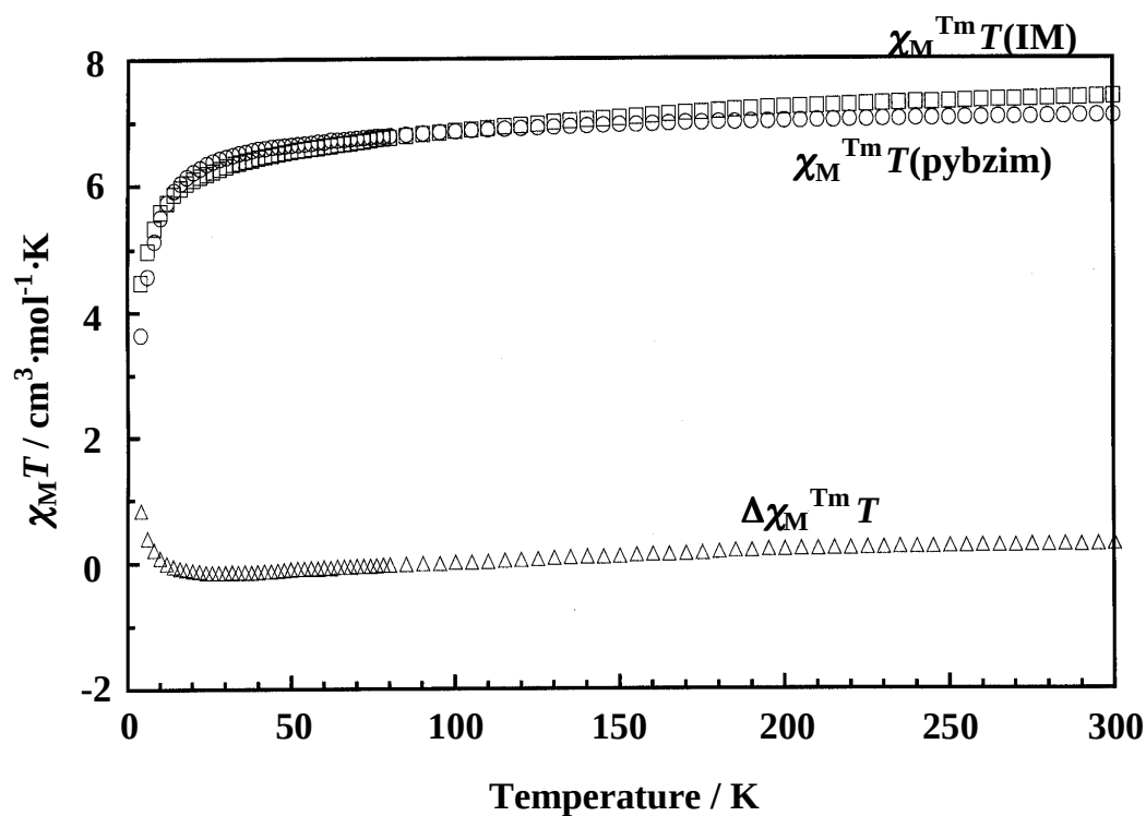
Figure 3-13. Temperature dependence of the \chi_M^{\text{Tm}} T(\text{IM}) ( \square ), \chi_M^{\text{Tm}} T(\text{pybzim}) ( \circ ) and \Delta\chi_M^{\text{Tm}} T ( \triangle ) of Tm(III) complexes.
