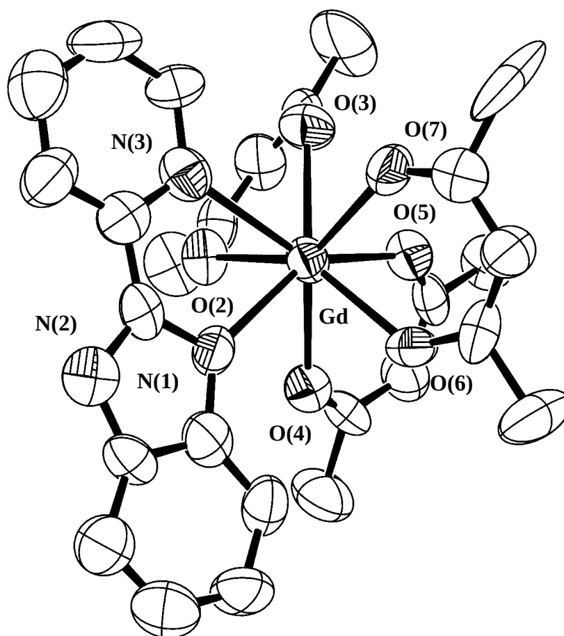
Figure 3-2. Molecular structure of [\text{Gd}(\text{hfac})_3(\text{IM-2py})] showing 50% probability ellipsoids(F atoms are omitted).
