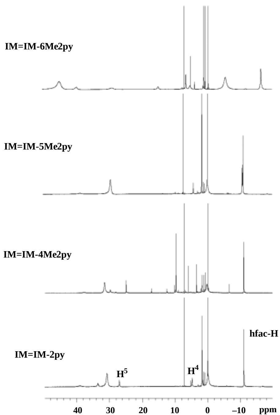
Figure 5-6. ^1\text{H} NMR spectra of [\text{Yb}(\text{hfac})_3(\text{IM})] ( \text{IM}=\text{IM}-n\text{Me}_2\text{py} ; n=x, 4, 5, 6 )
