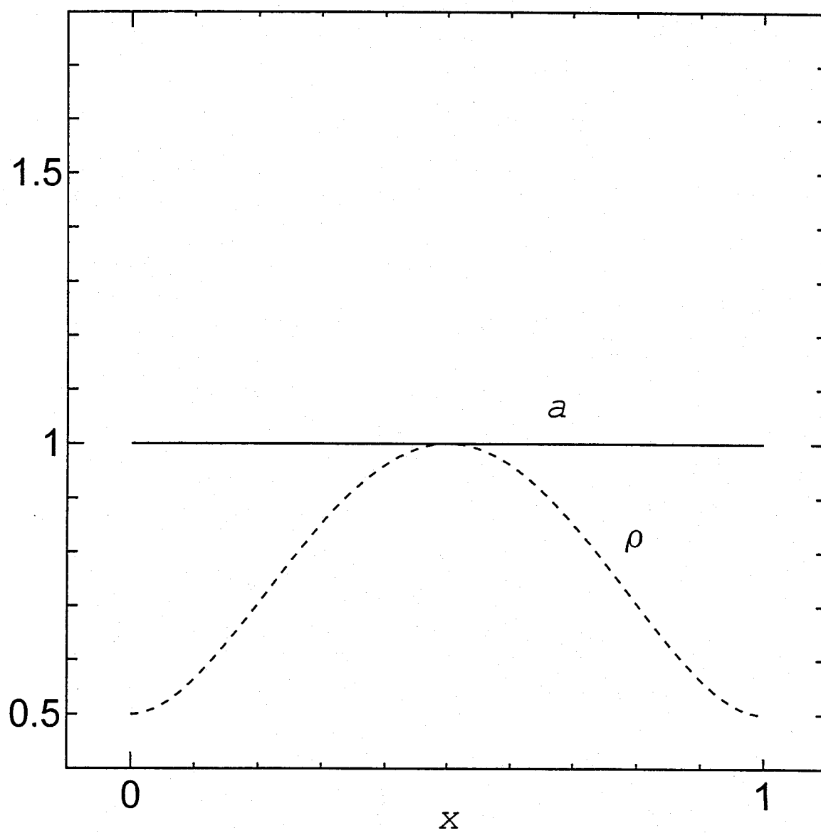
図 6.1 (a) t = 0
