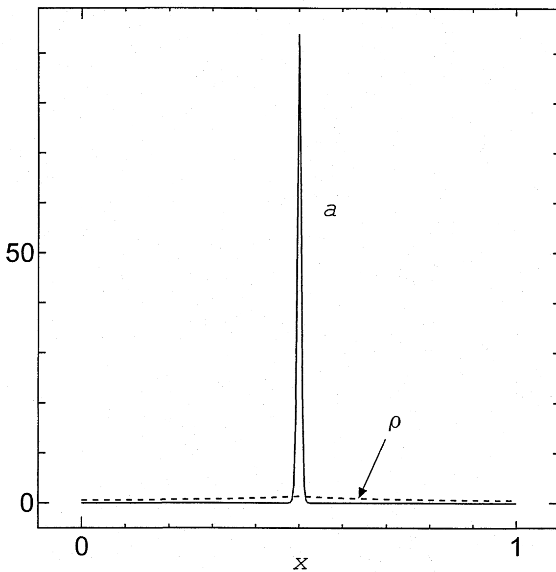
図 6.1 (c) t = 0.2
