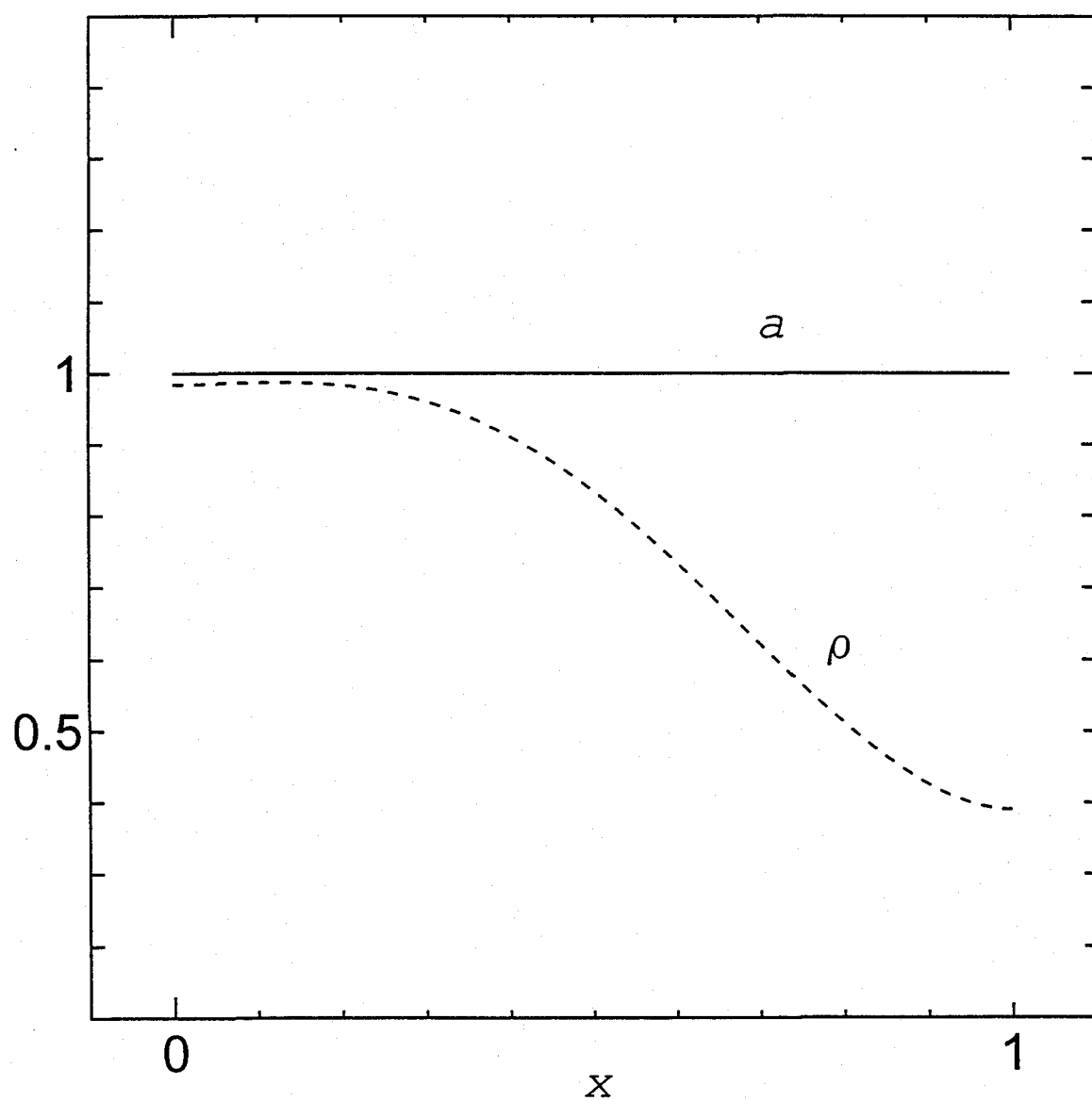
図 6.2 (a) t = 0
