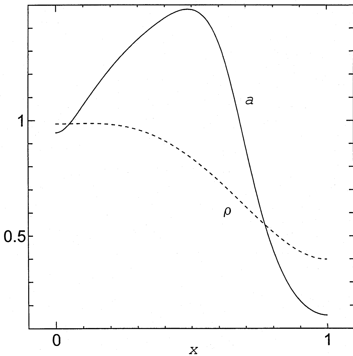
図 6.2 (c) t = 0.01
