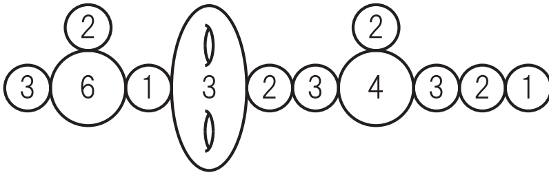
Fig. 3. This singular fiber has three cores, four branches and two trunks. The numbers stand for the multiplicity of each irreducible component and each intersection point is a node.
