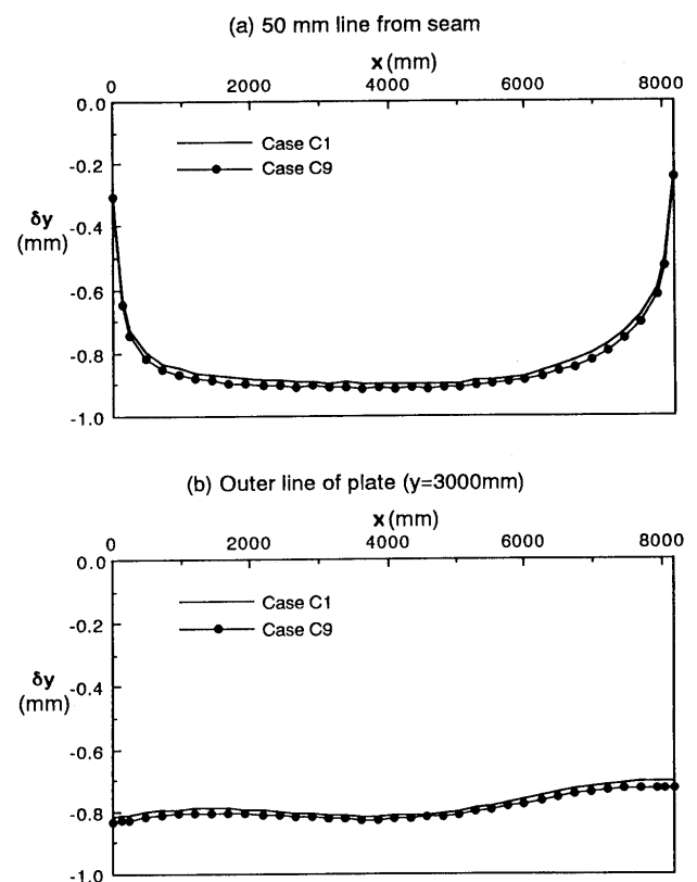
Fig. 17 Welding deformation considering the influence of residual stress produced by gas cutting (C9).
