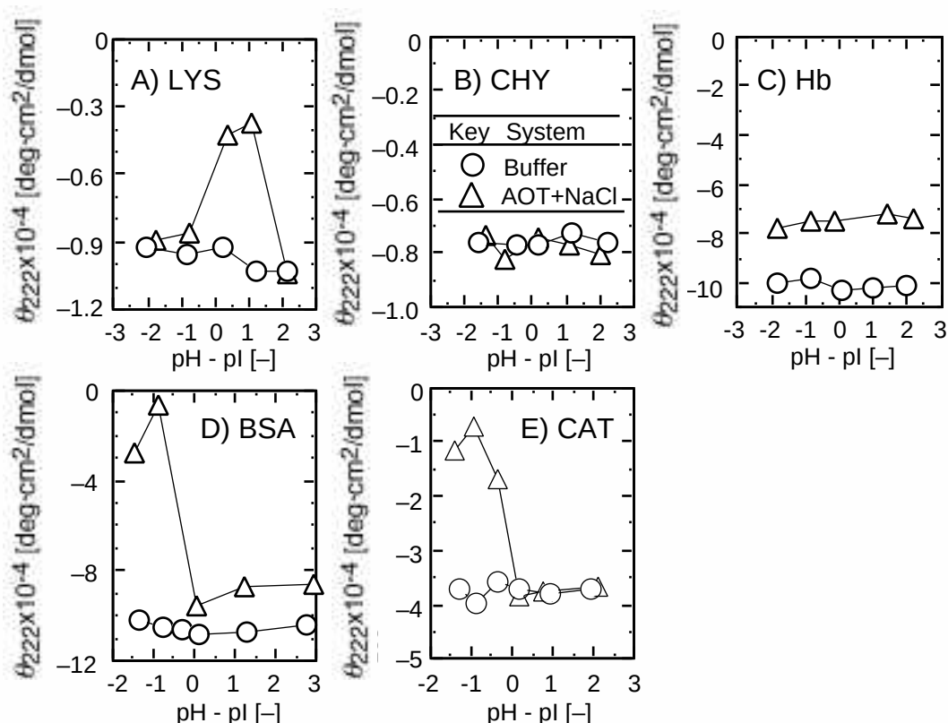
Fig. 1.6 Effect of pH on molecular ellipticities at 222 or 208 nm of proteins in the aqueous solution containing 1 mM AOT and 0.1 M NaCl and in the buffer solution. A) lysozyme; B) α-chymotrypsinogen; C) hemoglobin; D) BSA; E) catalase.
