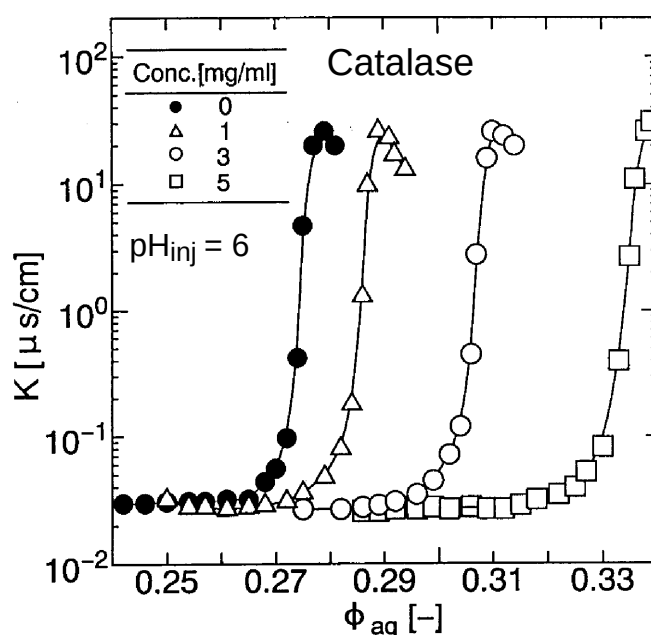
Fig. 1.10. The variation of the electric conductivity as a function of the volume fraction of water containing catalase for the AOT reverse micellar solution
