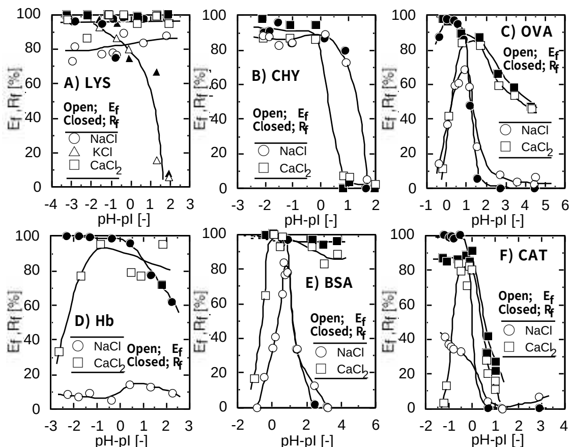
Fig. 3.12 Effect of pH on the extraction of proteins by the AOT reverse micellar system using \text{CaCl}_2 as a salt in the aqueous phase.
