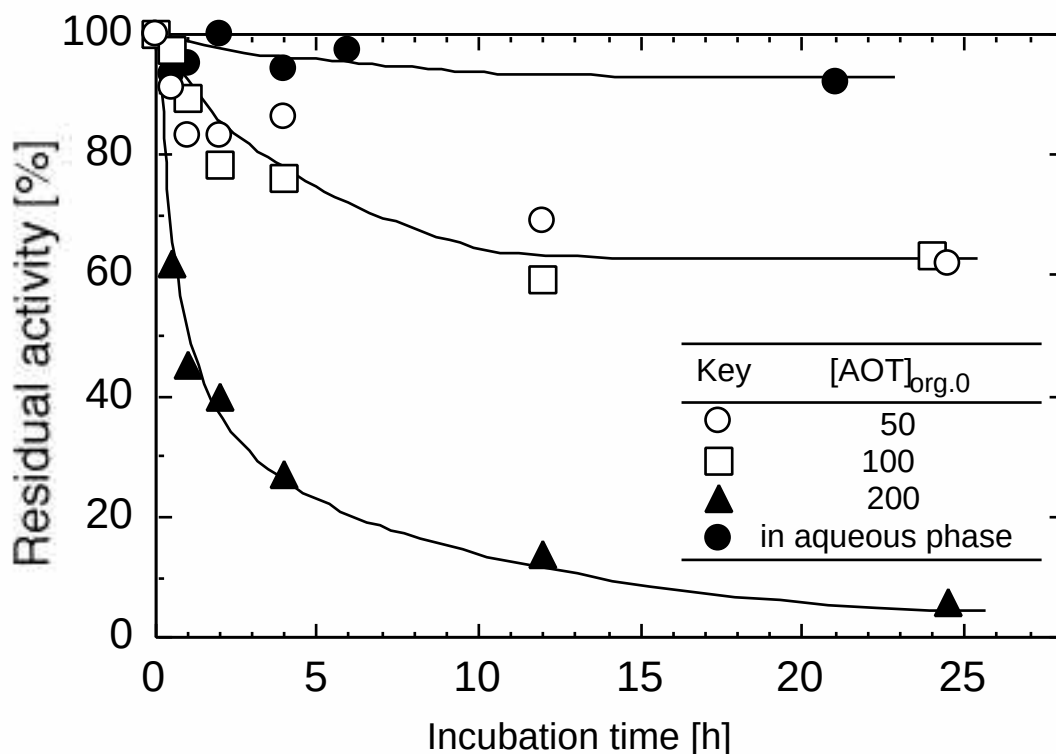
Fig. 2.8. Effect of concentration of AOT on lipase stability in reverse micelles at C_{E,ov} = 0.4 \text{ kg/m}^3 , W_0 = 7 and pH 7.2.
