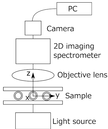
Fig. 2 Experimental setup of 2-D transmission spectroscopy.
