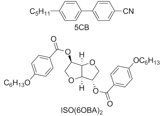
Fig. 1 Molecular structures of 5CB and ISO(6OBA) 2 .
