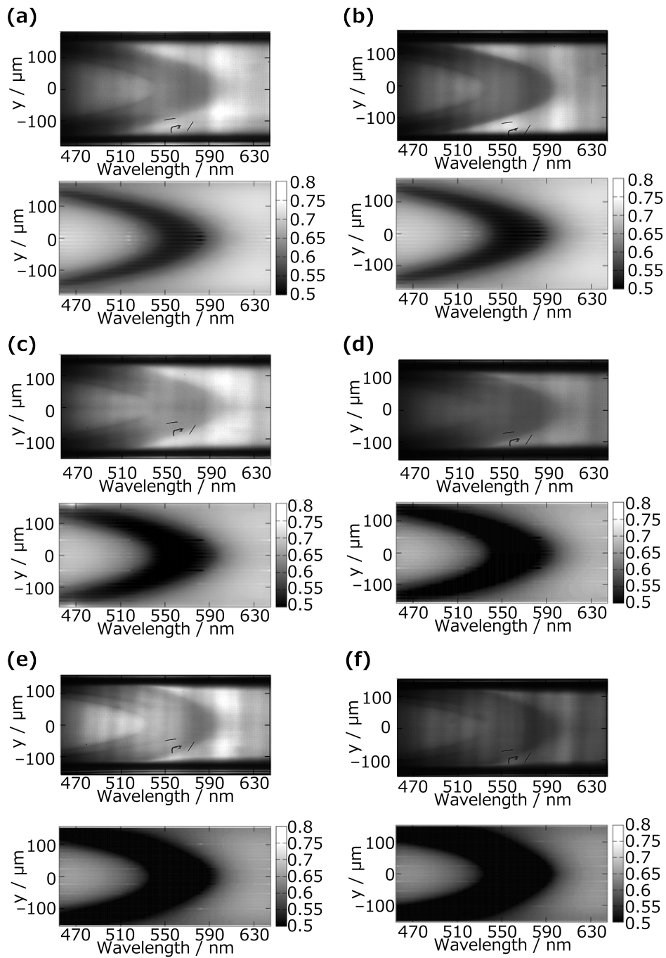
Fig. 5 2-D transmission spectra of CLC microcapsules for mapping of the spectra on the shell surface. Experimental (above) and simulated (below) 2-D transmission spectra of CLC microcapsules with (a) (R, a) = (200 \mu\text{m}, 179 \mu\text{m}) , (b) with (R, a) = (200 \mu\text{m}, 174 \mu\text{m}) , (c) with (R, a) = (200 \mu\text{m}, 163 \mu\text{m}) , (d) with (R, a) = (200 \mu\text{m}, 159 \mu\text{m}) , (e) with (R, a) = (210 \mu\text{m}, 157 \mu\text{m}) , and (f) with (R, a) = (210 \mu\text{m}, 153 \mu\text{m}) .
