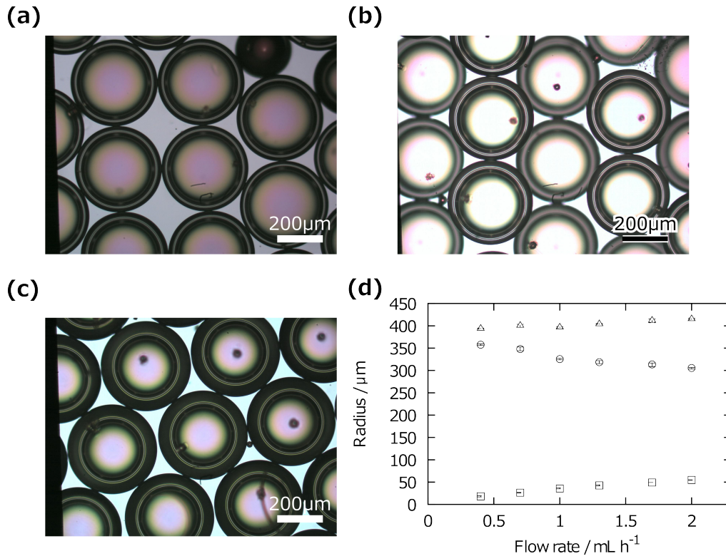
Fig. 4 Dependence of the size of the CLC microcapsules on the flow rate of the shell phase. Bright-field microphotographs of the CLC microcapsules fabricated at the flow rate of the shell phase of (a) 0.4, (b) 1.0, and (c) 2.0 mL h -1 . (d) Plots of the diameter for core radius a (open circle), outer radius R (open triangle), and the thickness of the CLC shell R - a (open square) as a function of the flow rate of the shell phase. These values are the mean values of three measurements at each flow rate.
