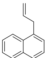
1-allylnaphthalene ( 3o ) S21
