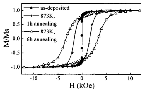
FIG. 3. In-plane hysteresis loops for a\text{-Al}_2\text{O}_3/\text{Fe}/\text{Pt} films on the (100) MgO substrate (unannealed and annealed at 600^\circ\text{C} for different times).
