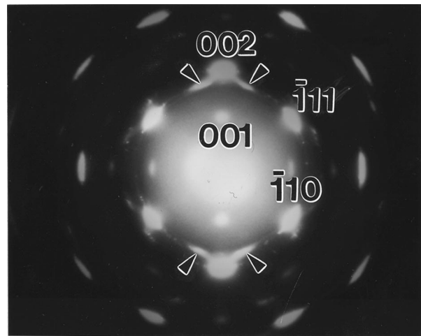
FIG. 2. SAED pattern of 600^\circ\text{C} annealed a\text{-Al}_2\text{O}_3/\text{Fe}/\text{Pt} film obtained with the electron beam parallel to the \langle 110 \rangle direction of the film. Besides the superlattice reflections due to L1_0 and the fundamental reflections, there exist extra reflections (as marked by arrows) from \{111\} twins and stacking faults.
