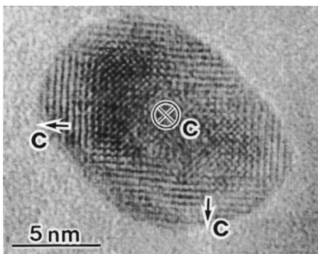
FIG. 5. HREM image of a typical ordered FePt particle. The c axis of the central region of the particle is perpendicular to the film plane and that of the other two orthogonal variants in the outer regions of the crystallite, are in the horizontal plane.
