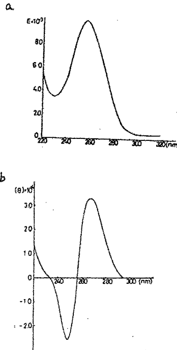
Fig.6 UV CD spectrum of poly (Az) in the presence of 0.15M Na + at pH 7.0 and 16°.
