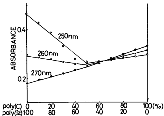
Fig.5 Mixing experiment of \text{poly(Iz)} and \text{poly(C)}
