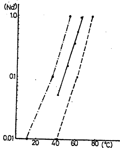
Fig23. Relationship of \text{Na}^+ concentration and T_m of \text{poly(Iz)} \cdot \text{poly(C)} ( — ), \text{Poly(I)} \cdot \text{poly(C)} ( ---- ) and \text{poly(dI)} \cdot \text{poly(C)} ( - - - - - ).
