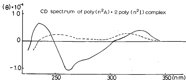
Fig. 12. CD spectra of poly(n^2I) \cdot poly(n^2I) (1:2) complex. Measured in the presence of 0.15 M Na^+ (pH 7.0). —, observed curve; ----, calculated curve from CD curves of components.
