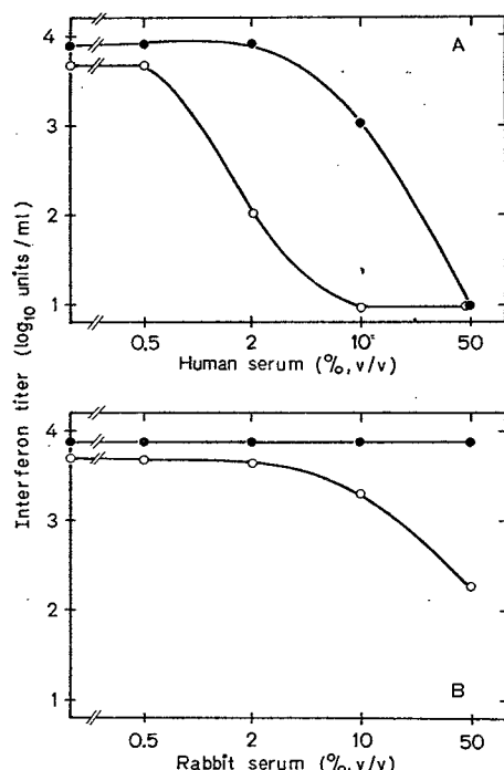
Fig. 3. Sensitivity of (\text{dIn}_3)_n \cdot (\text{C})_n (○) and (\text{I})_n \cdot (\text{C})_n (●) to degradation by: (A) human serum and (B) rabbit serum, as monitored by residual interferon-inducing activity. The polynucleotide-serum mixtures contained 1 \mu\text{g} of polynucleotide and varying concentrations of (A) human or (B) rabbit serum (as indicated) per ml Eagle's minimum essential medium. The mixtures were incubated for 1 h at 37 °C and then assayed for interferon induction in human skin fibroblasts 'primed' with interferon and 'superinduced' with cycloheximide and actinomycin D.
