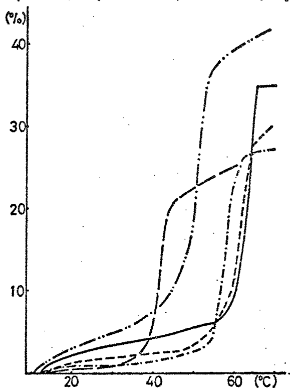
Fig 22 Temperature absorbance profile of \text{poly(I}_2)\text{poly(C)} complexes at various \text{Na}^+ concentration --- 0.04 M, --- 0.15 M, --- 0.35 M, --- 0.55 M, --- 0.95 M,
