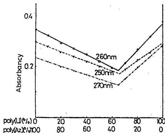
Mixing curves of poly (Az) and poly (U) at \text{Na}^+ concentration of 0.15M.
