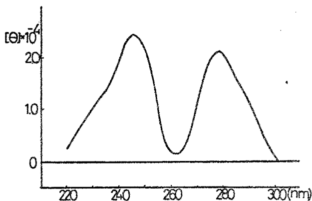
Fig. 54 CD spectrum of poly(If)·poly(C) complex.
