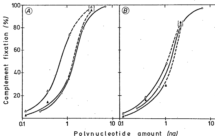
Fig. 4. Quantitative complement fixation of (\text{dIn}_3)_n \cdot (\text{C})_n (Δ), (\text{dIn}_3)_n \cdot (\text{br}^5\text{C})_n (▲) and (\text{I})_n \cdot (\text{C})_n (○) with antibody to (\text{A})_n \cdot (\text{U})_n . The antibodies had been purified with (\text{I})_n \cdot (\text{C})_n and were used at 1/1500 dilution (A) or 1/3000 dilution (B) from stock. Because of the anti-complementary activity of (\text{dIn}_3)_n \cdot (\text{C})_n and (\text{dIn}_3)_n \cdot (\text{br}^5\text{C})_n at amounts higher than 1 ng, the exact amounts of (\text{dIn}_3)_n \cdot (\text{C})_n and (\text{dIn}_3)_n \cdot (\text{br}^5\text{C})_n required for maximal complement fixation could not be determined. The complement fixation values obtained at doses at which (\text{dIn}_3)_n \cdot (\text{C})_n and (\text{dIn}_3)_n \cdot (\text{br}^5\text{C})_n showed partial anticomplementary activity are indicated in brackets.
