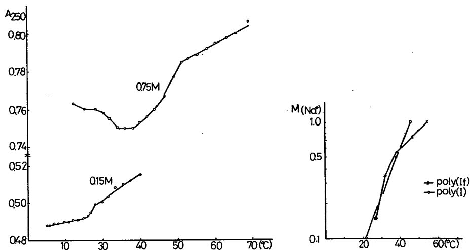
Fig. 3. Thermal melting profiles of poly(If) at Na + concentration of 0.15M and 0.75M.
