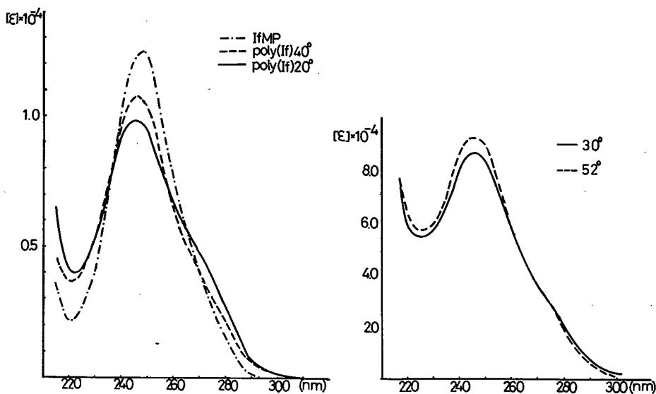
Fig. 1. UV spectrum of poly(If) and If 5'-MP at pH 7.0 in the presence of 0.15M Na + ion.
