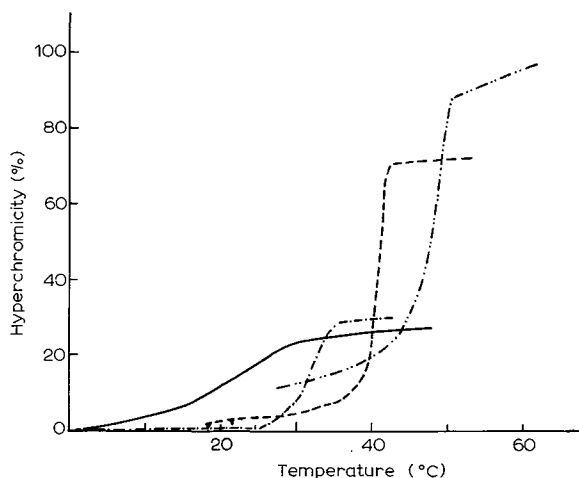
Fig. 6. Thermal melting of poly( n^2A ) · poly(U) (1 : 2) complex, Poly( n^2A ) · poly(I) (1 : 2) complex, poly( n^2I ) · poly(A) (1 : 2) complex and poly( n^2A ) · poly( n^2I ) (1 : 2) complex. ----, poly( n^2A )-poly(U), measured at 260 nm; —, poly( n^2A )-poly(I), measured at 249 nm; - · - · -, poly( n^2I )-poly(A), measured at 260 nm; - · - · -, poly( n^2A )-poly( n^2I ), measured at 250 nm.
