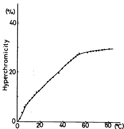
Fig. 3. Temperature-absorption profile of poly (Az) at pH 7.0.
