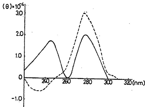
Fig 21 CD spectra of poly(I 2 ) and poly(C) (1:1) before and after mixing. ----- before mixing, ——— after mixing 20
