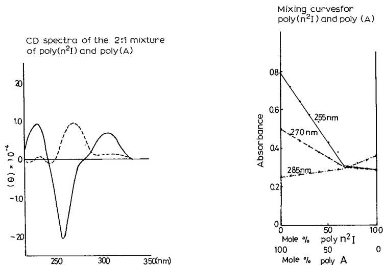
Fig. 9. Mixing curve of \text{poly}(\text{n}^2\text{I}) and \text{poly}(\text{A}) . ●—●, absorbance at 255 nm; ●—●, at 270 nm, X—X at 285 nm.
