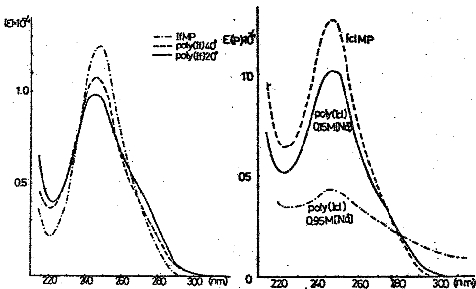
Fig3 a UV spectra of poly(If)
