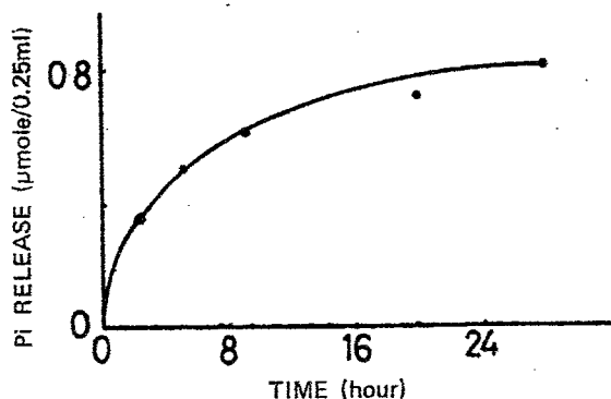
Fig 24 Time course of AaDP polymerization.
