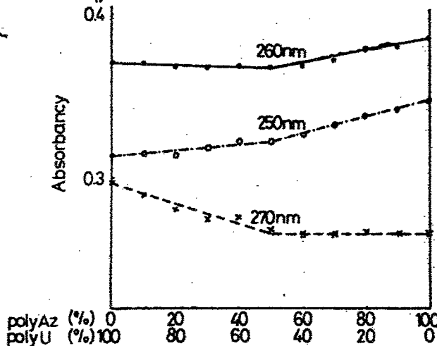
Mixing curves of poly (Az) and poly (U) at 0.04M Na + .
