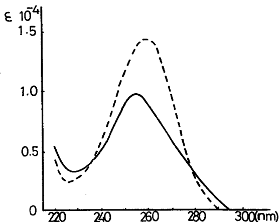
Fig. 1 U. V. absorption spectra of poly(Af) and Af 5'-MP. Poly(Af) —, Af-5'-MP ----.
