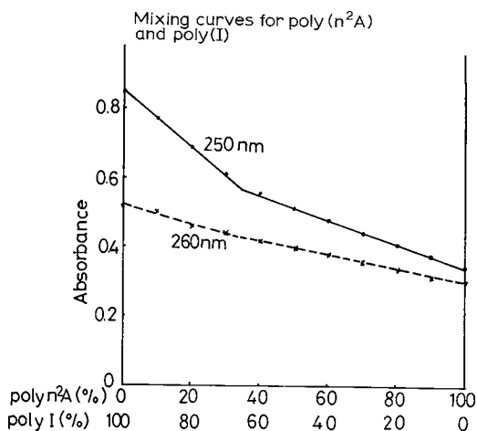
Fig. 7. Mixing curve of poly( n^2\text{A} ) and poly(I). X- - - -X, absorbance at 260 nm; ●—●, at 250 nm.
