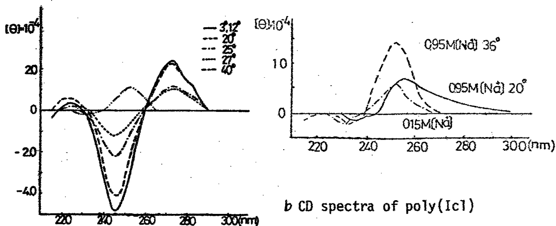
Fig4 a CD spectra of poly(If)
