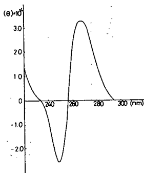
Fig. 4. CD spectrum of poly (Az) in the presence of 0.15 \text{ M Na}^+ at pH 7.0 and 16^\circ .
