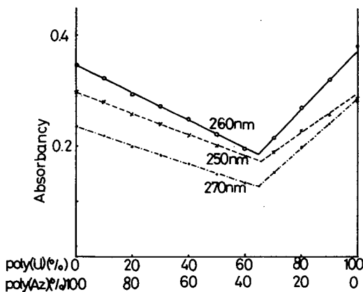
Fig. 7. Mixing curves of poly (Az) and poly (U) at \text{Na}^+ concentration of 0.15M.
