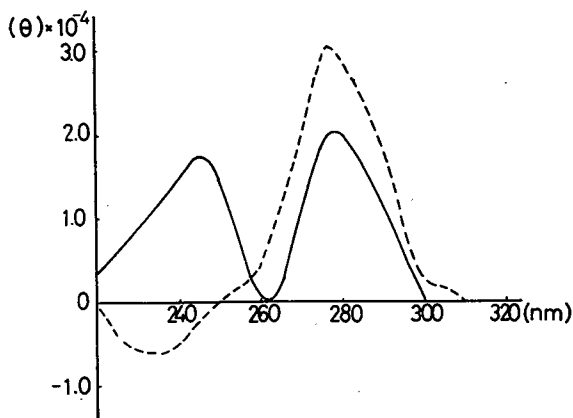
Fig. 6 CD spectra of \text{poly(Iz)} and \text{poly(C)} (1:1) before and after mixing. ---- before mixing, — after mixing
