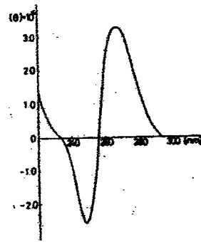
UV absorption spectrum of poly (Az) at pH 7.0. CD spectrum of poly (Az) at pH 7.0
