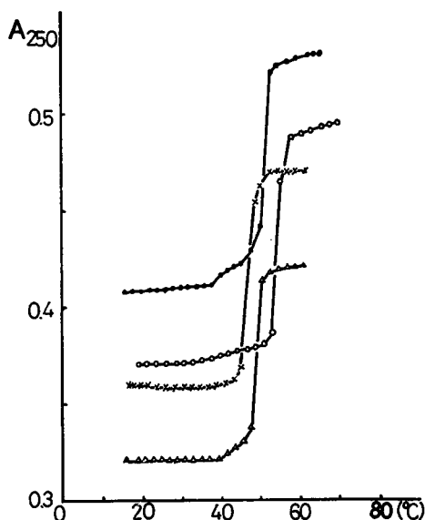
Fig. 7 Melting profiles of poly(A)-poly(I) complexes measured in the presence of 0.10M NaCl, 0.05M Na Cacodylate (pH 7.0) and 10mM \text{MgCl}_2 . Poly(Af)·2poly(I) ●-●-●, poly(A)·2poly(I) ○-○-○, poly-(Abr)·2poly(I) x-x-x, poly(Abr)·2poly(I) △-△-△.
