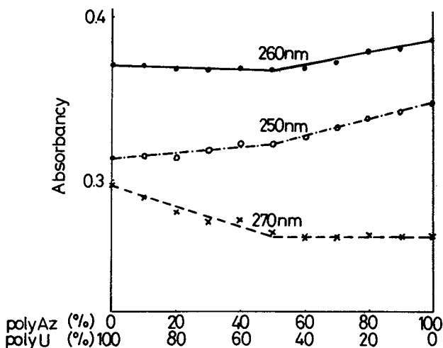
Fig. 6. Mixing curves of poly (Az) and poly (U) at 0.04M \text{Na}^+ .
