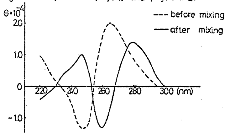
Fig 44 CD spectra of \text{poly}(\text{At}) and \text{poly}(\text{I}) (1:2)
