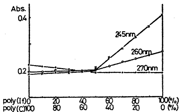
Fig 53. Mixing curves of poly(If) with poly(C)
