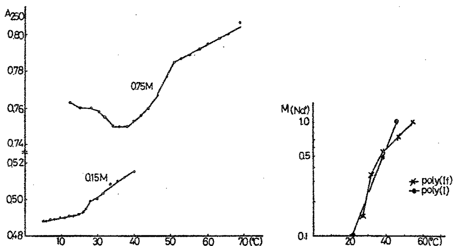
Fig 48(a) Thermal melting profiles of poly(If) at Na + concentration of 0.15M and 0.75M. Fig 48(b) Relationship of T m of poly(If) and poly(I) to Na + concentration.
