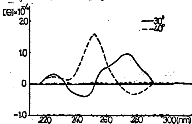
Fig 51 CD spectra of poly(I f ) at 0.75M(Na + )
