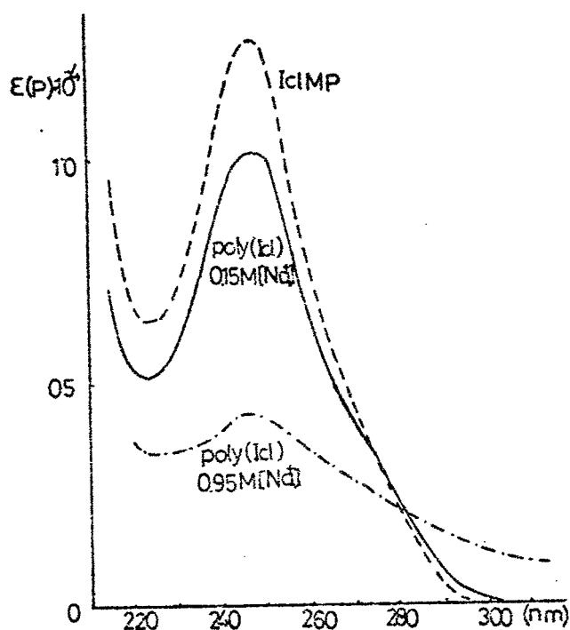
Fig 47 UV spectra of poly(Ic) and IcMP at pH7.0
