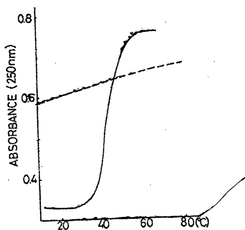
Fig. 20 T m of poly(Iz) — 0.95M Na + ---- 0.15M Na +
