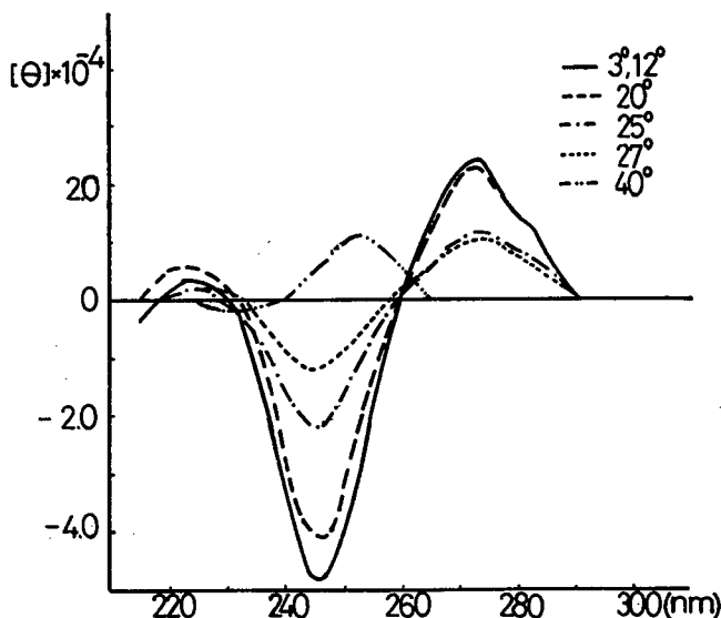
Fig. 5. CD spectra of poly(If) at 0.15M Na + concentration.
