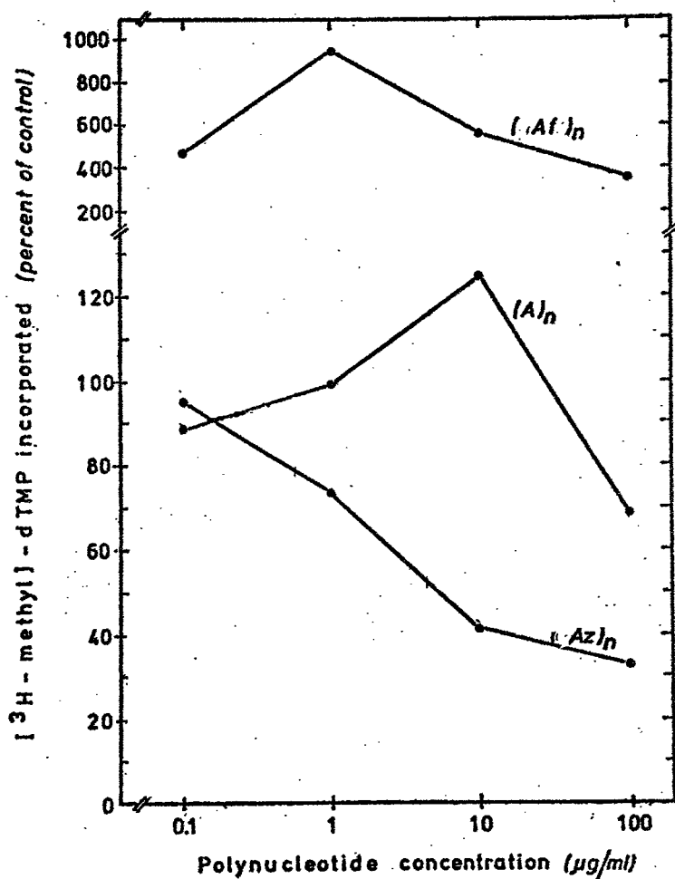
Fig 62 Effect of \text{poly}(\text{Az}) and \text{poly}(\text{Af}) on MuLV reverse-transcriptase in the absence of \text{poly}(\text{A}) , \text{oligo}(\text{dT}) as template-primer
