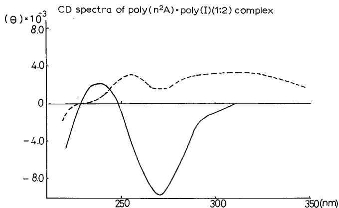
Fig. 8. CD spectra of \text{poly}(\text{n}^2\text{A}) \cdot \text{poly}(\text{I}) (1 : 2) complex. Measured in the presence of 0.15 M \text{Na}^+ (pH 7.0). —, observed curve; ----, calculated curve from CD curves of components.
