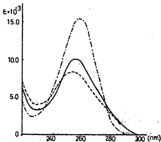
Fig. 37 UV absorption spectra of poly (AcI). — at pH 7.0. ..... at pH 4.5, ---- AcI-MP.
