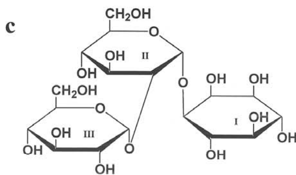
Saccharide 3
