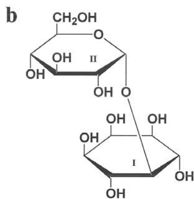
Saccharide 2
