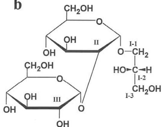
Saccharide B
