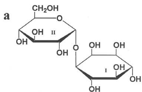
Saccharide 1
