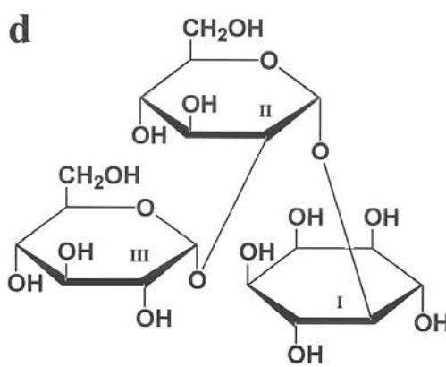
Saccharide 4
