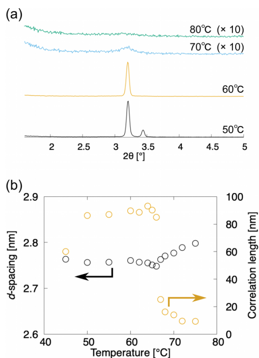
Figure 5. X-ray diffractometry of ( \pm )-3 upon the cooling run. Black and orange circles denote the d -spacing and the correlation length of the layer structure, respectively.
