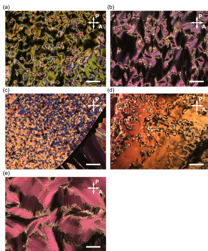
Figure 3. Polarised optical micrographs of ( \pm )- 1–3 in the cooling run. (a) A Schlieren texture for the N phase of ( \pm )- 1 at 65°C, (b) a fan-shaped texture for the SmA phase of ( \pm )- 1 at 45°C and (c) A Schlieren texture for the N phase (centre), an isotropic phase (left) and a Cr phase (right) of ( \pm )- 2 at 69°C. (d) A Schlieren texture for the N phase of ( \pm )- 3 at 80°C, (e) a fan-shaped texture for the SmA phase of ( \pm )- 3 at 55°C. The scale bars correspond to 100 \mu\text{m} .
