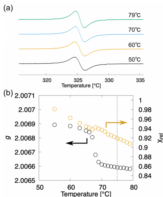
Figure 6. EPR spectroscopy of (±)- 3 upon the cooling run. Black and orange circles denote the g -value and \chi_{rel} , respectively. Vertical dotted line denotes N-to-N cyb phase transition point.
