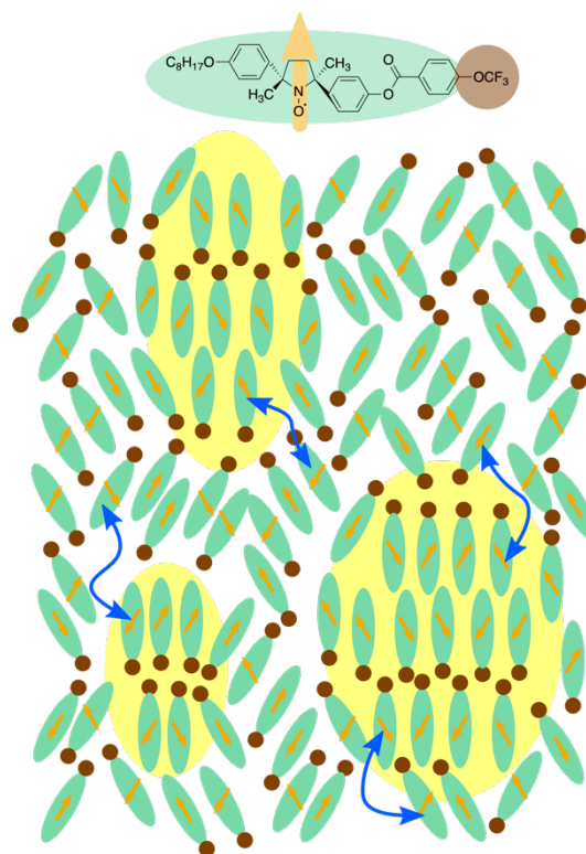
Figure 7. Molecular orientations in and out of the cybotactic cluster. Molecules of (±)- 3 have trifluoromethyl group (brown circles) and electron spins of nitroxide radical moieties (orange arrows). The molecules go into and out of the yellow-colored cybotactic clusters. Blue double-headed arrows denote molecular exchange inside and outside the cybotactic clusters.
