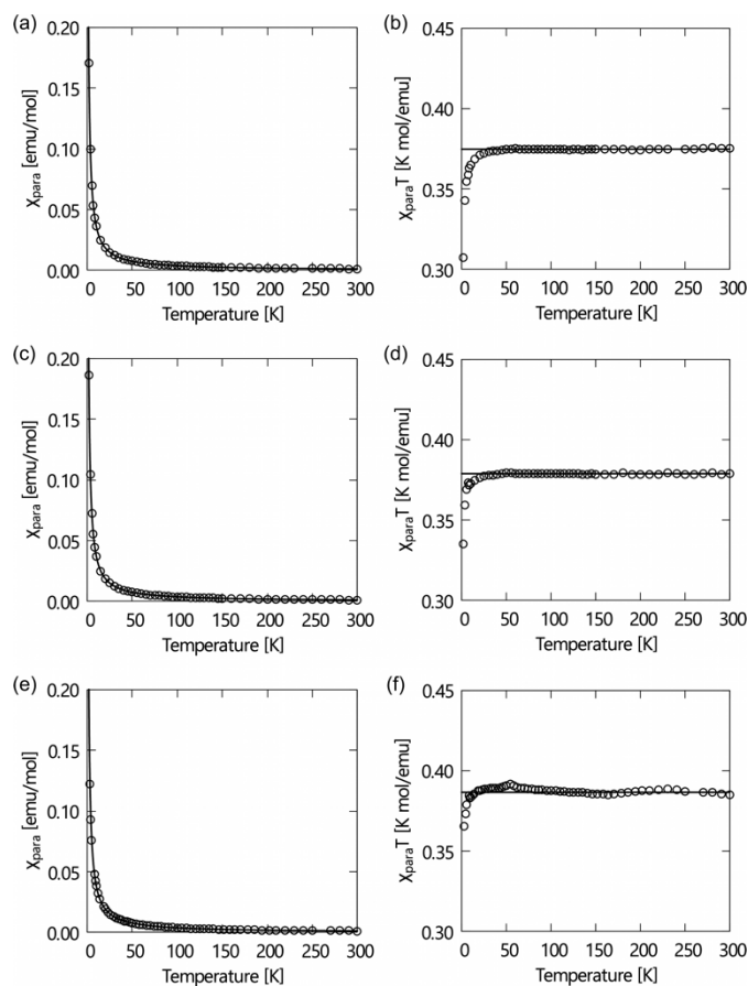
Figure 1. Magnetic properties of the newly synthesised compounds. Temperature dependences of molar paramagnetic susceptibility ( X_{para} ) and X_{para}T - T plots of (a), (b) ( \pm )- 1 , (c), (d) ( \pm )- 2 and (e), (f) ( \pm )- 3 at a field of 0.5 T in the heating process (2–300 K). Open circles represent the experimental data, solid lines in (a), (c) and (e) show Curie-Weiss fitting curves, and solid lines in (b), (d) and (f) are horizontal lines at 0.375.
