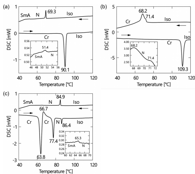
Figure 2. DSC curves of (a) ( \pm )- 1 , (b) ( \pm )- 2 and (c) ( \pm )- 3 . Standard notation gives the transition temperatures between the crystalline (Cr), smectic A (SmA), nematic (N) and isotropic (Iso) phases.
