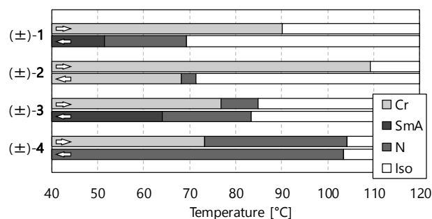
Figure 4. Phase transition behaviors of compounds ( \pm )- 1–4 . DSC analyses determined transition temperatures at a scanning rate of 5°C/min upon the heating and cooling run.
