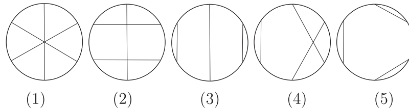
Fig. 17. Underlying Gauss chord diagrams
