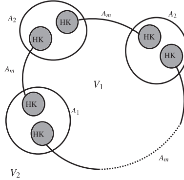
Fig.4.1. Schematic diagram of A \cap T .
