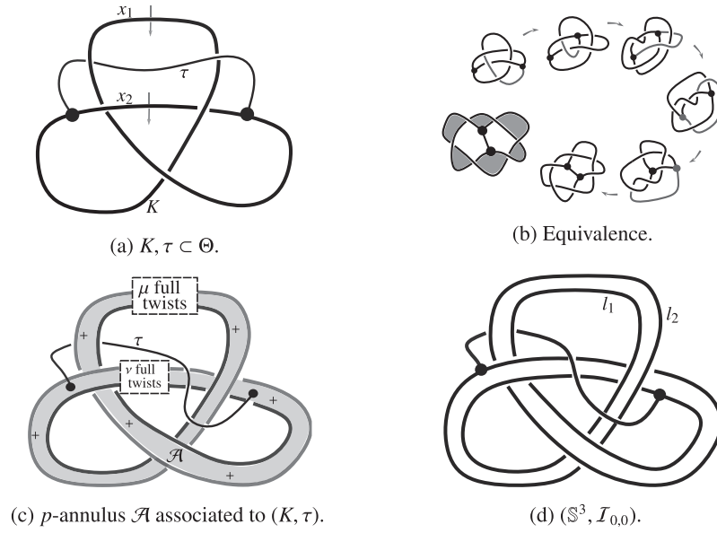
Fig. 4.3. Construction of handlebody family (\mathbb{S}^3, \mathcal{I}_{\mu,\nu}) .
