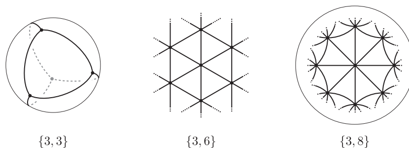
Fig. 1. Regular tessellations \{3, 3\} , \{3, 6\} and \{3, 8\} , for example
