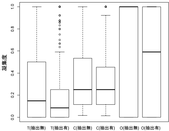
(a) jEdit
