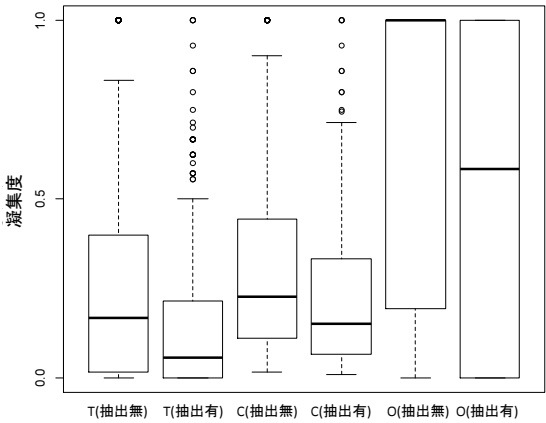
(b) Ant
