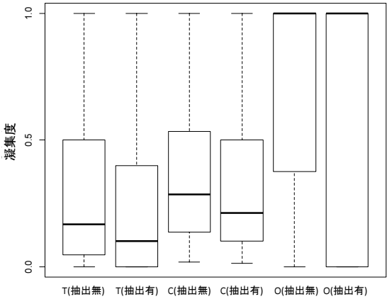
(c) ArgoUML
