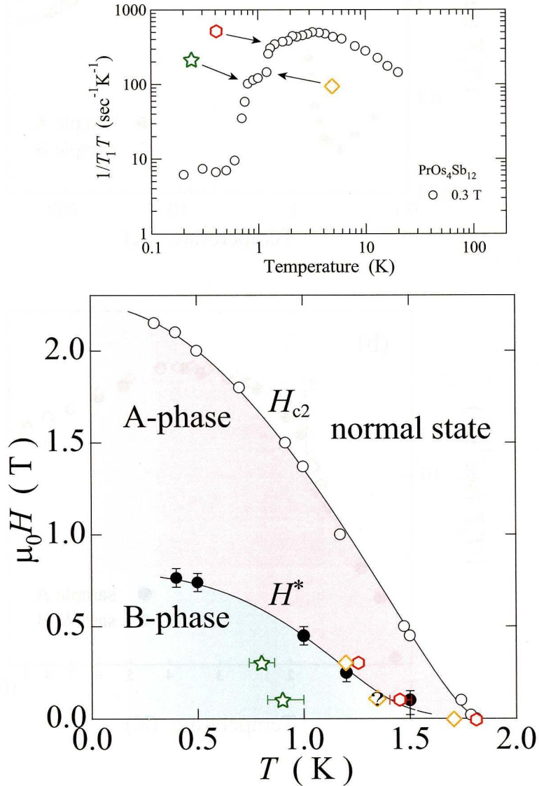
Figure 3.7: Magnetic field vs temperature phase diagram. The symbols of red open hexagons, yellow open quadrangles, and green stars represent the temperatures at which 1/T_1T indicates anomalies as shown in the upper figure.
