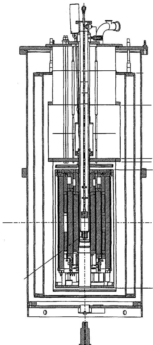
Figure 2.3: Cryostat for NMR measurement.
