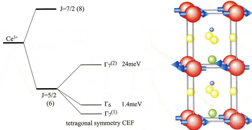
Figure 2.4: Left figure: Crystal electric field (CEF) energy scheme for CePt 3 Si. Right figure : Magnetic structure of CePt 3 Si. The Ce magnetic moments lie ferromagnetically in the c -plane and stacked antiferromagnetically along the c -axis. 5
