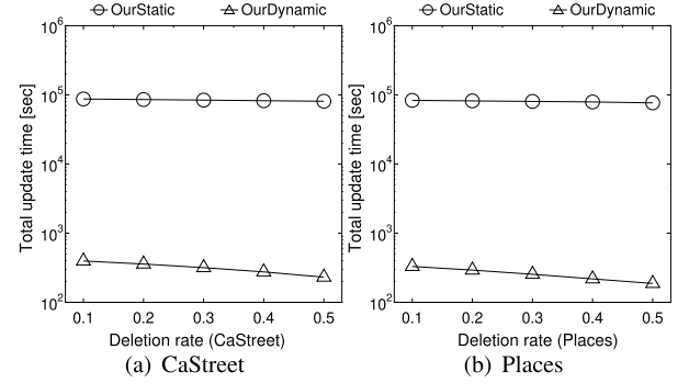
FIGURE 5. Impact of deletion rate.
