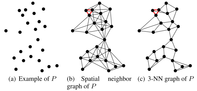
FIGURE 1. Illustration of our idea. Red edges form the top-1 weighted spatial triangle.
