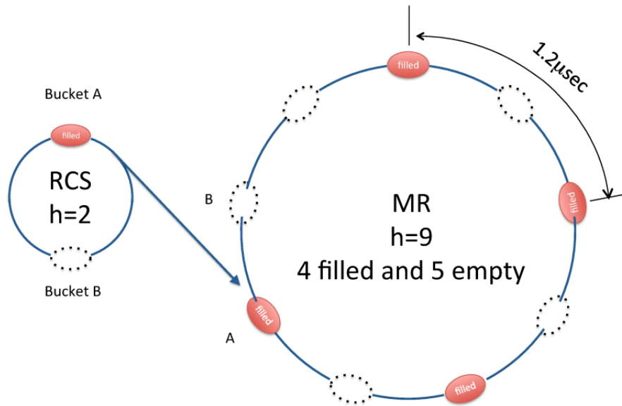
Figure 2.4: The COMET pulse beam layout [18]. The bunches are separated by 1.17 \mu\text{s} by filling protons in every other proton beam bucket.
