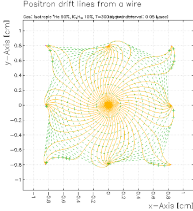
Figure 2.9: Typical drift lines for the CDC cell under a 1 T magnetic field from a Garfield simulation [18]
