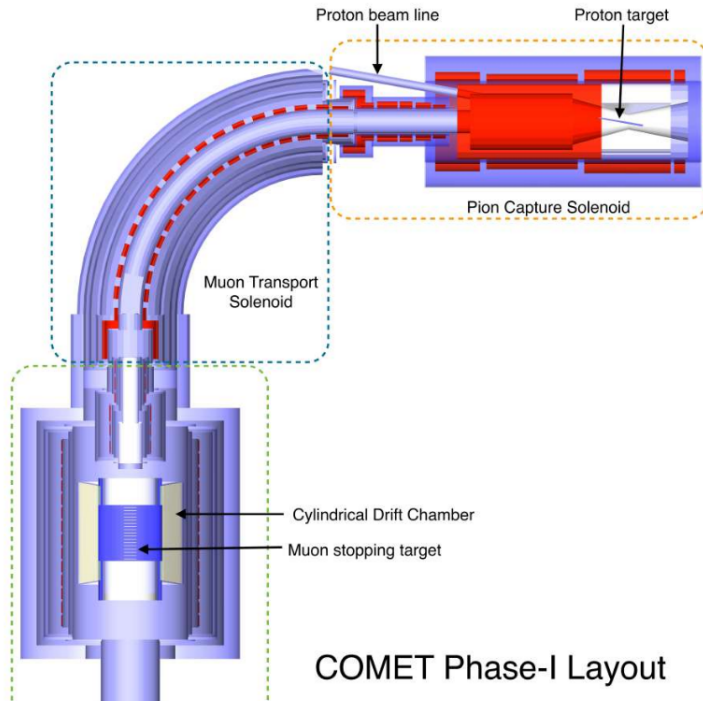
Figure 2.1: Layout of the COMET Phase-I experiment[18]
