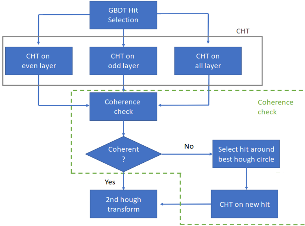
Figure 6.21: Sketch of process flow
