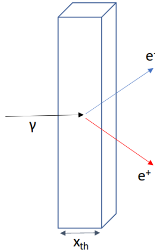
Figure 11.7: Monte-Carlo simulation setup to optimize converter inner wall thickness. Photon are shoot at a wall with a thickness x_{th} where they convert to produce electron-positron pairs
