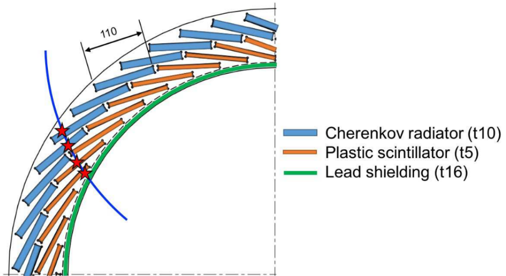
Figure 2.10: Layout of a hodoscope ring with the example of a 4-fold coincidence [18]
