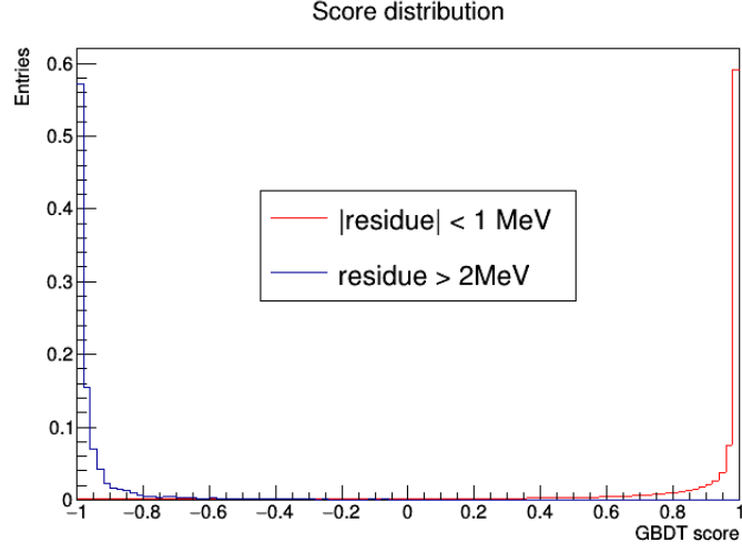
Figure B.7: Score distribution
