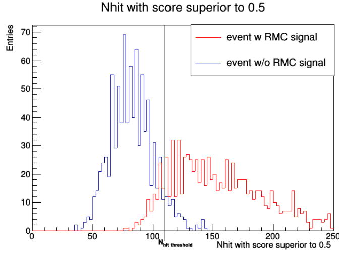
Figure 5.11: Number of hit with a GBDT score superior to 0.5 for event with RMC signal and without RMC signal. N_{\text{hit threshold}} = 110
