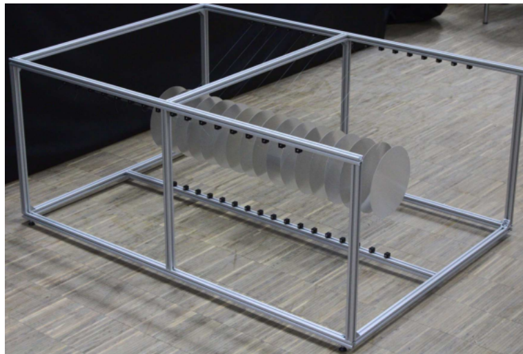
Figure 2.7: A mock-up muon stopping target [18]
