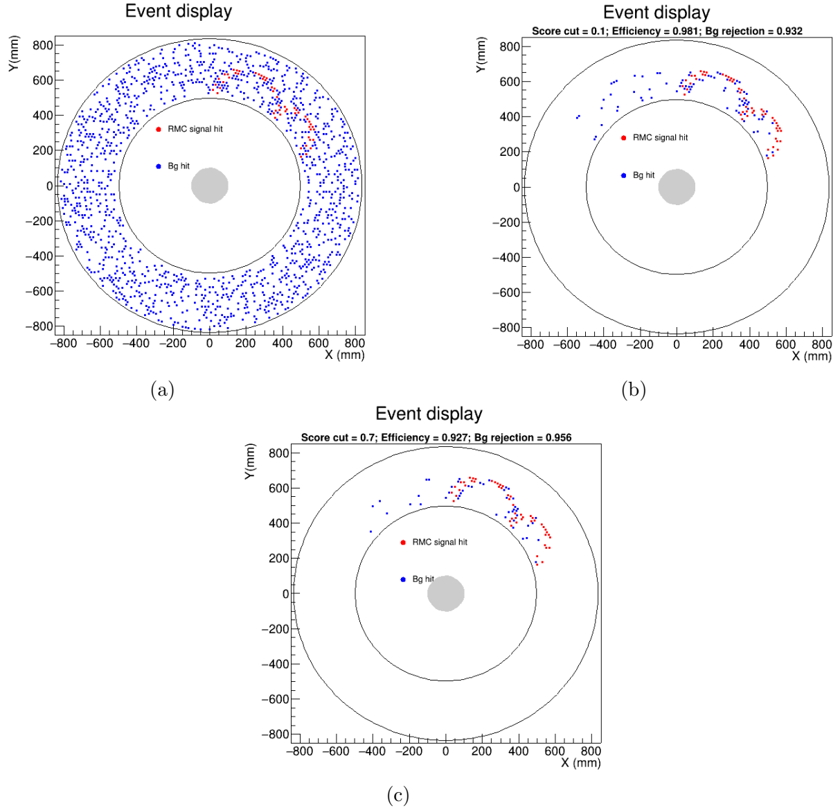
Figure 6.12: Projection of background and signal hits in the middle of the detector. (a) No selection on the hit, (b) hits with a cut on GBDT score superior to 0.1, and (c) hits with a cut on GBDT score superior to 0.7
