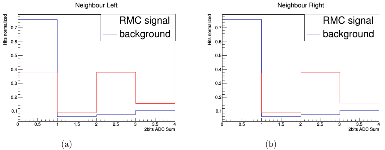
Figure 5.6: ADC sum distribution encoded in two bits for neighbors, (a) right neighbors and (b) left neighbors
