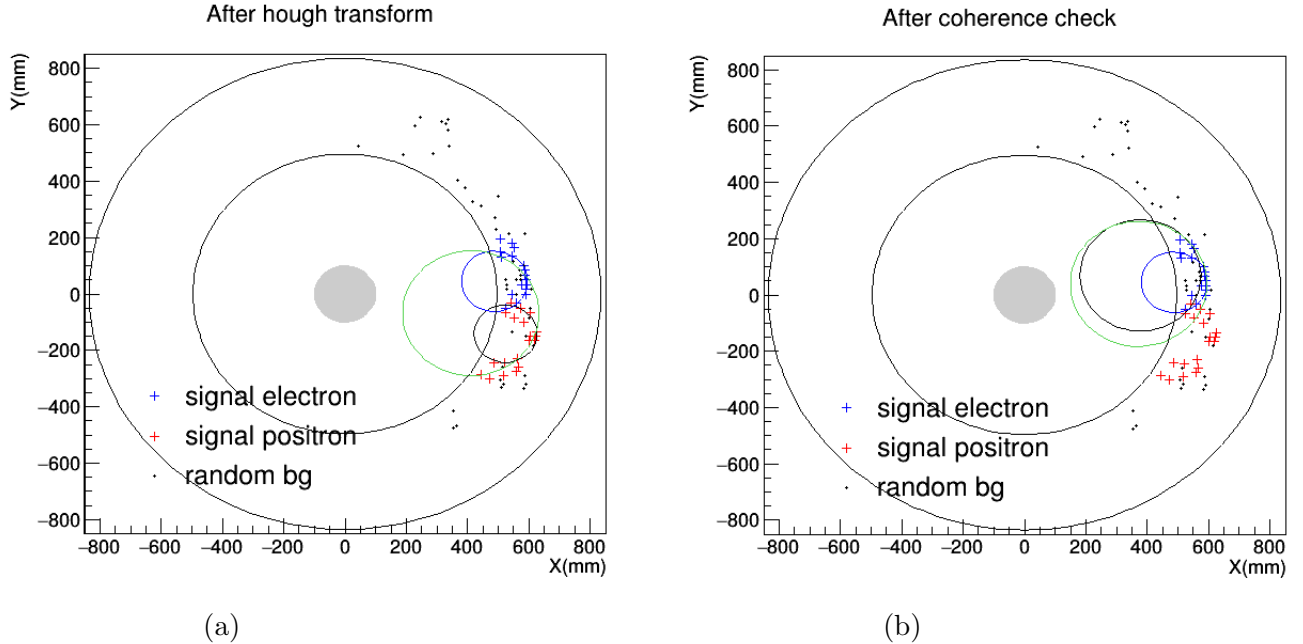
Figure 6.20: Event where none of 1st the Hough transform agree with each other, hit shown are hit with a GBDT score superior to 0.1. (a) shows that even layer found the positron track while odd layer found the electron track. All layer found a mixture of even- and odd-layer projections track (b) shows the Hough transform result adjusted to the odd layer circle
