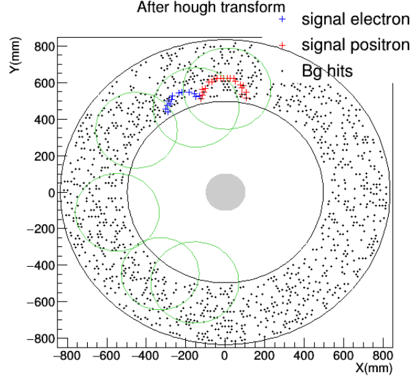
Figure 6.1: Circular Hough transform best 5 circles without applying any pre-filter.
