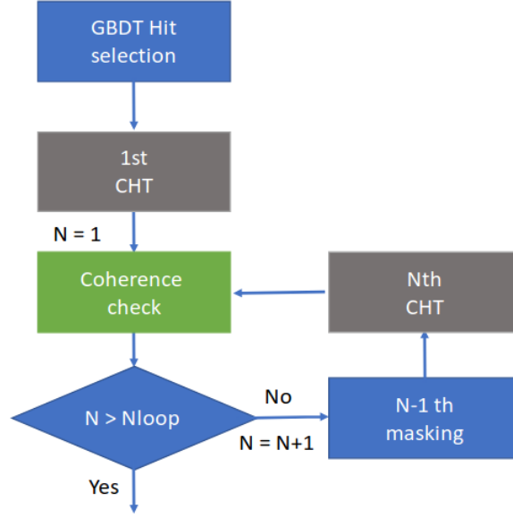
Figure 6.25: Hit filtering and track finding algorithm flow with CHT loop. The coherence check and 1st and N th CHT are shown in more detail in Figure 6.21
