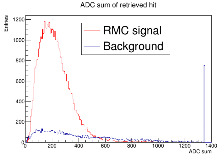
Figure 6.30: ADC sum distribution of hit retrieved with S_t = 0.4 , R_d = -20 mm and R_u = 15 mm
