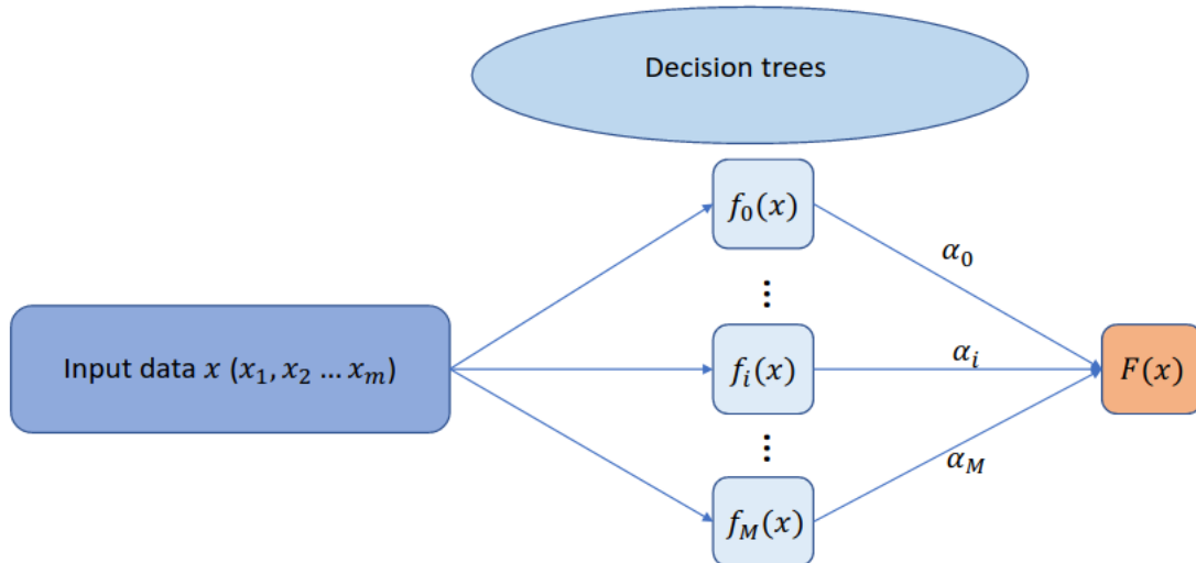
Figure A.3: Sketch of a gradient boosted tree architecture
