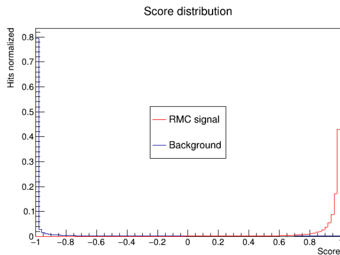
Figure 6.10: Score distribution for signal and background hits
