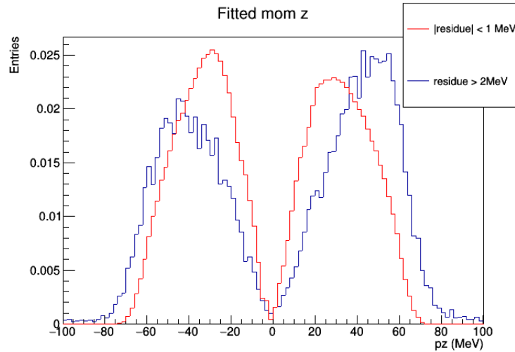
Figure B.5: Fitted Pz
