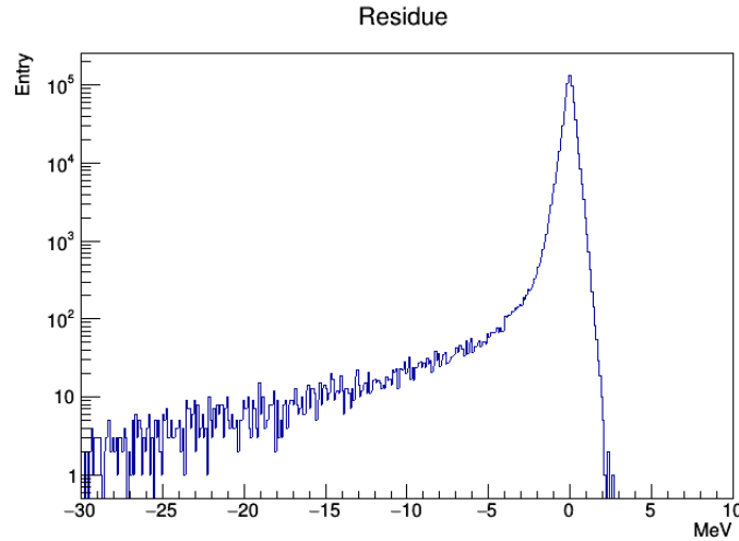
Figure 11.1: Fitting residue for \mu^- \rightarrow e^- after GBDT track fitting quality cut B
