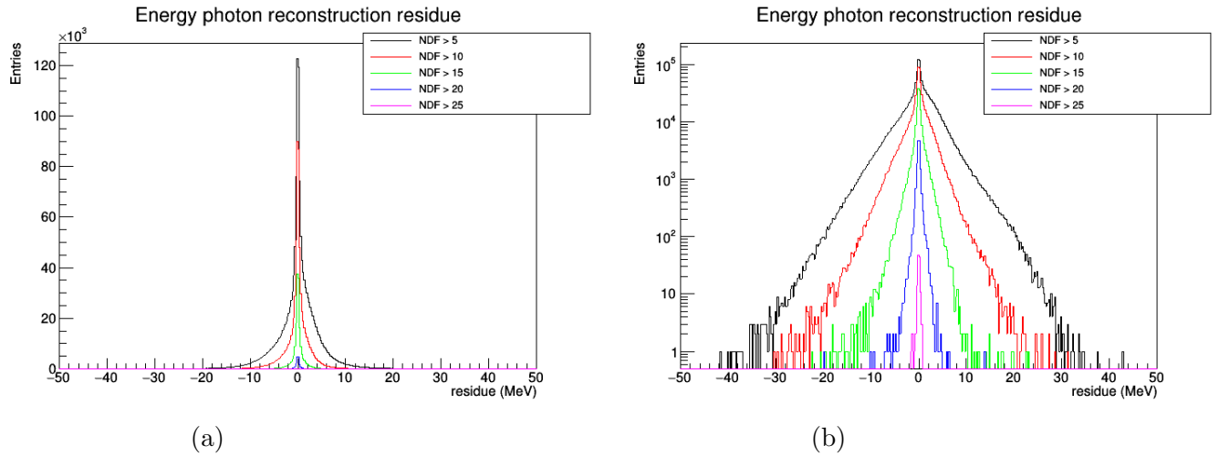
Figure 7.18: Residue on \gamma energy ( (P_{\text{fitted}})_{e^-} + (P_{\text{fitted}})_{e^+} + 2 \times m_e - E_\gamma at vertex) (a) and log scale (b) for different NDF requirement
