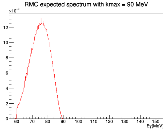
Figure 9.2: Al RMC predicted photon spectrum in the COMET Phase-I experiment by the Primakoff model with k_{\max} = 90 MeV
