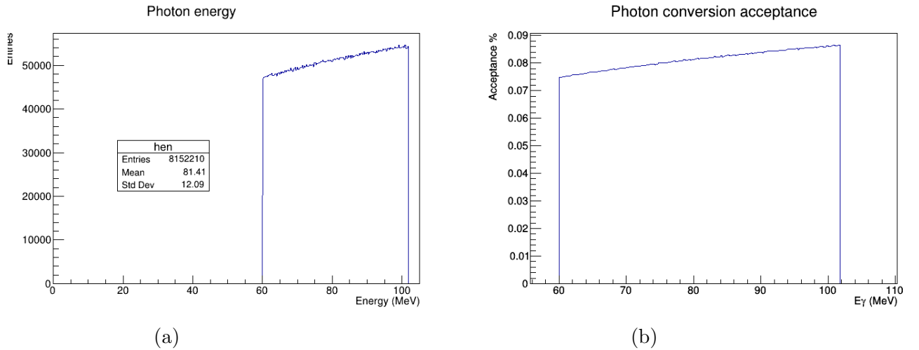
Figure 4.3: (a) Energy distribution of the photon conversion in inner wall (b) Inner wall photon conversion acceptance
