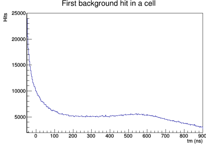
Figure 4.15: First background hit in a cell time t_m distribution [52]
