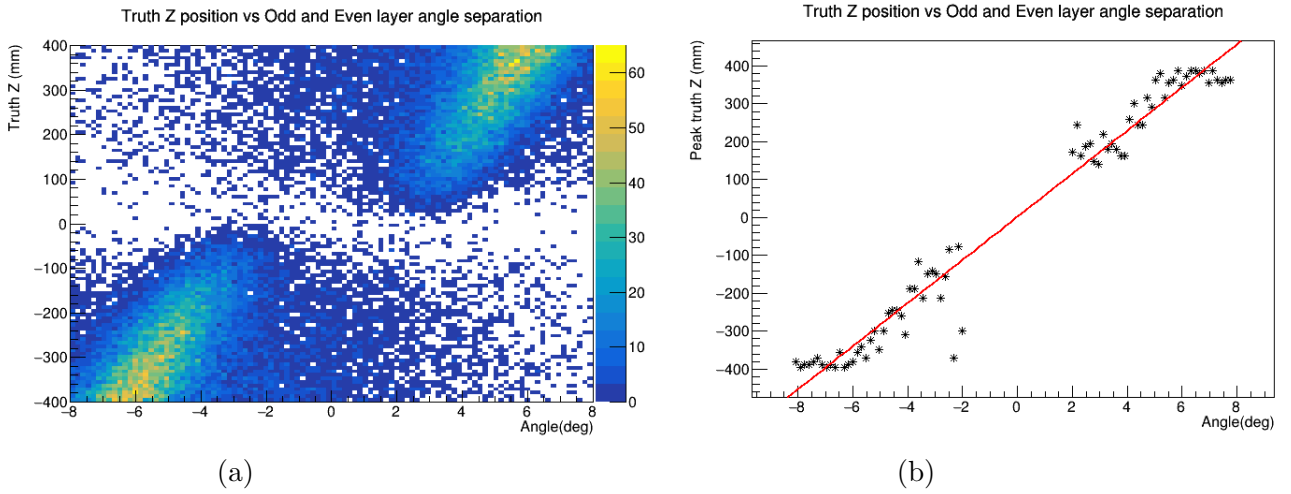
Figure 7.11: Truth first hit Z position vs Found Hough transform angle shift between the odd and even layer. (b) is showing mean Z distribution truth and 1st degree polynomial fit.
