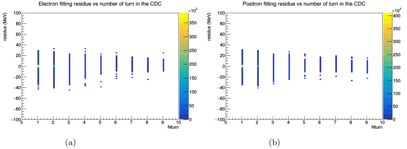
Figure 7.20: Residue of fitted electron (a) and fitted positron (b) versus the number of turn they make in the detector.
