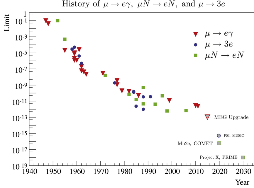
Figure 1.1: Historical search of muon decays and future experiment sensitivity projection of future experiment (MEG update, Mu2e, COMET, Project X and PRIME) [4]
