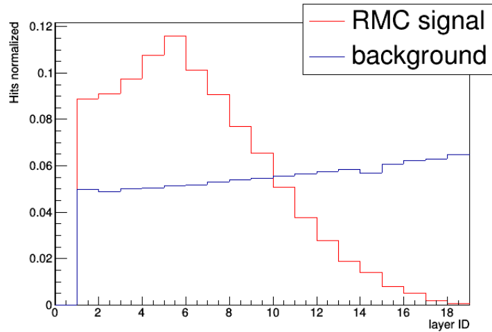
Figure 5.1: Radial position distribution of the RMC signal and background CDC hits. Guard layer hit are not shown.
