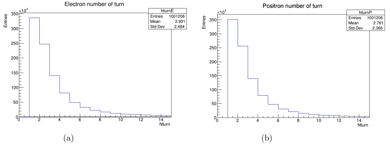
Figure 4.10: Number of turn in the chamber (a) for electron (b) for positron
