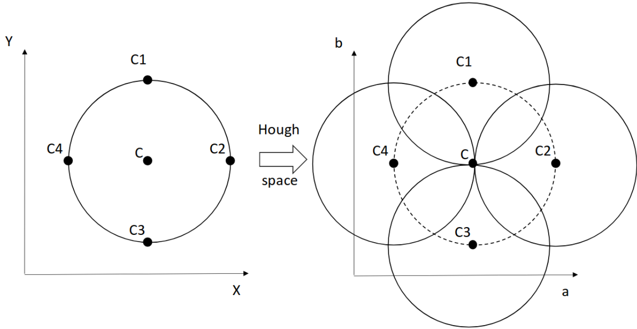
Figure 6.13: Transform of a circle C in the Hough phase space
