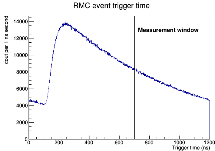
Figure 4.8: Trigger timing distribution. The COMET Phase-I experiment measurement time window is from 700 to 1170 ns. The measure time window contains 30.1% of the total triggered RMC events
