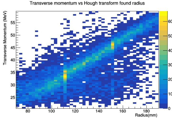
Figure 7.4: Transverse momentum vs. circular Hough transform found radius for electron and positron single turn events
