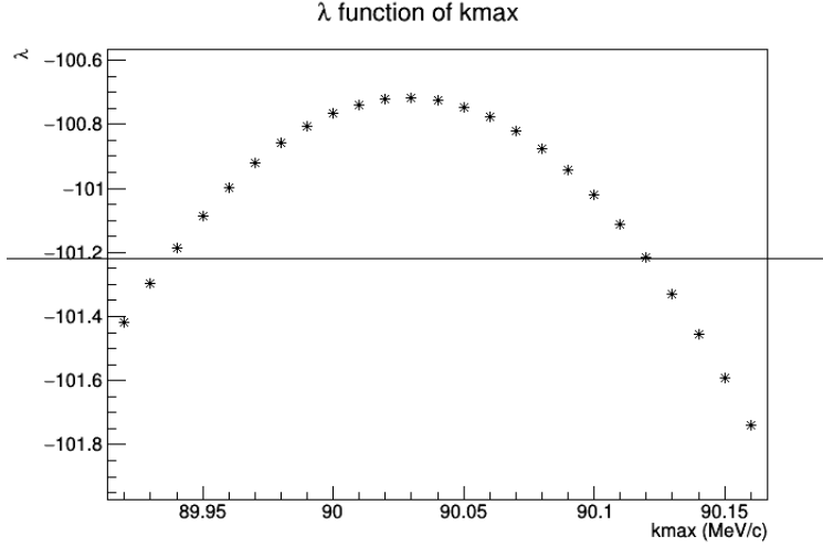
Figure 9.5: Log \lambda function of k_{\max} . The intersection between the black line and the \ln \lambda function shows the 63% confidence interval. k_{\max} = 90 \text{ MeV} , 200 bins were used to calculate the \ln \lambda function
