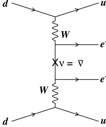
Figure 1.2: Feynman diagram of 0\nu\beta\beta in a Majorana neutrino model
