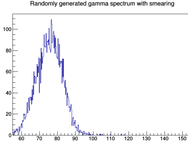
Figure 9.4: Spectrum generated with N_{\text{RMC}} = 16 k corresponding to 100 days running. R_\gamma = 1.40 \times 10^{-5} and k_{\max} = 90 MeV
