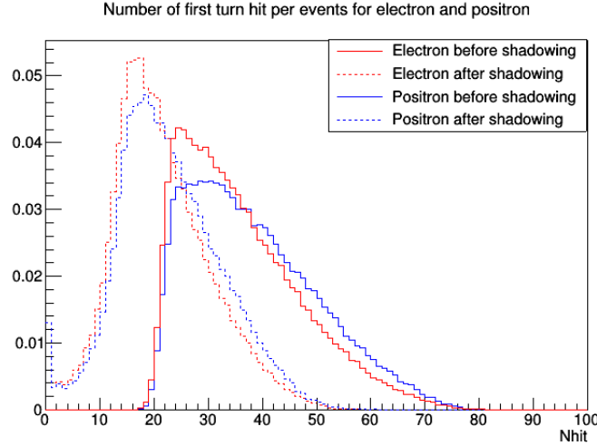
Figure 10.4: Number of first turn hit per events for electron and positron before and after shadowing effect with 45% background occupancy.
