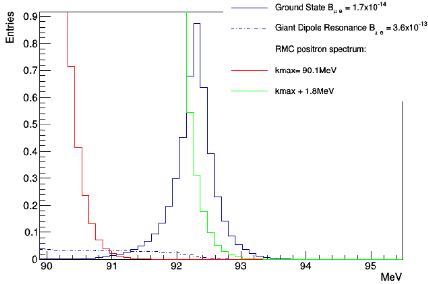
Figure 1.6: The expected reconstructed positron spectrum in the COMET Phase-I experiment. Calculation details are explained in chapter 11
