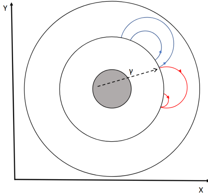
Figure 7.21: Sketch of an event where both the electron and positron track describes two turns in the CDC
