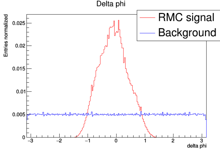
Figure 6.6: Delta \phi distribution
