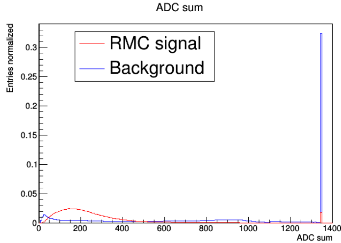
Figure 6.3: ADC sum distribution
