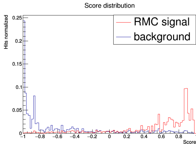
Figure 5.7: Score distribution for RMC signal and background hits
