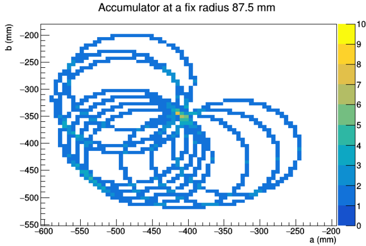
Figure 6.14: Image showing circular Hough transform accumulator at a fixed radius, color shows how many times a bin have been crossed by the different circles
