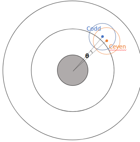
Figure 7.10: Sketch showing the shift between the Odd layer and Even layer Hough transform results
