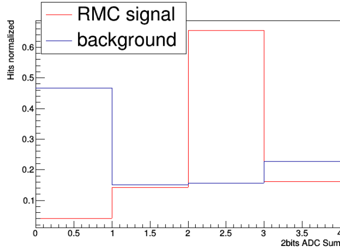
Figure 5.4: 2-bit encoded ADC sum distribution for signal and background hits
