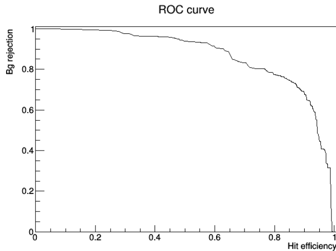
Figure 5.9: Hit filtering ROC curve.
