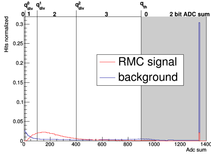
Figure 5.3: ADC sum distribution. q_{th} = 900 and q_{div}^i = (6, 100, 400) are threshold for the ADC conversion into the 2-bit ADC sum.
