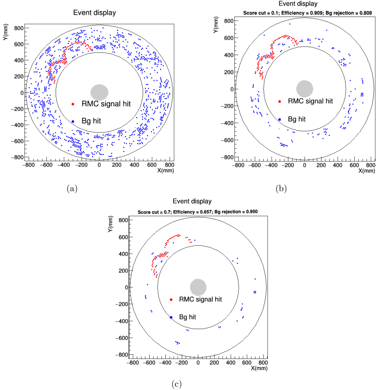
Figure 5.10: Projection of background and signal hits in the middle of the detector. (a) No selection on hit, (b) Hit with a LUT score superior to 0.1, and (c) Hit with a LUT score superior to 0.7
