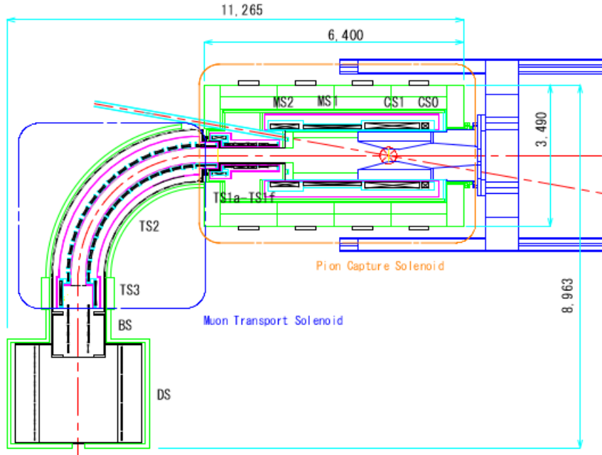
Figure 2.5: Layout of the COMET Phase-I Experiment [18]. The proportion of the different part are shown in m
