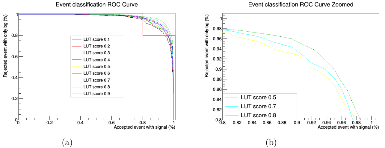
Figure 5.12: Event classification ROC Curve. (a) Event classification ROC curve for different LUT score (b) Event classification ROC curve only keeping the best 3 ROC curves
