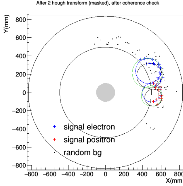
Figure 6.23: Event display with Hough transform result, hit shown are hit with a GBDT score superior to 0.1
