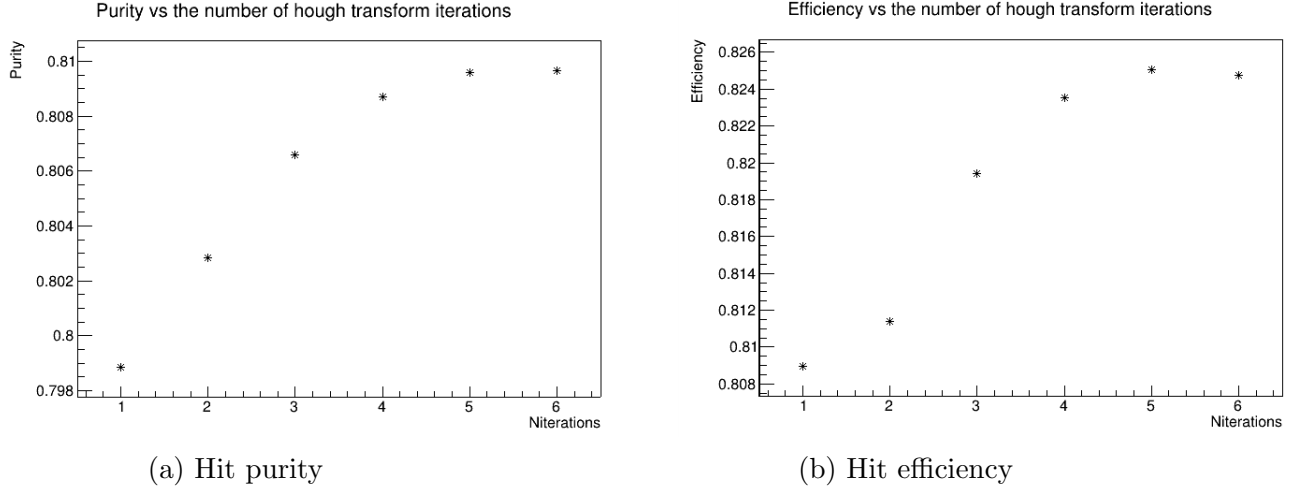
Figure 6.29: Hit purity and hit efficiency function of the number of Circular Hough transform iterations. The Circular Hough Transform is working at a score of 0.5.
