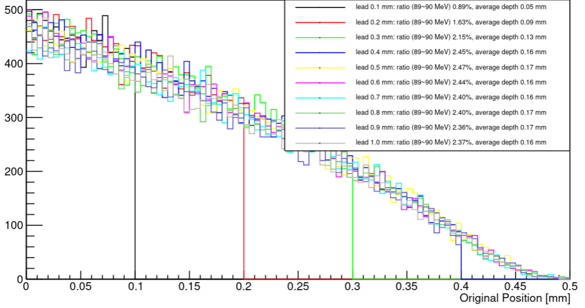
Figure 11.9: Converter thickness minus photon conversion depth for different converter thickness [74]
