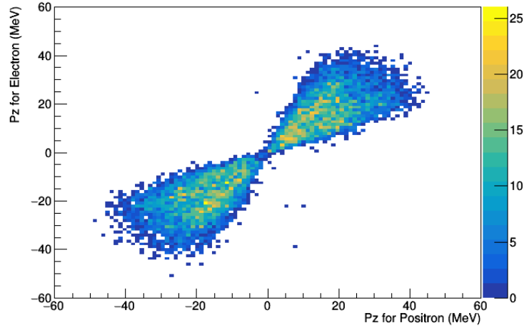
Figure 7.8: P_{Z_{ini}} for electron vs. P_{Z_{ini}} for positron from the Monte-Carlo.
