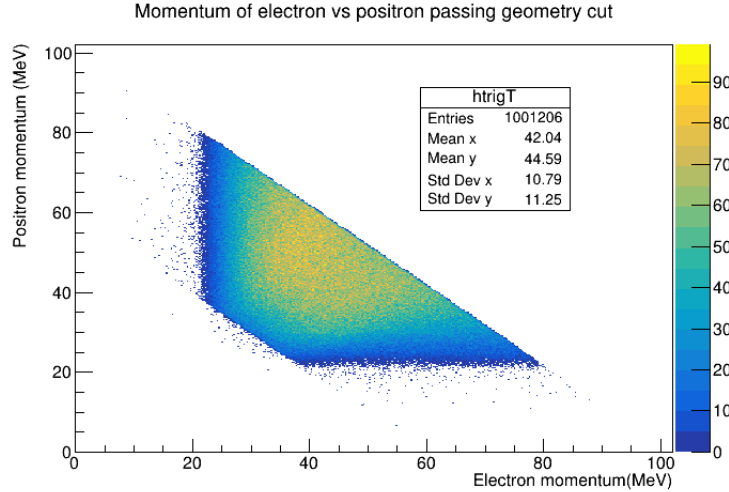
Figure 4.7: Momentum distribution of electron vs positron satisfying the geometrical condition of both reaching the 5th layer and having a CTH 4-fold coincidence
