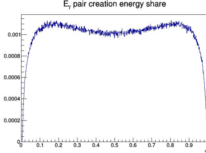
Figure 11.2: Energy share between the electron and the positron \epsilon = (E_{e^-} + m_e)/E_\gamma
