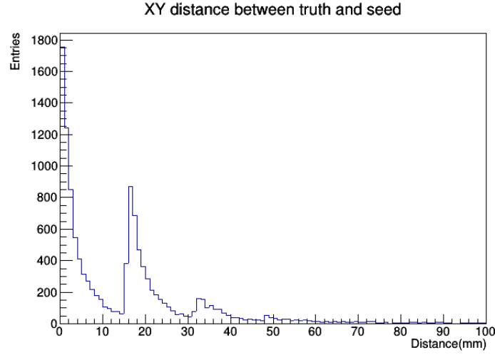
Figure 7.12: XY distance between truth and seed
