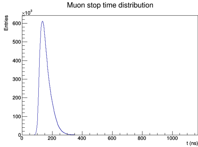
Figure 4.2: Muon stopping time distributio in the muon stopping target
