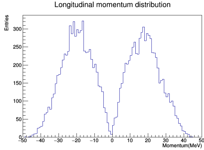
Figure 7.9: Distribution of longitudinal momentum for single turn electron and single turn positron
