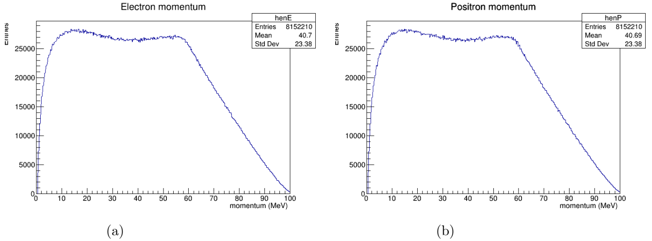
Figure 4.5: (a) Electron momentum at production. (b) Positron momentum at production
