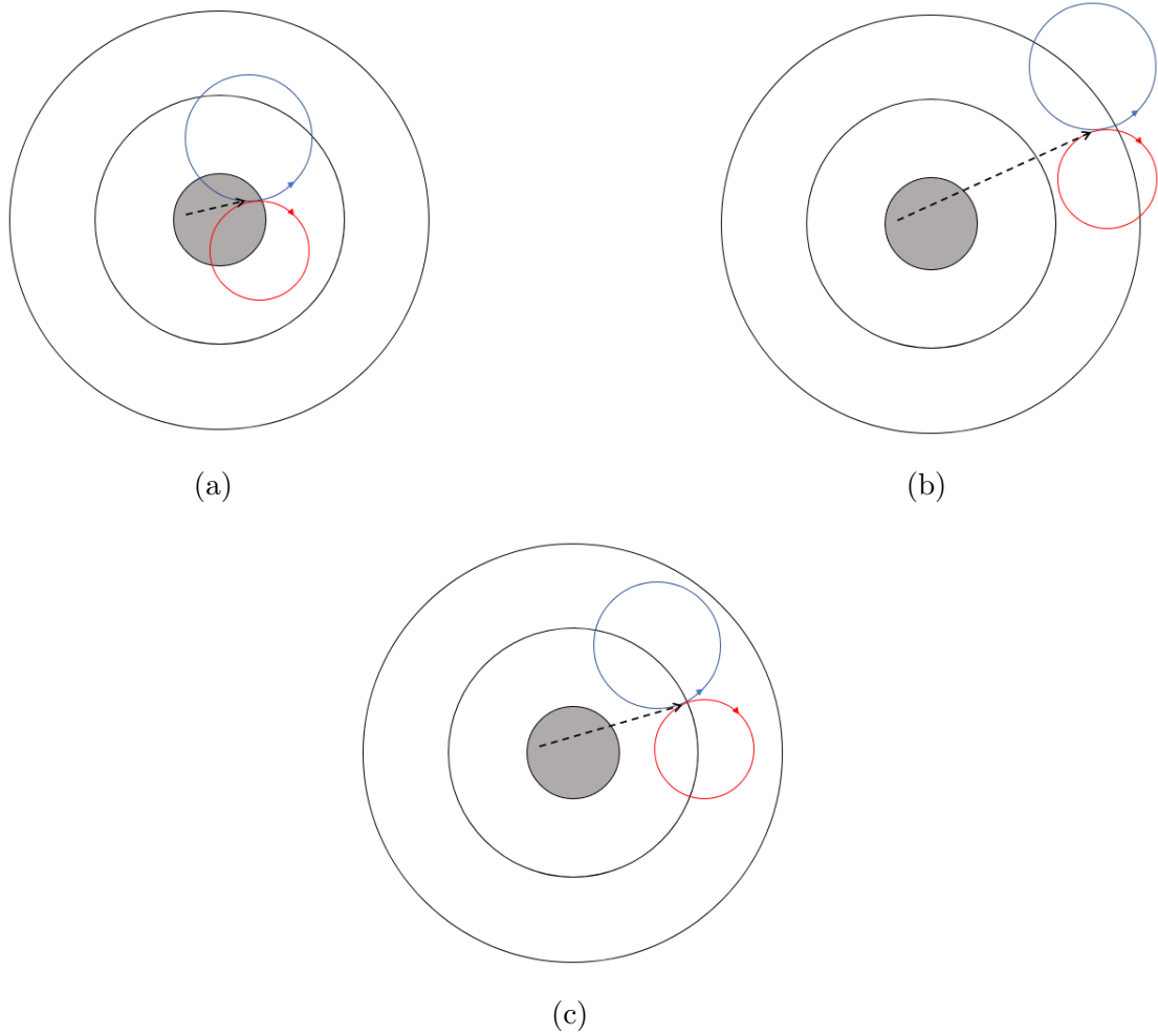
Figure 3.1: Sketch of a photon (dash line) converting into an electron (blue) and positron (red) pair in (a) the muon target, (b) deep within the CDC, and (c) within the CDC inner wall.
