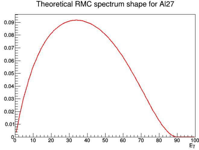
Figure 9.1: Theoretical RMC spectrum shape for ^{27}\text{Al} with k_{\max} = 90 MeV.
