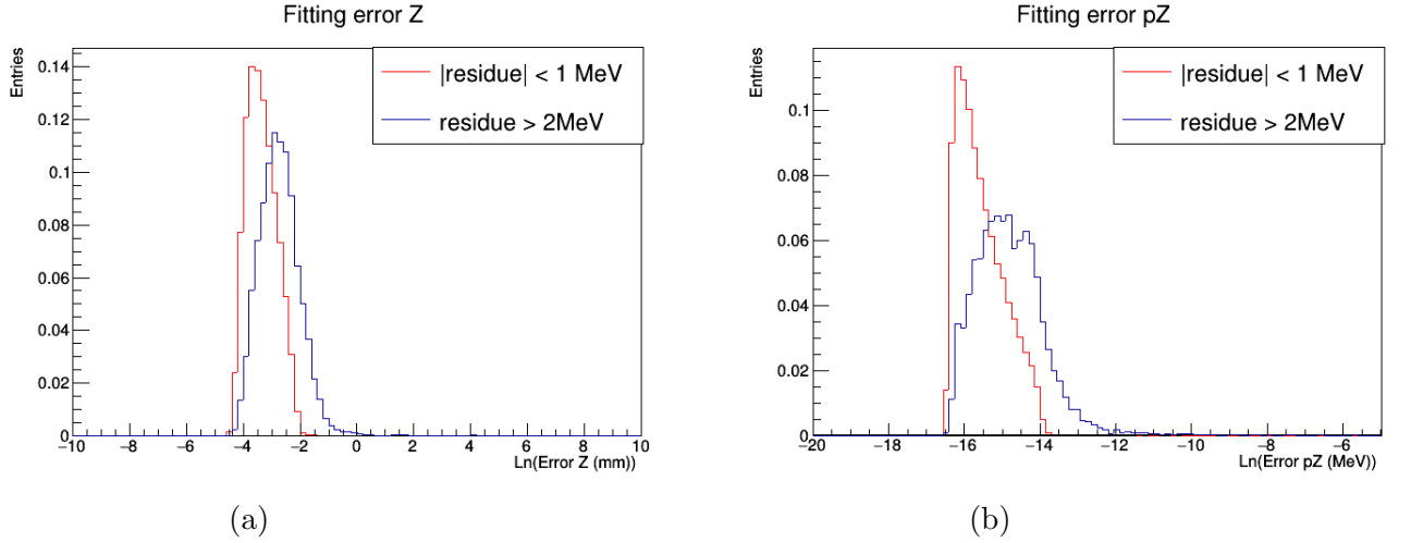
Figure B.6: Genfit longitudinal position (a) and momentum (b) fitting error
