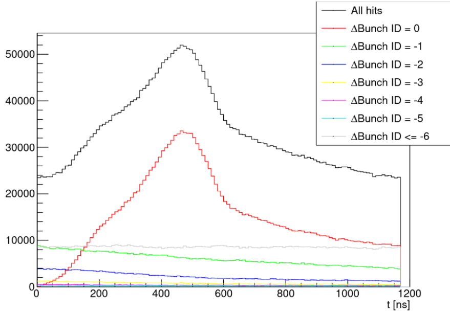
Figure 4.12: Number of hit in the detector function of the time. The total number of hit in the current frame is shown in black. The hit due to the different bunch are shown in different colors [52]
