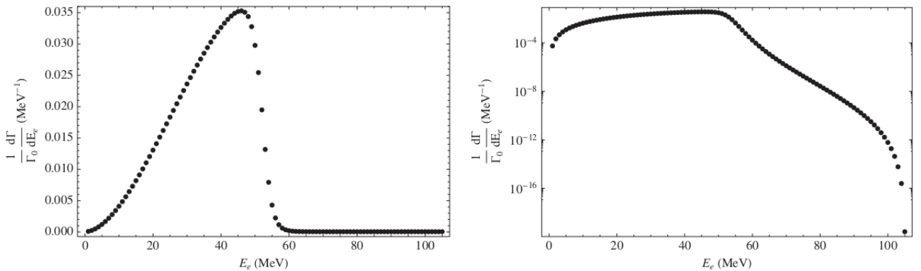
Figure 2.2: DIO electron spectrum for calculated for ^{27}\text{Al} [49]
