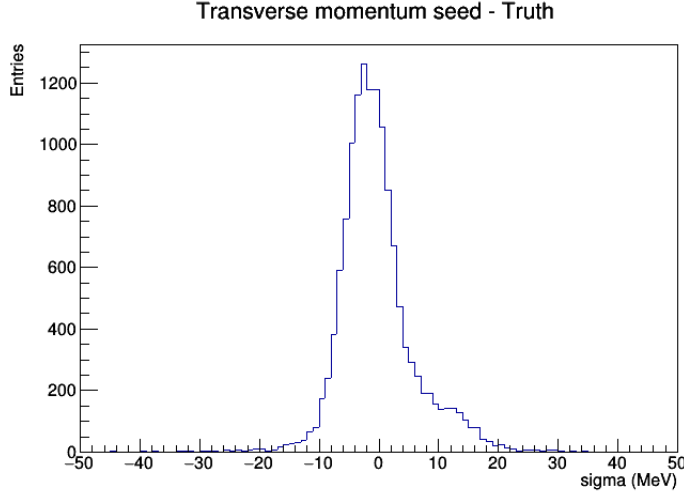
Figure 7.14: transverse momentum seed minus the Monte-Carlo initial transverse momentum
