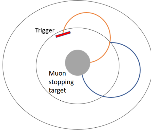
Figure 10.2: Sketch of coincidental DIO event
