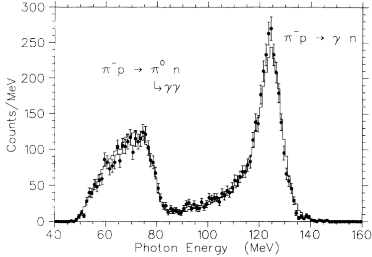
Figure 11.5: Photon energy spectrum from the TRIUMF experiment on a hydrogen target [41]. The data are given by the histogram line and the solid circles are the Monte Carlo results.
