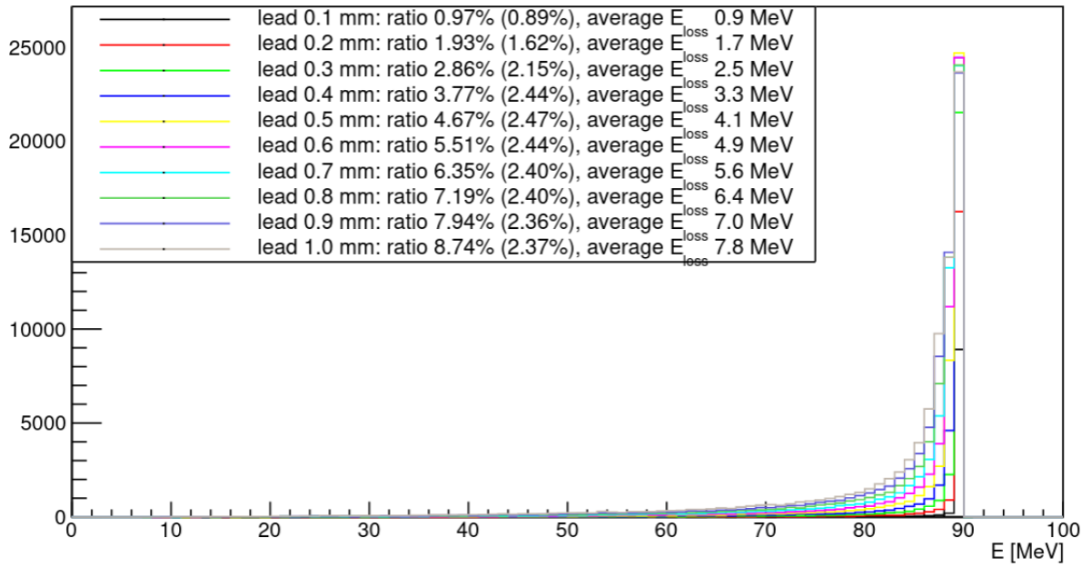
Figure 11.8: Electron-positron pairs energy after escaping the converter for different converter thickness[74]
