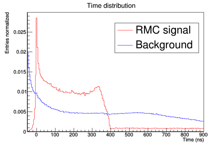
Figure 4.17: Time distribution of RMC signal and background hits
