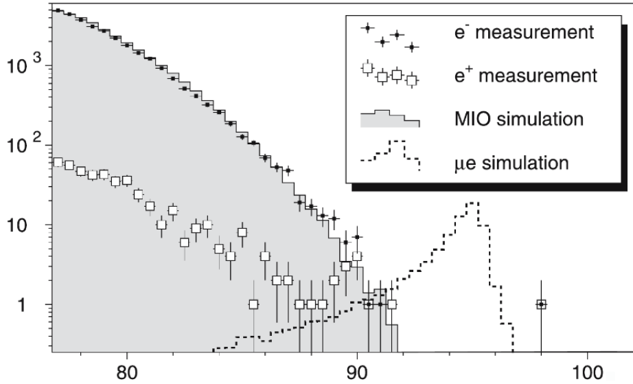
Figure 1.7: SINDRUM-II experiment e^- and e^+ spectra on an ^{197}\text{Au} target [21].
