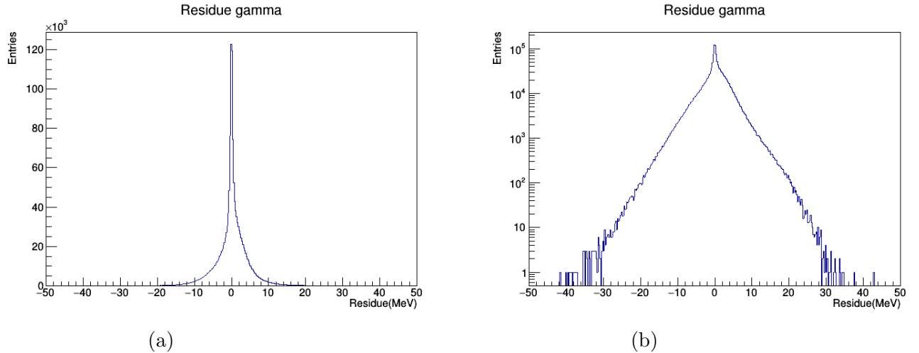
Figure 7.19: Residue on \gamma energy ( (P_{fitted})_{e^-} + (P_{fitted})_{e^+} + 2 \times mass_e - E_{\gamma \text{ at vertex}} ) (a) and log scale (b)
