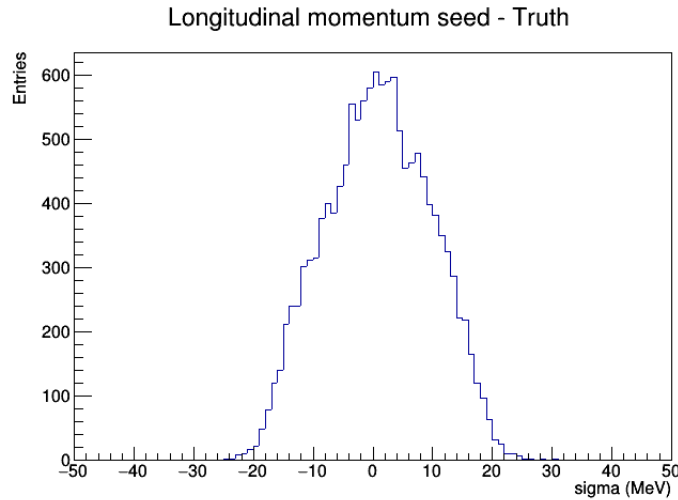
Figure 7.15: Longitudinal momentum found minus Monte-Carlo initial longitudinal momentum
