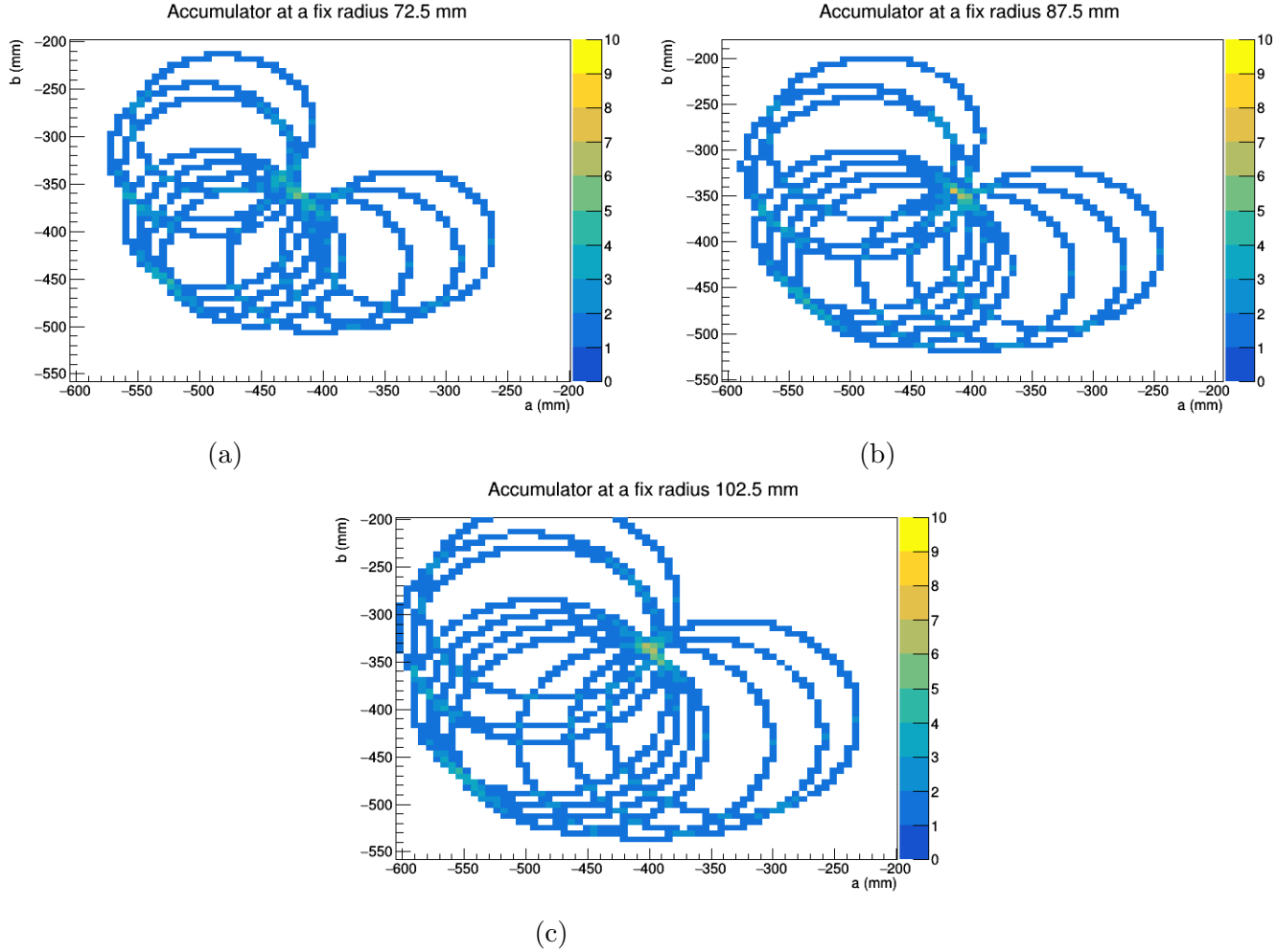
Figure 6.15: Circular Hough transform accumulator projection for 3 different radii. (a) R = 72.5 (b) R = 87.5 (real radius) (c) R = 102.5
