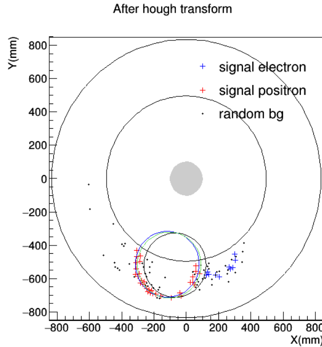
Figure 6.18: Event display with Hough transform result for all 3 projections, hit shown are hit with a GBDT score superior to 0.1.
