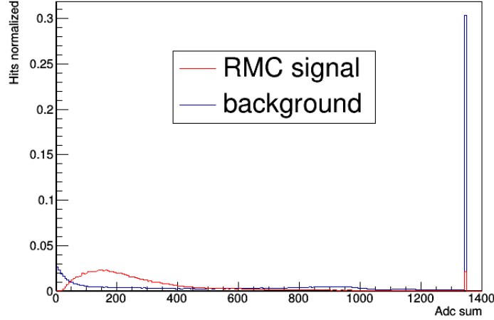
Figure 5.2: ADC sum distributions
