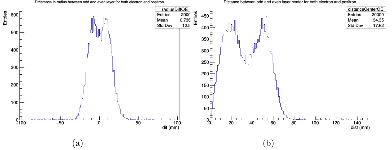
Figure 6.16: Fine tuning parameters for coherence check between odd- and even-layer projections. (a) shows the radius difference between odd- and even-layer projections circle fitting. (b) shows the distance between odd- and even-layer projections fitted circle center.
