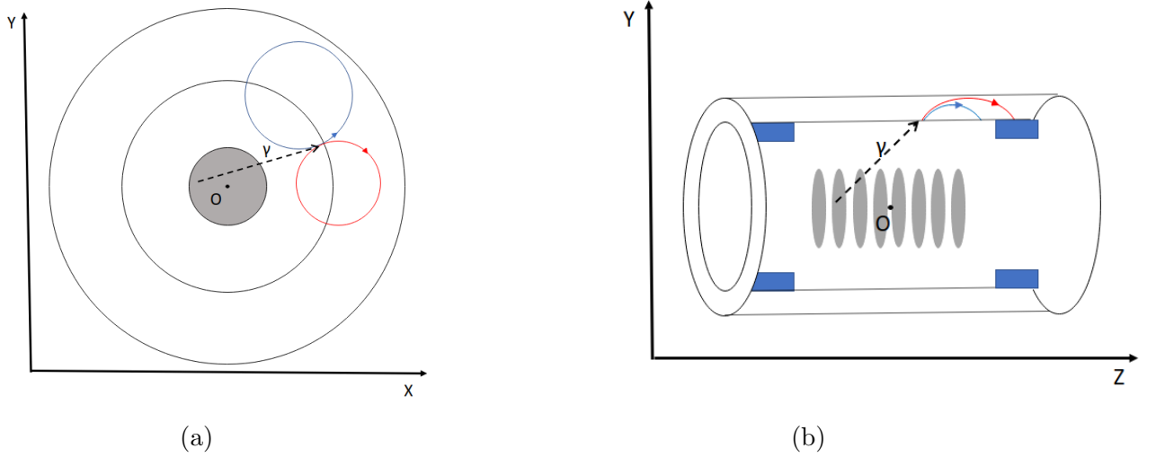
Figure 3.2: Sketch of a photon (dash line) converting into an electron (blue) and positron (red) pair in the CDC inner wall in (a) XY plane and (b) YZ plane.
