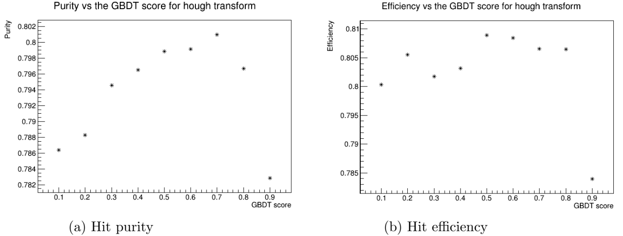
Figure 6.28: Hit purity and hit efficiency function of the GBDT score cut before the circular Hough transform
