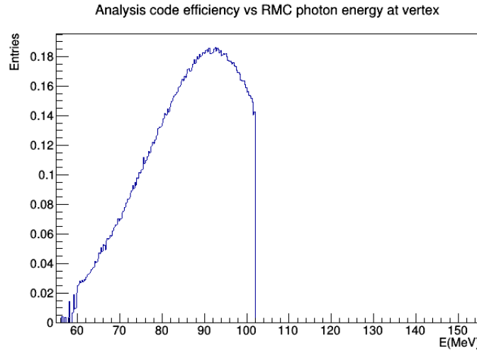
Figure 7.23: Analysis efficiency function of the photon energy before pair creation
