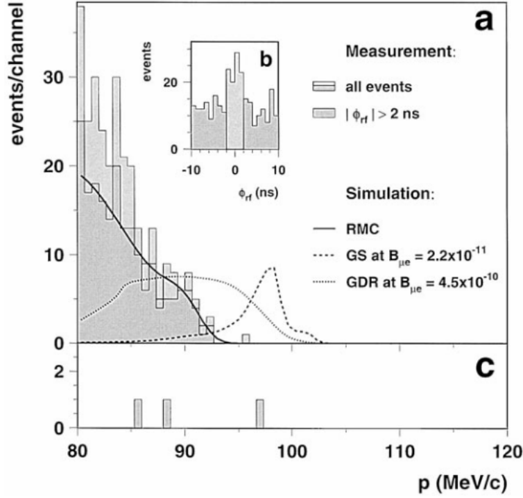
Figure 1.3: Reconstructed positron spectrum by the SINDRUM-II experiment with a titanium target overlap with simulation results [31]
