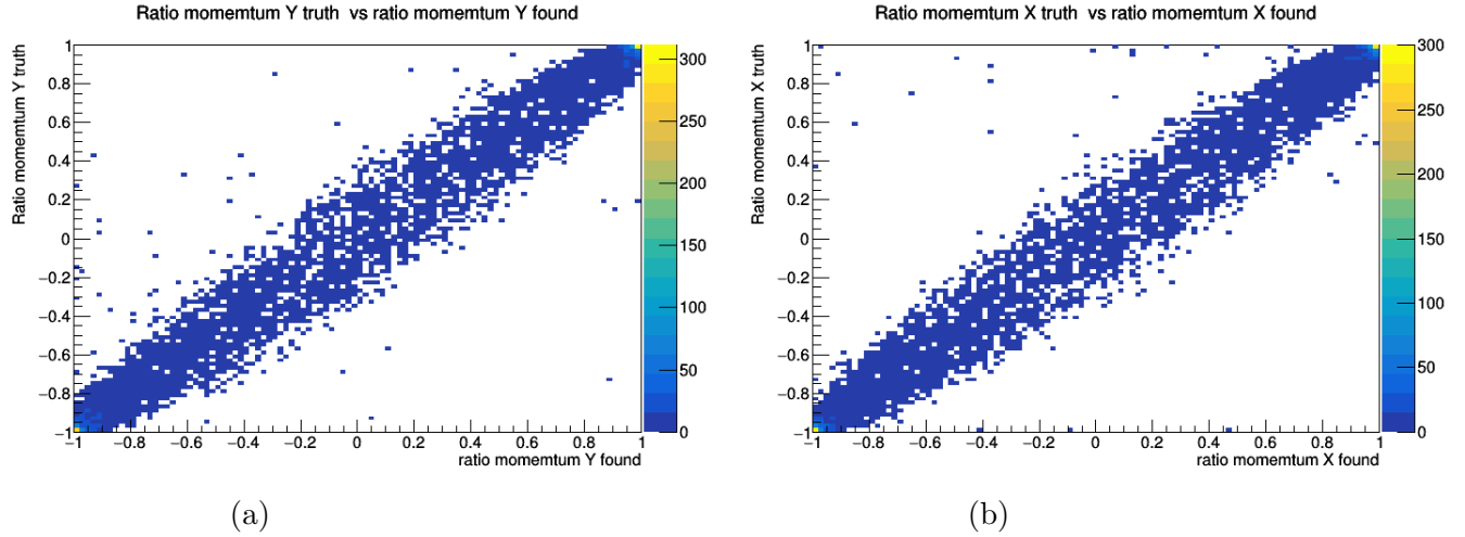
Figure 7.6: Repartition of the initial transverse momentum on the Y- (a) and X- (b) axes truth versus the ratio found
