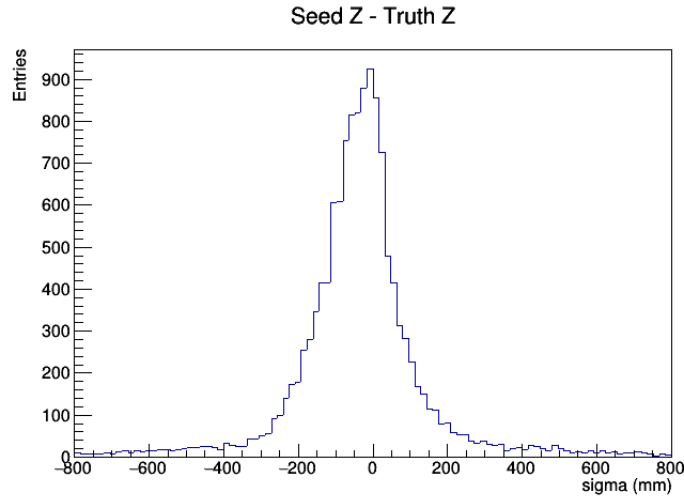
Figure 7.13: Found position Z_{\text{ini}} minus truth Monte-Carlo initial Z position
