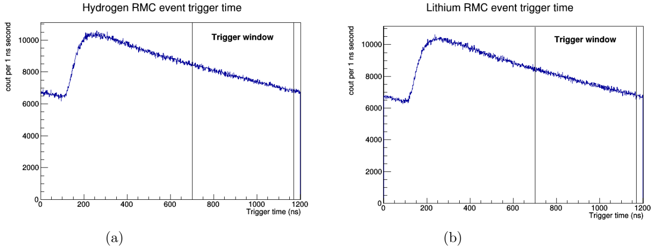
Figure 10.3: Measurement time window of RMC event by replacing the aluminum target with (a) hydrogen and (b) lithium target.
