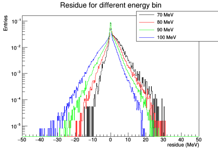
Figure 10.7: Residue function for different E_\gamma
