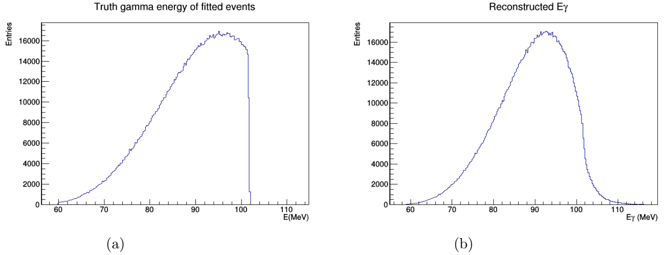
Figure 7.22: (a) Truth energy of the \gamma for fitted events. (b) Reconstructed energy of \gamma
