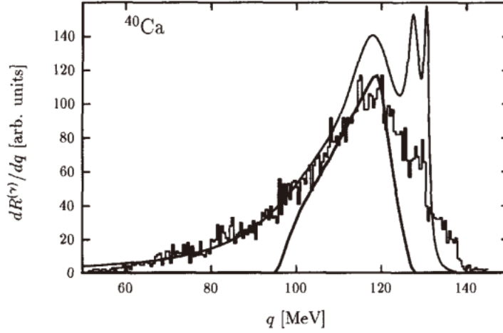
Figure 10.1: Measured momentum distribution of RPC-induced \gamma s in ^{40}\text{Ca} [64] (histogram), with two theoretical model (smooth lines)
