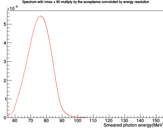
Figure 9.3: Spectrum expected to be reconstructed by the COMET Phase-I experiment assuming k_{\max} = 90 MeV
