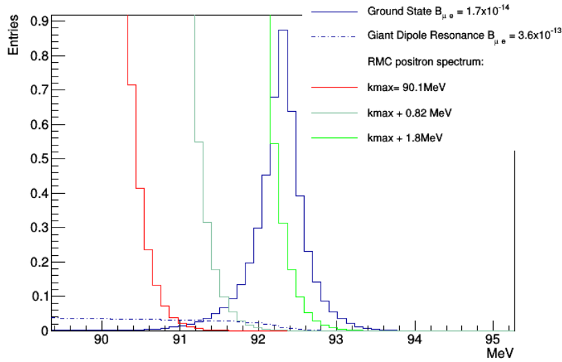
Figure 11.3: Positron spectrum due to RMC with k_{\max} at 90.1 MeV, k_{\max} + 0.82 MeV see sec. 10.2.3, k_{\max} + 1.8 MeV [43], and \mu^- \rightarrow e^+ .
