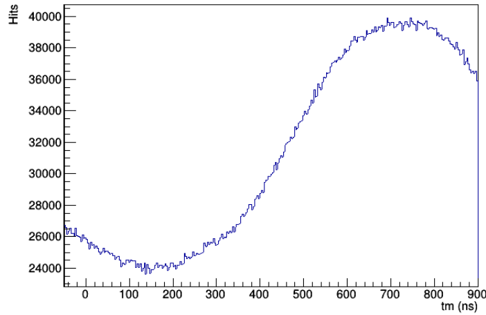
Figure 4.14: Background hits time t_m distribution [52]
