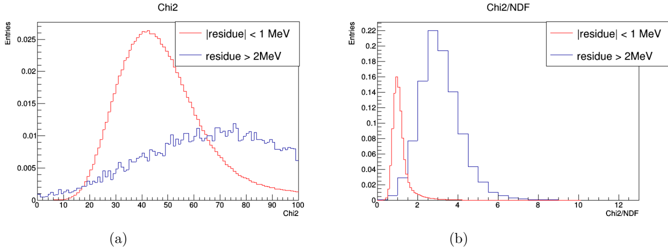
Figure B.3: \chi^2 and \chi^2/NDF for bad fitted event and for well fitted events
