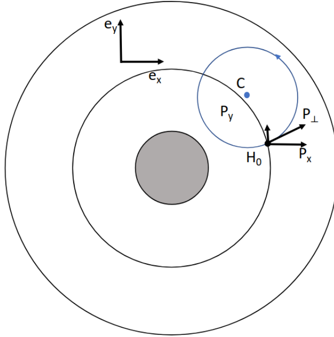
Figure 7.5: Sketch defining the different parameters from Eq. (7.4)
