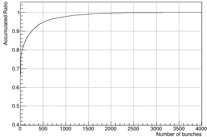
Figure 4.13: The accumulated ratio of hits in the event as a function of the number of bunches [52]
