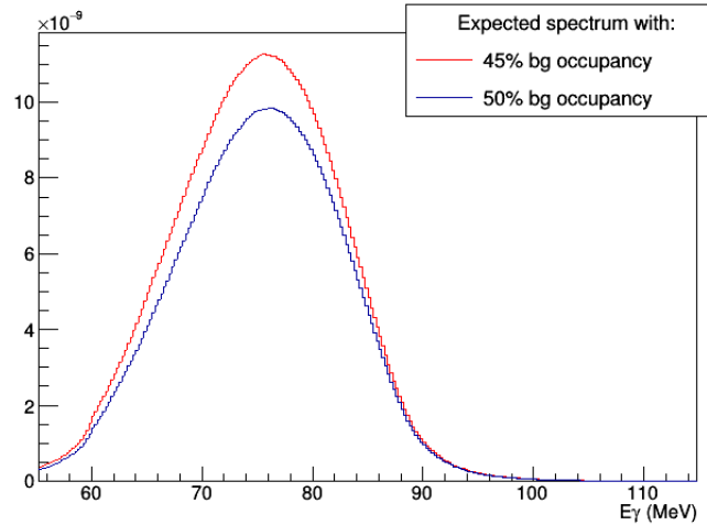
Figure 10.5: Expected shape of the RMC spectrum with analysis efficiency for 45% background occupancy and for 50% background occupancy
