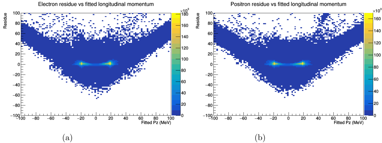
Figure 7.16: Residue function of the fitted p_z for the electron (a), and for the positron (b)
