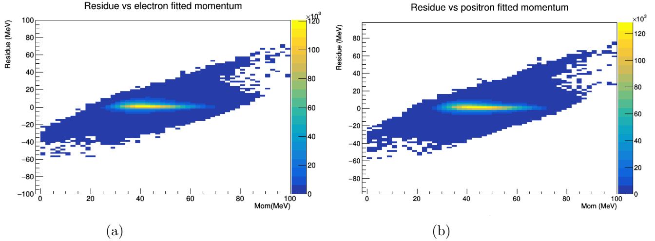
Figure 7.17: Residue function of the total fitted momentum for the electron (a), and for the positron (b)
