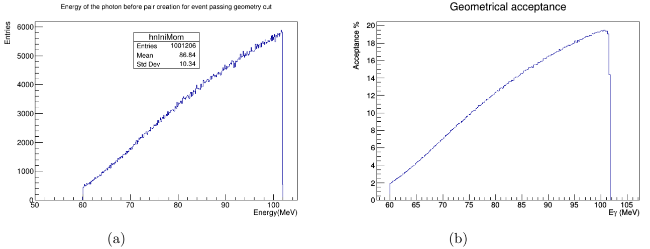
Figure 4.6: Energy distribution of the photon that created the positron-electron pair that pass the geometrical cut (a) and the geometrical acceptance (b)
