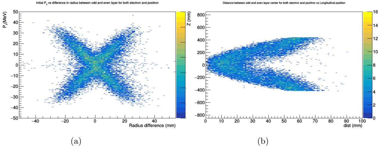
Figure 6.17: (a) Longitudinal momentum of the particle versus the even- and odd-layer projections radius difference. (b) Distance between odd- and even-layer projection circle center between longitudinal position.
