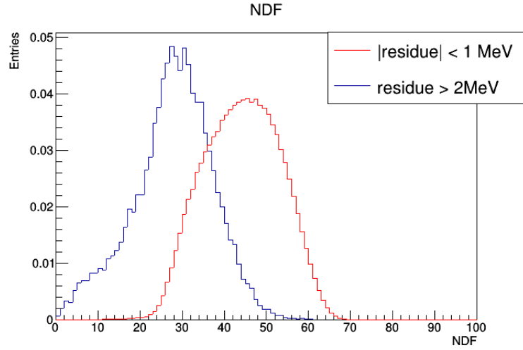
Figure B.2: NDF from the fitting
