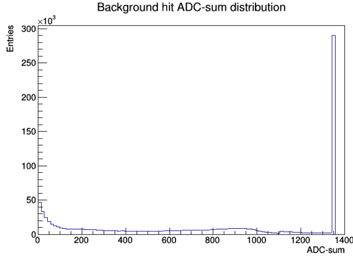
Figure 4.16: The energy deposit induced detector response, the ADC-sum, distribution for simulated background [52]
