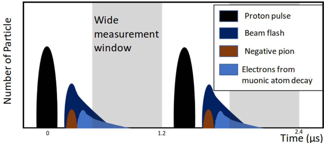
Figure 2.8: Sketch of the relation between the proton pulse, the beam flash (negative pion) and the electrons from the muonic atom decays with the trigger window.
