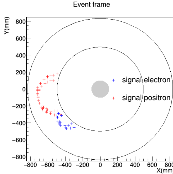
Figure 3.4: Typical RMC event projected in the XY plane coordinate. The hit position shows the wire position in the middle of the CDC.
