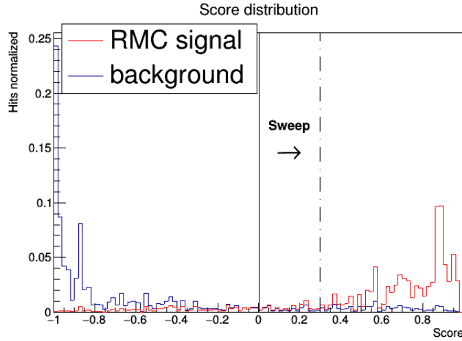
Figure 5.8: score distribution for signal and background hits with a sweeping example
