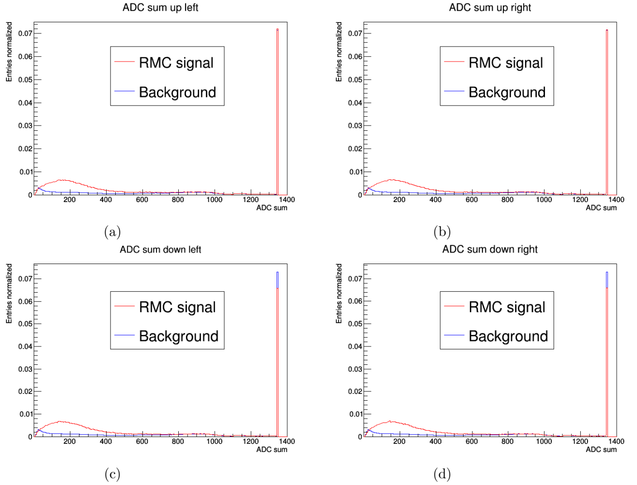
Figure 6.9: ADC sum distribution, hit with no neighbor (ADC sum = -1) have not been plotted (a) for up left neighbor (b) for up right neighbor (c) for down left neighbor (d) for down right neighbor
