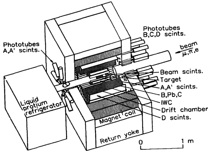
Figure 1.4: Sketch of TRIUMF RMC detector [43]
