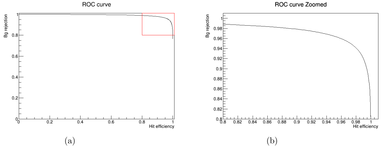
Figure 6.11: Hit filtering ROC curve. (a) full range , (b) Zoom on the right corner
