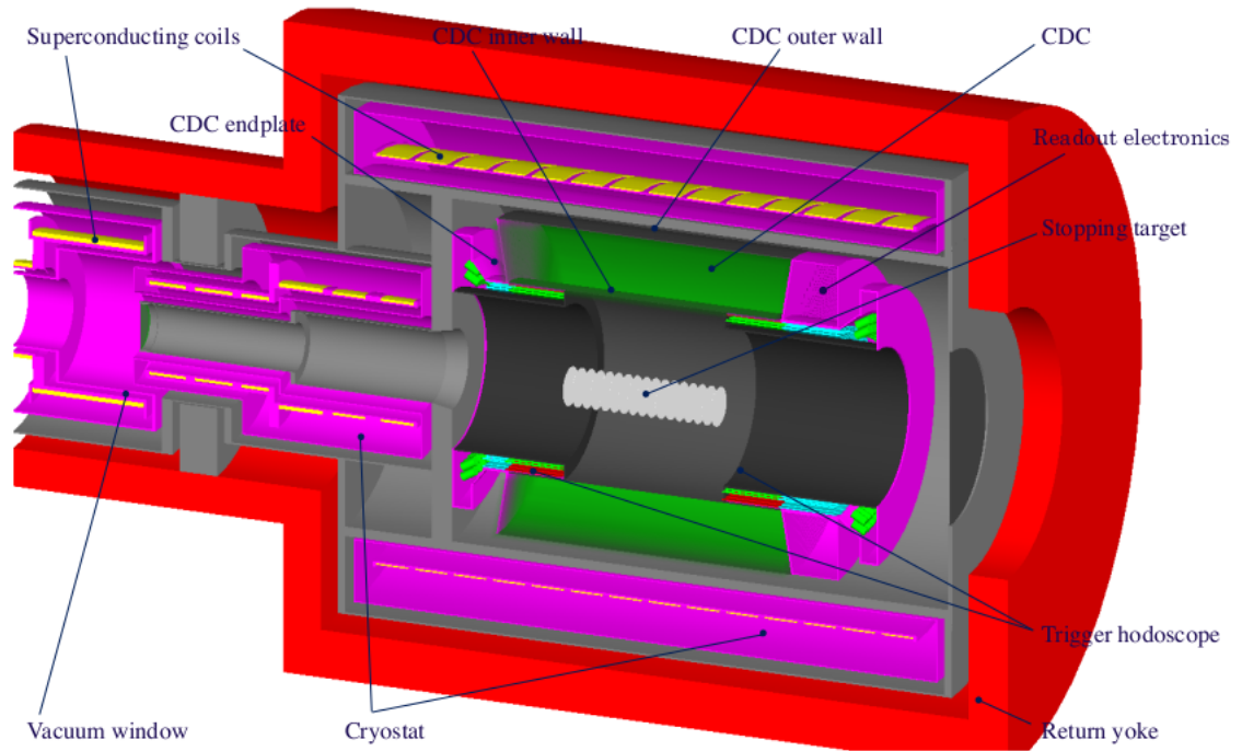
Figure 2.6: Schematic layout of the CyDet [18]
