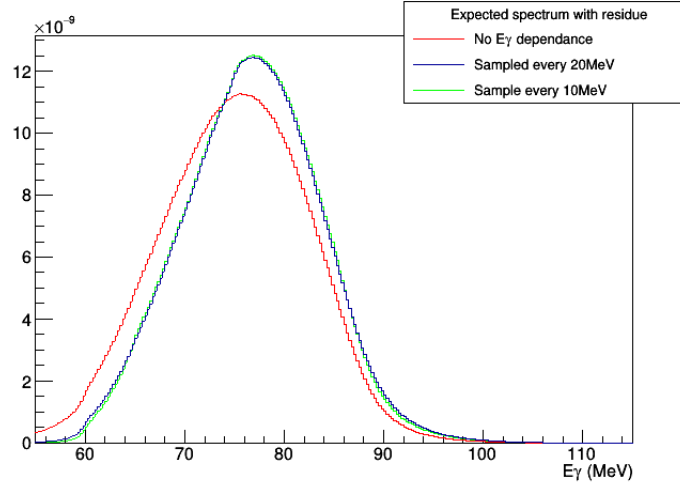
Figure 10.8: Expected ^{27}\text{Al} spectrum by taking into account 3 residue cases: with no E_\gamma dependence, with residue sampled every 20 MeV and with residue sampled every 10 MeV
