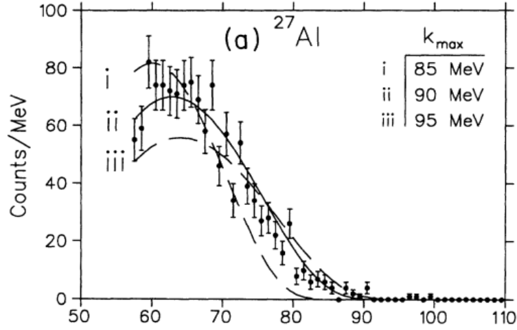
Figure 1.5: Reconstructed photon spectrum by the TRIUMF experiment with an ^{27}\text{Al} target. Solid circles are showing the measured events and the lines are showing spectrum fitting results using Primakoff model for different values of k_{\max} [43]
