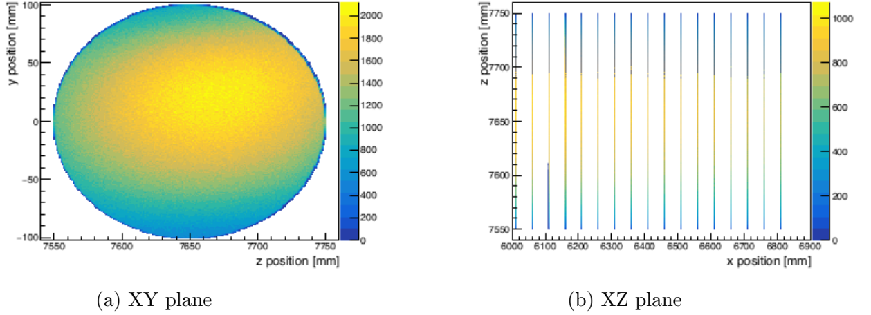
Figure 4.1: COMET Phase-I simulated muon stop position in the muon-stopping target system [18]
