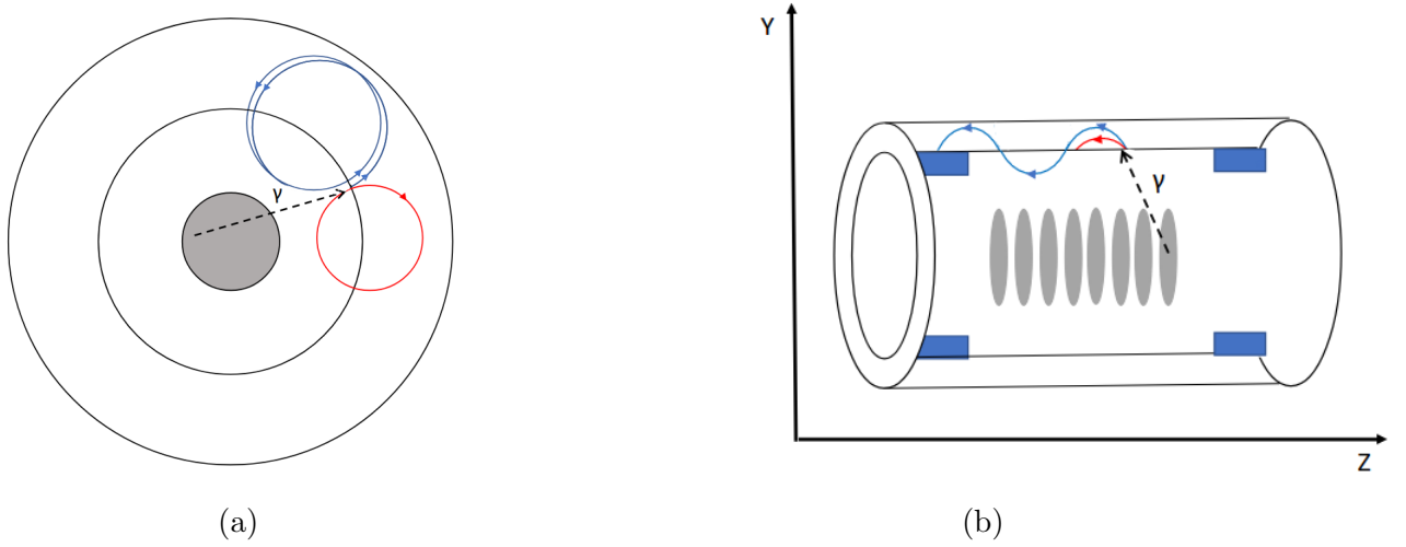
Figure 4.9: Sketch showing a case when the RMC induced electron makes two turns in the CDC before reaching the CTH in the XY plane (a) and in the YZ plane (b).
