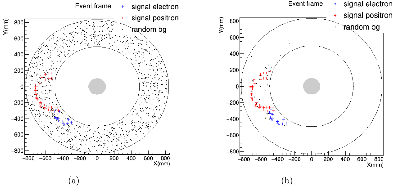
Figure 3.3: Event frame before denoising (a) and after denoising (b). The background has been generated uniformly across the sensing wires with an occupancy of 45%.
