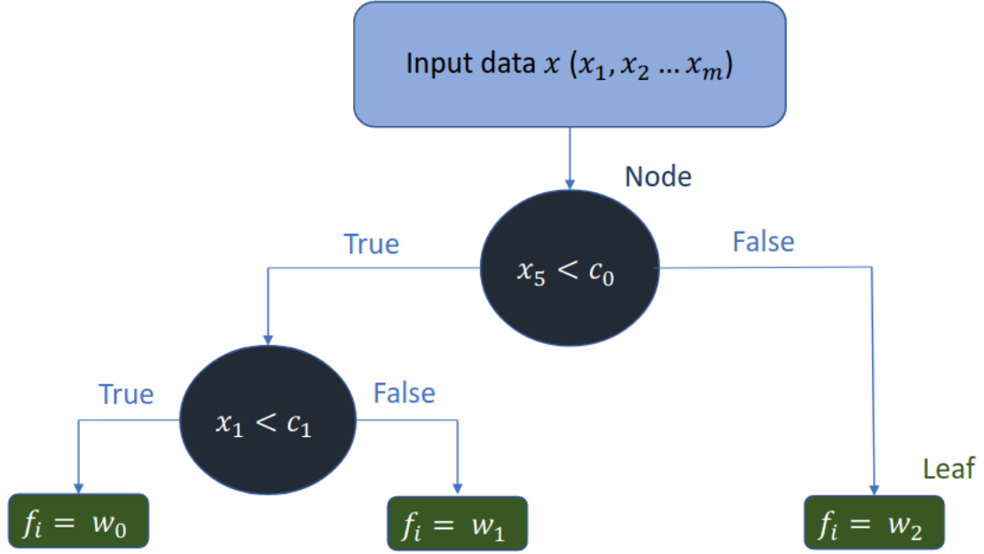
Figure A.1: Sketch of a decision tree. The tree have a depth of 2.
