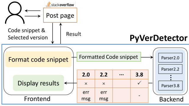
Fig. 1: Overview of PyVerDetector.
