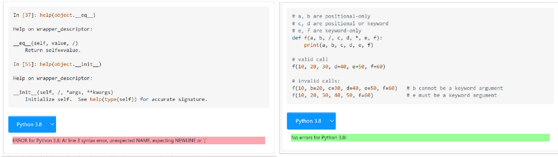
Fig. 2: Example of how the extension works in the default version. (Left): Parse error, (Right): Pass.
