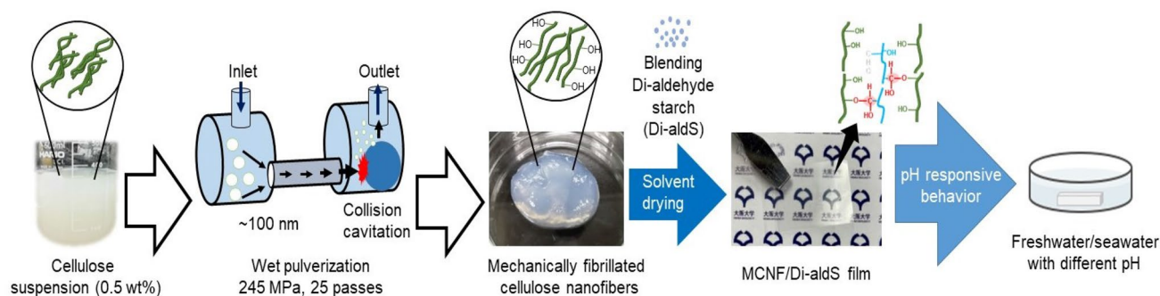
Fig. 1 Illustrative representation of film preparation and experimental scheme
