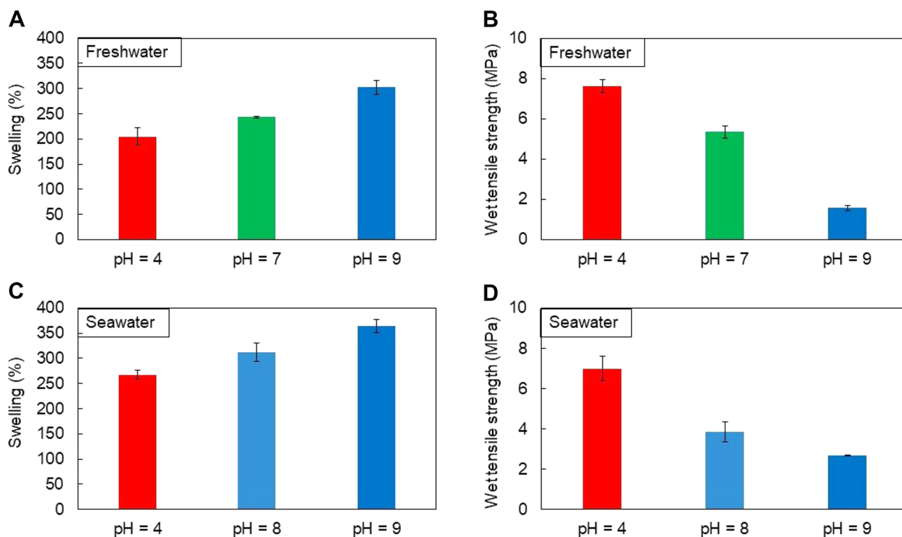
Fig. 2 MCNF/Di-aldS films a, c swelling behaviour and b, d wet tensile strength in freshwater and seawater, respectively, under different pH conditions
