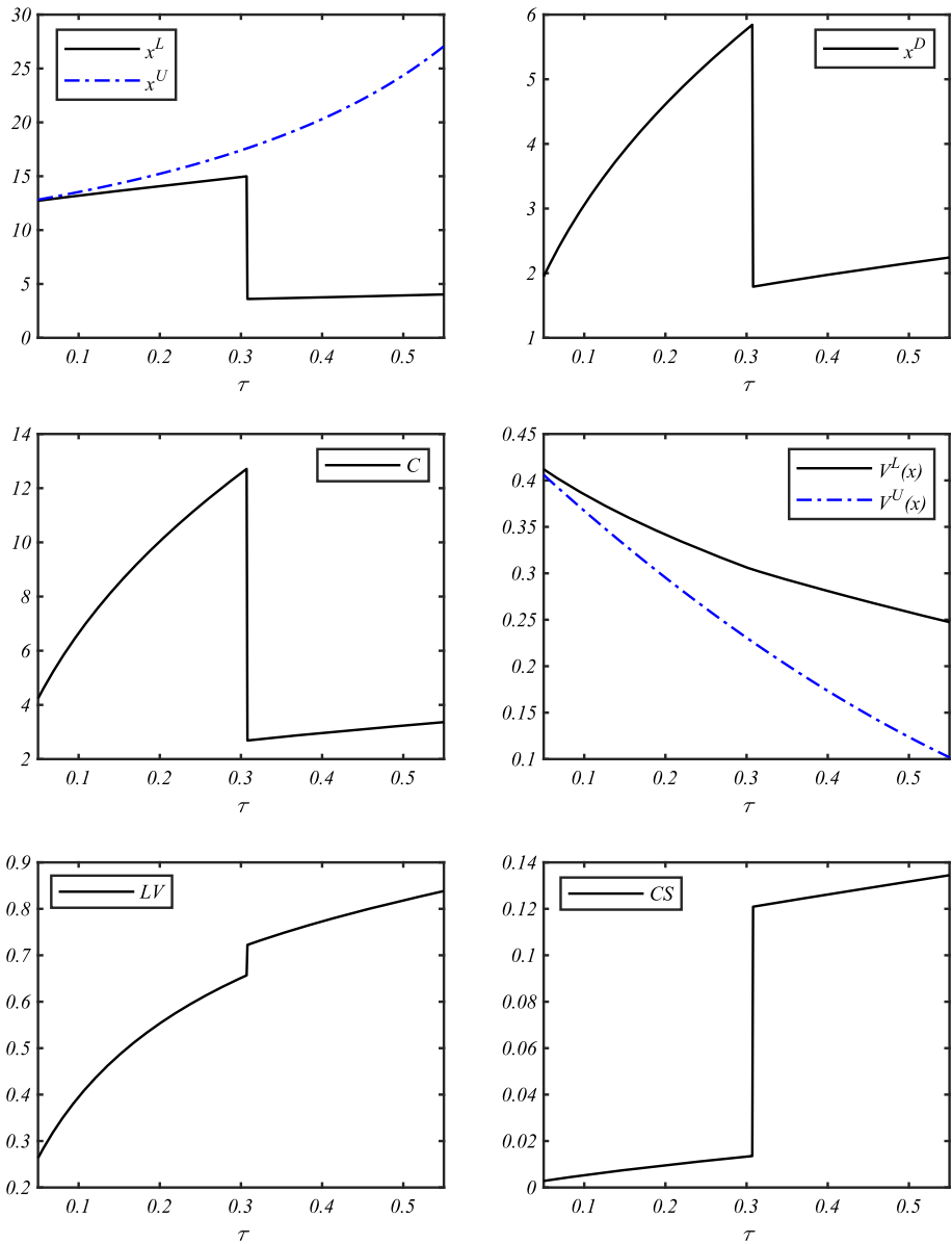
Fig. 5 Comparative statics with respect to corporate tax rate \tau . I_2 = 140
