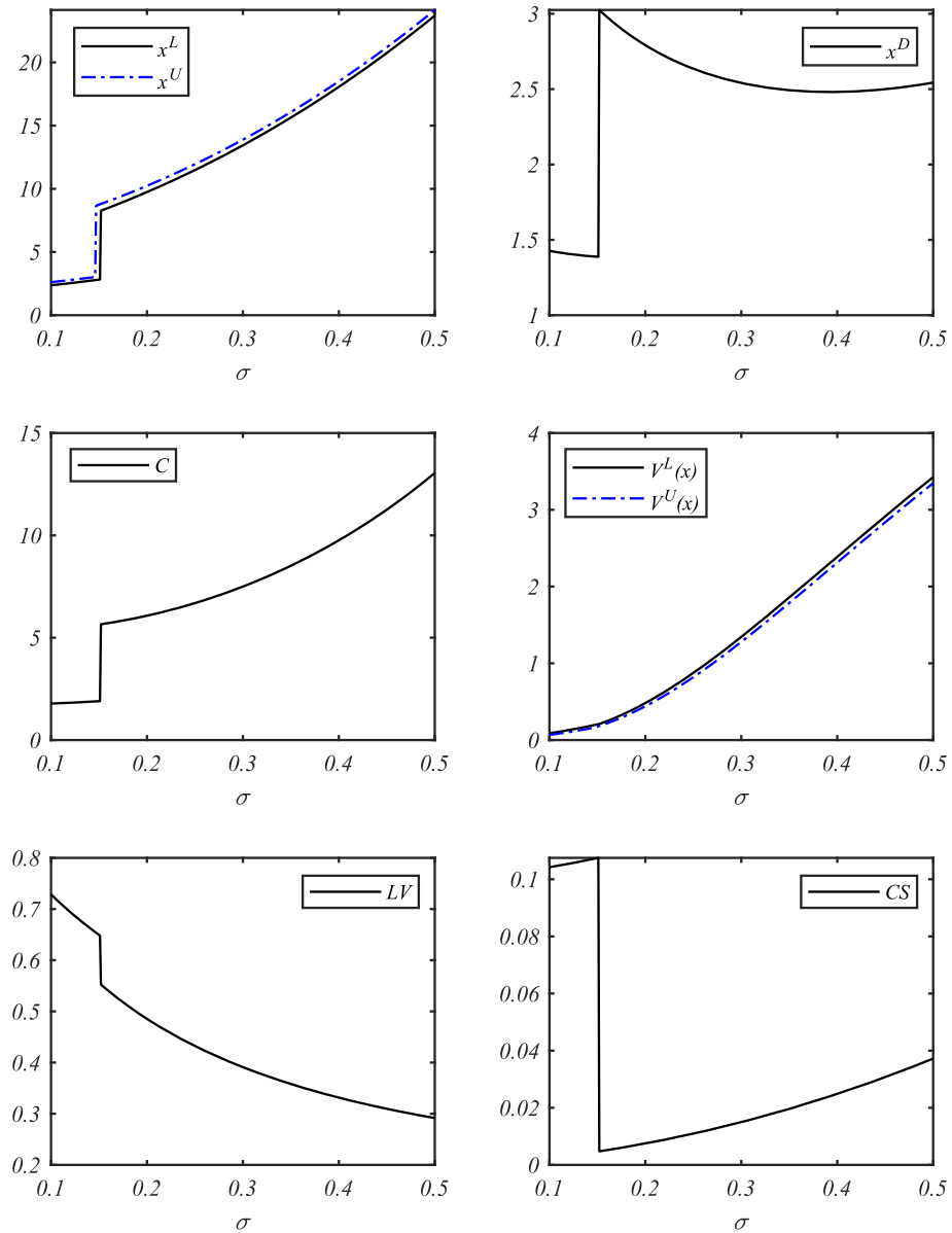
Fig. 4 Comparative statics with respect to volatility \sigma
