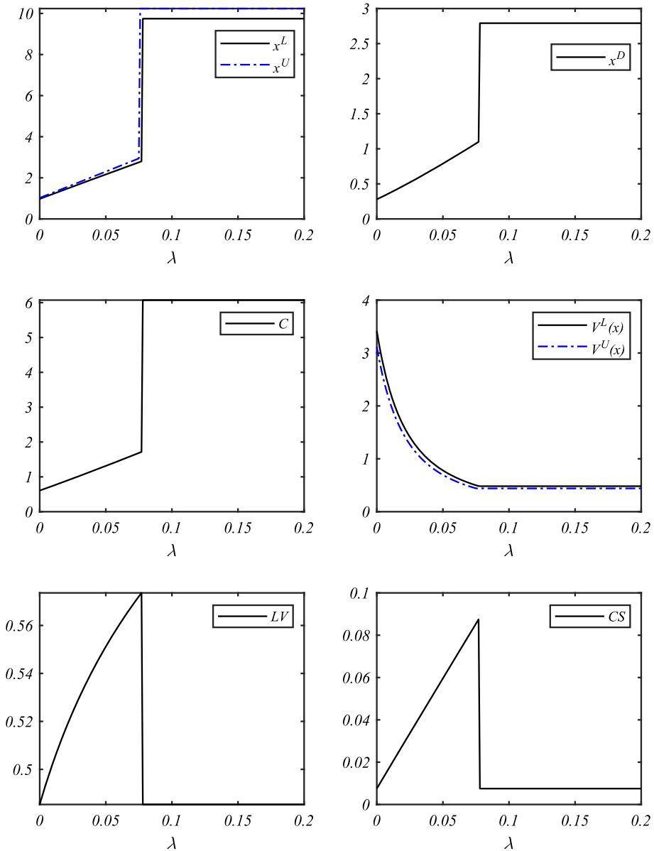
Fig. 1 Comparative statics with respect to sustainability parameter \lambda
