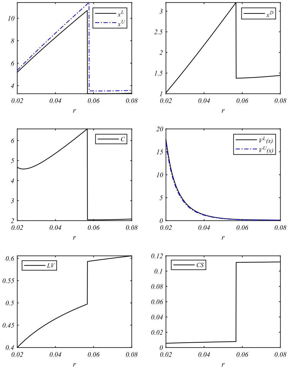
Fig. 2 Comparative statics with respect to discount rate r
