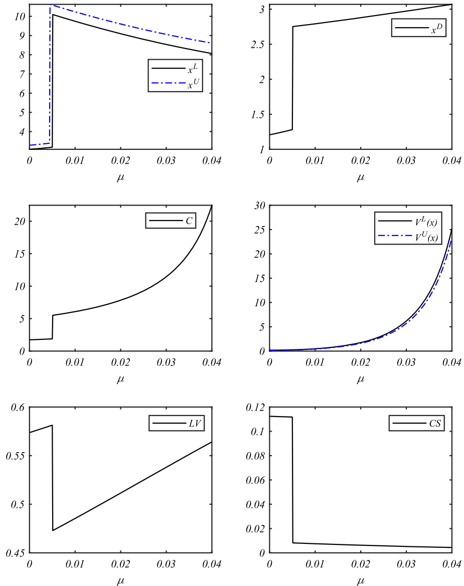
Fig. 3 Comparative statics with respect to growth rate \mu
