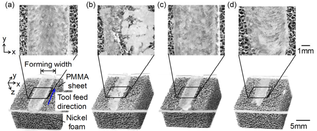
Fig. 4 Appearances of nickel foam and PMMA sheet after FSIF process: (a) \omega = 6000 rpm, f = 10 mm/min (joining), (b) \omega = 6000 rpm, f = 120 mm/min (no joining), (c) \omega = 1000 rpm, f = 10 mm/min (no joining), (d) \omega = 1000 rpm, f = 120 mm/min (no joining).
