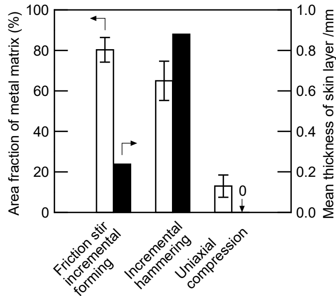
Fig. 11 Area fractions of metal matrix of fabricated surface and mean thicknesses of fabricated layers of formed aluminum foam in FSIF, IH, and uniaxial compression specimens ( np_z = 5 mm).
