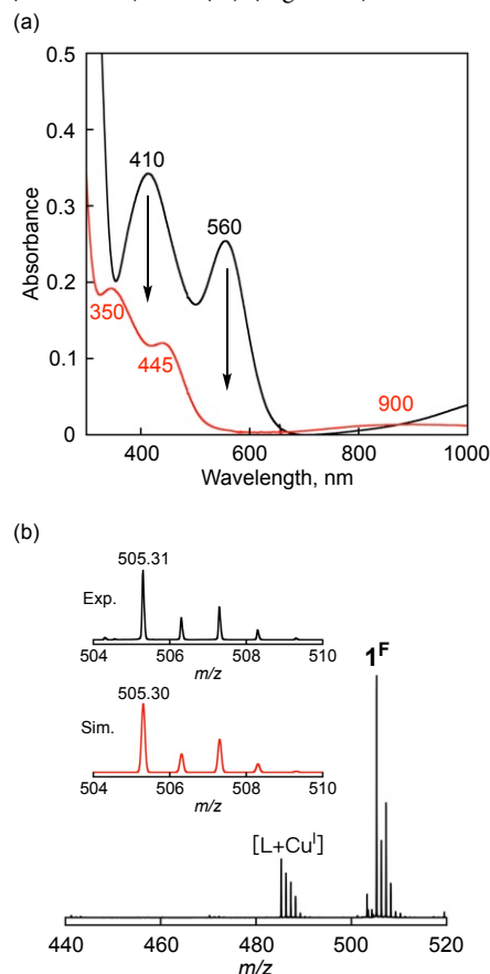
Figure 1. (a) UV-vis spectral change observed upon an addition of \text{Bu}_4\text{NF} (1 equiv) to a \text{CH}_3\text{CN} solution of 1 Br (0.25 mM, black) generating 1 F (red) at 25°C. (b) ESI-MS of 1 F in \text{CH}_3\text{CN} at 25°C. Inset: An expanded spectrum (black) and its simulation spectrum (red).
