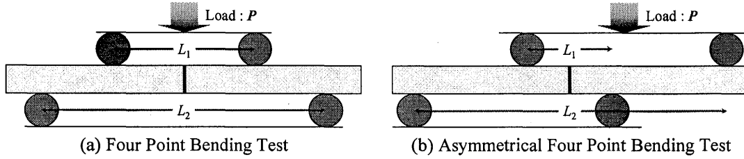
Fig.3 Schematic illustration of bending and asymmetrical bending tests.
