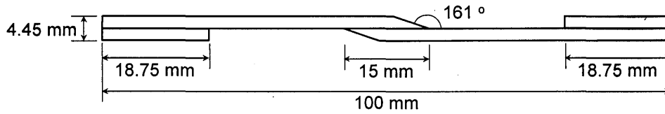
Fig.8 Schematic illustration of lap joint of SiC/SiC composites.
