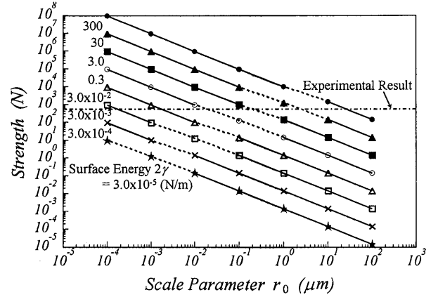
Fig.5 Effect of scale parameter and surface energy on shear strength of SiC/SiC composite joint
