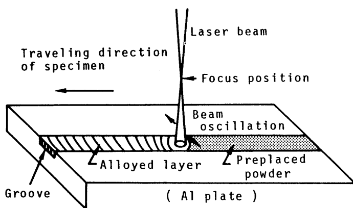
Fig. 1 Schematic illustration of laser alloying process
