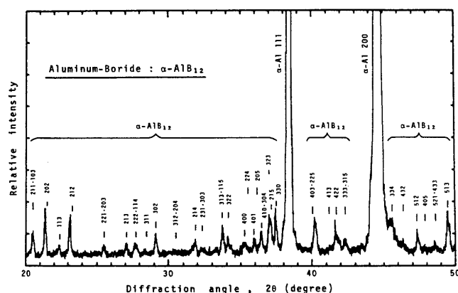
Fig. 4 X-ray diffraction pattern from the boron-alloyed layer surface
