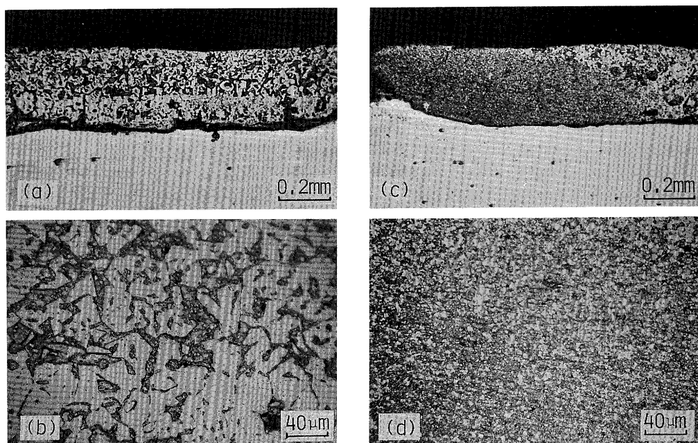
Fig. 3 Microstructures of the crosssection of the boron-alloyed layer: (a) and (b), center of the groove; (c) and (d), near the edge of the groove
