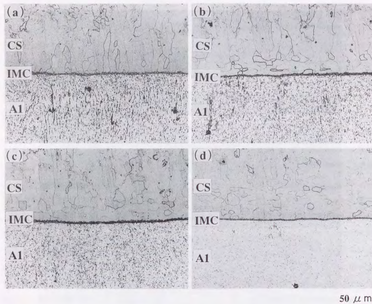
Fig. 6.20 Microstructures at steel/aluminum interfaces of aluminum clad steel sheets after spot welding (10.0kA-0.2s): (a) F-FA1-A5, (b) F-FA2-A5, (c) F-FA3-A5, (d) F-FA4-A5.
