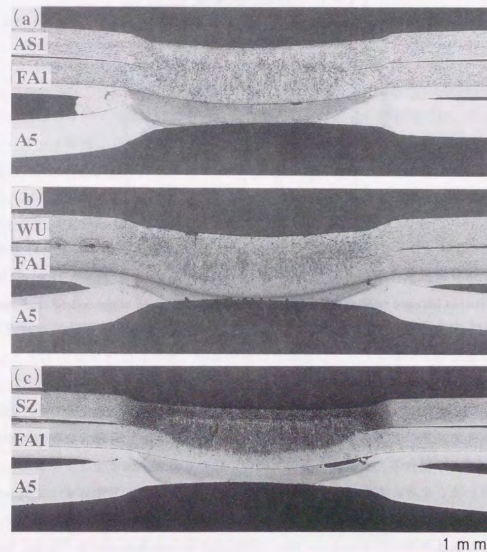
Fig. 6.55 Macrostructures of galvanized steel-aluminum clad steel-aluminum spot weld joints (12.0kA-0.2s): (a) AS1-FA1-A5, (b) WU-FA1-A5, (c) SZ-FA1-A5.
