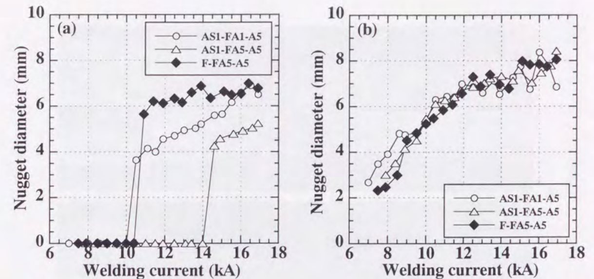
Fig. 6.46 Relation between welding current and nugget diameter of galvanized steel-aluminum clad steel-aluminum (AS1-FA1-A5, AS1-FA5-A5) and steel-aluminum clad steel-aluminum (F-FA5-A5) joints: (a) Steel sheet side, (b) Aluminum sheet side.
