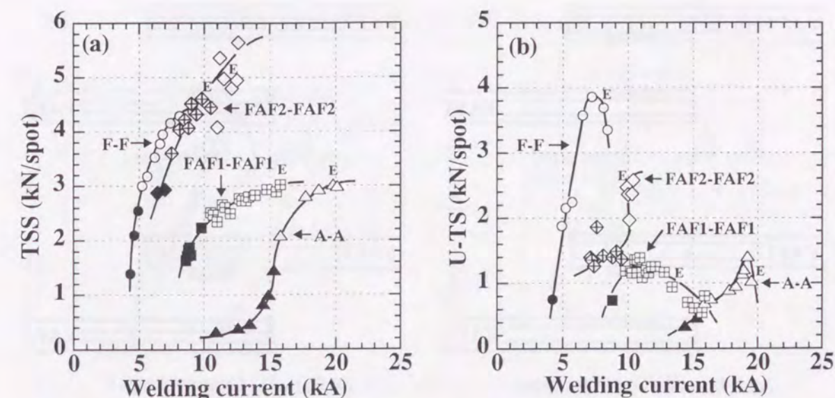
Fig. 5.25 Relation between welding current and tensile strength of steel/aluminum laminate-steel/aluminum laminate (FAF1-FAF1, FAF2-FAF2) joints: (a) Tensile shear strength (TSS), (b) U-tension strength (U-TS).
