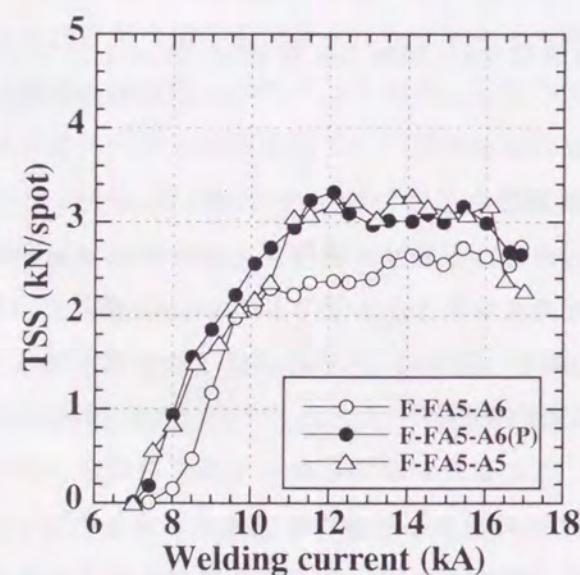
Fig. 6.31 Effects of ageing treatment on tensile shear strength of steel-aluminum clad steel-aluminum joints (F-FA5-A6).
