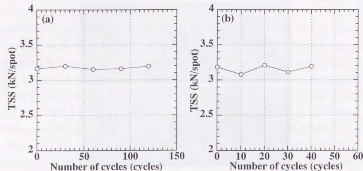
Fig. 6.67 Relation between corrosion cycles and tensile shear strength of galvanized steel-aluminum clad steel-aluminum (AS1-FA1-A5) joints: (a) SST, (b) CCT.
