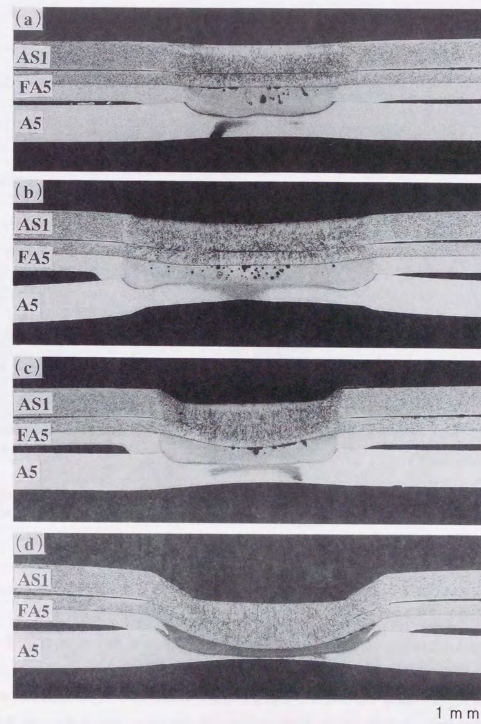
Fig. 6.40 Nugget formation process of galvanized steel-aluminum clad steel-aluminum (AS1-FA5-A5) spot weld joints: (a) DR-DR 14.0kA-0.04s, (b) DR-DR 14.0kA-0.12s, (c) CF-R 14.0kA-0.04s, (d) CF-R 14.0kA-0.12s.
