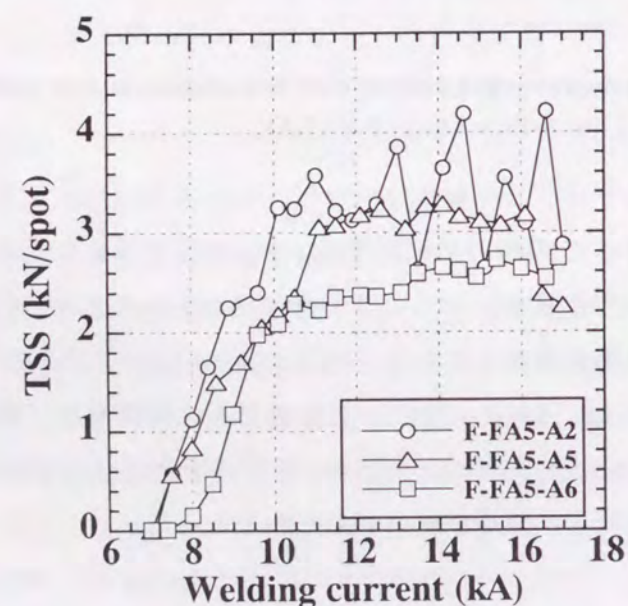
Fig. 6.27 Effects of types of aluminum alloy sheets on tensile shear strength of joints.
