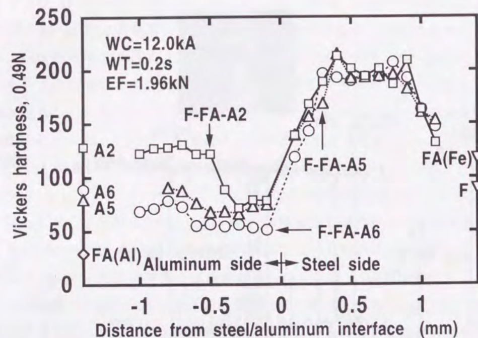
Fig. 6.30 Distributions of Vickers hardness in spot weld zones of steel-aluminum clad steel-aluminum joints (12.0kA-0.2s).
