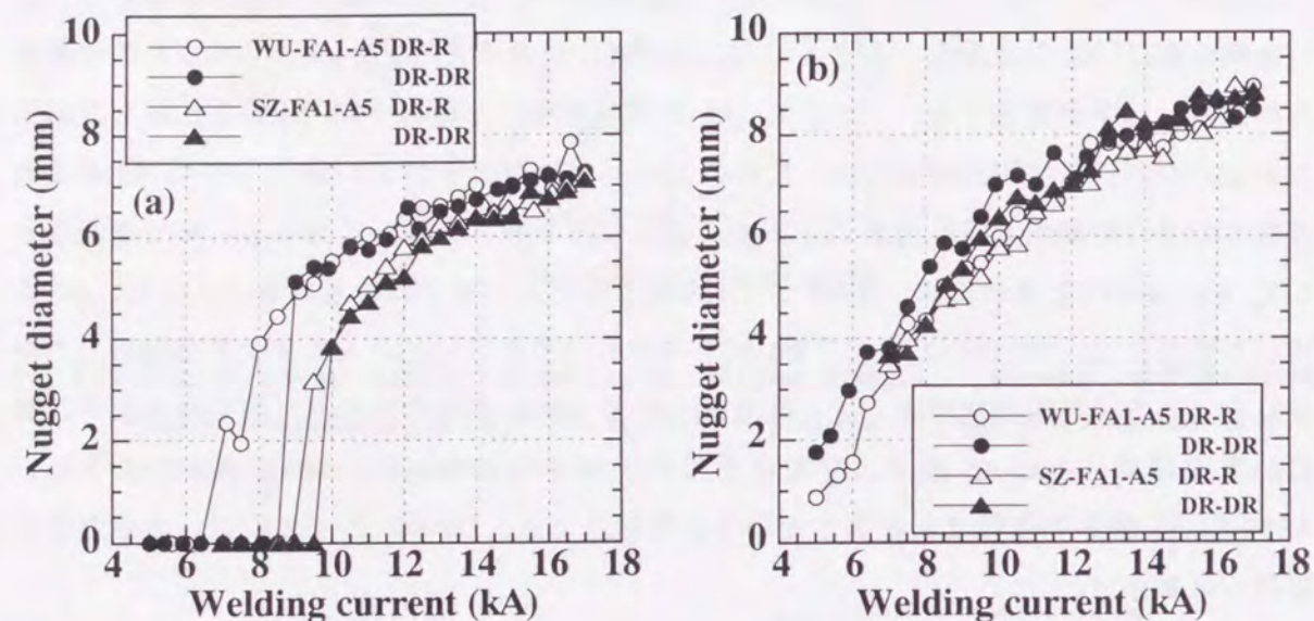
Fig. 6.61 Relation between welding current and nugget diameter of galvanized steel-aluminum clad steel-aluminum (WU-FA1-A5, SZ-FA1-A5) and steel-aluminum clad steel-aluminum (F-FA5-A5) joints: (a) Steel sheet side, (b) Aluminum sheet side.
