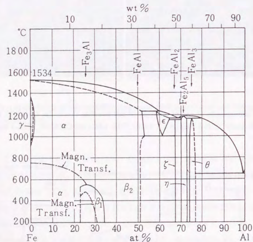
Fig. 3.9 Iron-aluminum binary phase diagram.
