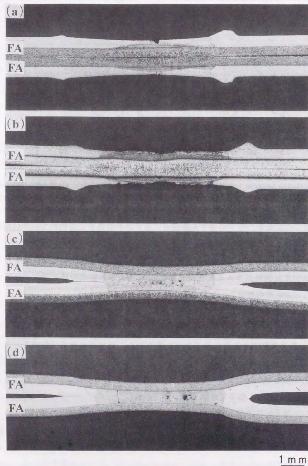
Fig. 5.10 Macrostructures of aluminum clad steel-aluminum clad steel (FA-FA(F), FA-FA(A)) spot weld joints: (a) FA-FA(F) 14.3kA-0.2s, (b) FA-FA(F) 17.4kA-0.2s, (c) FA-FA(A) 10.8kA-0.2s, (d) FA-FA(A) 13.1kA-0.2s.
