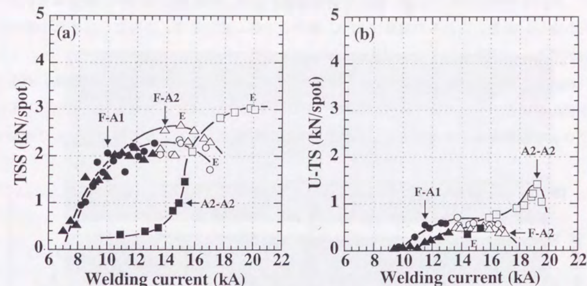
Fig. 4.5 Relation between welding current and tensile strength of steel-aluminum (F-A1, F-A2) and aluminum-aluminum (A2-A2) joints: (a) Tensile shear strength, (b) U-tension strength.
