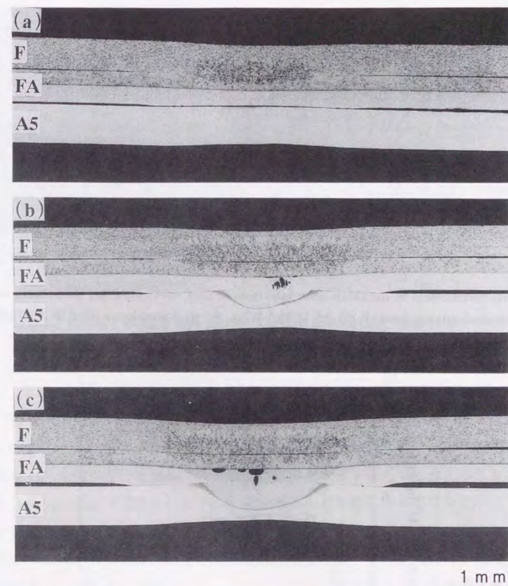
Fig. 6.5 Macrostructures of steel-aluminum clad steel-aluminum (F-FA-A5) spot weld joints: (a) 8.7kA-0.04s, (b) 8.7kA-0.08s, (c) 8.7kA-0.12s.
