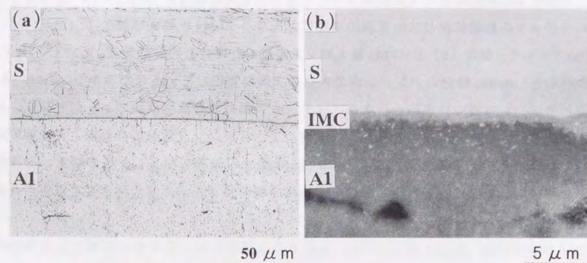
Fig. 4.10 Microstructures at stainless steel/aluminum interface of spot weld zone (S-A1 11.0kA-0.2s): (a) Optical microscope, (b) Scanning electron microscope.
