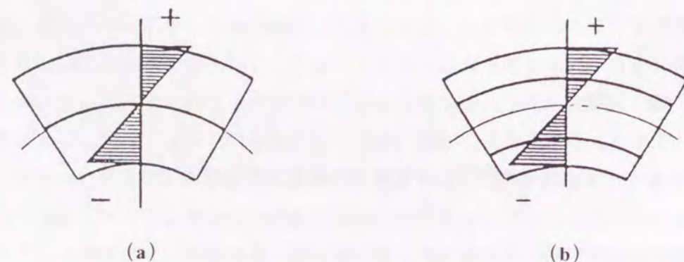
Fig. 2.19 Distribution of distortion in laminate: (a) Two layer laminate, (b) Three layer laminate.
