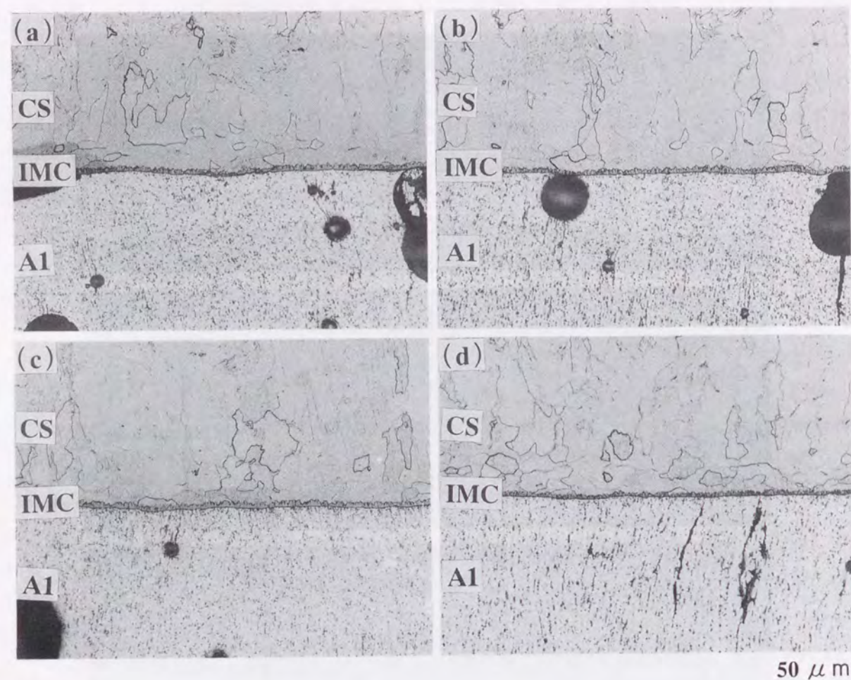
Fig. 6.51 Microstructures at steel/aluminum interfaces of spot weld zones of galvanized steel-aluminum clad steel-aluminum spot weld joints (11.0kA-0.2s): (a) AS1-FA1-A5, (b) AS2-FA1-A5, (c) AS3-FA1-A5, (d) AS4-FA1-A5.
