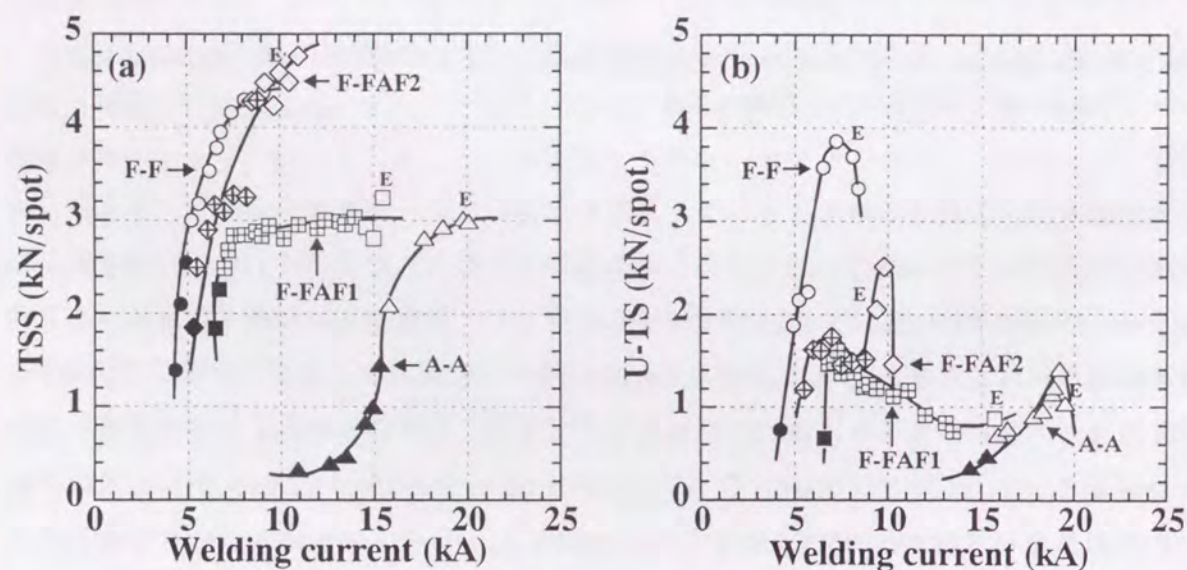
Fig. 5.18 Relation between welding current and tensile strength of steel-steel/aluminum laminate (F-FAF1, F-FAF2) joints: (a) Tensile shear strength (TSS), (b) U-tension strength (U-TS).
