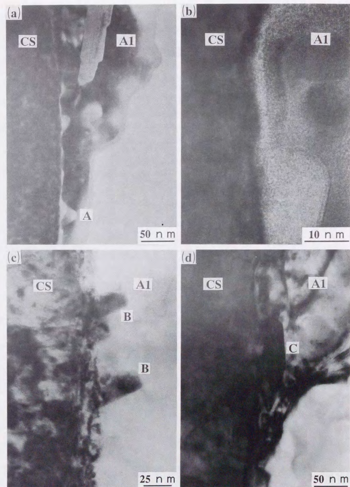
Fig. 2.10 TEM micrographs of typical microstructures at interface of aluminum clad steel sheet (FA1): (a) Indirect bonding section, (b) Amorphous layer at interface, (c) Direct bonding section, (d) Precipitate in aluminum sheet side.
