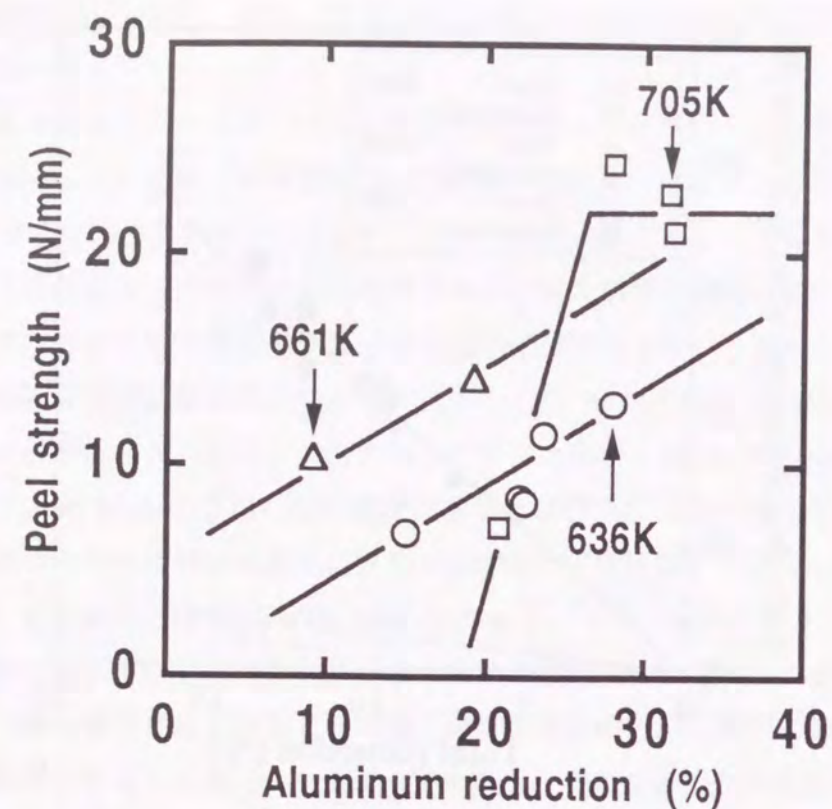
Fig. 2.6 Effects of aluminum sheet reduction and rolling temperature on peel strength of steel/aluminum laminates.
