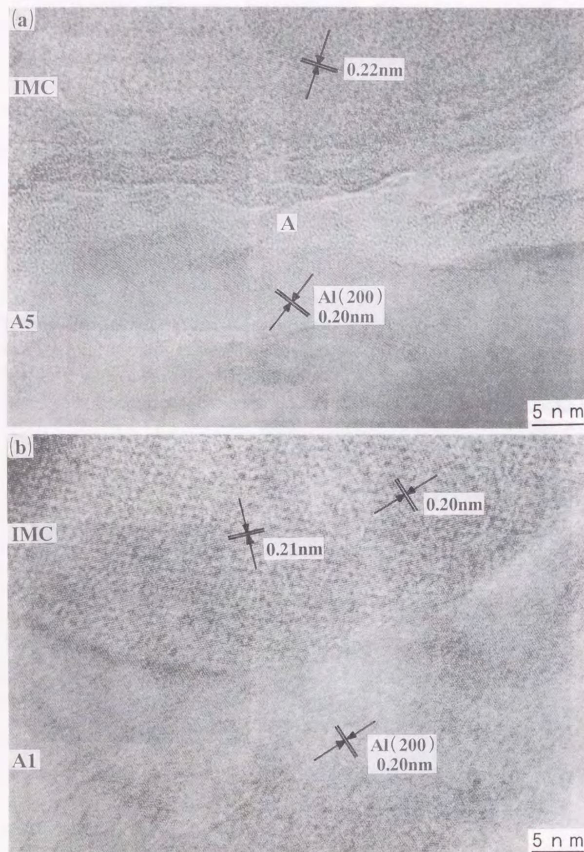
Fig. 3.11 TEM micrographs at IMC/aluminum interfaces of roll bonding sheets: (a) CS/A5, (b) SS/A1.
