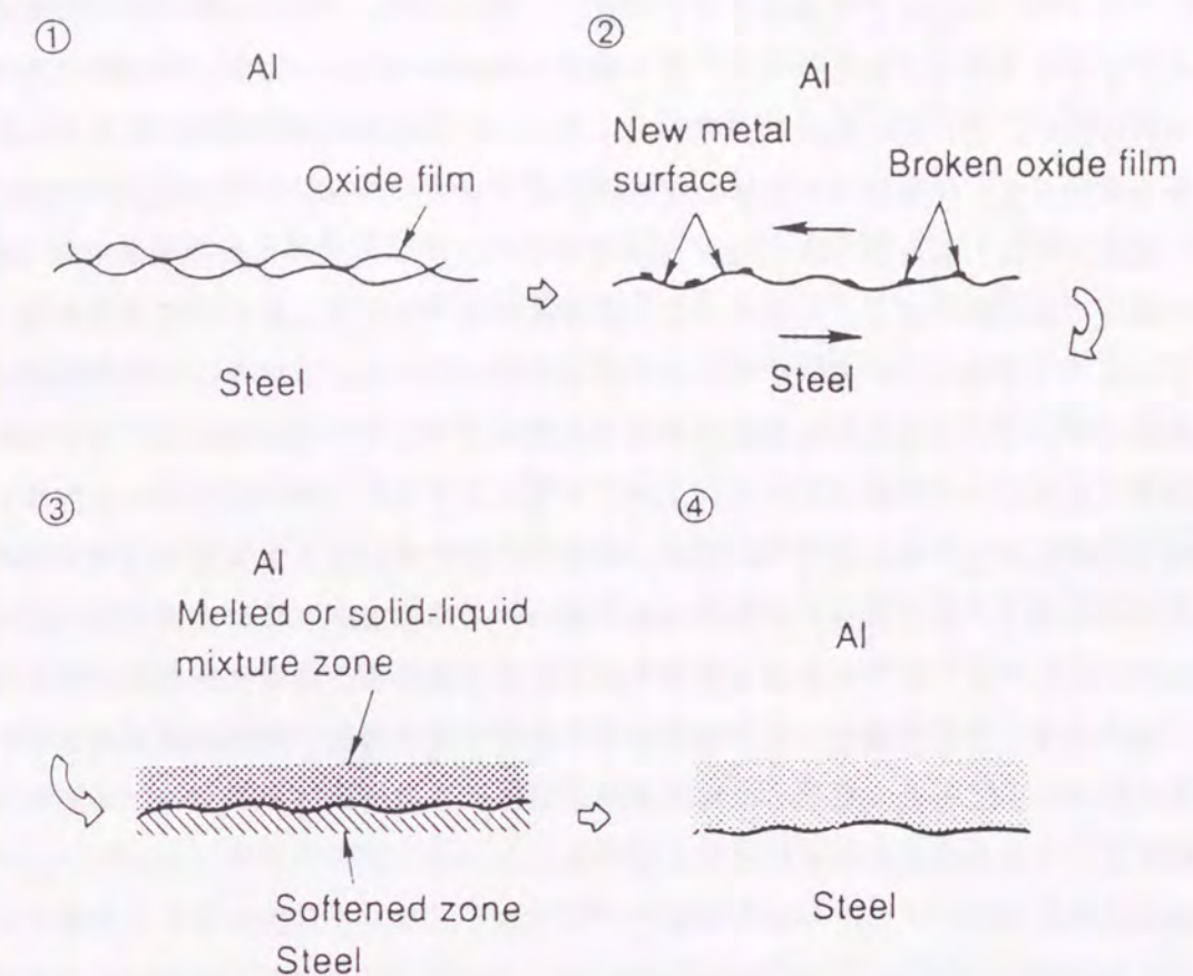
Fig. 2.16 Roll bonding model at interface of steel and aluminum sheet.
