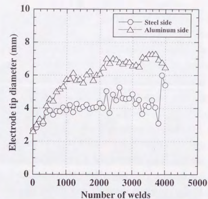
Fig. 6.64 Relation between number of welds and diameter of electrode tip.
