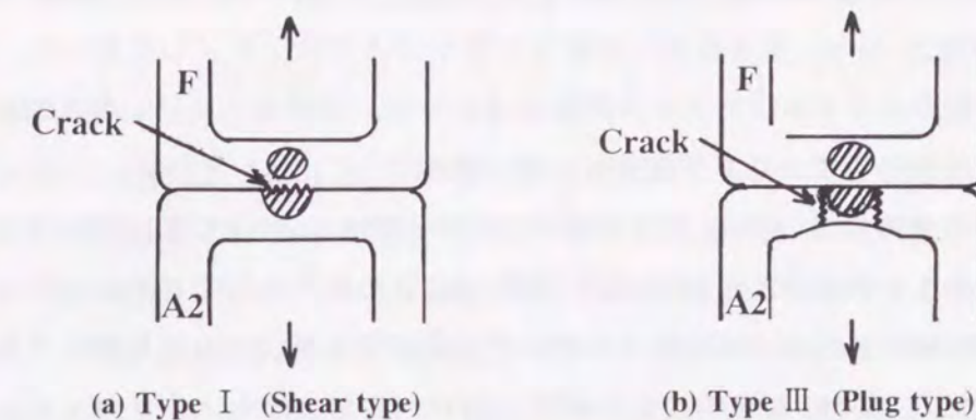
Fig. 4.19 Fracture modes in U-tension testing of steel-aluminum joint: (a) Type I (Shear type), (b) Type III (Plug type).
