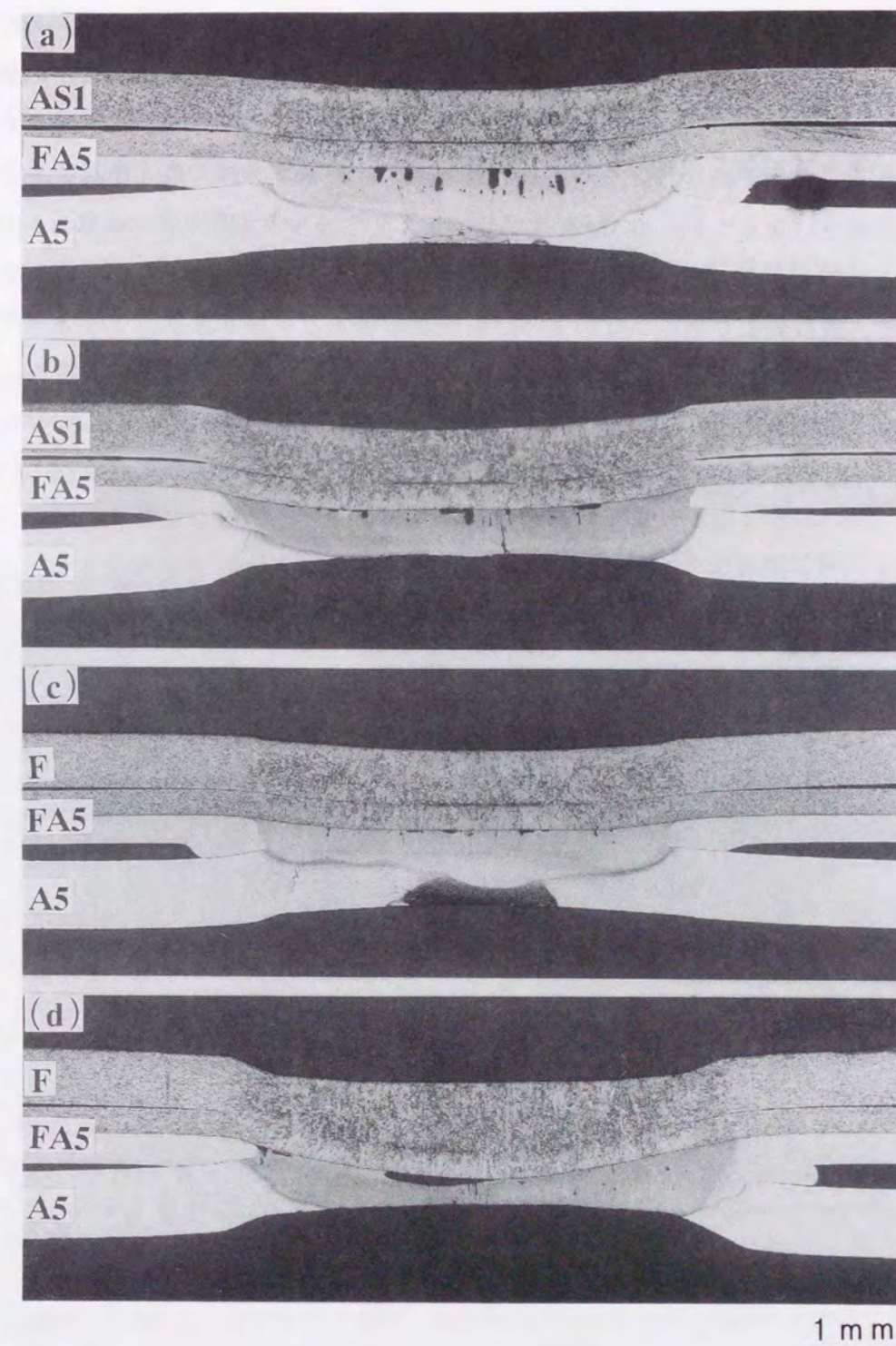
Fig. 6.32 Macrostructures of galvanized steel-aluminum clad steel-aluminum (AS1-FA5-A5) and steel-aluminum clad steel-aluminum (F-FA5-A5) spot weld joints: (a) AS1-FA5-A5 11.0kA-0.2s, (b) AS1-FA5-A5 14.1kA-0.2s, (c) F-FA5-A5 11.1kA-0.2s, (d) F-FA5-A5 14.1kA-0.2s.
