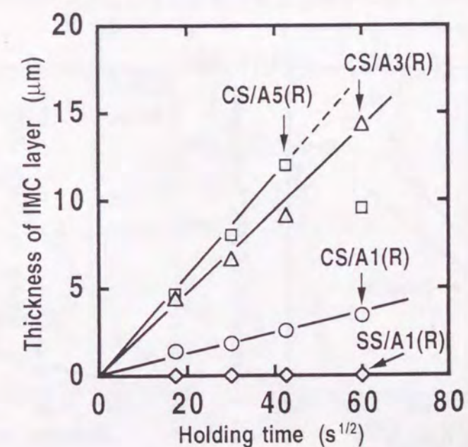
Fig. 3.3 Comparison of growth rate of intermetallic compound (IMC) layers at 773K.
