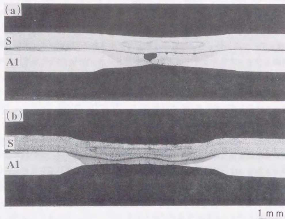
Fig. 4.9 Macrostructures of stainless steel-aluminum (S-A1) spot weld joints: (a) 11.0kA-0.2s, (b) 14.3kA-0.2s.
