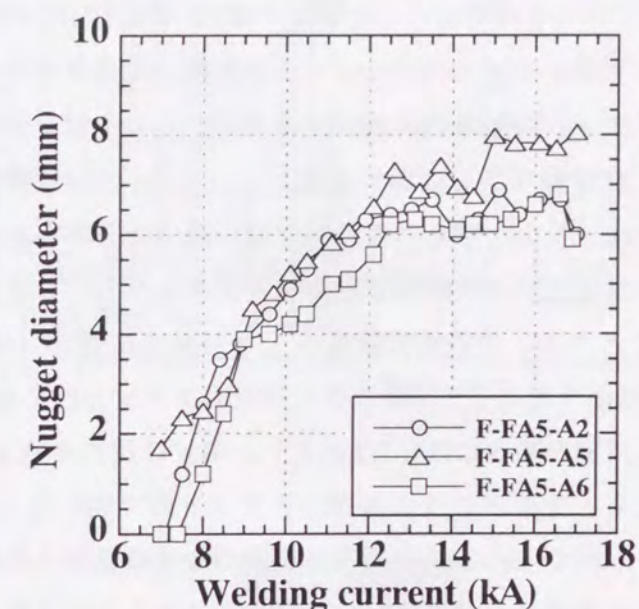
Fig. 6.28 Effects of types of aluminum alloy sheets on nugget diameter on aluminum sheet sides of joints.
