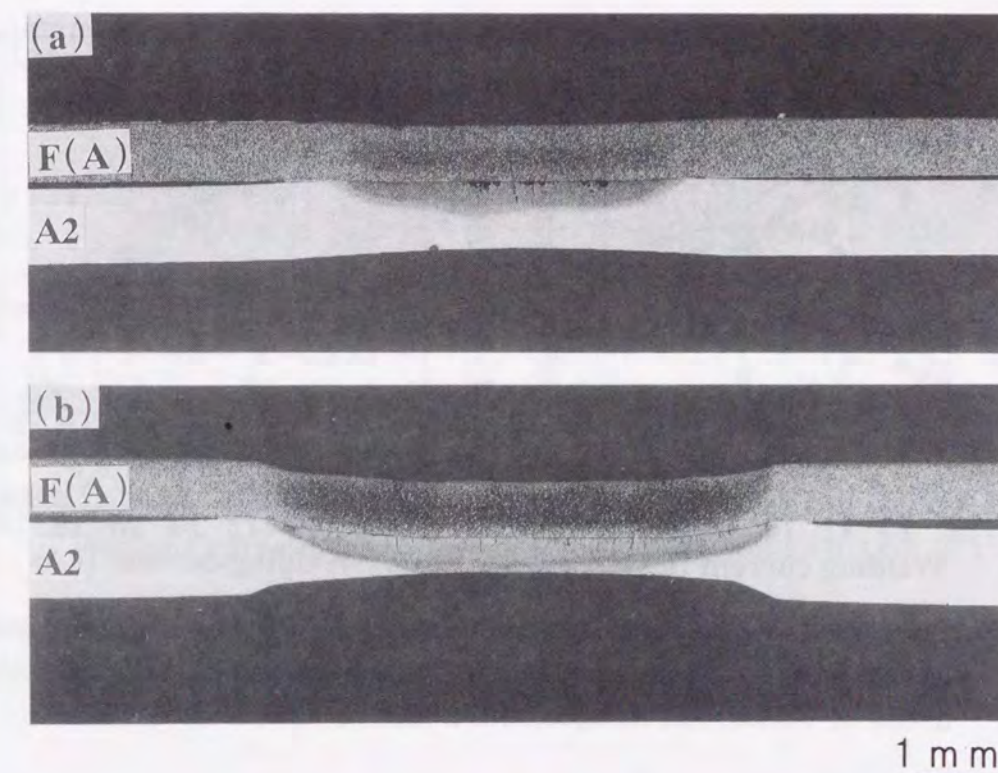
Fig. 4.13 Macrostructures of aluminum coated steel-aluminum spot weld joints: (a) F(A)-A2 10.1kA-0.2s, (b) F(A)-A2 14.0kA-0.2s.
