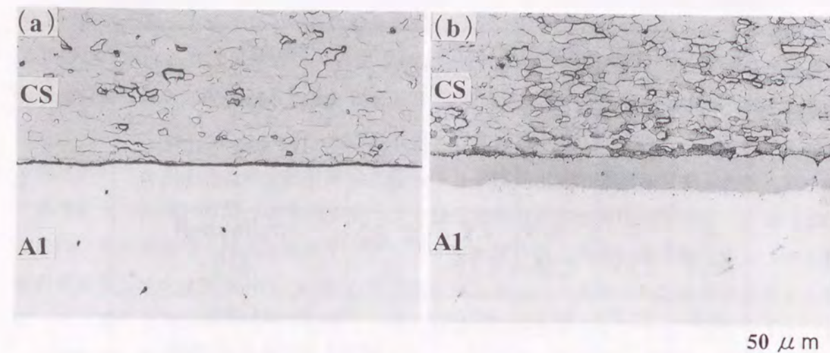
Fig. 2.3 Effect of oxide film on diffusion reaction at interfaces in diffusion bonding of steel and aluminum sheets (FAD2): (a) Oxidation in steel sheet side, (b) Oxidation in aluminum sheet side.
