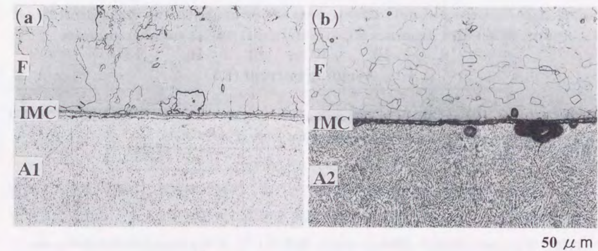
Fig. 4.3 Microstructures at steel/aluminum interfaces of spot weld zones: (a) F-A1 10.0kA-0.2s, (b) F-A2 10.0kA-0.2s.
