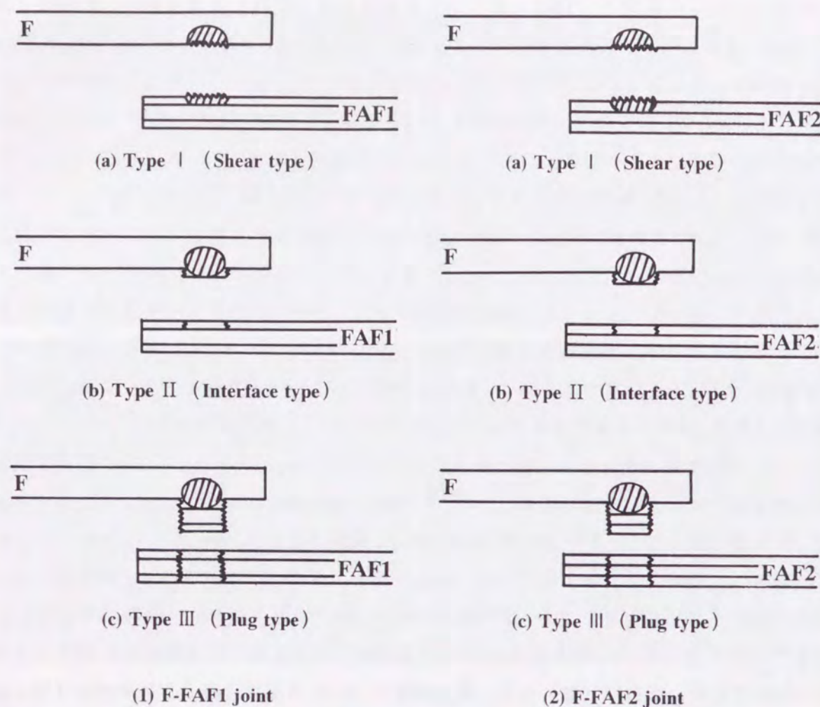
Fig. 5.19 Fracture modes observed in tensile shear testing and U-tension testing of steel-steel/aluminum laminate (F-FAF1, F-FAF2) joints.
