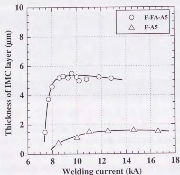
Fig. 6.7 Effect of welding current on thickness of intermetallic compound (IMC) layers formed at steel/aluminum interfaces of steel-aluminum clad steel-aluminum joints (F-FA-A5) and steel-aluminum joints (F-A5).
