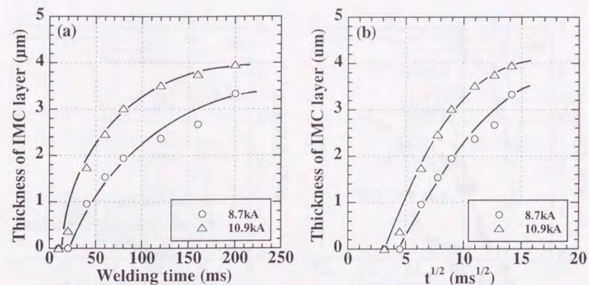
Fig. 6.8 Relation between welding time and thickness of intermetallic compound (IMC) layers formed at steel/aluminum interfaces of steel-aluminum clad steel-aluminum joints (F-FA-A5).
