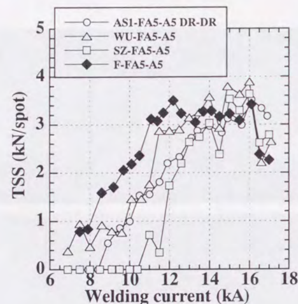
Fig. 6.56 Relation between welding current and tensile shear strength of galvanized steel-aluminum clad steel-aluminum (AS1-FA5-A5, WU-FA5-A5, SZ-FA5-A5) and steel-aluminum clad steel-aluminum (F-FA5-A5) joints.
