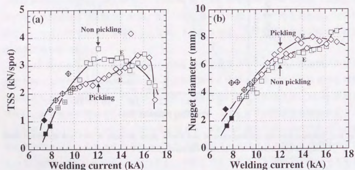
Fig. 6.15 Comparison of tensile shear strength and nugget diameter of F-FA5-A5 (Non pickling) and F-FA5-A5 (Pickling) joints: (a) Tensile shear strength, (b) Nugget diameter.
