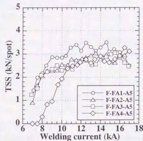
Fig. 6.23 Effects of thickness ratio of aluminum clad steel sheets on tensile shear strength of joints.
