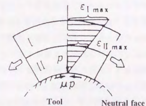
Fig. 2.21 Distribution of distortion in laminate in bending test.
