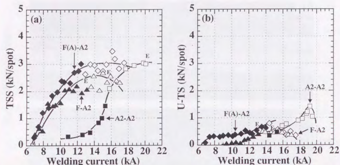
Fig. 4.15 Relation between welding current and tensile strength of aluminum coated steel-aluminum (F(A)-A2), steel-aluminum (F-A2) and aluminum-aluminum (A2-A2) joints: (a) Tensile shear strength, (b) U-tension strength.
