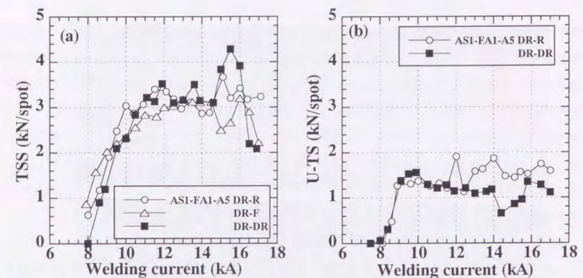
Fig. 6.48 Relation between welding current and tensile strength of galvanized steel-aluminum clad steel-aluminum (AS1-FA1-A5) joints: (a) Tensile shear strength, (b) U-tension strength.
