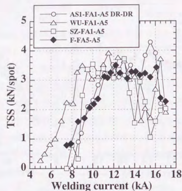
Fig. 6.58 Relation between welding current and tensile shear strength of galvanized steel-aluminum clad steel-aluminum (AS1-FA1-A5, WU-FA1-A5, SZ-FA1-A5) and steel-aluminum clad steel-aluminum (F-FA5-A5) joints.
