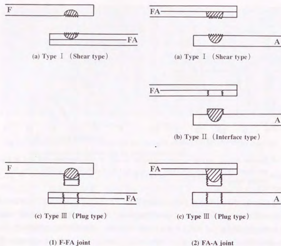
Fig. 5.8 Fracture modes observed in tensile shear testing and U-tension testing of steel-aluminum clad steel (F-FA) and aluminum clad steel-aluminum (FA-A) joints.
