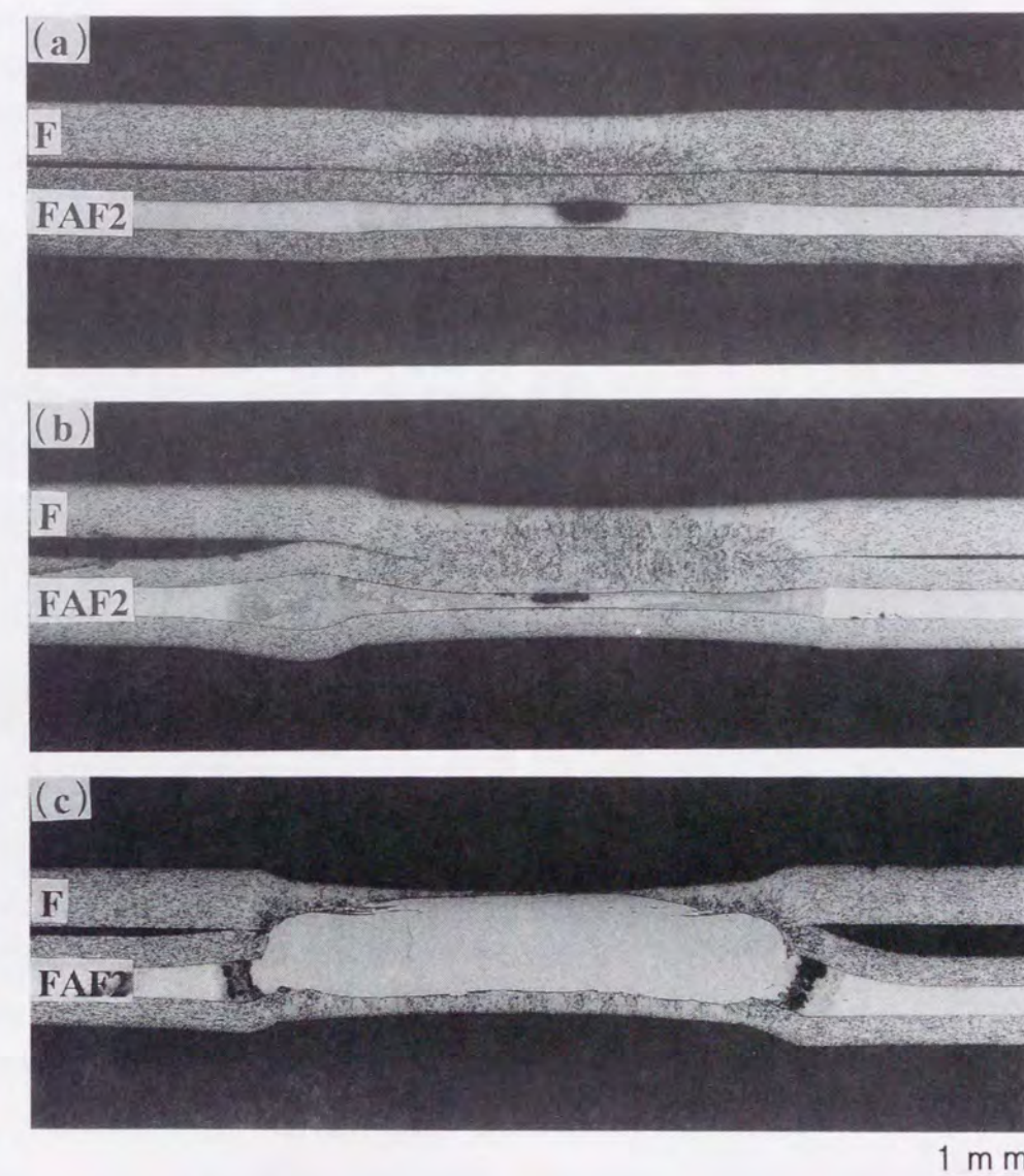
Fig. 5.16 Macrostructures of steel-steel/aluminum laminate (F-FAF2) spot weld joints: (a) 6.1kA-0.2s, (b) 8.2kA-0.2s, (c) 10.0kA-0.2s.
