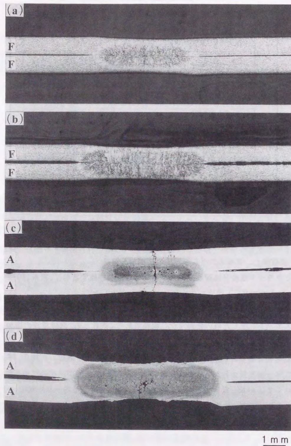
Fig. 5.1 Macrostructures of steel-steel (F-F) and aluminum-aluminum (A-A) spot weld joints: (a) F-F 5.6kA-0.2s, (b) F-F 7.4kA-0.2s, (c) A-A 14.9kA-0.2s, (d) A-A 19.8kA-0.2s.
