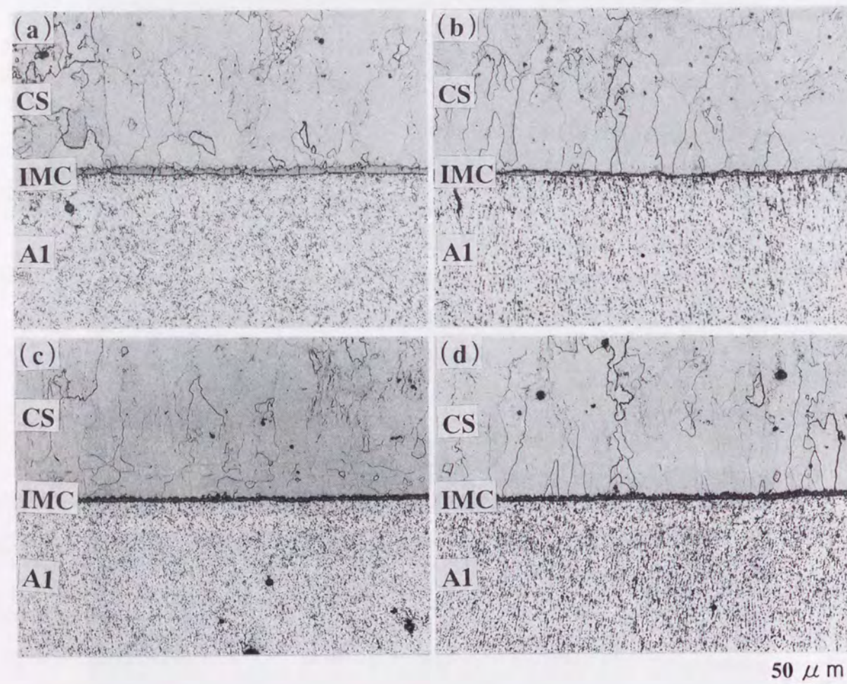
Fig. 6.43 Microstructures at steel/aluminum interfaces of spot weld zones of galvanized steel-aluminum clad steel-aluminum (AS1-FA1-A5, AS1-FA5-A5) spot weld joints: (a) AS1-FA1-A5 11.1kA-0.2s, (b) AS1-FA1-A5 13.9kA-0.2s, (c) AS1-FA5-A5 11.0kA-0.2s, (d) AS1-FA5-A5 14.1kA-0.2s.
