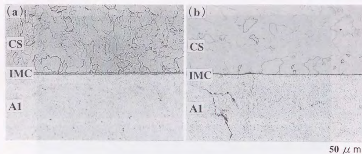
Fig. 5.6 Microstructures at steel/aluminum interfaces of aluminum clad steel sheets after spot welding: (a) F-FA 10.5kA-0.2s, (b) FA-A 14.6kA-0.2s.
