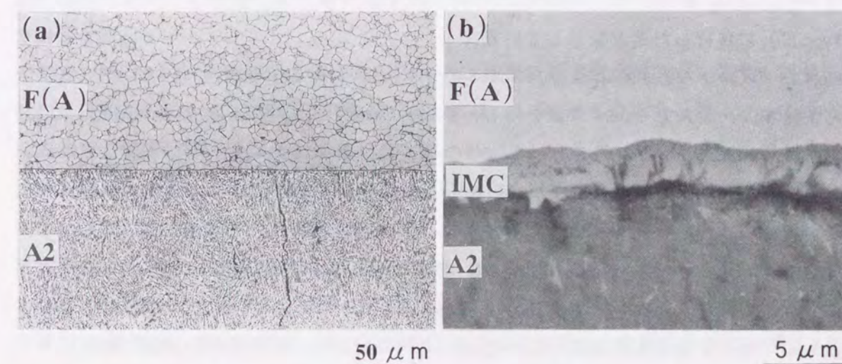
Fig. 4.14 Microstructures at aluminum coated steel/aluminum interface of spot weld zone (F(A)-A2 12.1kA-0.2s): (a) Optical microscope, (b) Scanning electron microscope.
