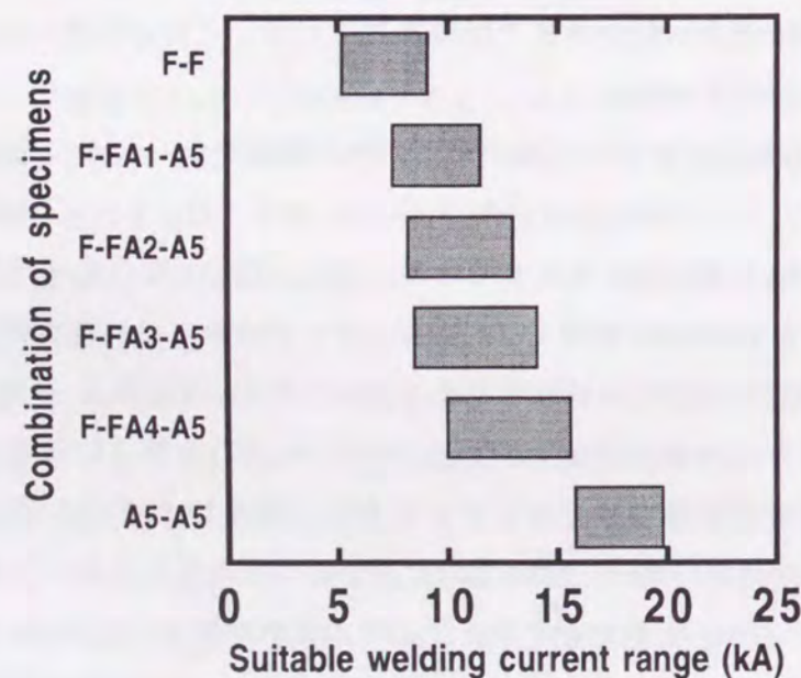
Fig. 6.24 Effects of thickness ratio of aluminum clad steel sheets on suitable welding current range of joints.
