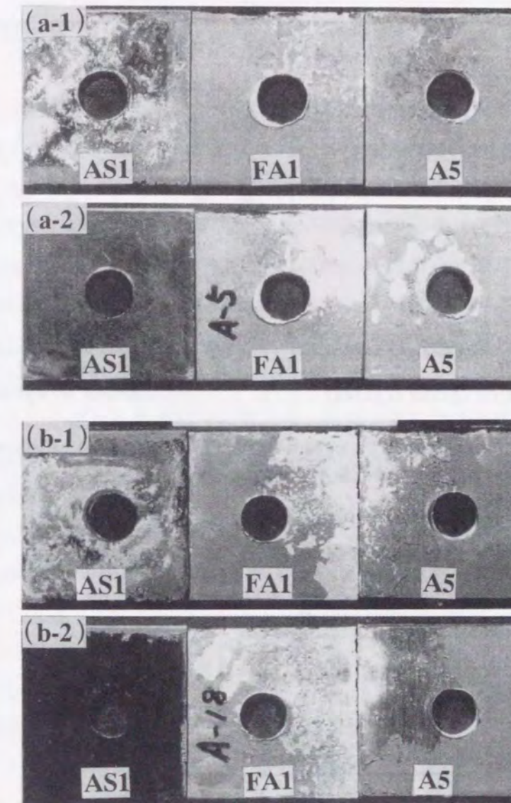
Fig. 6.66 Appearance of spot weld zones of galvanized steel-aluminum clad steel-aluminum (AS1-FA1-A5) joints after corrosion test: (a-1) SST-90cycles Before washing, (a-2) SST-90 cycles After washing, (b-1) CCT-90cycles Before washing, (b-2) CCT-90 cycles After washing.
