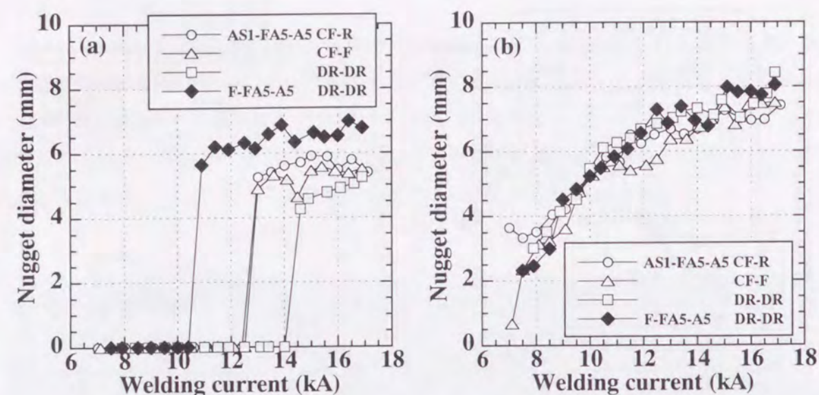
Fig. 6.39 Relation between welding current and nugget diameter of galvanized steel-aluminum clad steel-aluminum (AS1-FA5-A5) and steel-aluminum clad steel-aluminum (F-FA5-A5) joints: (a) Steel sheet side, (b) Aluminum sheet side.
