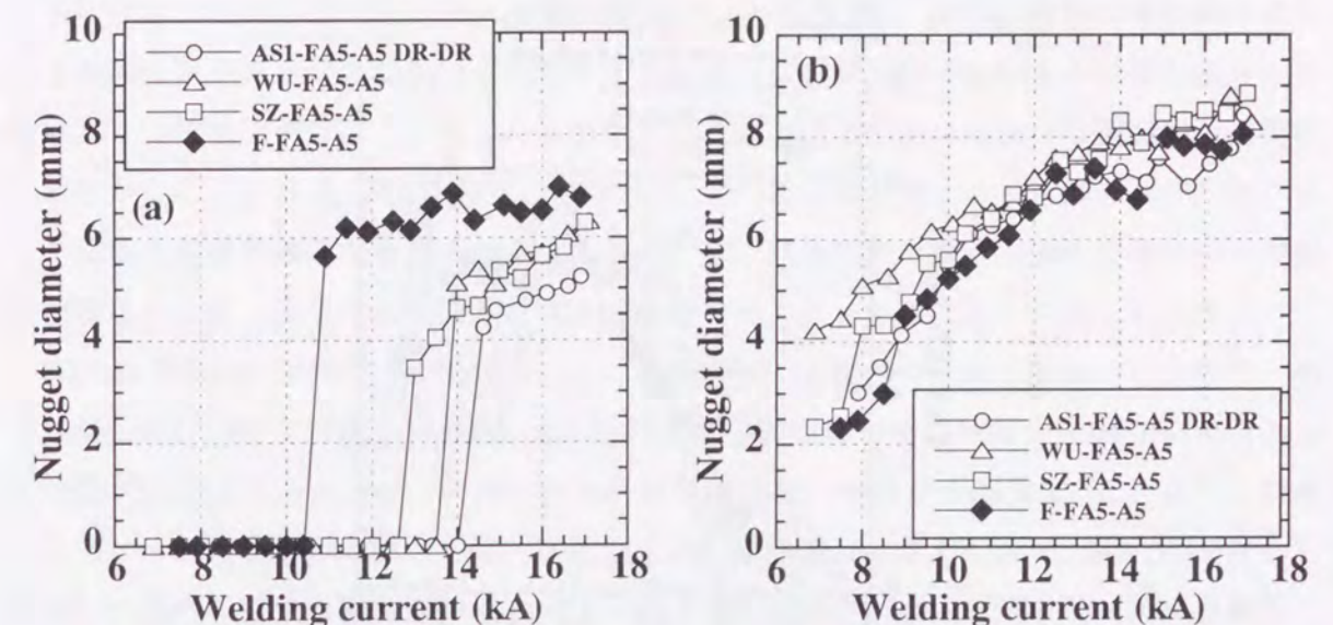
Fig. 6.57 Relation between welding current and nugget diameter of galvanized steel-aluminum clad steel-aluminum (AS1-FA5-A5, WU-FA5-A5, SZ-FA5-A5) and steel-aluminum clad steel-aluminum (F-FA5-A5) joints: (a) Steel sheet side, (b) Aluminum sheet side.
