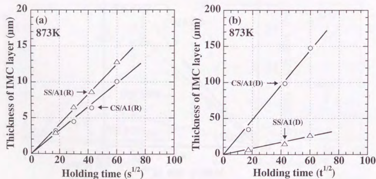
Fig. 3.4 Comparison of growth rate of intermetallic compound (IMC) layers: (a) CS/A1(R) and SS/A1(R), (b) CS/A1(D) and SS/A1(D).
