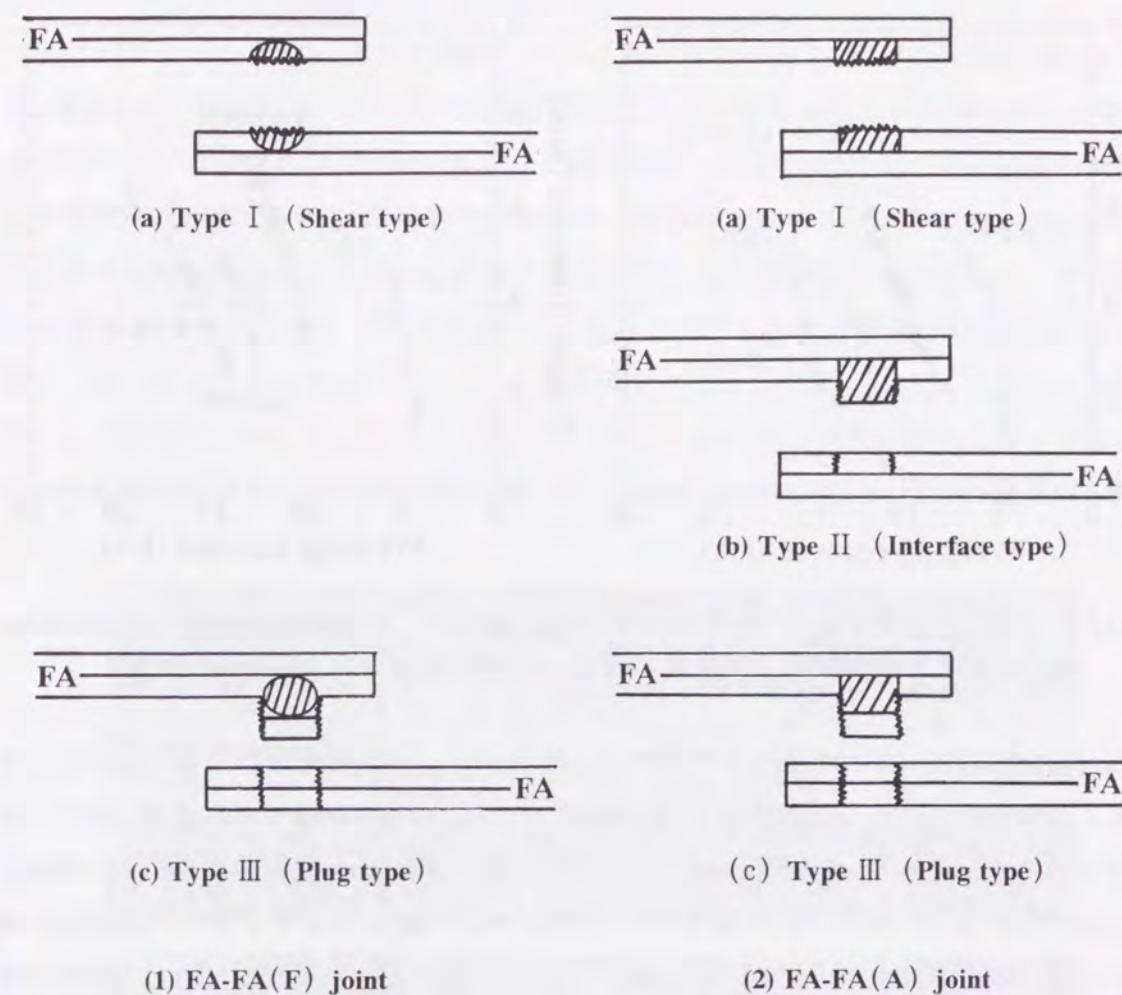
Fig. 5.13 Fracture modes observed in tensile shear testing and U-tension testing of aluminum clad steel-aluminum clad steel (FA-FA(F), FA-FA(A)) joints.
