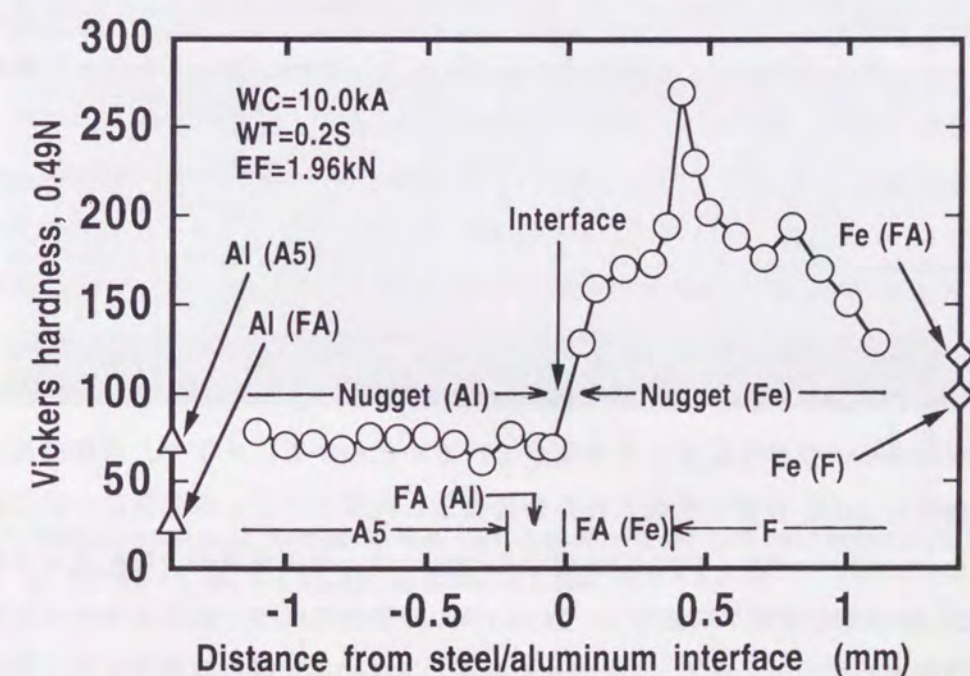
Fig. 6.18 Distribution of Vickers hardness in spot weld zone of steel-aluminum clad steel-aluminum (F-FA-A5) joint.
