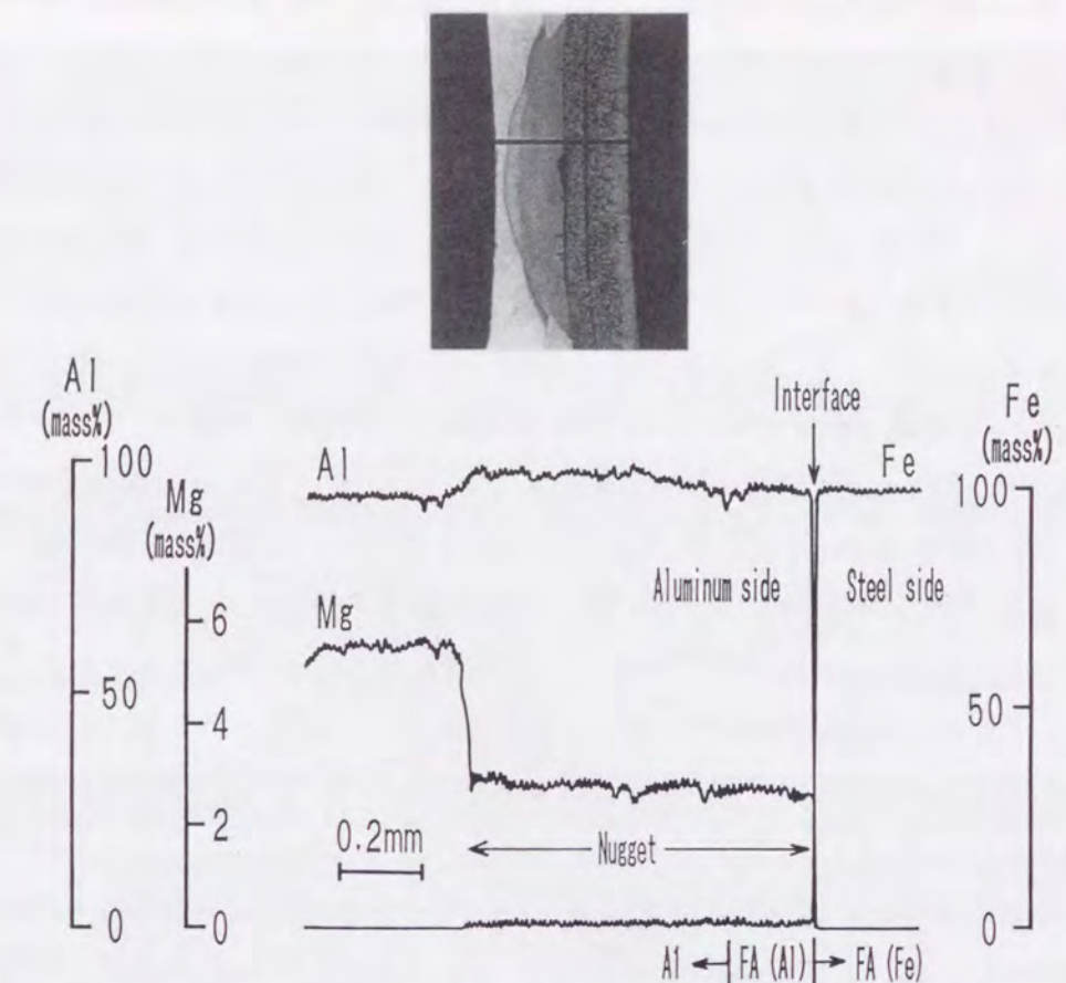
Fig. 6.17 EPMA line analysis in spot weld zone of steel-aluminum clad steel-aluminum (F-FA-A5) joint.
