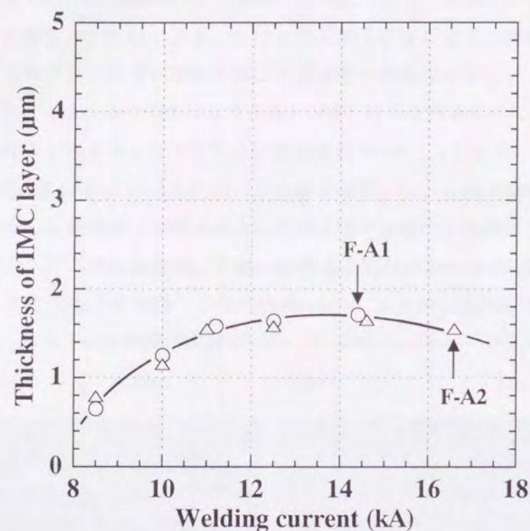
Fig. 4.4 Effect of welding current on thickness of intermetallic compound (IMC) layers formed at steel/aluminum interfaces of steel-aluminum joints (F-A1, F-A2).
