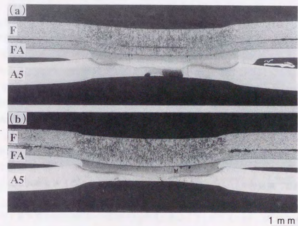
Fig. 6.4 Macrostructures of steel-aluminum clad steel-aluminum (F-FA5-A5) spot weld joints: (a) Non pickling 12.2kA-0.2s, (b) Pickling 11.9kA-0.2s.
