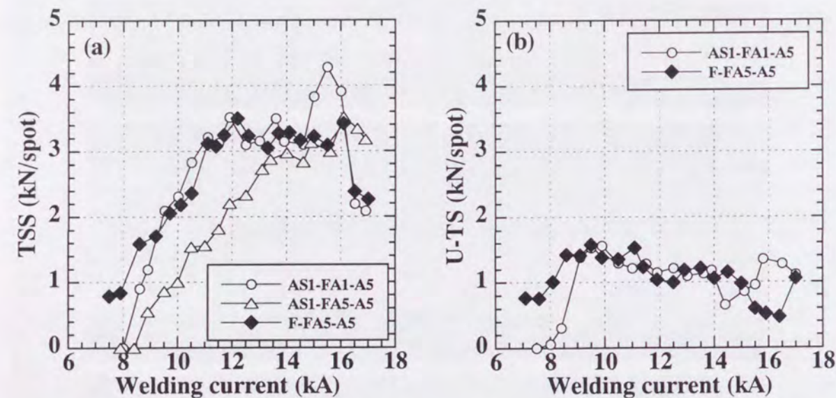
Fig. 6.45 Relation between welding current and tensile strength of galvanized steel-aluminum clad steel-aluminum (AS1-FA1-A5, AS1-FA5-A5) and steel-aluminum clad steel-aluminum (F-FA5-A5) joints: (a) Tensile shear strength, (b) U-tension strength.
