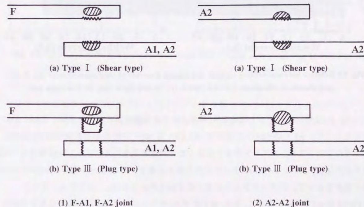
Fig. 4.6 Fracture modes observed in tensile shear testing and U-tension testing of steel-aluminum (F-A1, F-A2) and aluminum-aluminum (A2-A2) joints.
