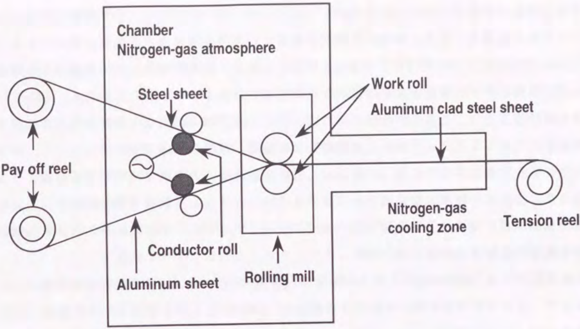
Fig. 2.1 Schematic diagram of direct resistance heating and rolling apparatus.
