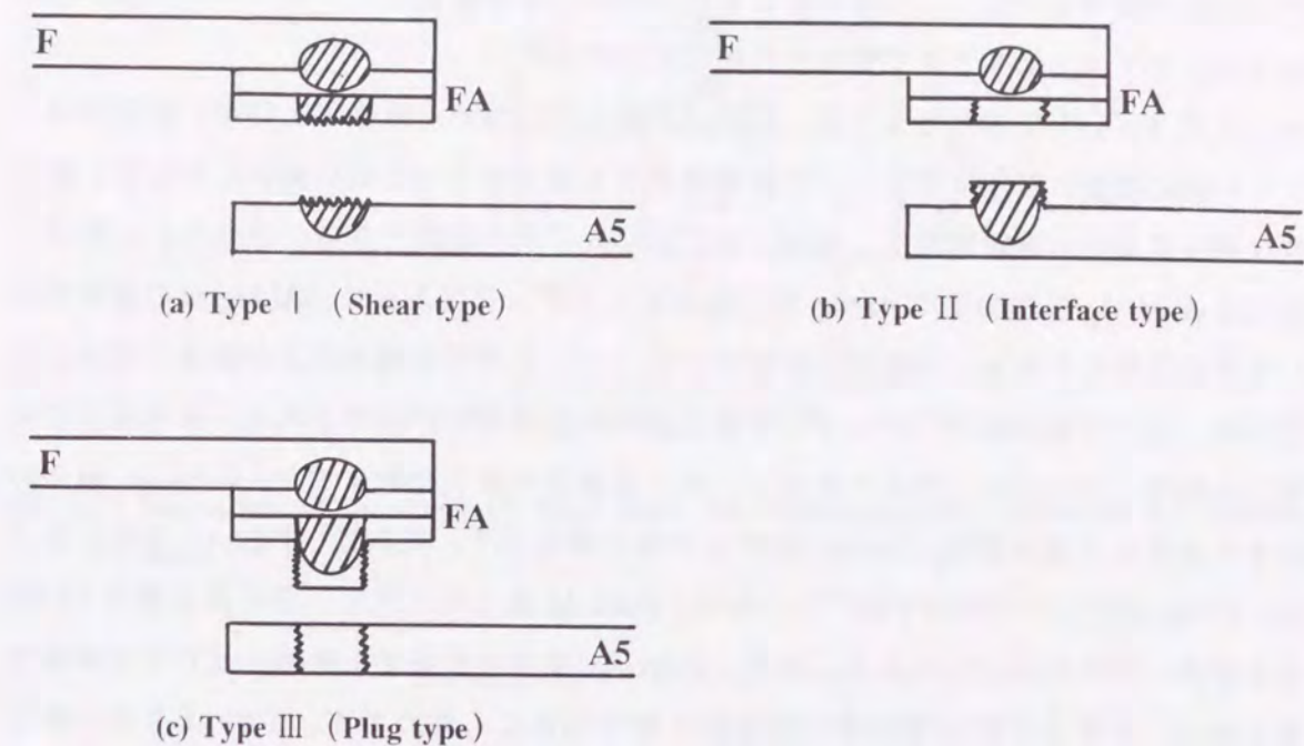
Fig. 6.10 Fracture modes observed in tensile shear testing of steel-aluminum clad steel-aluminum joints (F-FA-A5).
