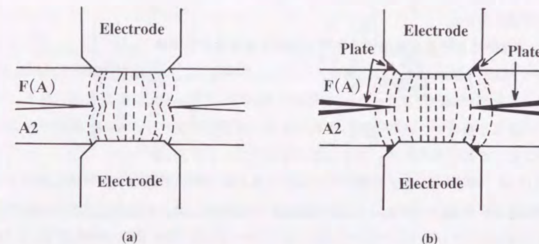
Fig. 4.17 Spot welding process of aluminum coated steel sheet to aluminum sheet: (a) First stage, (b) Second stage.
