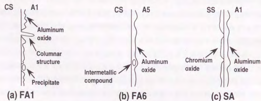
Fig. 2.17 Schematic illustration of microstructures at interfaces of roll bonding sheets: (a) FA1, (b) FA6, (c) SA.
