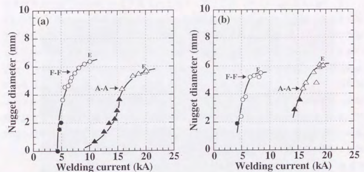
Fig. 5.4 Relation between welding current and nugget diameter of steel-steel (F-F) and aluminum-aluminum (A-A) joints: (a) Tensile shear test, (b) U-tension test.
