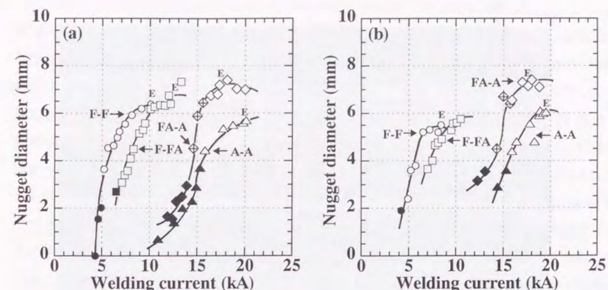
Fig. 5.9 Relation between welding current and nugget diameter of steel-aluminum clad steel (F-FA) and aluminum clad steel-aluminum (FA-A) joints: (a) Tensile shear test, (b) U-tension test.
