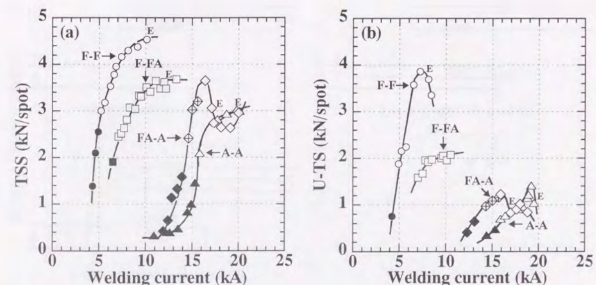
Fig. 5.7 Relation between welding current and tensile strength of steel-aluminum clad steel (F-FA) and aluminum clad steel-aluminum (FA-A) joints: (a) Tensile shear strength (TSS), (b) U-tension strength (U-TS).
