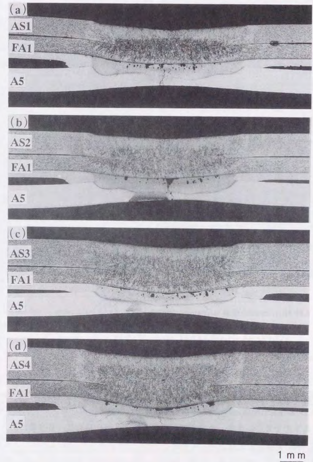
Fig. 6.50 Macrostructures of galvanized steel-aluminum clad steel-aluminum spot weld joints (11.0kA-0.2s): (a) AS1-FA1-A5, (b) AS2-FA1-A5, (c) AS3-FA1-A5, (d) AS4-FA1-A5.
