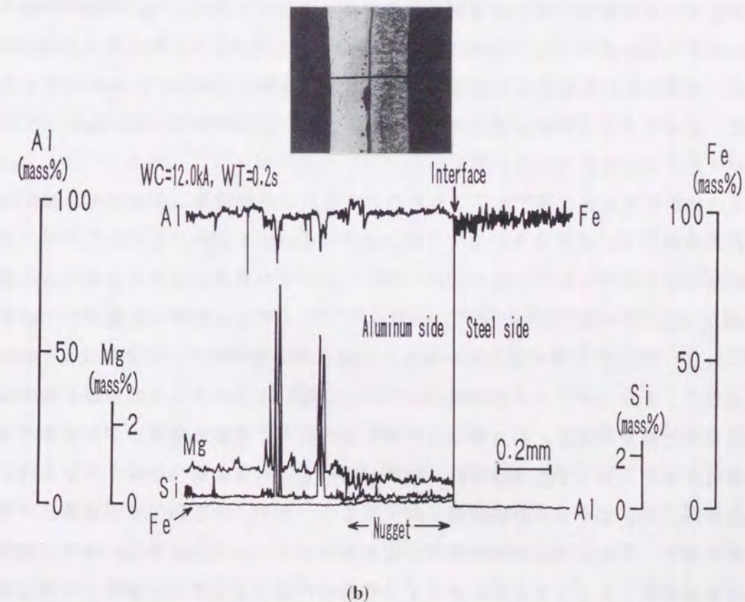
Fig. 6.29 EPMA line analyses in spot weld zones of steel-aluminum clad steel-aluminum joints (12.0kA-0.2s): (a) F-FA5-A2, (b) F-FA5-A6.
