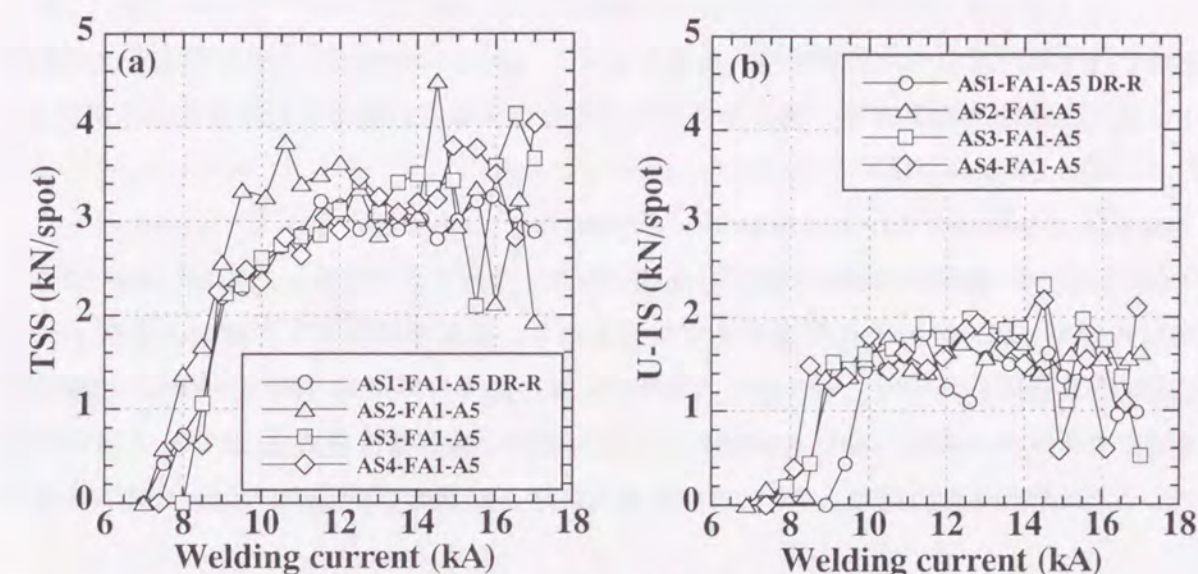
Fig. 6.52 Relation between welding current and tensile strength of galvanized steel-aluminum clad steel-aluminum (AS1-FA1-A5, AS2-FA1-A5, AS3-FA1-A5, AS4-FA1-A5) joints: (a) Tensile shear strength, (b) U-tension strength.
