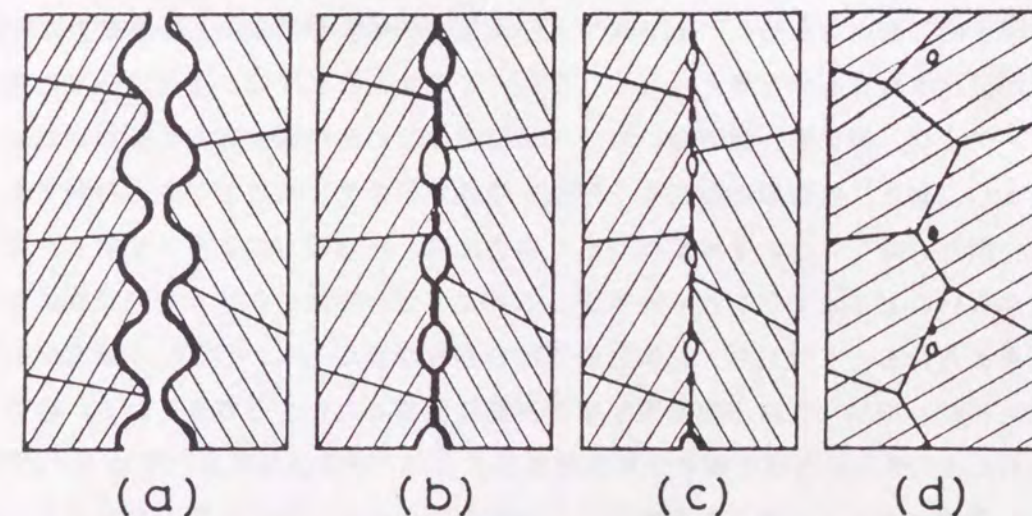
Fig. 2.18 Diffusion bonding model at interface of steel and aluminum.
