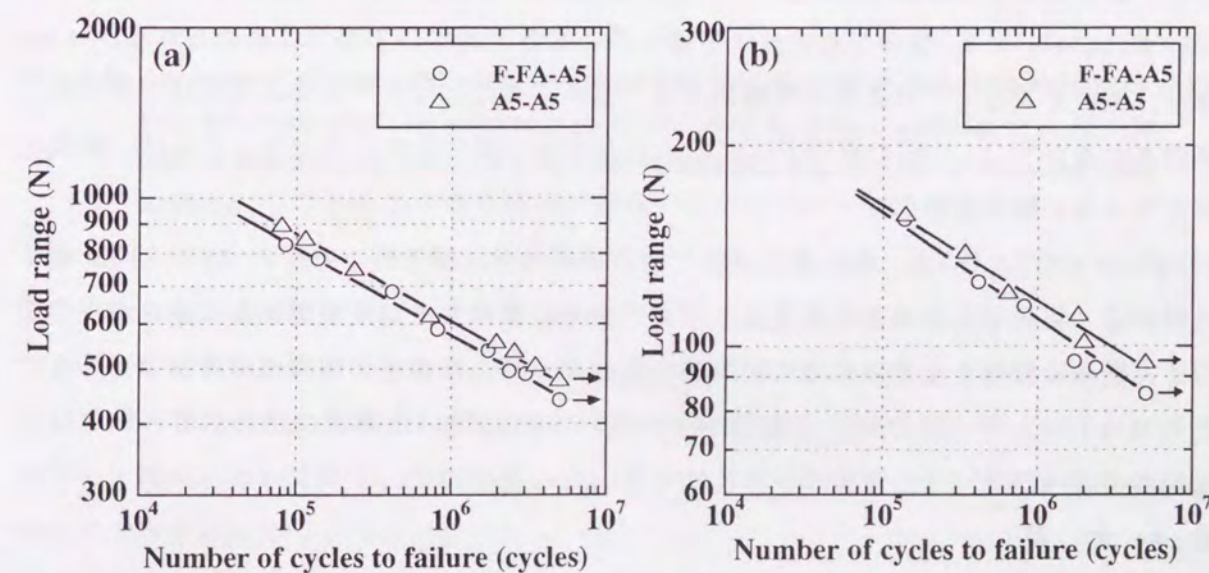
Fig. 6.65 Comparison of fatigue strength of steel-aluminum clad steel-aluminum (F-FA-A5) and aluminum-aluminum (A5-A5) joints: (a) Tensile shear, (b) Cross tension.
