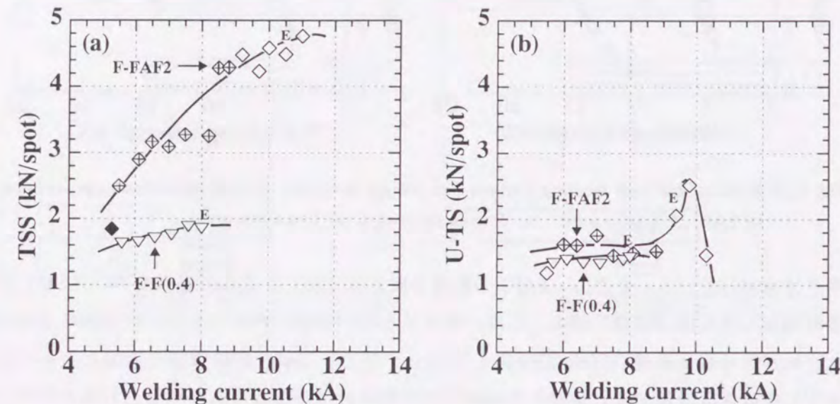
Fig. 5.21 Comparison of tensile strength of steel-steel/aluminum laminate (F-FAF2) and steel-steel (F-F(0.4)) joints: (a) Tensile shear strength (TSS), (b) U-tension strength (U-TS).
