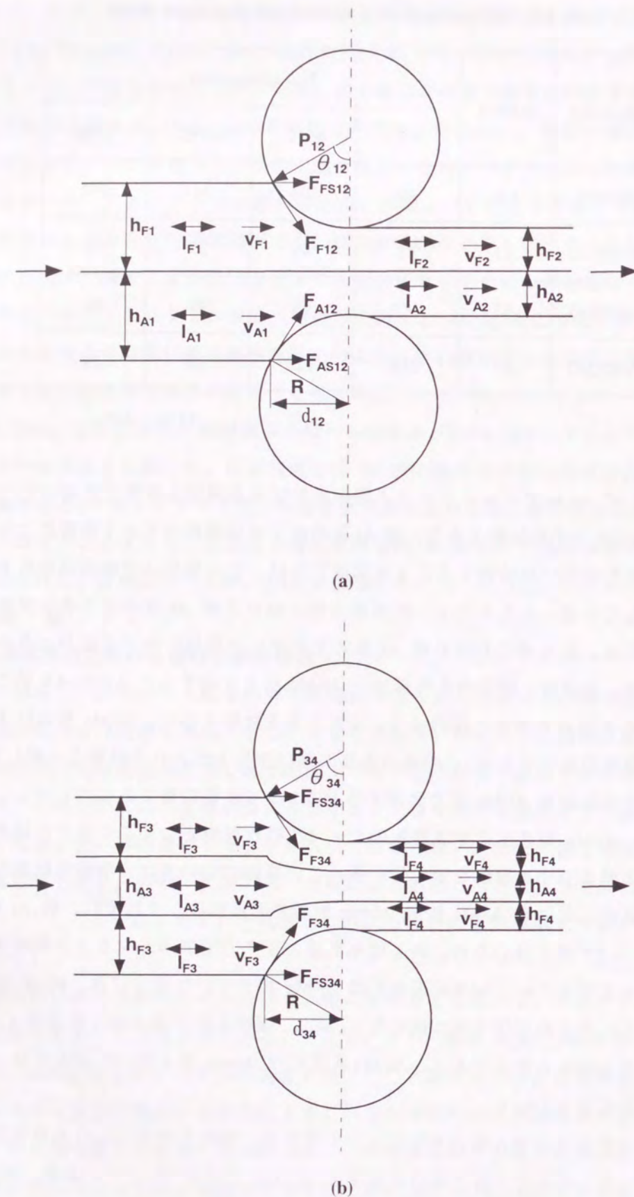
Fig. 2.15 Schematic diagram of rolling bonding of steel and aluminum sheet: (a) Aluminum clad steel sheet, (b) Steel/aluminum laminate.
