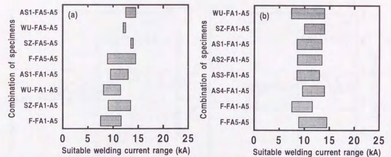
Fig. 6.62 Suitable welding current range of galvanized steel-aluminum clad steel-aluminum and steel-aluminum clad steel-aluminum joints: (a) DR-DR, (b) DR-R.
