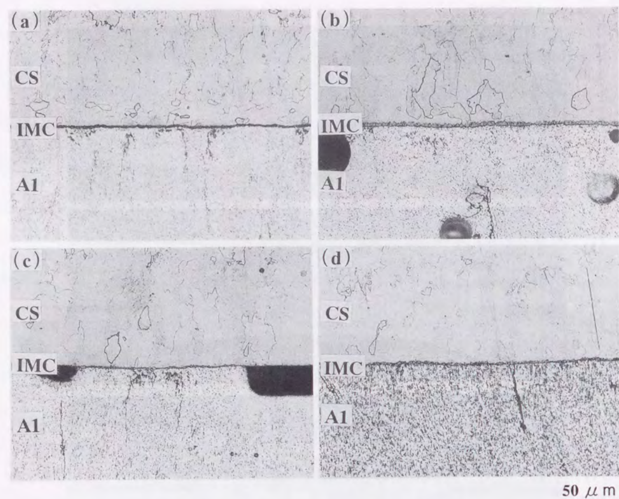
Fig. 6.41 Microstructures at steel/aluminum interfaces of spot weld zones of galvanized steel-aluminum clad steel-aluminum (AS1-FA5-A5) spot weld joints: (a) DR-DR 14.0kA-0.04s, (b) DR-DR 14.0kA-0.12s, (c) CF-R 14.0kA-0.04s, (d) CF-R 14.0kA-0.12s.
