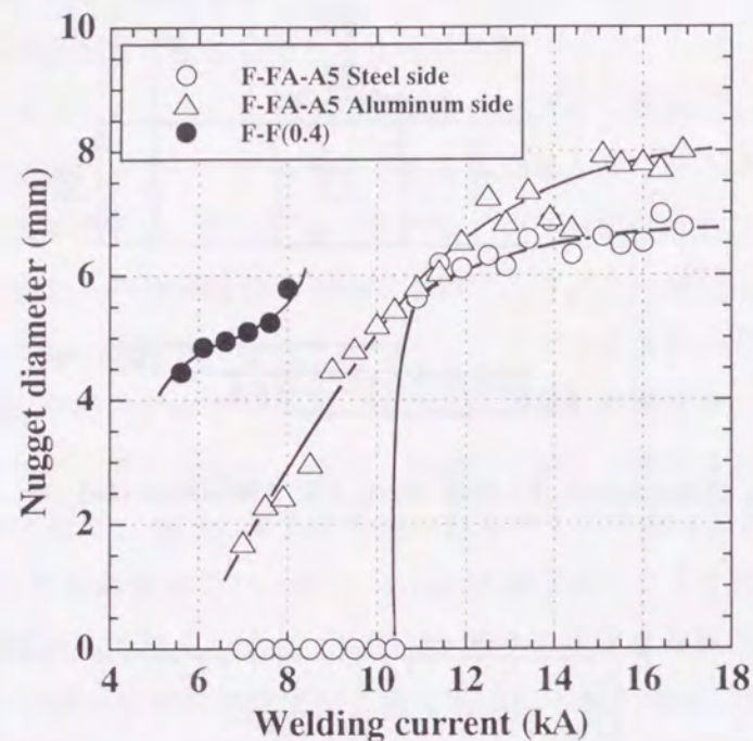
Fig. 6.14 Comparison of nugget diameter in steel and aluminum sheet sides of steel-aluminum clad steel-aluminum (F-FA-A5) joint and steel-steel (F-F(0.4)) joint.
