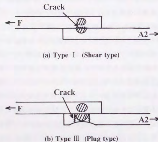
Fig. 4.18 Fracture modes in tensile shear testing of steel-aluminum joint: (a) Type I (Shear type), (b) Type III (Plug type).
