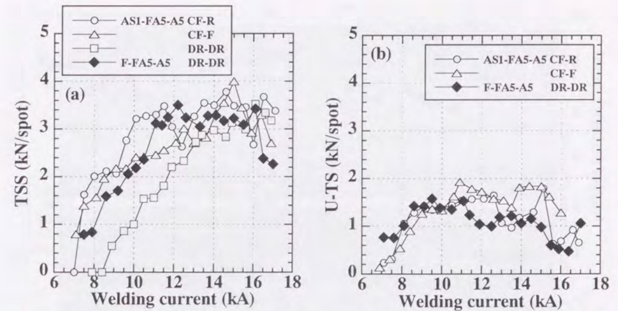
Fig. 6.38 Relation between welding current and tensile strength of galvanized steel-aluminum clad steel-aluminum (AS1-FA5-A5) and steel-aluminum clad steel-aluminum (F-FA5-A5) joints: (a) Tensile shear strength, (b) U-tension strength.
