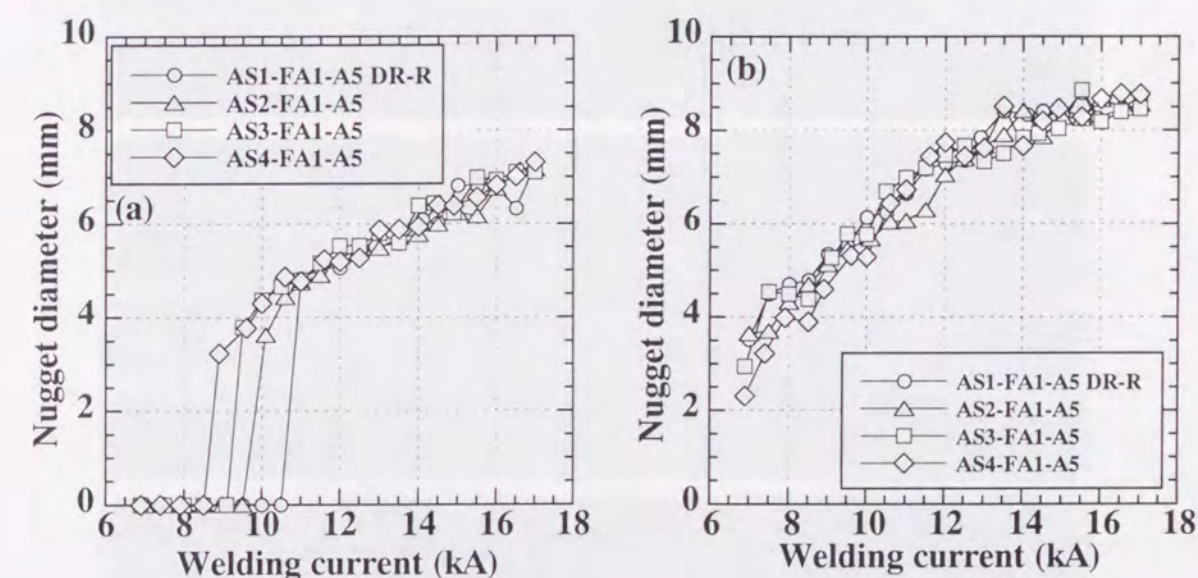
Fig. 6.53 Relation between welding current and nugget diameter of galvanized steel-aluminum clad steel-aluminum (AS1-FA1-A5, AS2-FA1-A5, AS3-FA1-A5, AS4-FA1-A5) joints: (a) Steel sheet side, (b) Aluminum sheet side.
