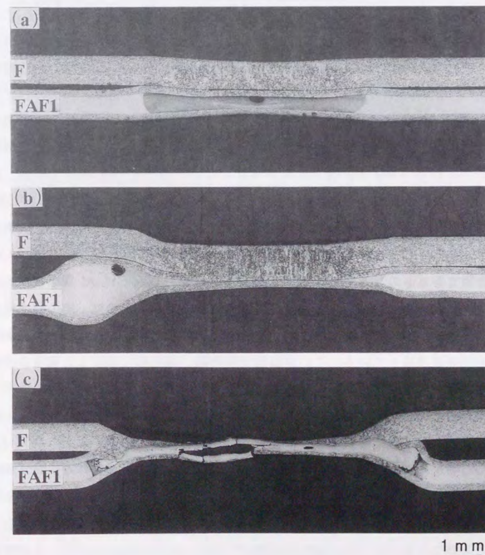
Fig. 5.15 Macrostructures of steel-steel/aluminum laminate (F-FAF1) spot weld joints: (a) 8.1kA-0.2s, (b) 11.9kA-0.2s, (c) 15.5kA-0.2s.
