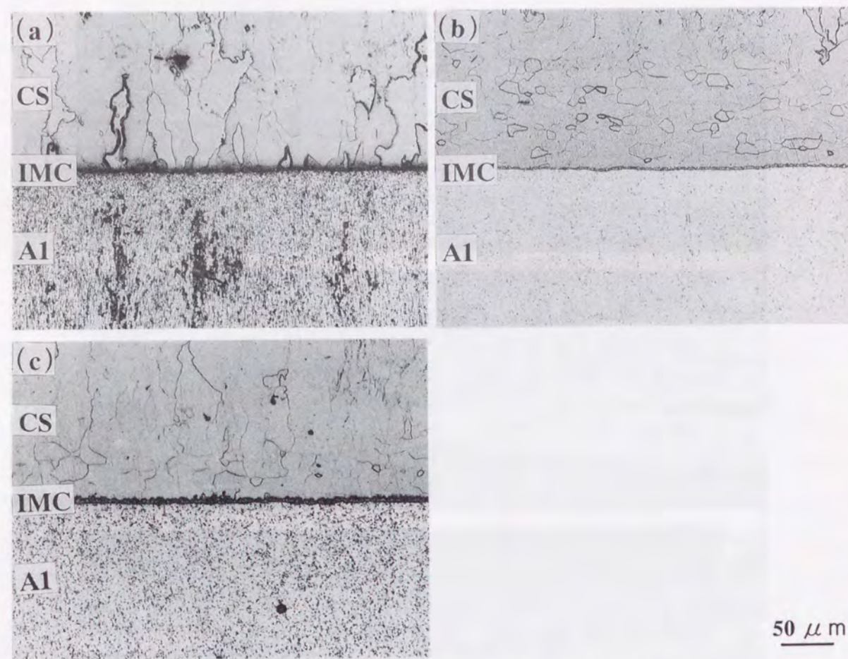
Fig. 6.26 Microstructures at steel/aluminum interfaces of aluminum clad steel sheets after spot welding (10.0kA-0.2s): (a) F-FA5-A2, (b) F-FA5-A5, (c) F-FA5-A6.
