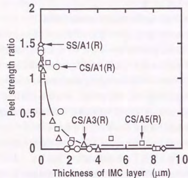
Fig. 3.6 Effect of thickness of intermetallic compound (IMC) layers on peel strength of roll bonding sheets.
