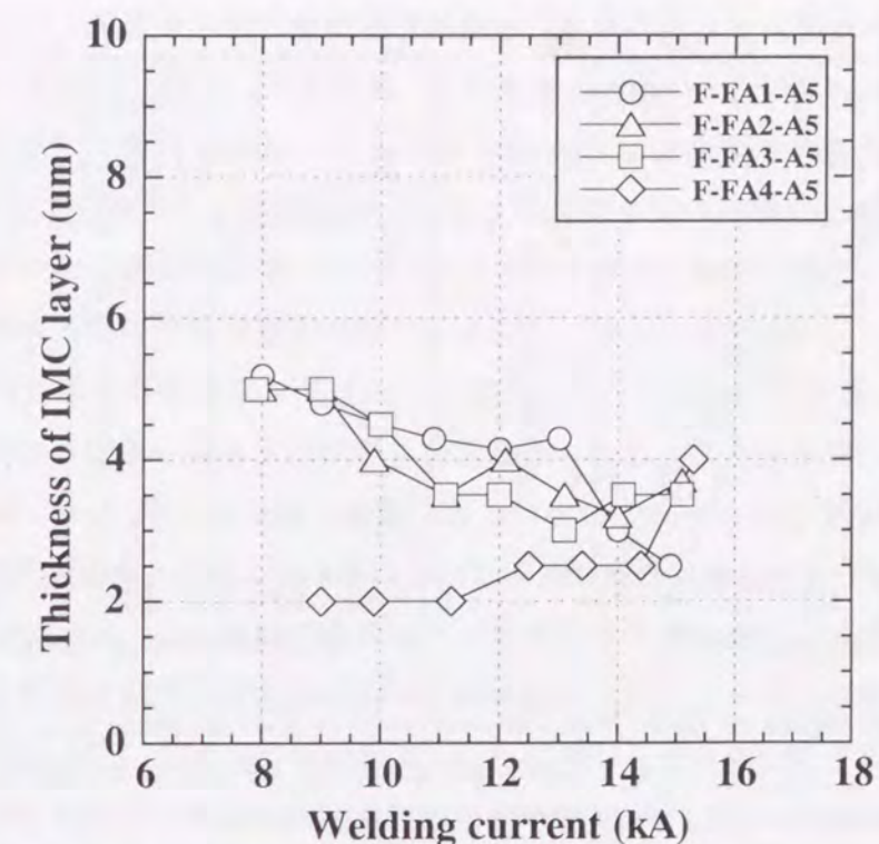
Fig. 6.21 Effects of thickness ratio of aluminum clad steel sheets on thicknesses of iron-aluminum intermetallic compound (IMC) layers formed at steel/aluminum interfaces of steel-aluminum clad steel-aluminum joints.
