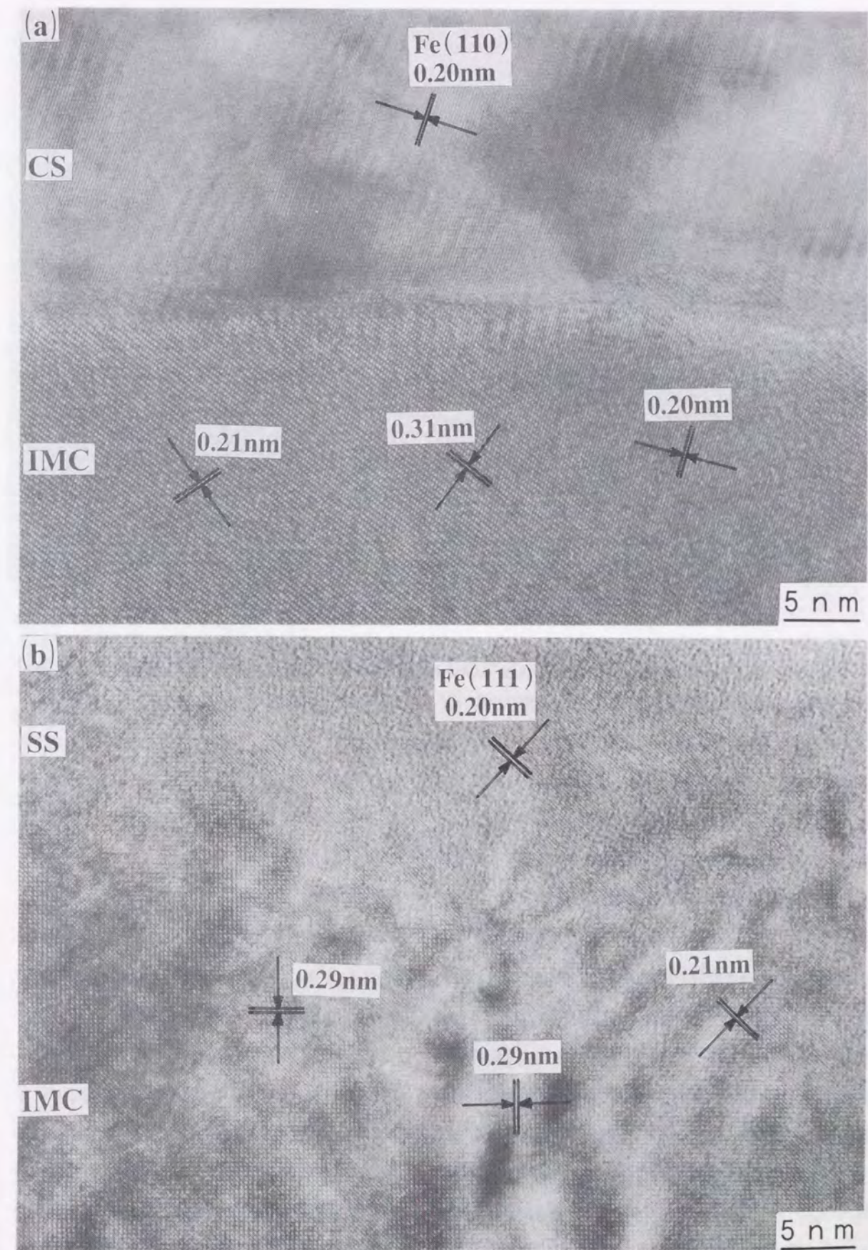
Fig. 3.12 TEM micrographs at steel/IMC interfaces of roll bonding sheets: (a) CS/A5, (b) SS/A1.
