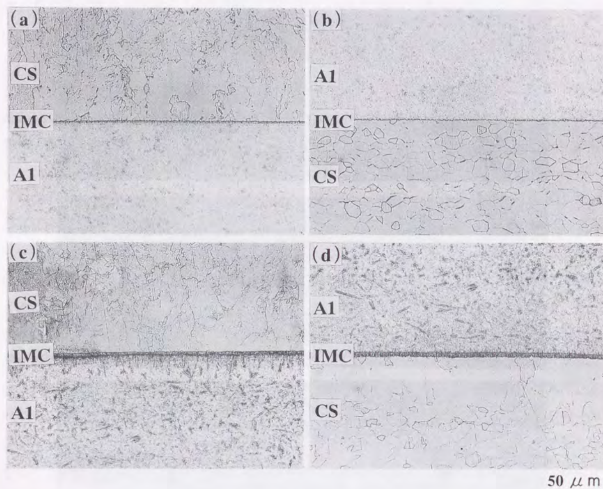
Fig. 5.17 Microstructures at steel/aluminum interfaces of steel/aluminum laminate after spot welding: (a) (b) F-FAF1 8.1kA-0.2s, (c) (d) F-FAF2 8.2kA-0.2s.
