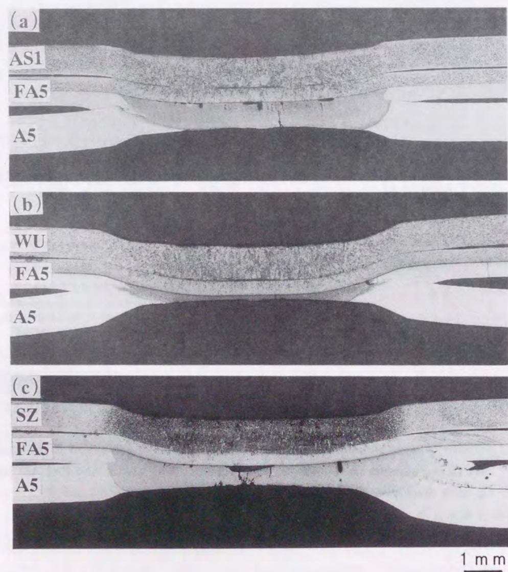
Fig. 6.54 Macrostructures of galvanized steel-aluminum clad steel-aluminum spot weld joints (14.0kA-0.2s): (a) AS1-FA5-A5, (b) WU-FA5-A5, (c) SZ-FA5-A5.
