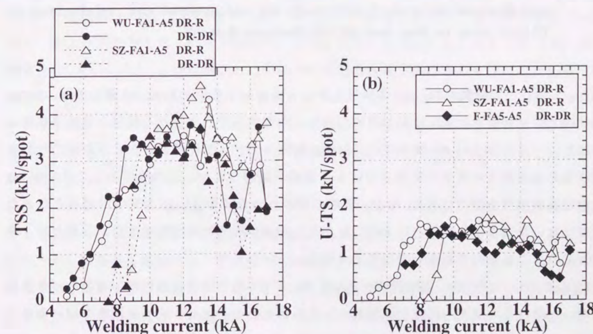
Fig. 6.60 Relation between welding current and tensile strength of galvanized steel-aluminum clad steel-aluminum (WU-FA1-A5, SZ-FA1-A5) and steel-aluminum clad steel-aluminum (F-FA5-A5) joints: (a) Tensile shear strength, (b) U-tension strength.
