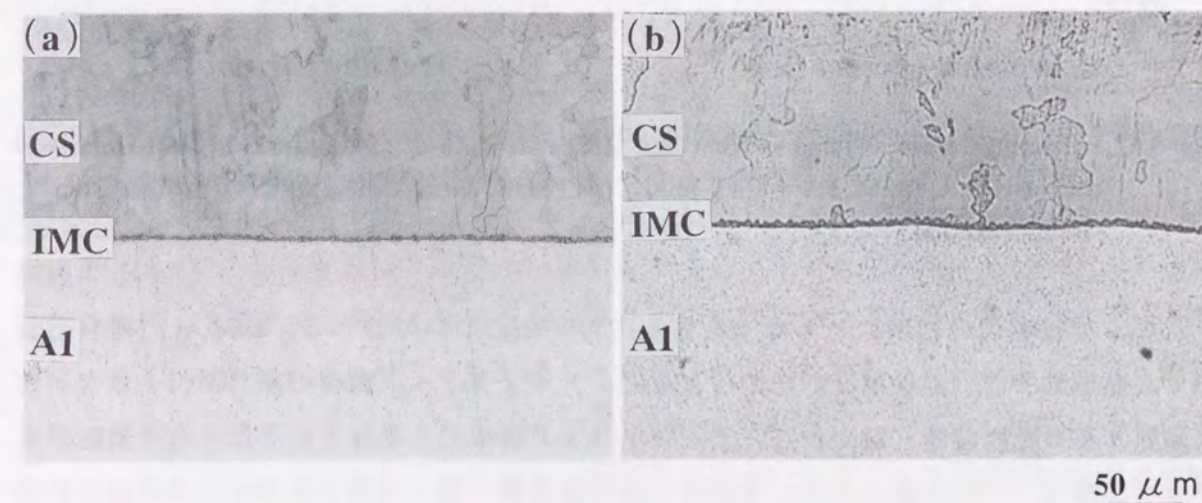
Fig. 5.11 Microstructures at steel/aluminum interfaces of aluminum clad steel sheets after spot welding: (a) FA-FA(F) 14.3kA-0.2s, (b) FA-FA(A) 10.8kA-0.2s.
