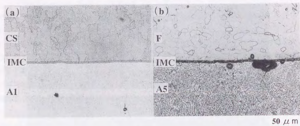
Fig. 6.6 Microstructures at steel/aluminum interfaces of spot weld zones: (a) steel-aluminum clad steel-aluminum joint (F-FA-A5 10.8kA-0.2s), (b) steel-aluminum joint (F-A5 10.0kA-0.2s).
