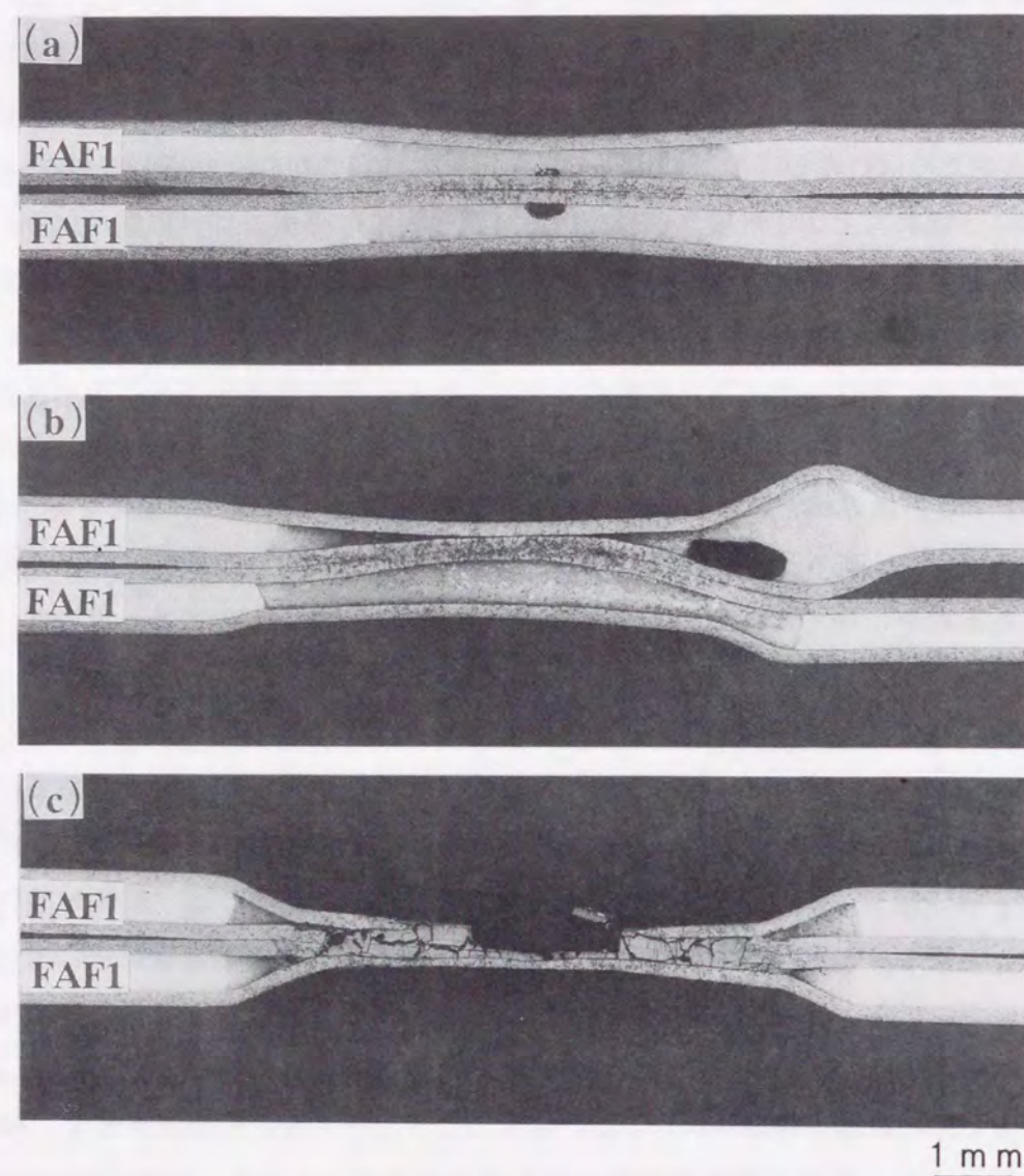
Fig. 5.22 Macrostructures of steel/aluminum laminate-steel/aluminum laminate (FAF1-FAF1) spot weld joints: (a) 9.0kA-0.2s, (b) 12.9kA-0.2s, (c) 16.0kA-0.2s.
