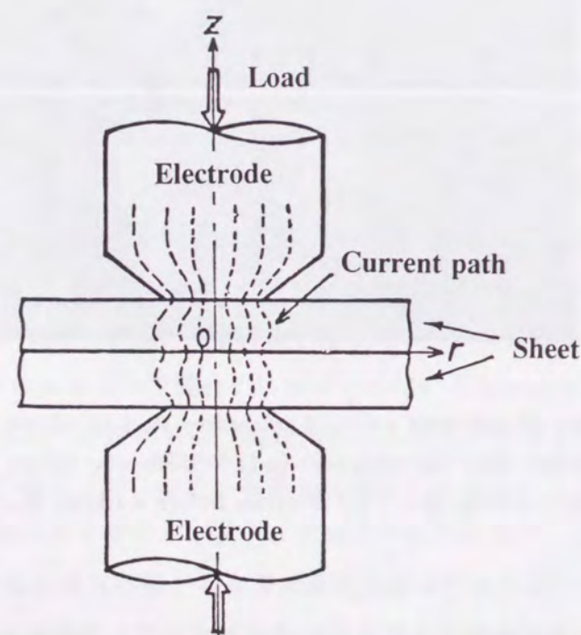
Fig. 6.68 Principal of resistance spot welding.
