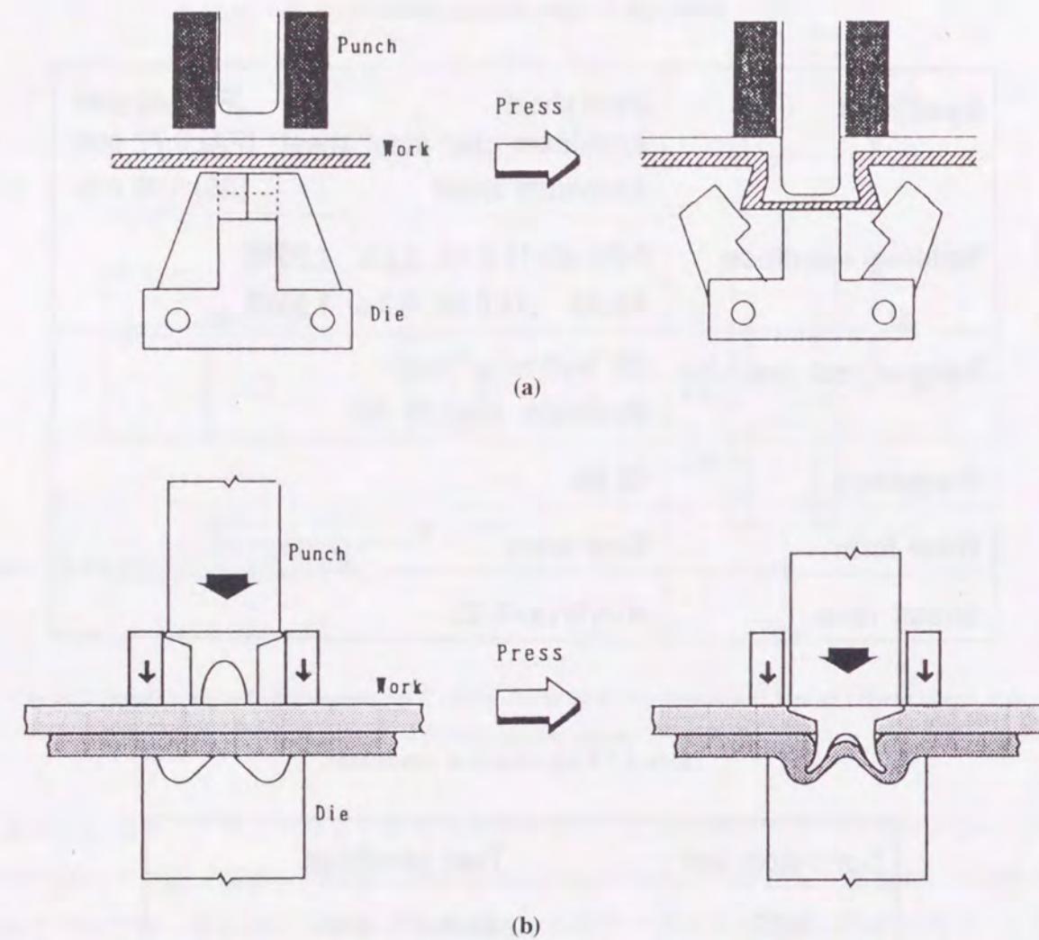
Fig. 6.2 Mechanical joining methods: (a) Tog lock (TGL) method, (b) Self piercing & riveting (SPR) method.
