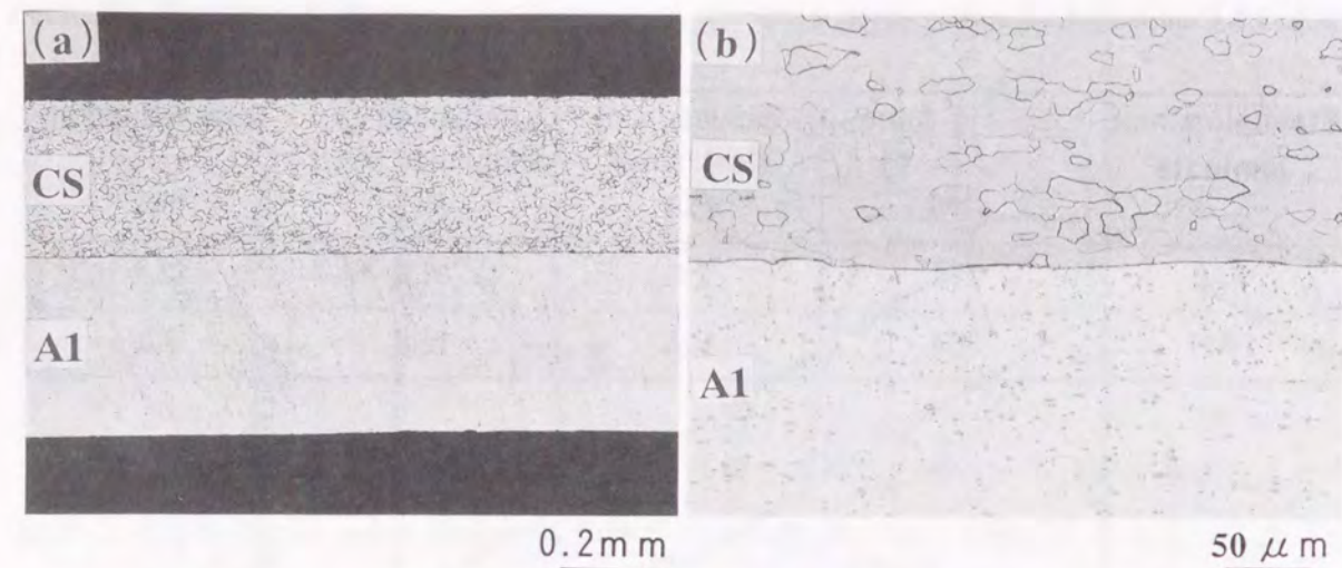
Fig. 2.7 Cross-section of aluminum clad steel sheet: (a) Macrostructure, (b) Microstructure.
