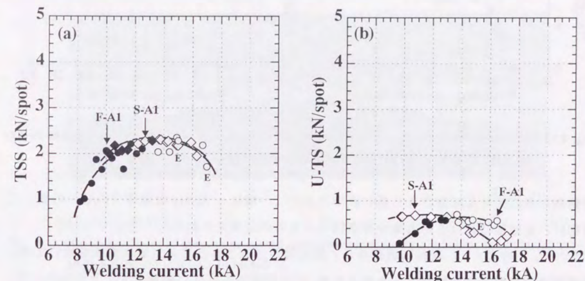
Fig. 4.11 Relation between welding current and tensile strength of stainless steel-aluminum (S-A1) and steel-aluminum (F-A1) joints: (a) Tensile shear strength, (b) U-tension strength.
