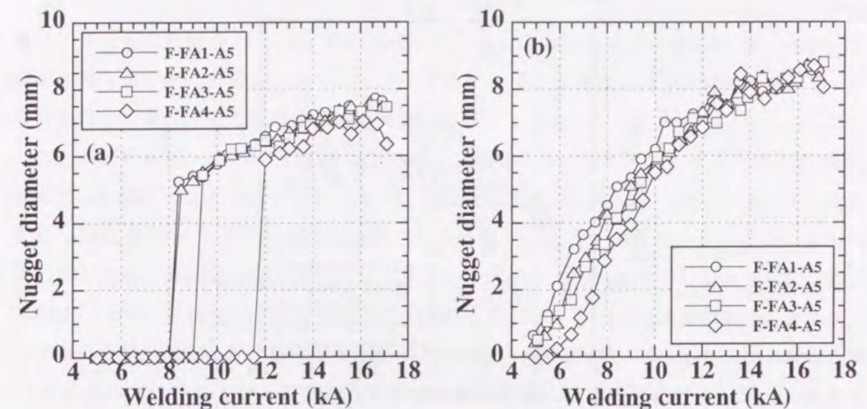
Fig. 6.22 Effects of thickness ratio of aluminum clad steel sheets on nugget diameters of joints: (a) Steel sheet side, (b) Aluminum sheet side.
