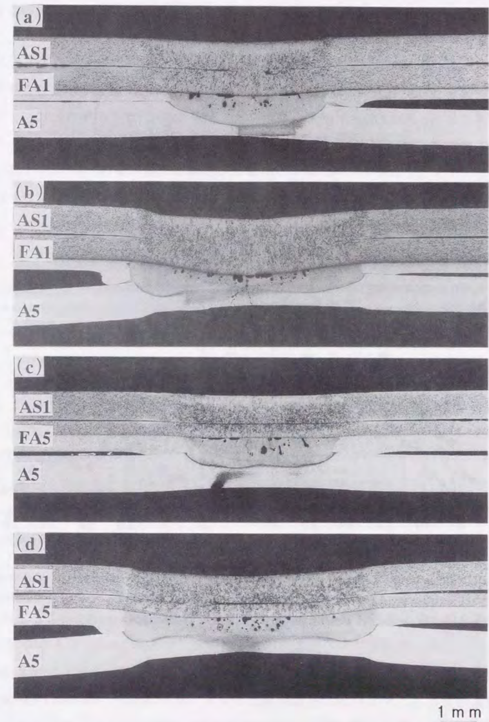
Fig. 6.44 Nugget formation process of galvanized steel-aluminum clad steel-aluminum (AS1-FA1-A5, AS1-FA5-A5) spot weld joints: (a) AS1-FA1-A5 14.0kA-0.04s, (b) AS1-FA1-A5 14.0kA-0.08s, (c) AS1-FA5-A5 14.0kA-0.04s, (d) AS1-FA5-A5 14.0kA-0.08s.
