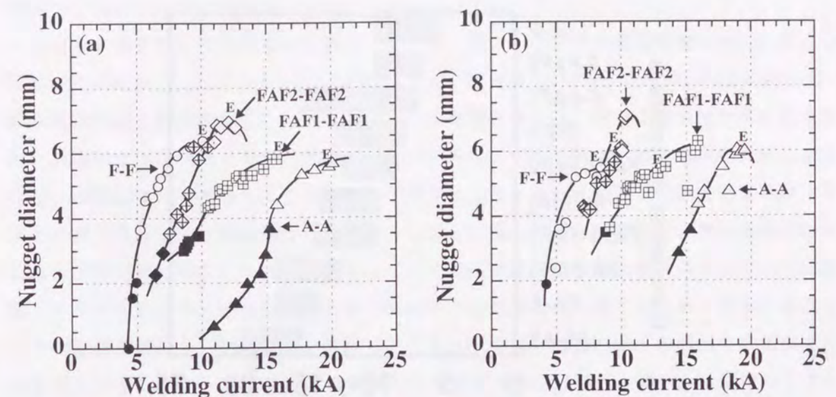
Fig. 5.27 Relation between welding current and nugget diameter of steel/aluminum laminate-steel/aluminum laminate (FAF1-FAF1, FAF2-FAF2) joints: (a) Tensile shear test, (b) U-tension test.
