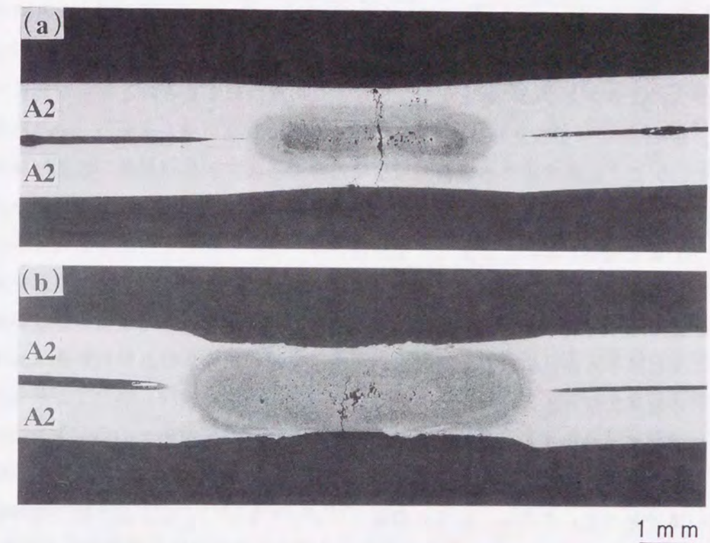
Fig. 4.8 Macrostructures of aluminum-aluminum (A2-A2) spot weld joints: (a) 14.9kA-0.2s, (b) 19.8kA-0.2s.
