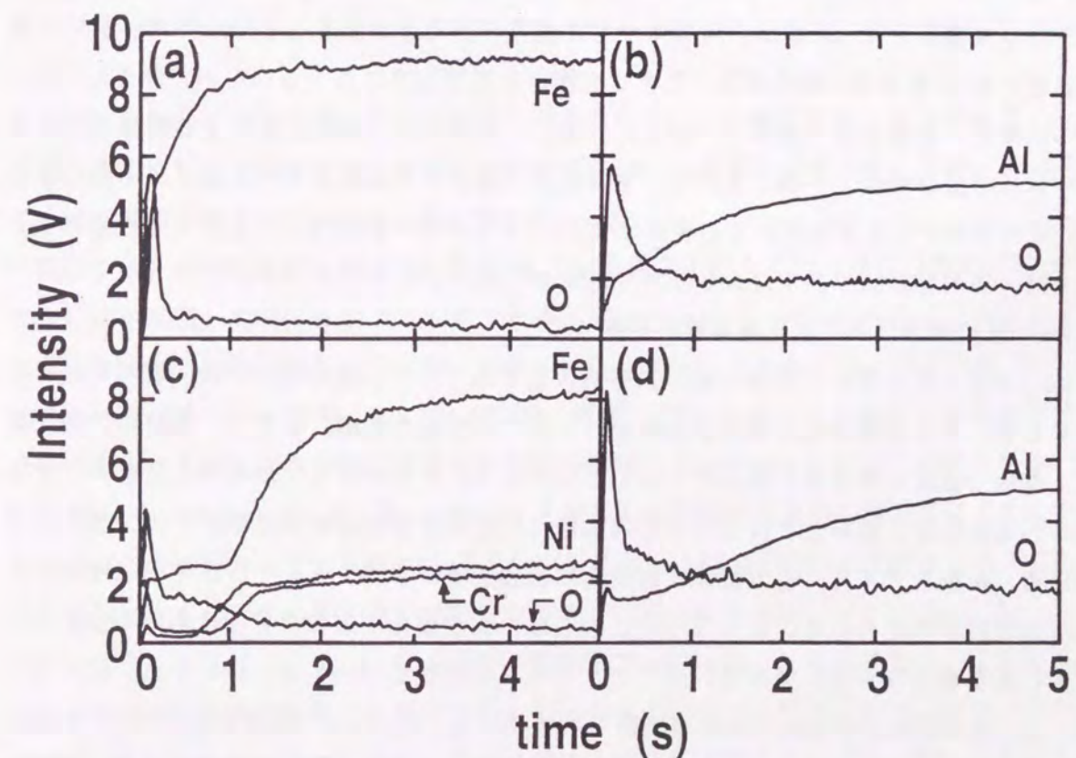
Fig. 2.4 GDS depth profiles of steel and aluminum sheets just before roll bonding: (a) Steel sheet side (FA1), (b) Aluminum sheet side (FA1), (c) Stainless steel sheet side (SA), (d) Aluminum sheet side (SA).
