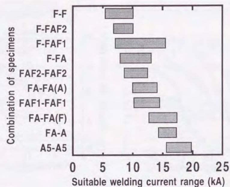
Fig. 5.28 Comparison of suitable welding current range of various joints.
