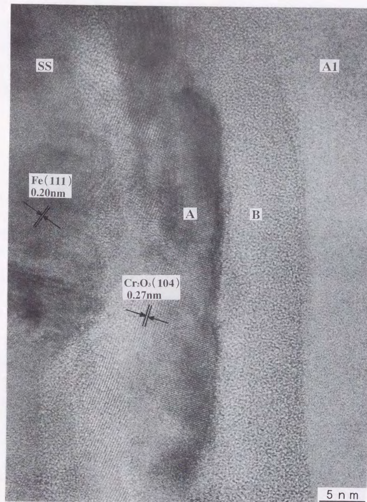
Fig. 2.13 TEM micrograph at interface of aluminum clad stainless steel sheet (SA).
