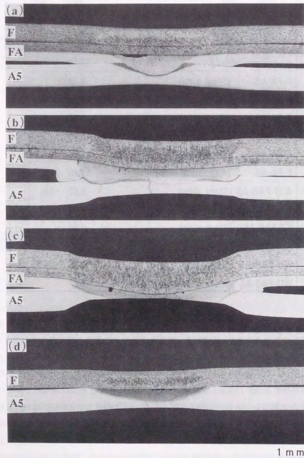
Fig. 6.3 Macrostructures of steel-aluminum clad steel-aluminum (F-FA-A5) and steel-aluminum (F-A5) spot weld joints: (a) F-FA-A5 8.0kA-0.2s, (b) F-FA-A5 10.8kA-0.2s, (c) F-FA-A5 14.4kA-0.2s, (d) F-A5 10.0kA-0.2s.
