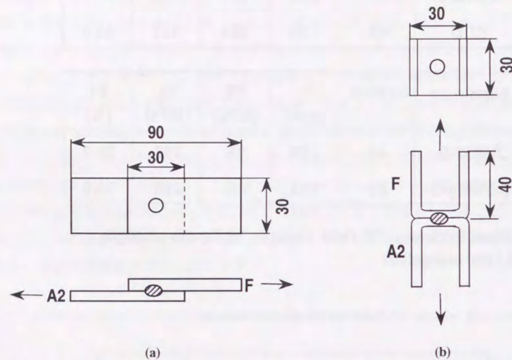
Fig. 4.1 Dimensions of specimens (mm): (a) Tensile shear test, (b) U-tension test (F: steel sheet, A2: aluminum sheet).
