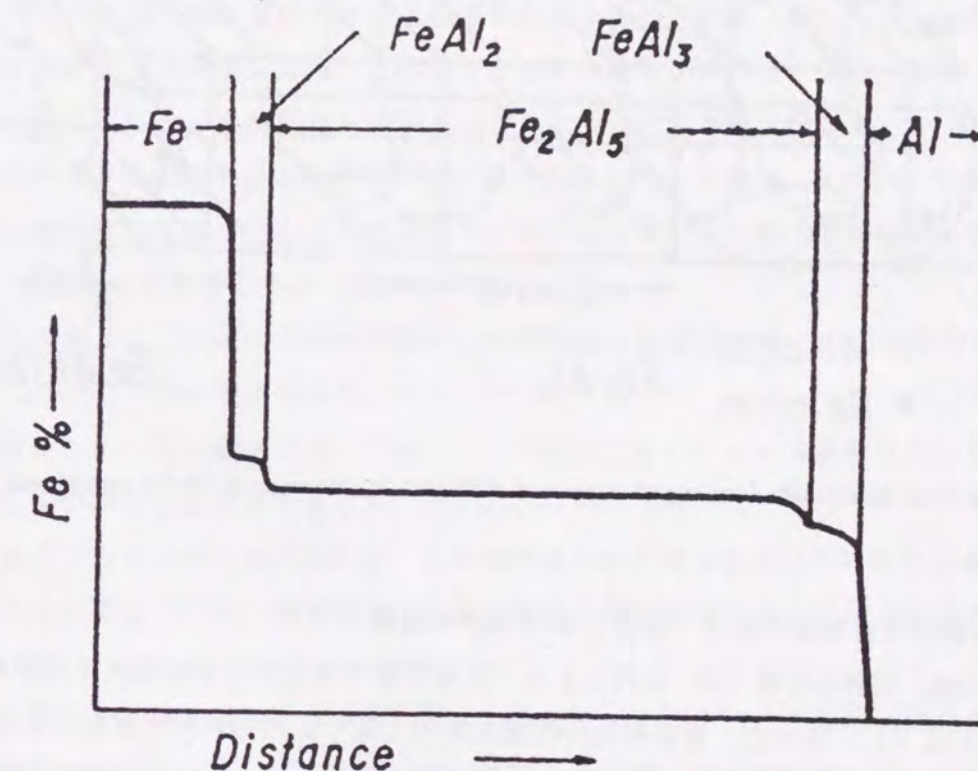
Fig. 3.15 Change of iron content in iron-aluminum intermetallic compound (IMC) layer formed at interface of bonding sheets.
