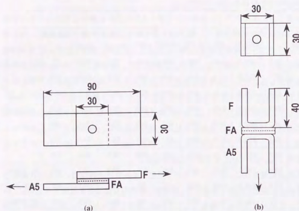
Fig. 6.1 Dimensions of specimens: (a) Tensile shear test, (b) U-tension test (F: Steel sheet, FA: Aluminum clad steel sheet, A5: Aluminum sheet).
