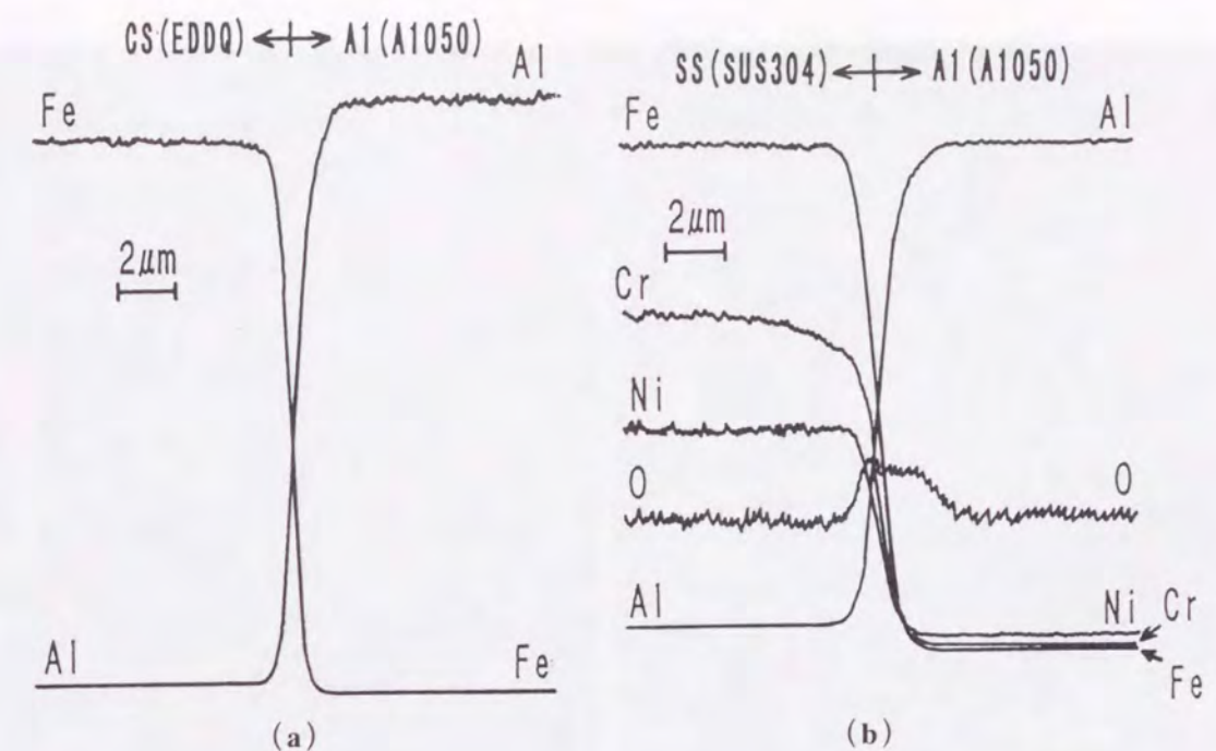
Fig. 2.8 EPMA line analyses at interfaces of aluminum clad steel sheet and aluminum clad stainless steel sheet: (a) FA1, (b) SA.
