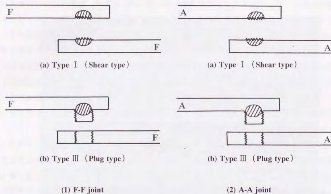
Fig. 5.3 Fracture modes observed in tensile shear testing and U-tension testing of steel-steel (F-F) and aluminum-aluminum (A-A) joints.
