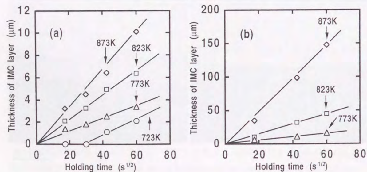
Fig. 3.2 Relation between square root of holding time and thickness of intermetallic compound (IMC) layers: (a) CS/A1(R), (b) CS/A1(D).
