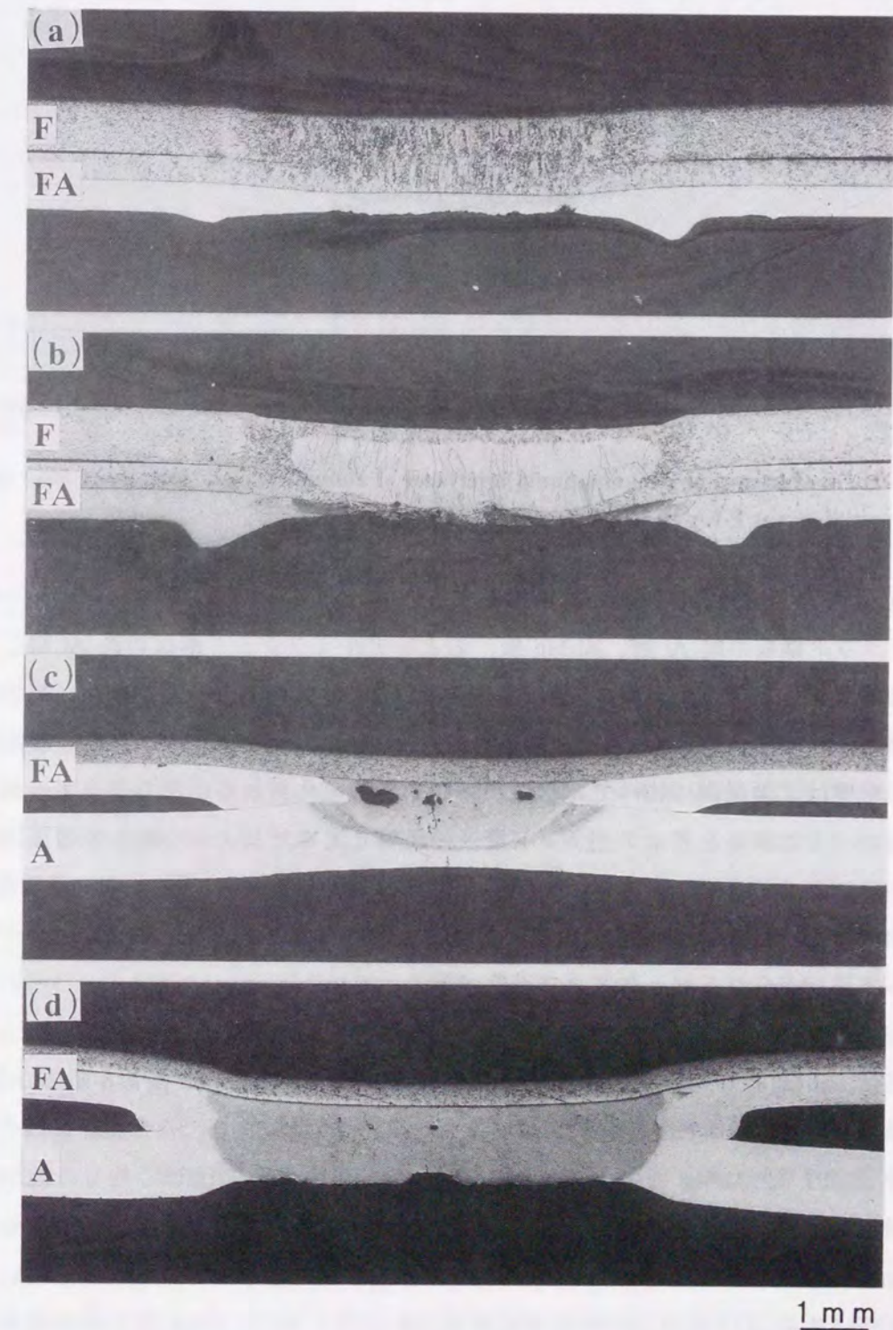
Fig. 5.5 Macrostructures of steel-aluminum clad steel (F-FA) and aluminum clad steel-aluminum (FA-A) spot weld joints: (a) F-FA 10.5kA-0.2s, (b) F-FA 12.2kA-0.2s, (c) FA-A 14.6kA-0.2s, (d) FA-A 17.3kA-0.2s.
