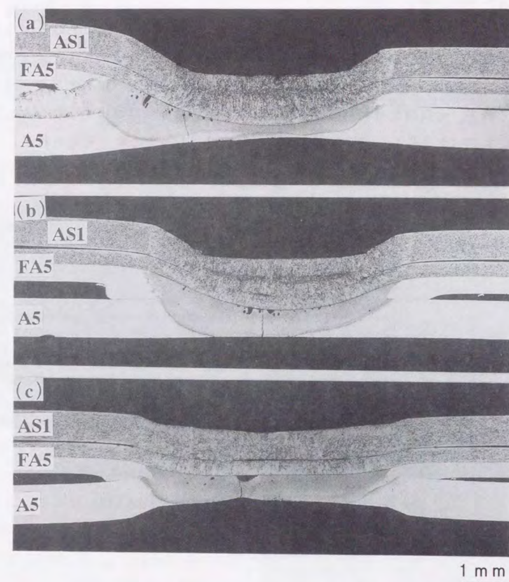
Fig. 6.36 Macrostructures of galvanized steel-aluminum clad steel-aluminum (AS1-FA5-A5) spot weld joints: (a) CF-R 13.1kA-0.2s, (b) CF-F 13.0kA-0.2s, (c) DR-DR 13.0kA-0.2s.
