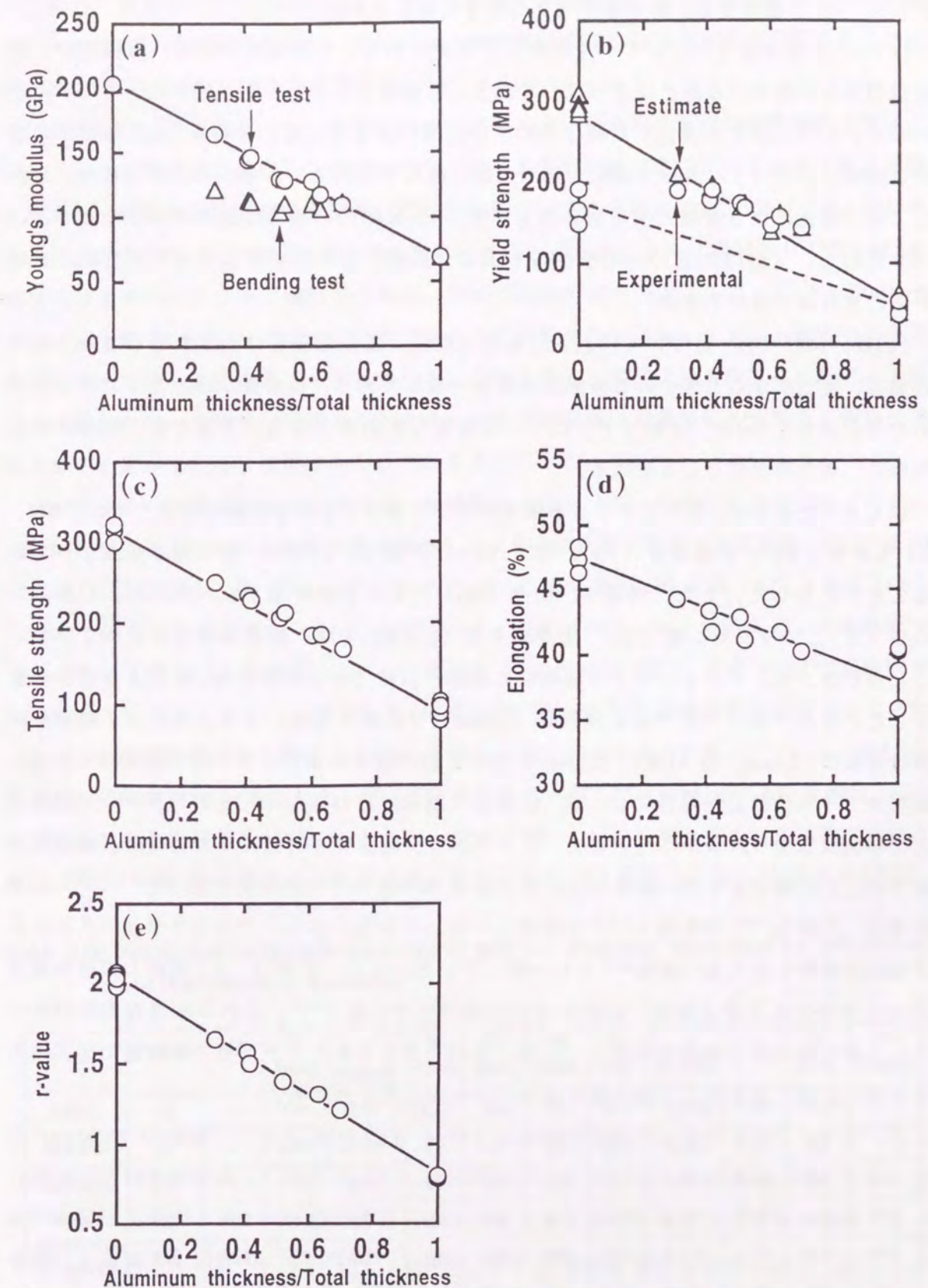
Fig. 2.14 Effect of aluminum layer thickness ratio on mechanical properties of aluminum clad steel sheets: (a) Young's modulus, (b) Yield strength, (c) Tensile strength, (d) Total elongation, (e) r-value.
