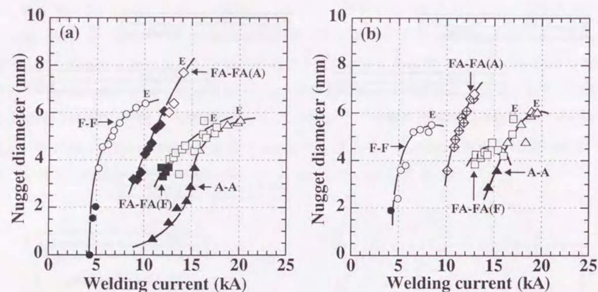
Fig. 5.14 Relation between welding current and nugget diameter of aluminum clad steel-aluminum clad steel (FA-FA(F), FA-FA(A)) joints: (a) Tensile shear test, (b) U-tension test.
