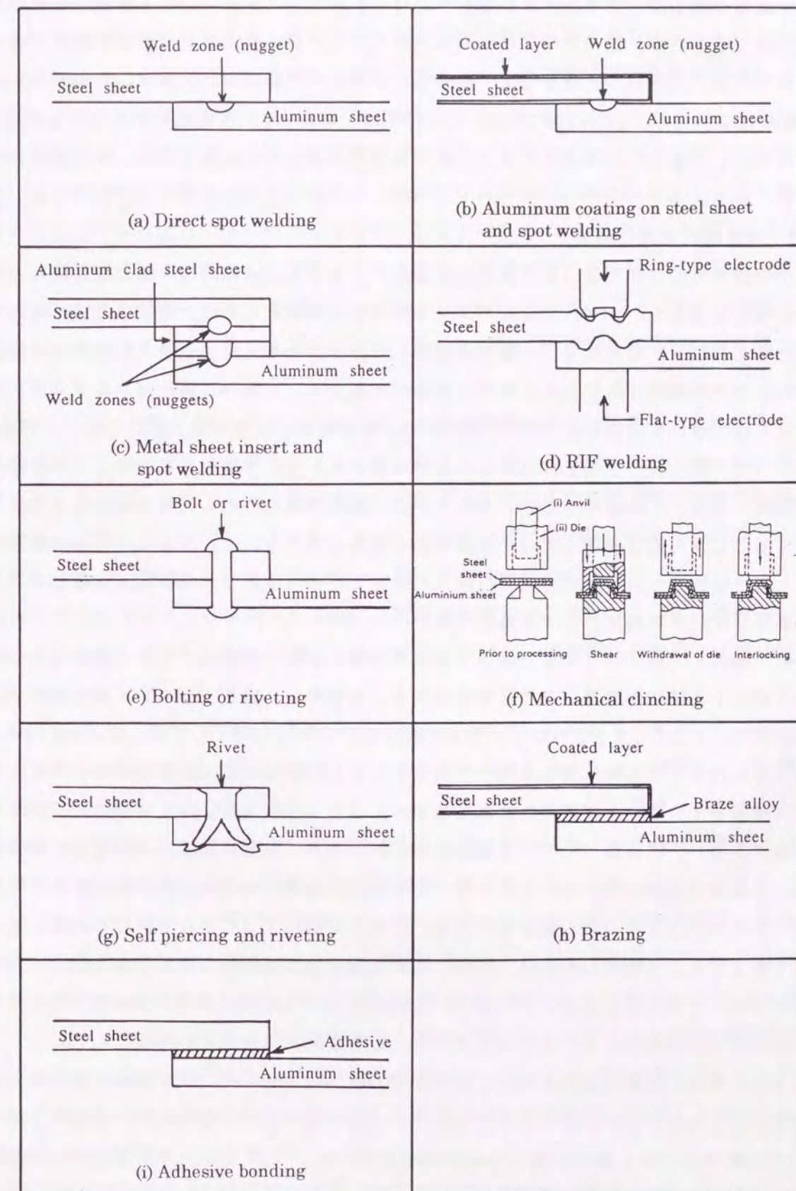
Fig. 1.1 Comparison of steel-aluminum joining methods.
