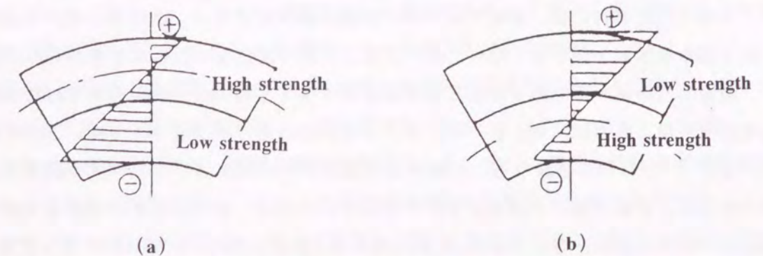
Fig. 2.20 Movement of neutral face in laminate by bending: (a) High strength material sheet existed in outside, (b) High strength material sheet existed in inside.
