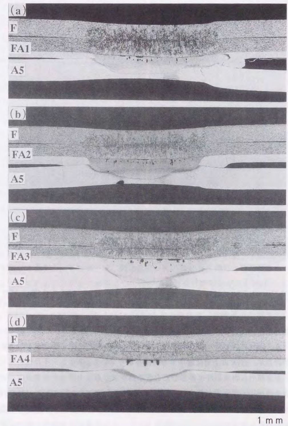
Fig. 6.19 Macrostructures of steel-aluminum clad steel-aluminum spot weld joints (9.0kA-0.2s): (a) F-FA1-A5, (b) F-FA2-A5, (c) F-FA3-A5 and (d) F-FA4-A5.
