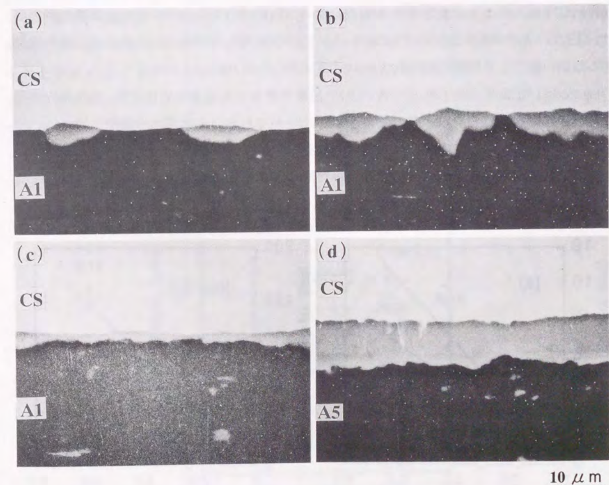
Fig. 3.1 SEM micrographs of intermetallic compound (IMC) layers formed at interfaces of roll bonding sheets: (a) CS/A1(R) 723K-1.8ks, (b) CS/A1(R) 723K-3.6ks, (c) CS/A1(R) 773K-0.3ks, (d) CS/A5(R) 723K-1.8ks.
