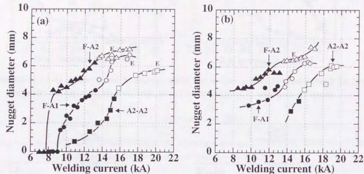
Fig. 4.7 Relation between welding current and nugget diameter of steel-aluminum (F-A1, F-A2) and aluminum-aluminum (A2-A2) joints: (a) Tensile shear test, (b) U-tension test.
