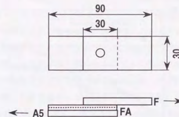
Fig. 6.12 Dimensions of specimens (F: Steel sheet, FA: Aluminum clad steel sheet, A5: Aluminum sheet).
