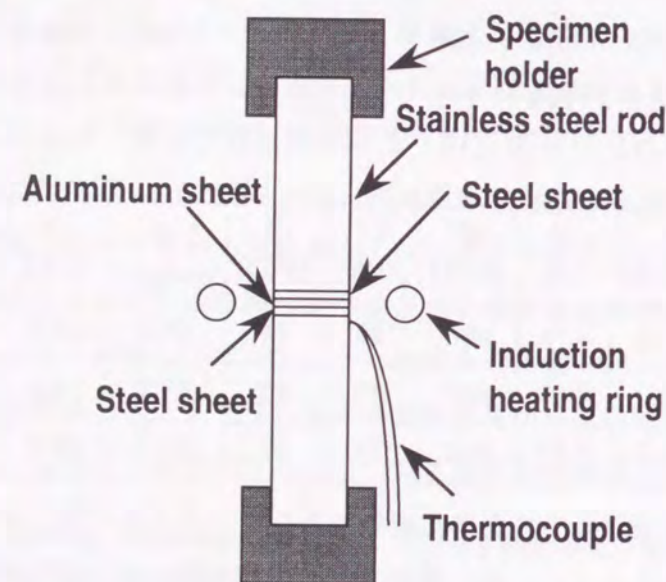
Fig. 2.2 Schematic diagram of diffusion bonding apparatus.
