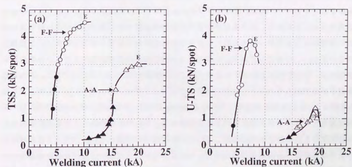
Fig. 5.2 Relation between welding current and tensile strength of steel-steel (F-F) and aluminum-aluminum (A-A) joints: (a) Tensile shear strength (TSS), (b) U-tension strength (U-TS).
