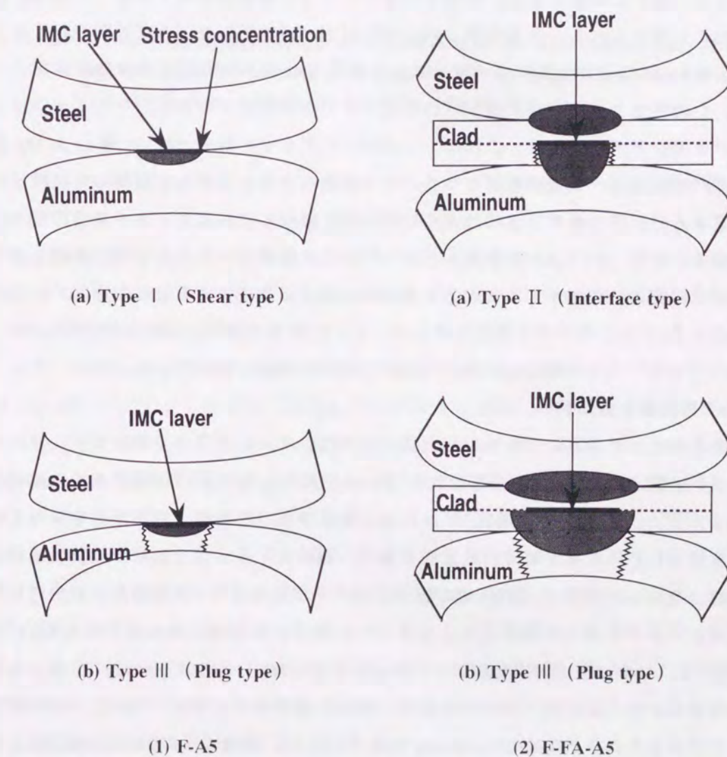
Fig. 6.69 Comparison of fracture modes of steel-aluminum (F-A5) and steel-aluminum clad steel-aluminum (F-FA-A5) joints.
