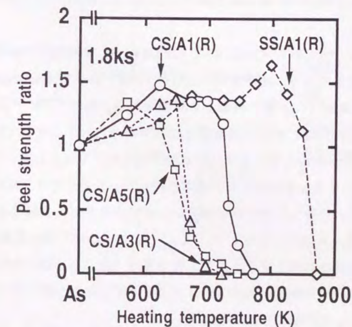
Fig. 3.5 Effect of heating temperature on peel strength of roll bonding sheets.
