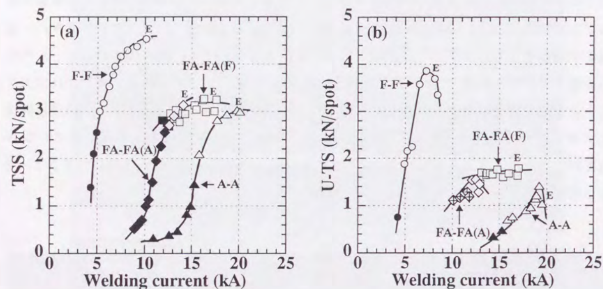
Fig. 5.12 Relation between welding current and tensile strength of aluminum clad steel-aluminum clad steel (FA-FA(F), FA-FA(A)) joints: (a) Tensile shear strength (TSS), (b) U-tension strength (U-TS).
