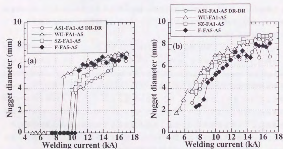
Fig. 6.59 Relation between welding current and nugget diameter of galvanized steel-aluminum clad steel-aluminum (AS1-FA1-A5, WU-FA1-A5, SZ-FA1-A5) and steel-aluminum clad steel-aluminum (F-FA5-A5) joints: (a) Steel sheet side, (b) Aluminum sheet side.
