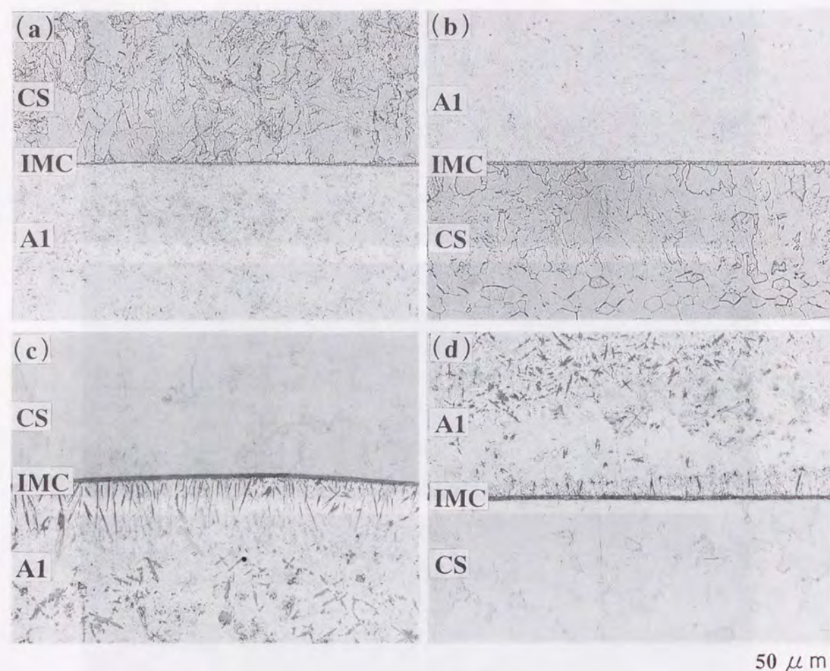
Fig. 5.24 Microstructures at steel/aluminum interfaces of steel/aluminum laminates after spot welding: (a) (b) FAF1-FAF1 12.9kA-0.2s, (c) (d) FAF2-FAF2 8.8kA-0.2s.
