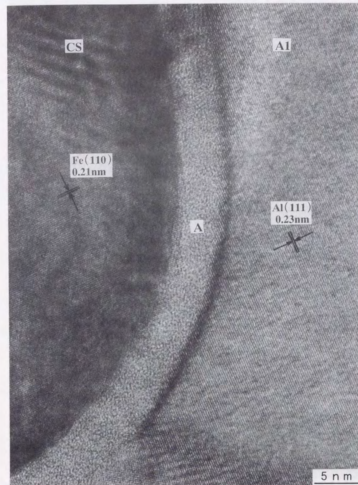
Fig. 2.11 TEM micrograph at interface of aluminum clad steel sheet (FA1).
