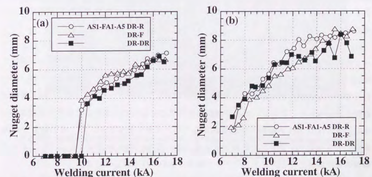
Fig. 6.49 Relation between welding current and nugget diameter of galvanized steel-aluminum clad steel-aluminum (AS1-FA1-A5) joints: (a) Steel sheet side, (b) Aluminum sheet side.
