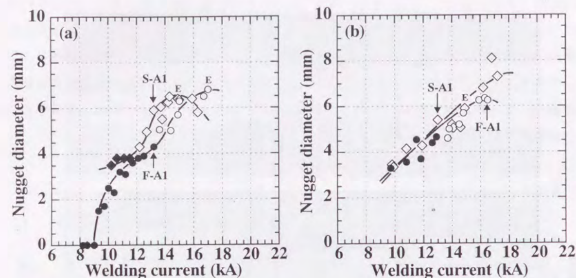
Fig. 4.12 Relation between welding current and nugget diameter of stainless steel-aluminum (S-A1) and steel-aluminum (F-A1) joints: (a) Tensile shear test, (b) U-tension test.
