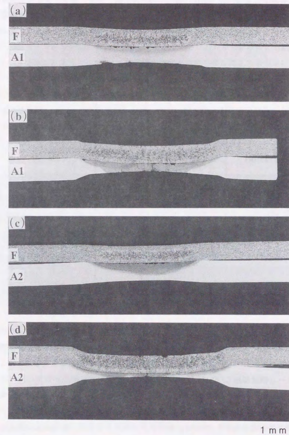
Fig. 4.2 Macrostructures of steel-aluminum spot weld joints: (a) F-A1 10.0kA-0.2s, (b) F-A1 14.4kA-0.2s, (c) F-A2 10.0kA-0.2s, (d) F-A2 14.6kA-0.2s.
