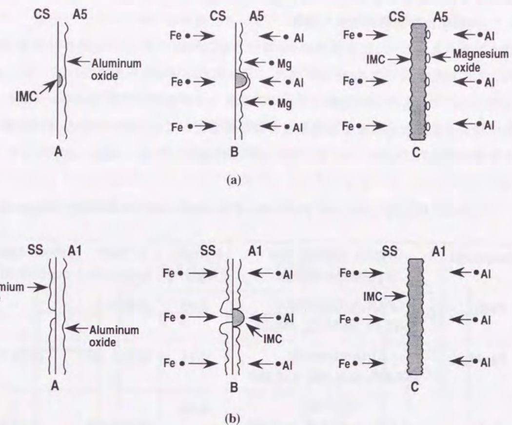
Fig. 3.14 Reaction model at interfaces of roll bonding sheets: (a) CS/A5, (b) SS/A1.
