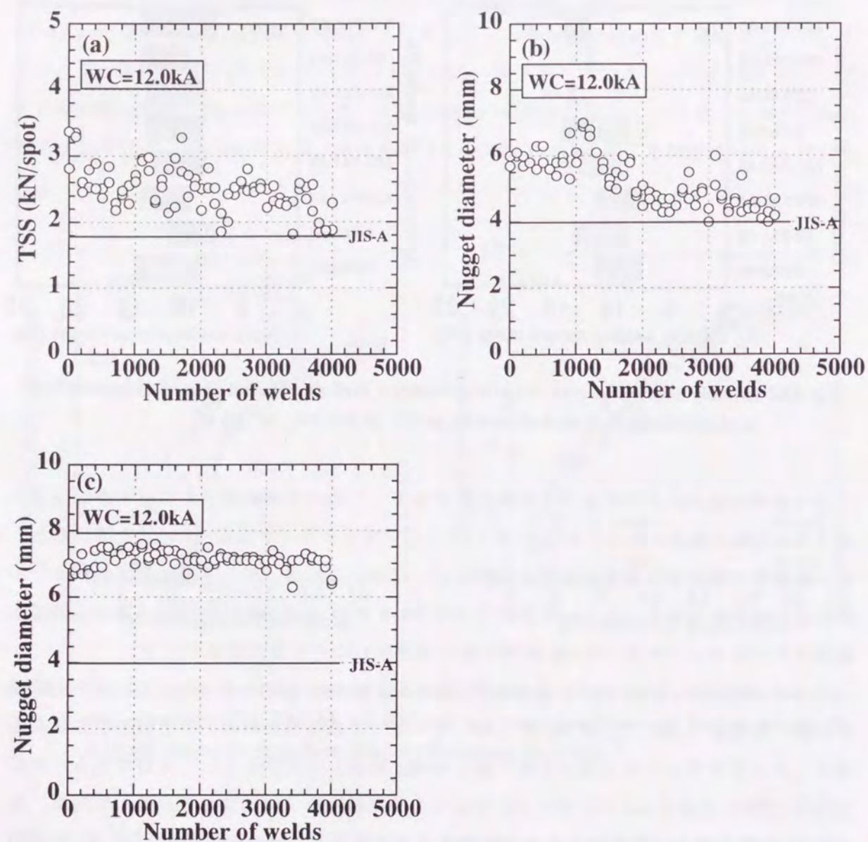
Fig. 6.63 Tensile shear strength and nugget diameter of galvanized steel-aluminum clad steel-aluminum (AS1-FA1-A5) joints as a function of number of welds: (a) Tensile shear strength, (b) Nugget diameter on steel sheet side, (c) Nugget diameter on aluminum sheet side.
