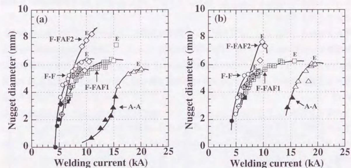
Fig. 5.20 Relation between welding current and nugget diameter of steel-steel/aluminum laminate (F-FAF1, F-FAF2) joints: (a) Tensile shear test, (b) U-tension test.
