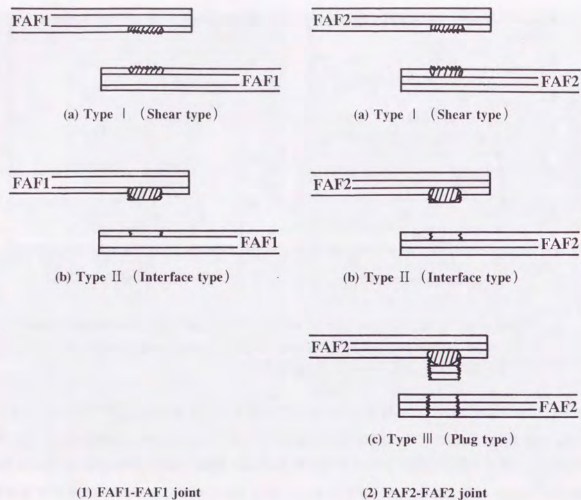
Fig. 5.26 Fracture modes observed in tensile shear testing and U-tension testing of steel/aluminum laminate-steel/aluminum laminate (FAF1-FAF1, FAF2-FAF2) joints.
