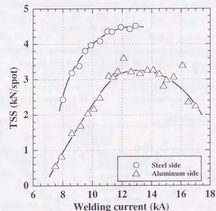
Fig. 6.13 Relation between welding current and tensile shear strength in steel and aluminum sheet sides of steel-aluminum clad steel-aluminum joints (F-FA-A5).
