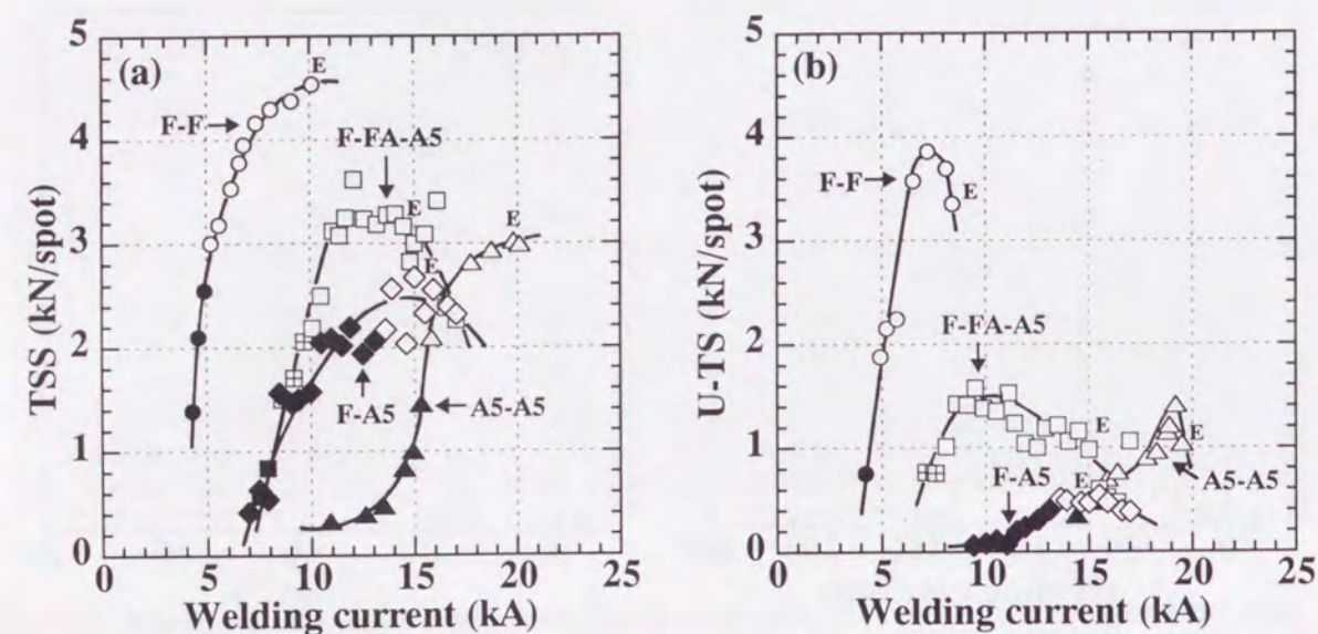
Fig. 6.9 Relation between welding current and tensile strength of steel-aluminum clad steel-aluminum joints (F-FA-A5), steel-aluminum joints (F-A5), steel-steel joints (F-F) and aluminum-aluminum joints (A5-A5): (a) Tensile shear strength, (b) U-tension strength.
