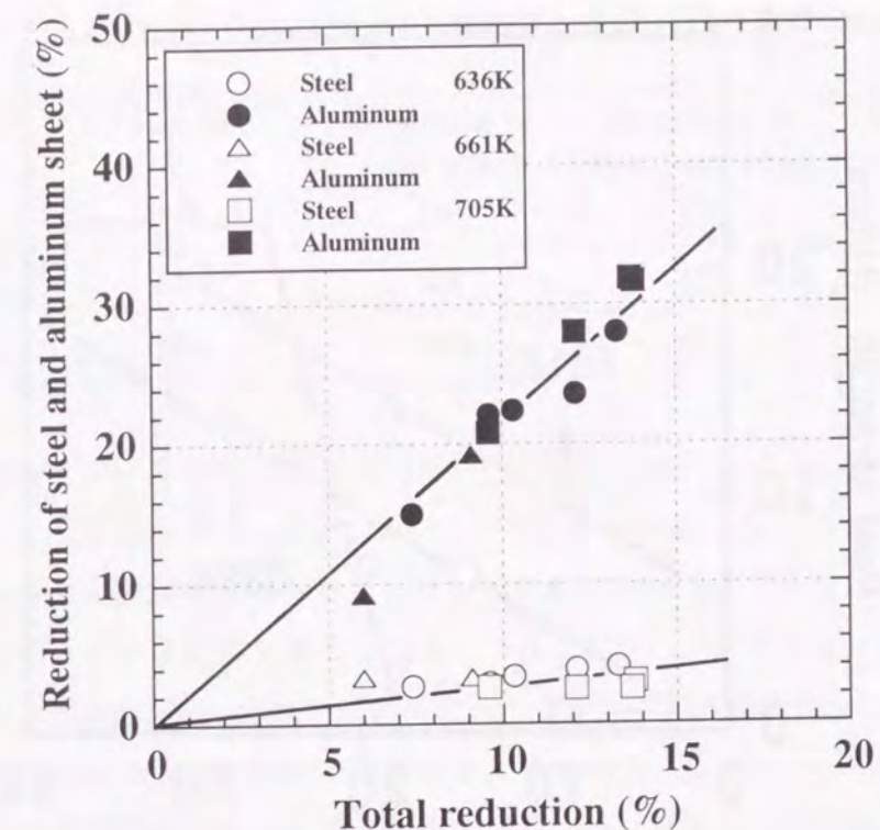
Fig. 2.5 Effects of total reduction and rolling temperature on reduction of steel and aluminum sheets.
