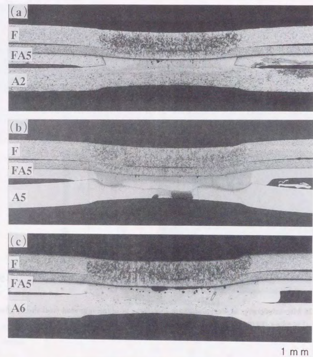
Fig. 6.25 Macrostructures of steel-aluminum clad steel-aluminum spot weld joints (12.0kA-0.2s): (a) F-FA5-A2, (b) F-FA5-A5, (c) F-FA5-A6.
