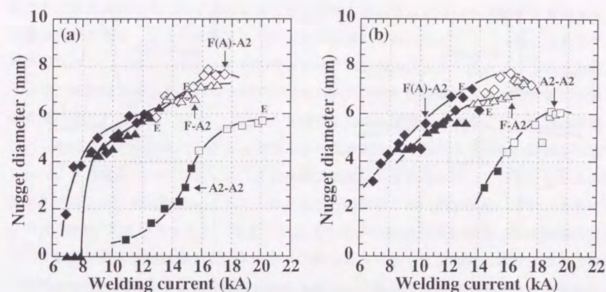
Fig. 4.16 Relation between welding current and nugget diameter of aluminum coated steel-aluminum (F(A)-A2), steel-aluminum (F-A2) and aluminum-aluminum (A2-A2) joints: (a) Tensile shear test, (b) U-tension test.
