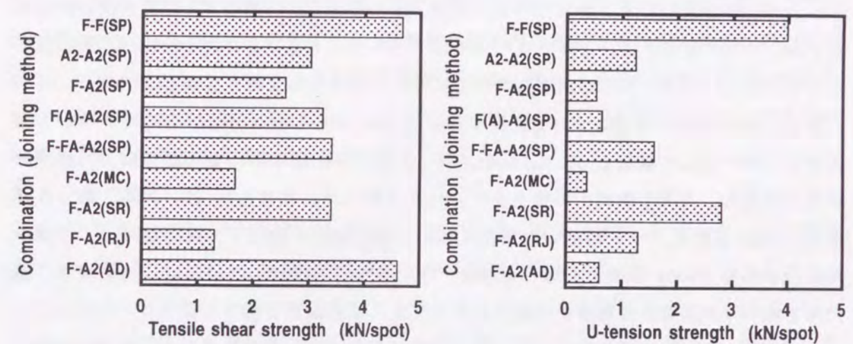
Fig. 6.70 Comparison of joint strength by various method (SP: Spot welding, MC: Mechanical clinching, SR: Self piercing & riveting, RJ: Rivet joining, AD: Adhesion bonding): (a) Tensile shear strength, (b) U-tension strength.
