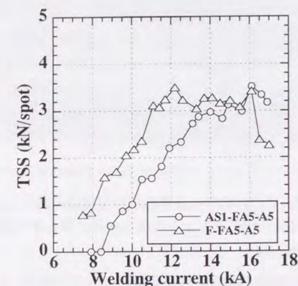
Fig. 6.34 Relation between welding current and tensile shear strength of galvanized steel-aluminum clad steel-aluminum (AS1-FA5-A5) and steel-aluminum clad steel-aluminum (F-FA5-A5) joints.
