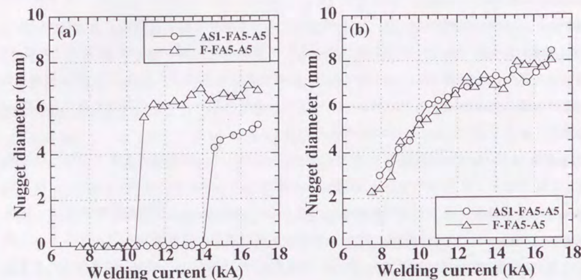
Fig. 6.35 Relation between welding current and nugget diameter of galvanized steel-aluminum clad steel-aluminum (AS1-FA5-A5) and steel-aluminum clad steel-aluminum (F-FA5-A5) joints: (a) Steel sheet side, (b) Aluminum sheet side.
