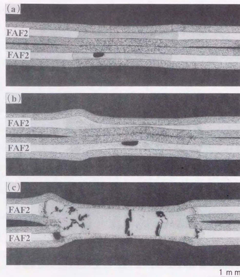
Fig. 5.23 Macrostructures of steel/aluminum laminate-steel/aluminum laminate (FAF2-FAF2) spot weld joints: (a) 7.0kA-0.2s, (b) 8.8kA-0.2s, (c) 11.3kA-0.2s.
