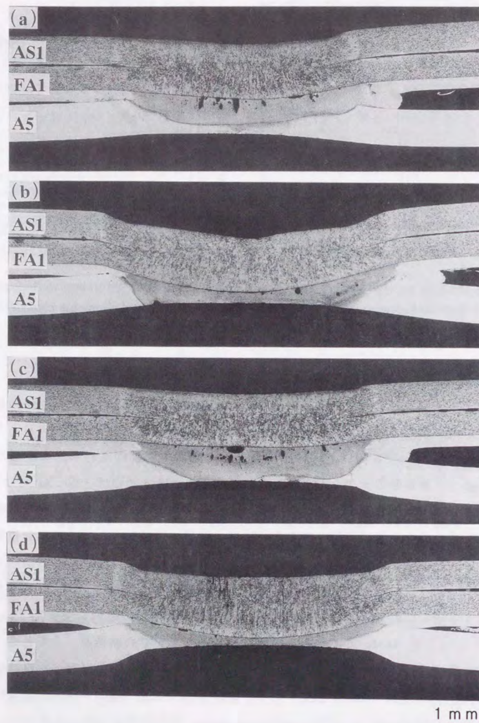
Fig. 6.47 Macrostructures of galvanized steel-aluminum clad steel-aluminum (AS1-FA1-A5) spot weld joints: (a) DR-R 10.9kA-0.2s, (b) DR-R 14.0kA-0.2s, (c) DR-DR 11.1kA-0.2s, (d) DR-DR 13.9kA-0.2s.
