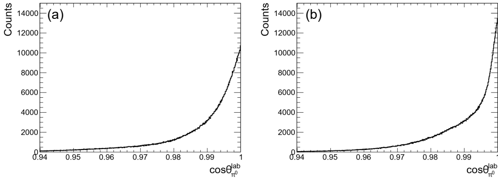
Figure 4.34: Calculated angular distributions for the {}^4_{\Lambda}\text{H} and {}^3_{\Lambda}\text{H} production via the {}^4\text{He}(K^-, \pi^0) reactions at p_{K^-} = 1.0 GeV/c. (a) This is the distribution of angles at which \pi^0 is emitted when {}^4_{\Lambda}\text{H} is produced. (b) This is the distribution of angles at which \pi^0 is emitted when {}^3_{\Lambda}\text{H} is produced. These plots were output in the simulation calculation with input of theoretical calculations by Harada et al. [44].
