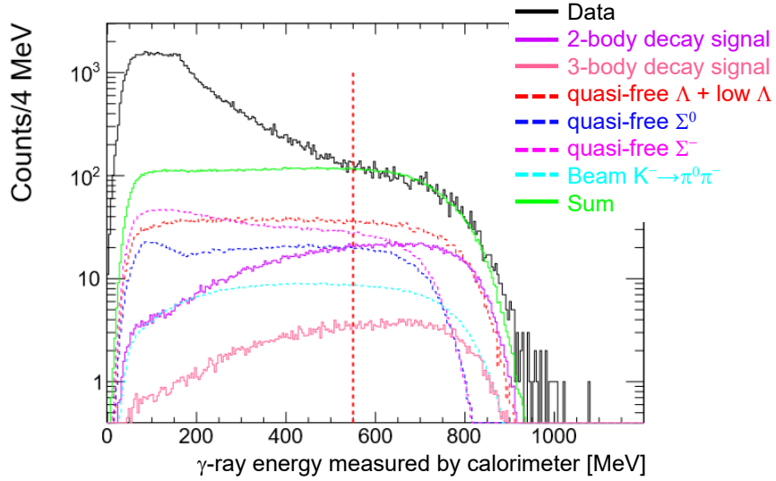
Figure 4.33: The gamma-ray energy distribution with signal and background components for the helium-3 dataset. The elements shown here are the same as in Fig. 4.31.
