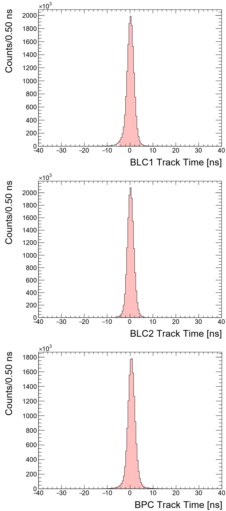
Figure 3.6: Track timing distributions of BLC1 (top), BLC2 (middle) and BPC (bottom). The timing windows of the trigger association were selected to be (-5, 5) ns and (-10, 10) ns for the BLCs and the BPC in red filled region, respectively.
