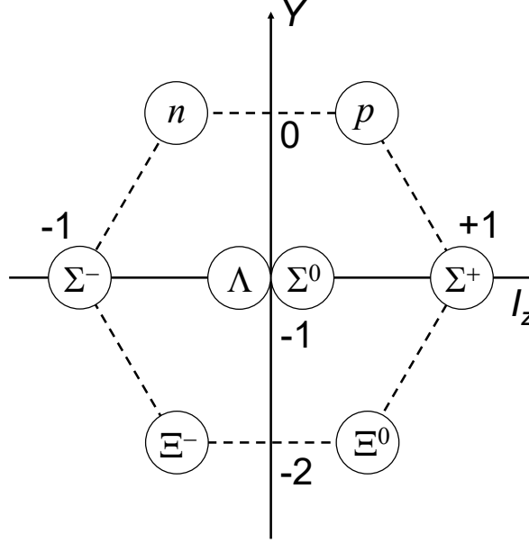
Figure 1.1: Baryon octet is a group of baryons consisting of combinations of three u, d or s quarks with a half spin and a positive parity. I_z and Y represent z component of isospin and hyper charge, respectively.
