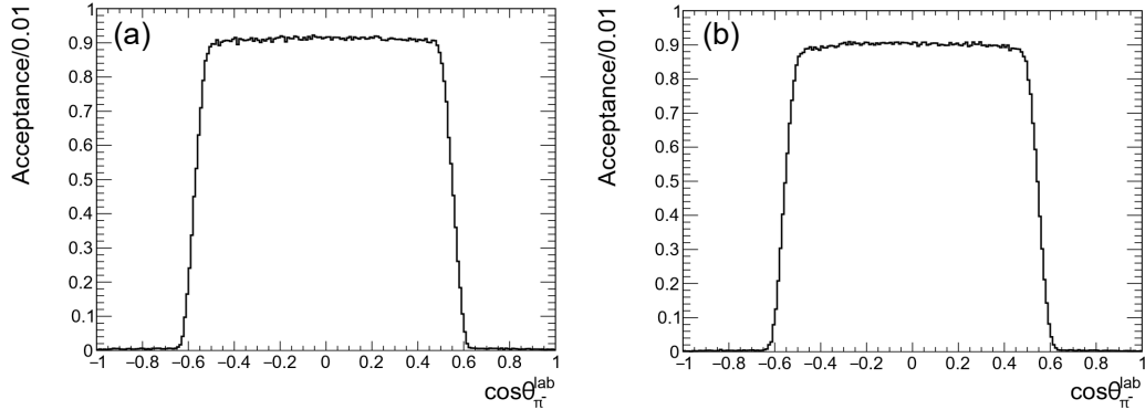
Figure 4.38: The \pi^- acceptances by CDS were estimated for \pi^- of the decay from the hypernuclei. (a) The plot displays the acceptances for two-body MWD of {}^4_\Lambda\text{H} at 133 MeV/c \pi^- detected by CDS. (b) The plot displays the acceptances for two-body MWD of {}^3_\Lambda\text{H} at 114 MeV/c \pi^- detected by CDS.
