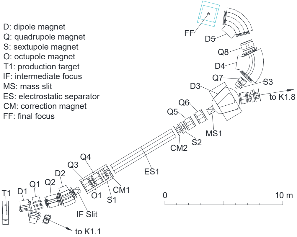
Figure 2.1: Schematic drawing of K1.8BR beam line in the J-PARC hadron experimental facility[49].
