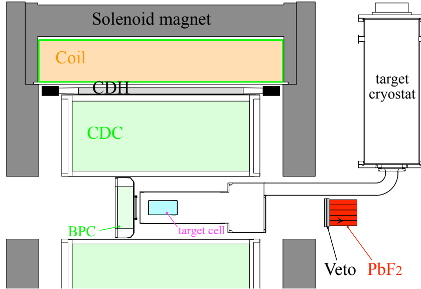
Figure 2.12: A schematic view of the Cylindrical Detector System (CDS) including the liquid helium target system[52].
