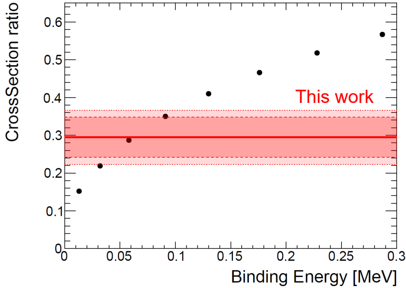
Figure 5.1: Dots show the estimation of the theoretical calculation of the production cross section ratio as a function of the binding energy of {}^3_{\Lambda}\text{H} . The horizontal red line is the value of the cross section ratio from present work, the long dashed lines shows the range of the statistical errors, and the short dashed lines shows the total errors.
