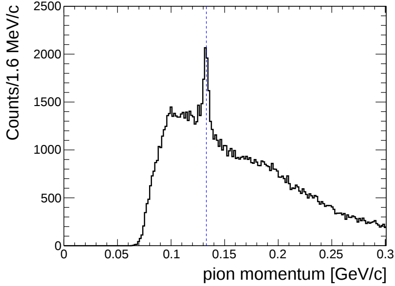
Figure 4.2: \pi^- momentum distribution for the helium-4 dataset with the physics trigger data. A clear peak at around 133 MeV/c represents the contribution of \pi^- from the two-body decay of {}^4_{\Lambda}\text{H} \rightarrow {}^4\text{He} + \pi^- .
