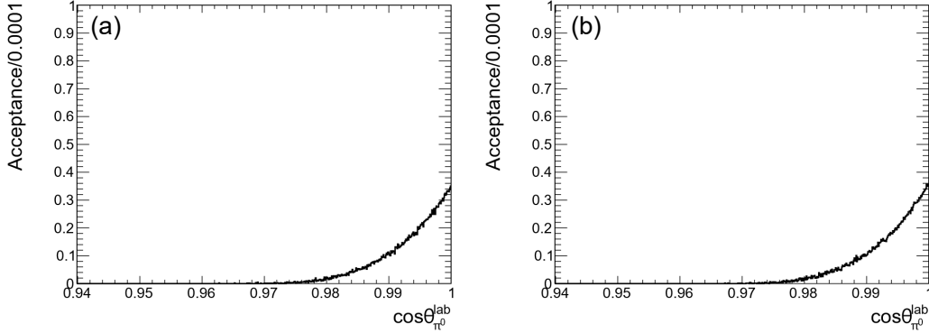
Figure 4.36: Acceptance of the PbF 2 calorimeter after selecting gamma-ray. (a) The acceptance of \pi^0 is shown when {}^4_{\Lambda}\text{H} is generated. (b) The acceptance of \pi^0 is shown when {}^3_{\Lambda}\text{H} is generated. The acceptance is the fraction of events in which the PbF 2 energy deposit is larger than 550 MeV within events that can be detected every angle.
