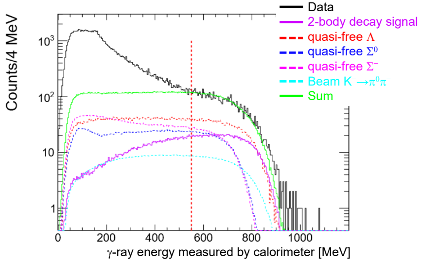
Figure 4.25: The gamma-ray energy distribution with signal and background components for the helium-4 dataset. The elements shown here are the same as in Fig. 4.23.
