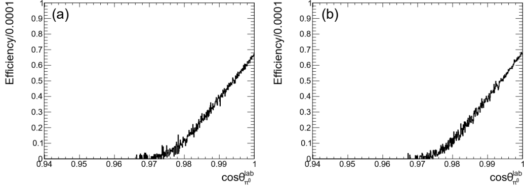
Figure 4.37: Gamma-ray selection efficiency by the PbF 2 calorimeter. (a) The efficiency of further selecting gamma-rays from the \pi^0 acceptance when {}^4_\Lambda\text{H} is generated is shown. (b) The efficiency of further selecting gamma-rays from the \pi^0 acceptance when {}^3_\Lambda\text{H} is generated is shown. The efficiency is the fraction of events in which the PbF 2 energy deposit is larger than 550 MeV.
