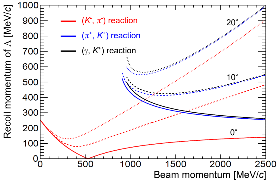
Figure 1.5: The momentum transfer from beam K^- to \Lambda as a function of the beam momentum. There are nine lines in combination of three reactions (red: ( K^- , \pi^- ), blue: ( \pi^+ , K^+ ) and black: ( \gamma , K^+ )) and three different opening angles between beam and scattering particle in the laboratory system ( 0^\circ : solid line, 10^\circ : dashed line and 20^\circ : dotted line). In the ( K^- , \pi^- ) reaction, the recoil momenta have minimum values around 500 MeV/c. In particular, at the forward angle ( 0^\circ ) in the ( K^- , \pi^- ) reaction, the magic momentum, at where the recoil \Lambda momentum is zero, exists around 500 MeV/c.
