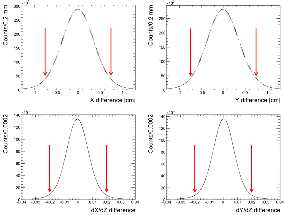
Figure 3.9: (top) The difference in position between the tracks extrapolated from BPC and BLC2 is evaluated at a point 73 cm upstream of final focus point, which corresponds to the midpoint between BLC2 and BPC. In each histogram, the acceptable range is shown by two red vertical arrows. The differences in the x and y positions are chosen to be within a range from -0.75 to 0.75 cm. (bottom) The differences in the angles dx/dz and dy/dz are limited to a range from -0.02 to 0.02.
