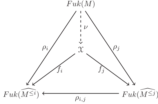
Fig. 12. Restriction functor diagram
