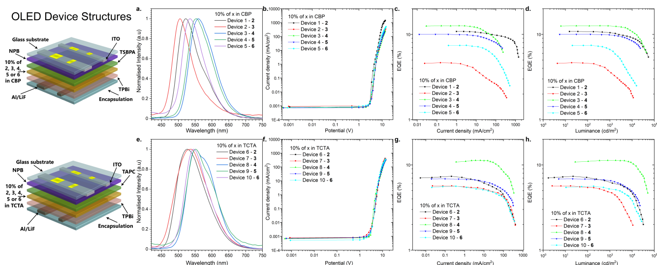
Fig. 5 The characteristics of the OLED devices. a), e) Electroluminescence spectra. b), f) Current density-bias characteristics. c), g) EQE-current density characteristics. d), h) EQE - luminance characteristics.
