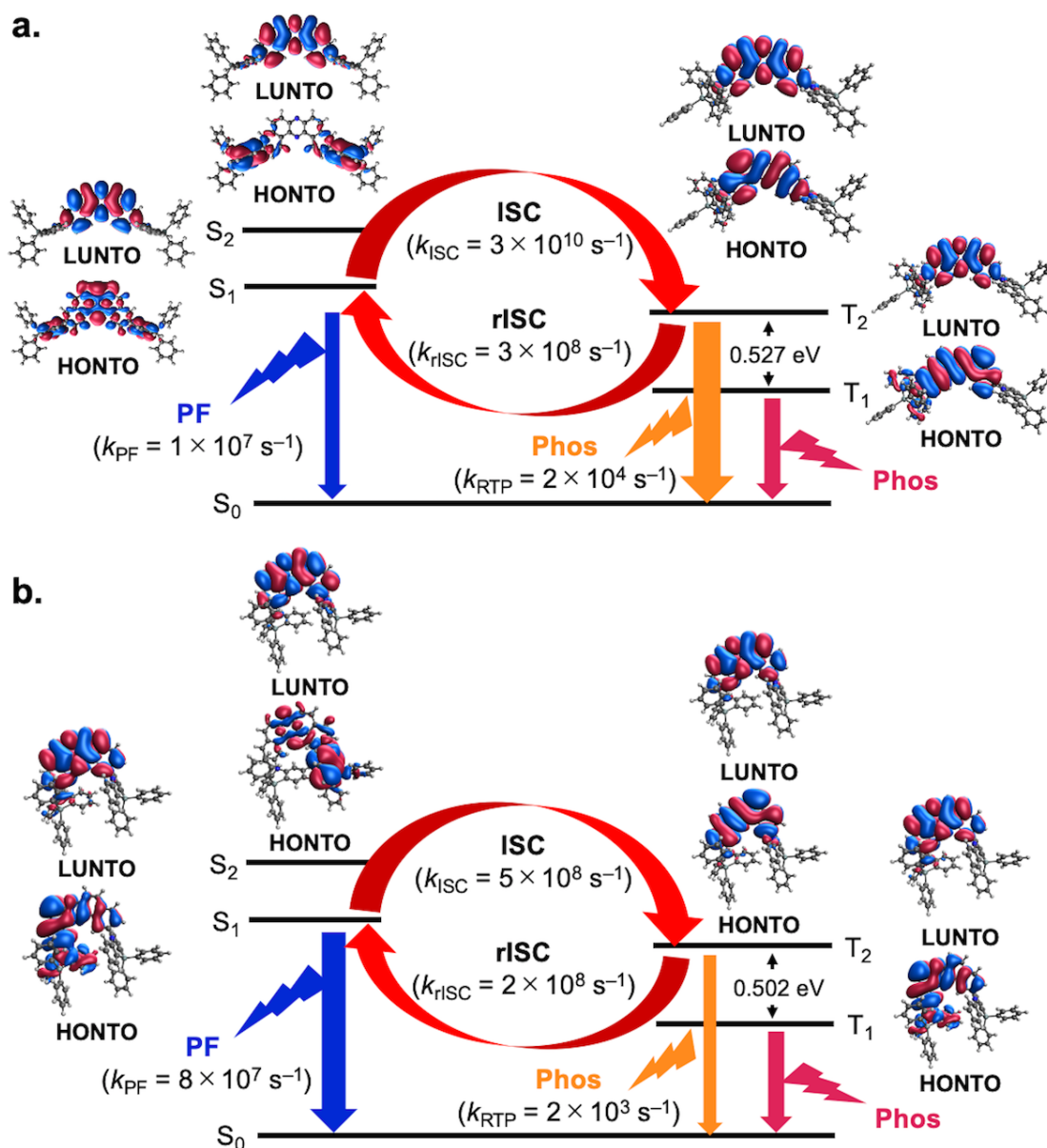
Fig. 6 Schematics showing the NTOs for the first two singlet and triplet states as well as rate estimates for different photophysical processes for compounds a) 1 and b) 4 . ISC rates correspond to the sum of rates from S_1 to the first 5 triplet states.
