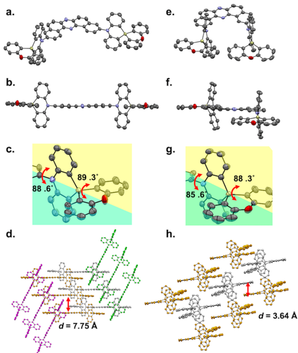
Fig. 2 The ORTEP drawings of 3 and 6 obtained by the X-ray crystallographic analysis (thermal ellipsoids set at 50% probability; hydrogen atoms are omitted for clarity). a) Molecular structure, b) side view, c) an enlarged view of the donor, and d) packing structure of 3 ; e) Molecular structure, f) side view, g) an enlarged view of the donor, and h) packing structure of 6 .
