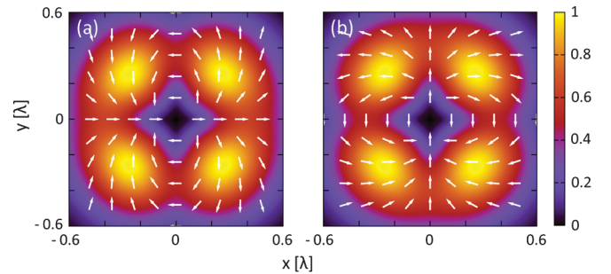
FIG. 2 (color). The distributions of the amplitudes (colors) and directions (white arrows) of (a) the polarization \mathbf{P} and (b) the magnetization \mathbf{M} described by Eq. (3) in the focal plane for \theta = 100^\circ . The amplitudes of \mathbf{P} and \mathbf{M} are given by \sqrt{\langle|\mathbf{P}|^2\rangle} and \sqrt{\langle|\mathbf{M}|^2\rangle} , respectively. The x and y axes are expressed in units of the laser wavelength \lambda . The amplitudes are normalized to the peak value.
