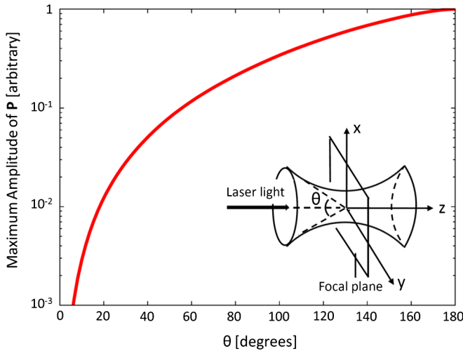
FIG. 3 (color online). Angular aperture dependence of the maximum amplitude of the polarization \mathbf{P} in the focal plane under a fixed laser intensity, and geometric configuration of the incident laser light. The maximum amplitude of \mathbf{P} is equal to that of the magnetization \mathbf{M} . The amplitude is normalized to the value for \theta = 180^\circ .
