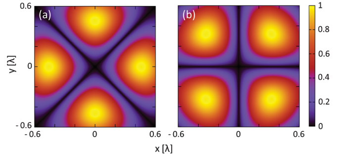
FIG. 1 (color). The distributions of the Lorentz invariants (a) |\langle\mathcal{F}\rangle| and (b) |\langle\mathcal{G}\rangle| of the focused laser beam in the focal plane for \theta = 100^\circ . The x and y axes are expressed in units of the laser wavelength \lambda . The Lorentz invariants are normalized to the peak value.
