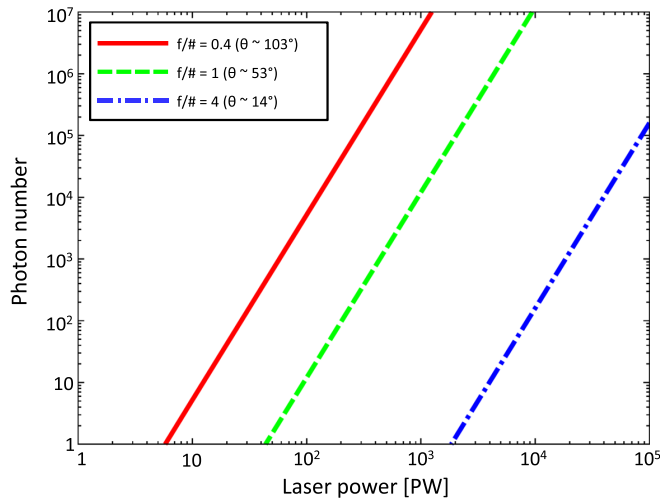
FIG. 5 (color online). The number of the radiated photons polarized perpendicular to the incident laser light per shot as a function of the laser power for \tau = 100 fs.
