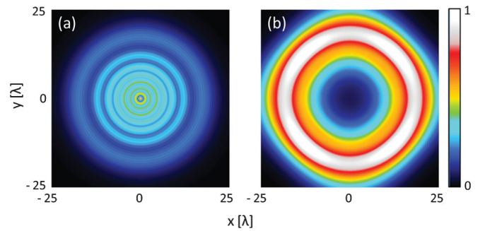
FIG. 4 (color). The intensity distributions of (a) the focused laser beam with no interaction with vacuum and (b) the electromagnetic field radiated from the vacuum irradiated by a focused beam in the plane located 20\lambda = 20 \mu\text{m} from the focal plane in the propagation direction of the incident laser beam. The f number is assumed to be 0.4 (i.e., \theta \simeq 103^\circ ). The peak intensities of the focused light and the radiated field are about 10^{22} \text{ W/cm}^2 and 10^4 \text{ W/cm}^2 for a laser power of 100 PW, respectively. The intensities are normalized to their peak values.
