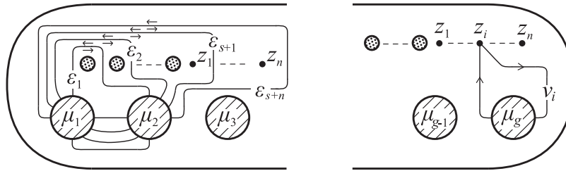
Fig. 3. Circles \varepsilon_1, \varepsilon_2, \dots, \varepsilon_{s+n} and paths v_1, \dots, v_n .
